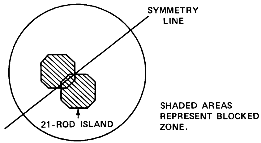
Figure 4-4. Partial Blockage-Bypass Cases
