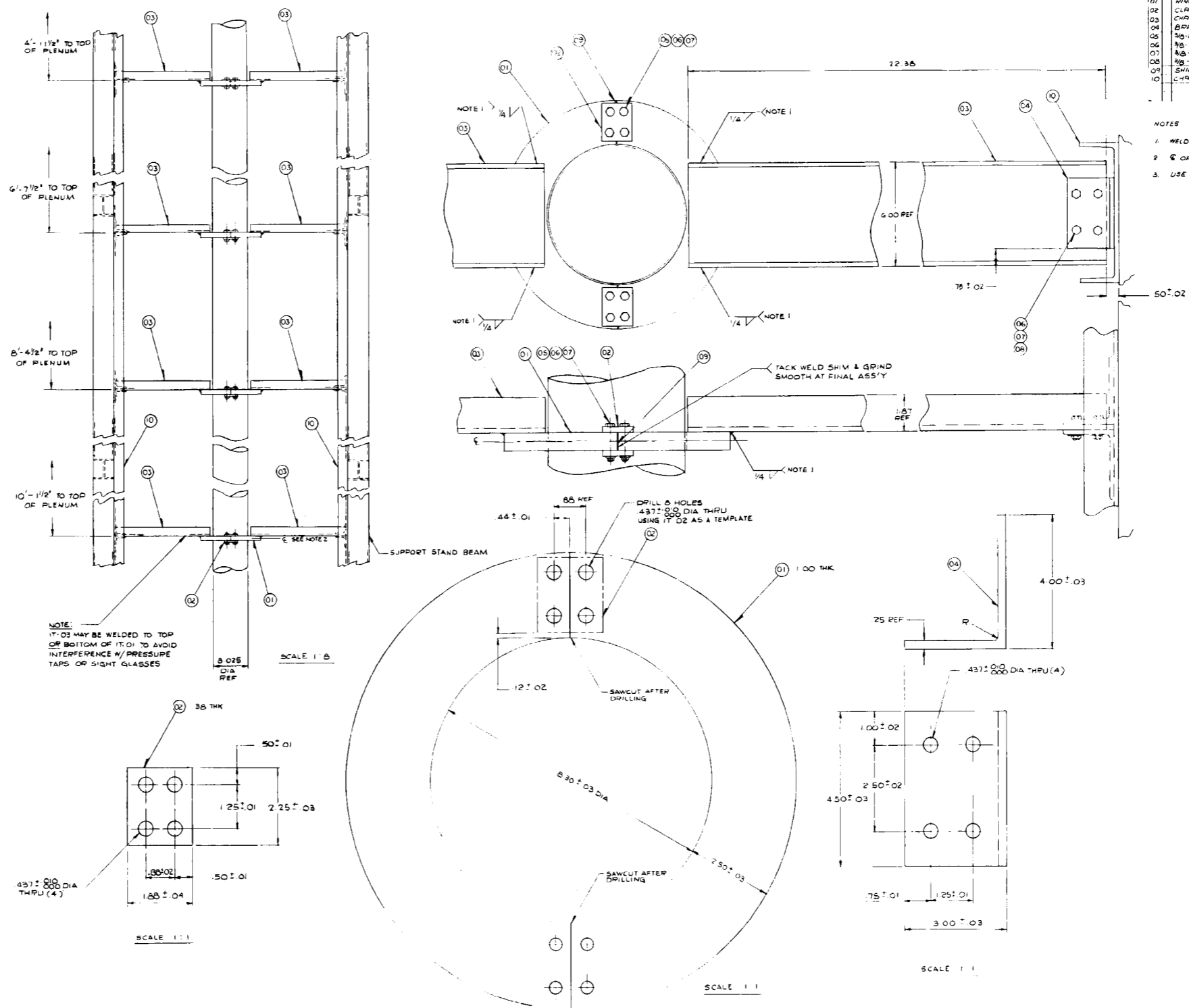
Figure B-6. FLECHT SEASET 161-Rod Blocked Bundle Facility Housing Lateral Brace
