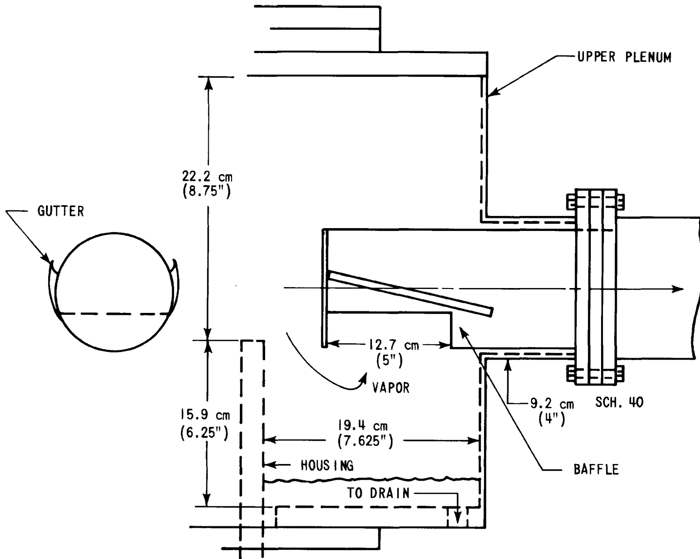
Figure 6-6. FLECHT SEASET Upper Plenum Baffle
