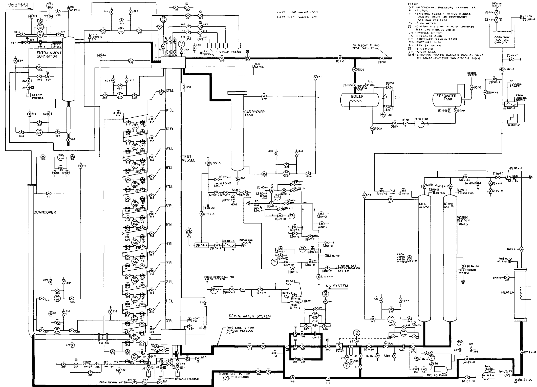
Figure 6-1. Forced and Gravity Reflood Configuration Flow Diagram
