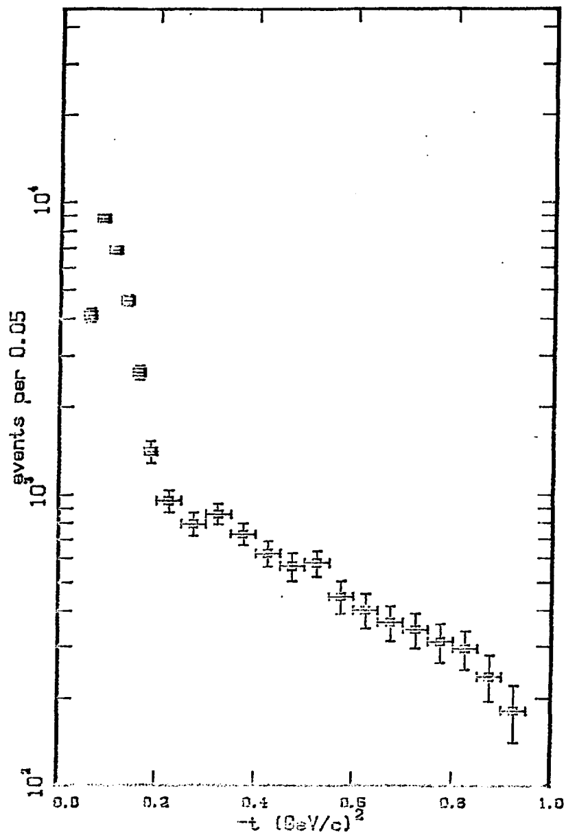
Fig. 4. The t distribution for events with w_p mass less than 1.9 GeV.
