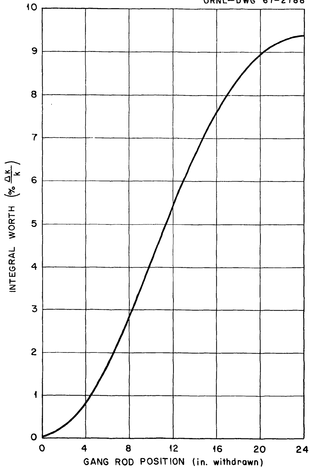
Fig. 4.15. Integral worth of shim-safety rods 1 through 4.
