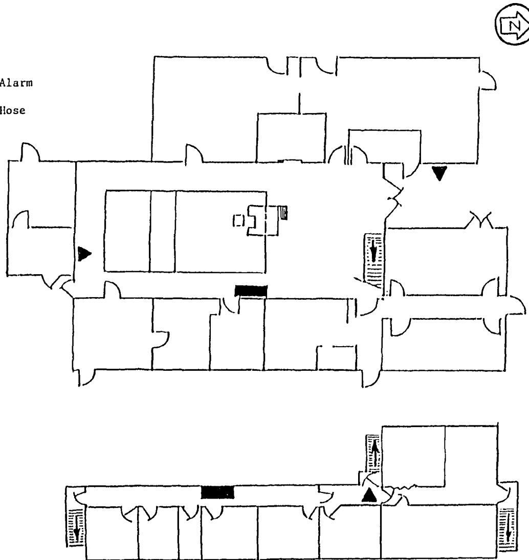
Fig. 9.2. Fire protection equipment.
