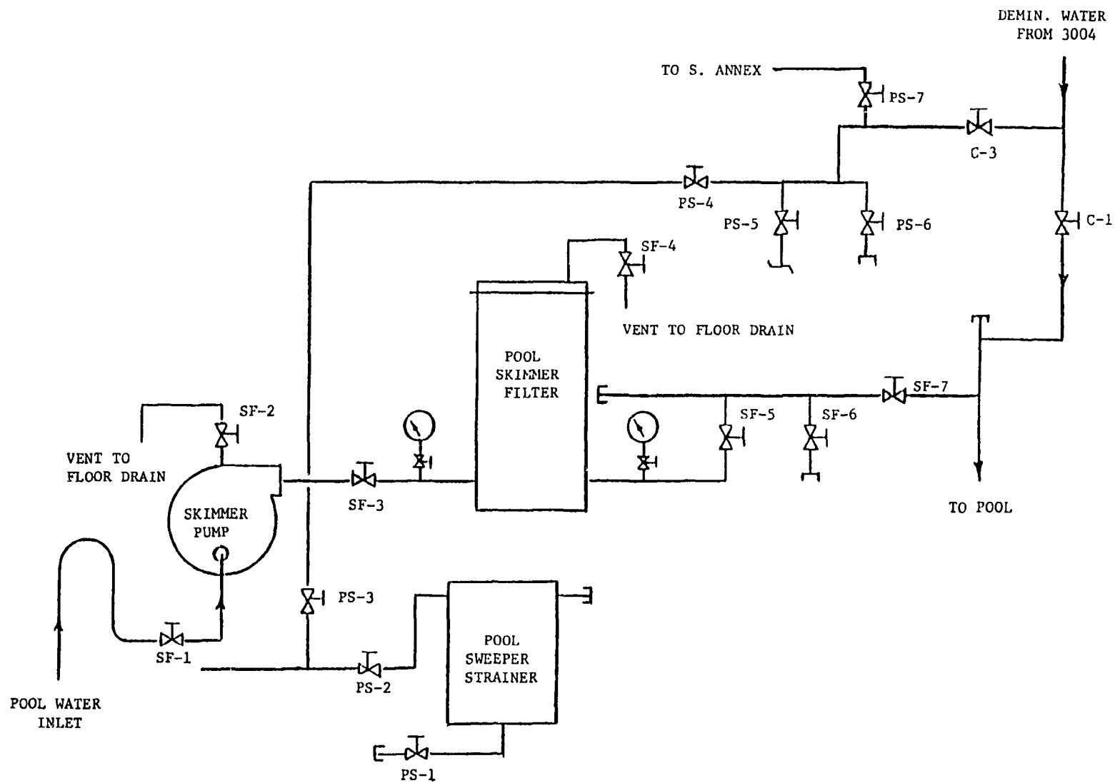
Fig. 6.6. BSR pool skimmer filter and pool sweeper strainer systems.
