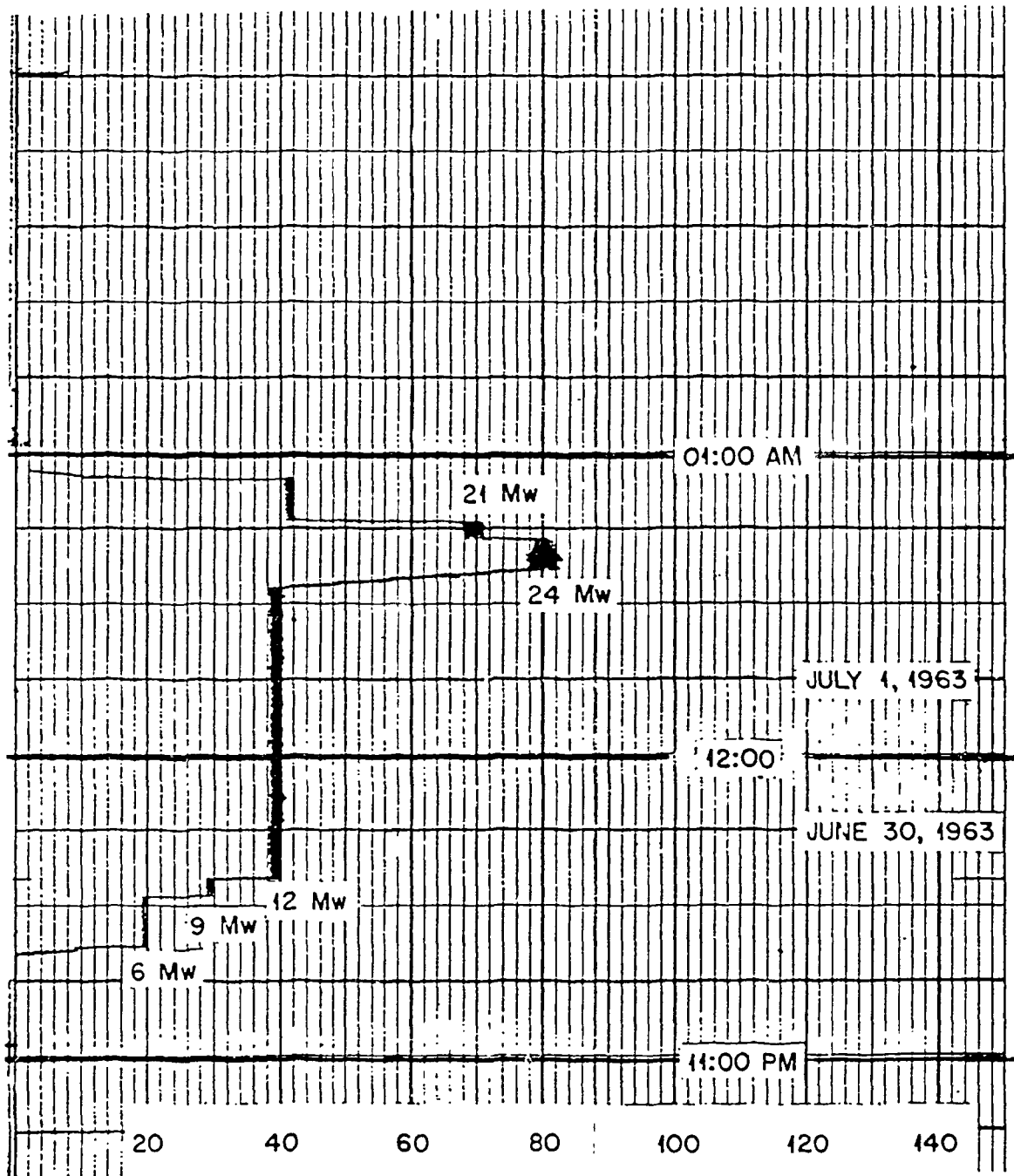
Fig. 2.9. ORR No. 1 safety channel.
