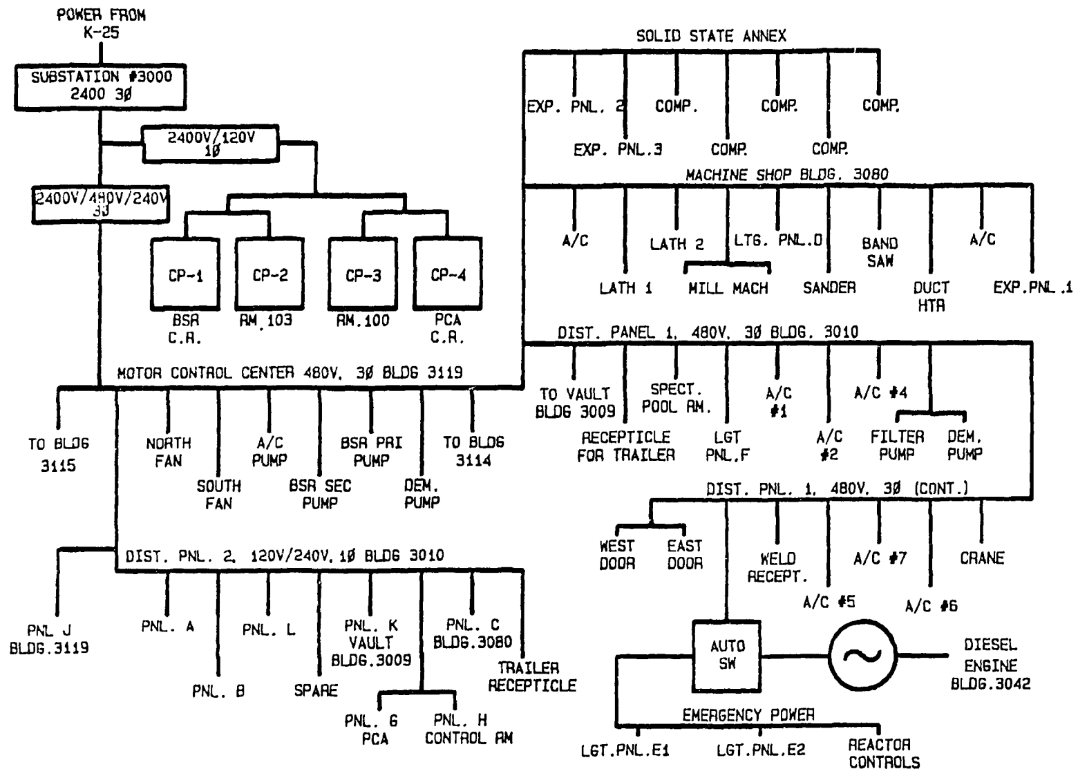
Fig. 8.5. BSR electrical one-line diagram.
