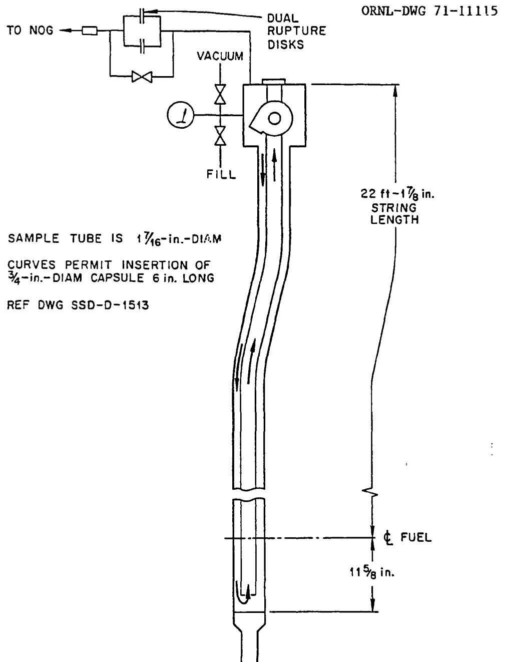
Fig. 5.6. Ambient-Temperature Neutron Irradiation Facility, ATNIF.
