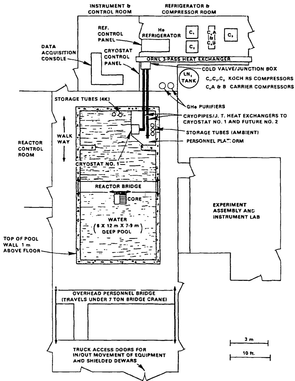
Fig. 5.7. Layout plan for LTNIF at ORNL's Bulk Shielding Reactor.
