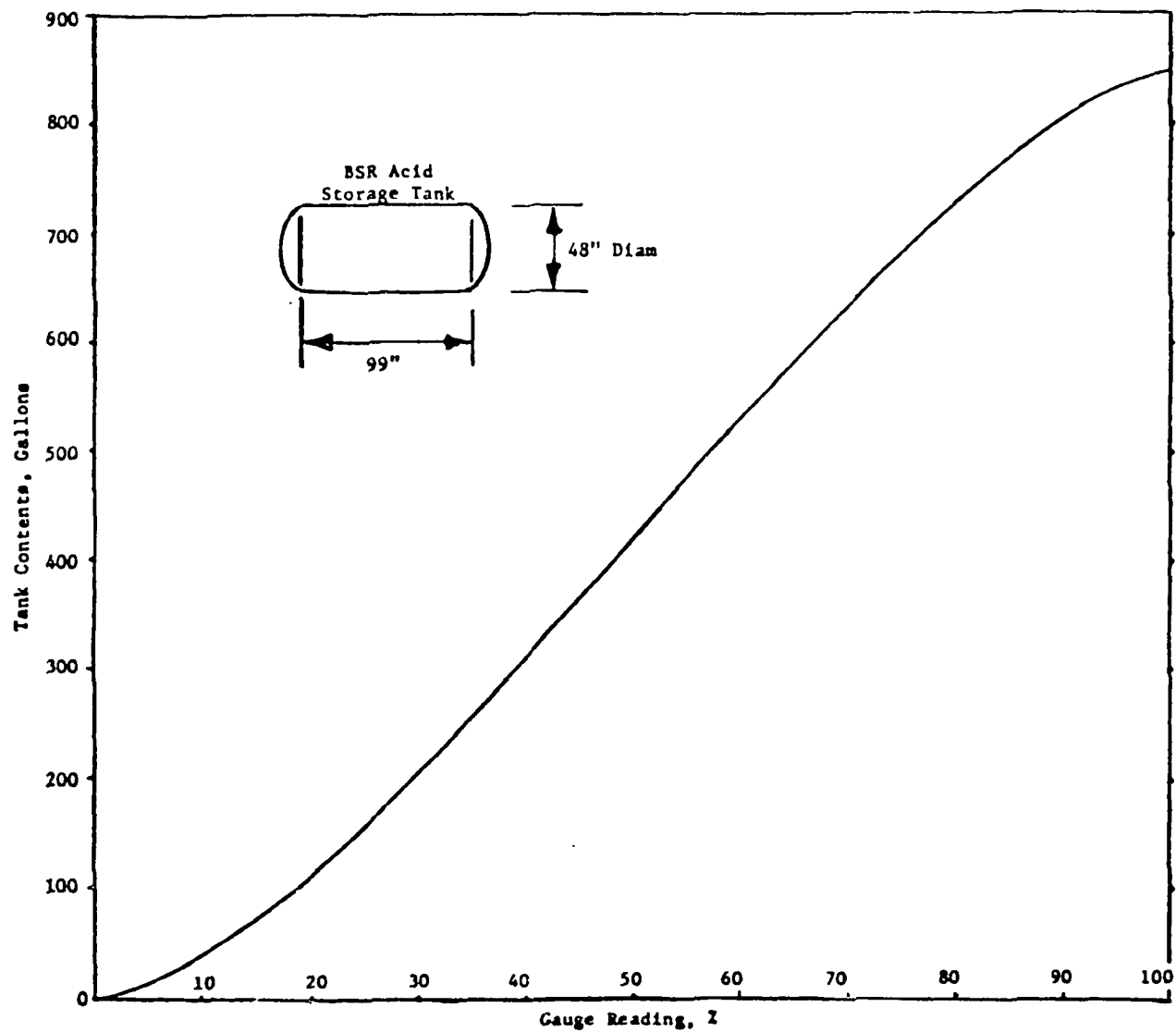
Fig. 11.5. BSR acid storage tank.
