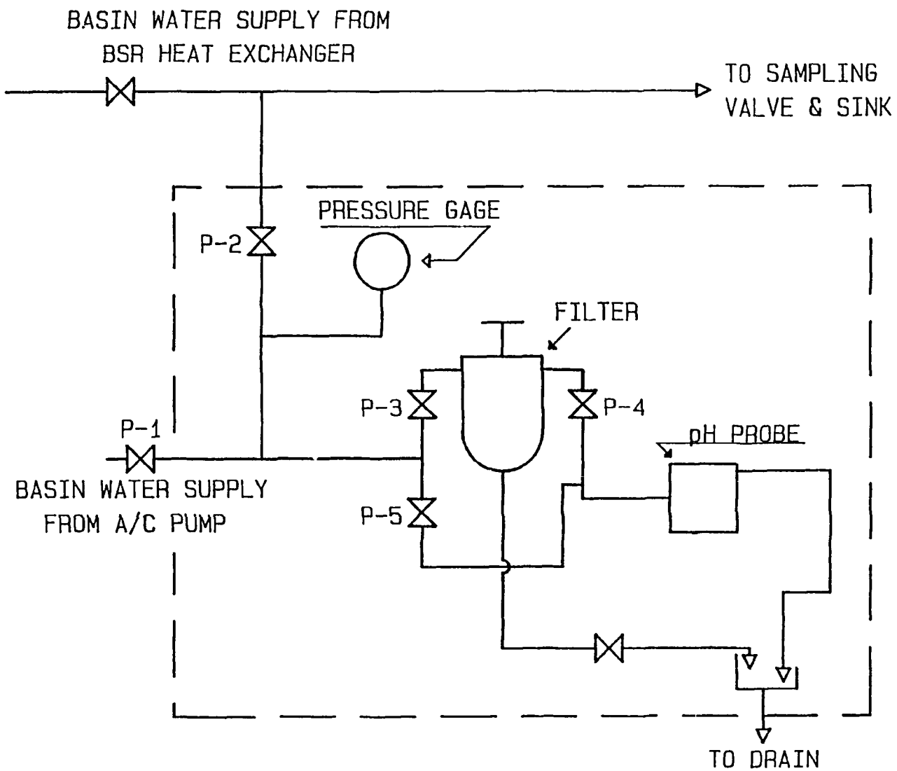
Fig. 6.9. BSR secondary pH control probe.
