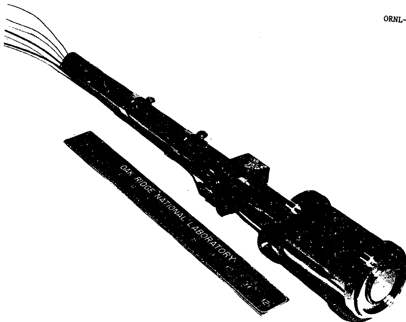
Fig. 4.7. Electromagnet for BSR-PCA shim-safety rod.
