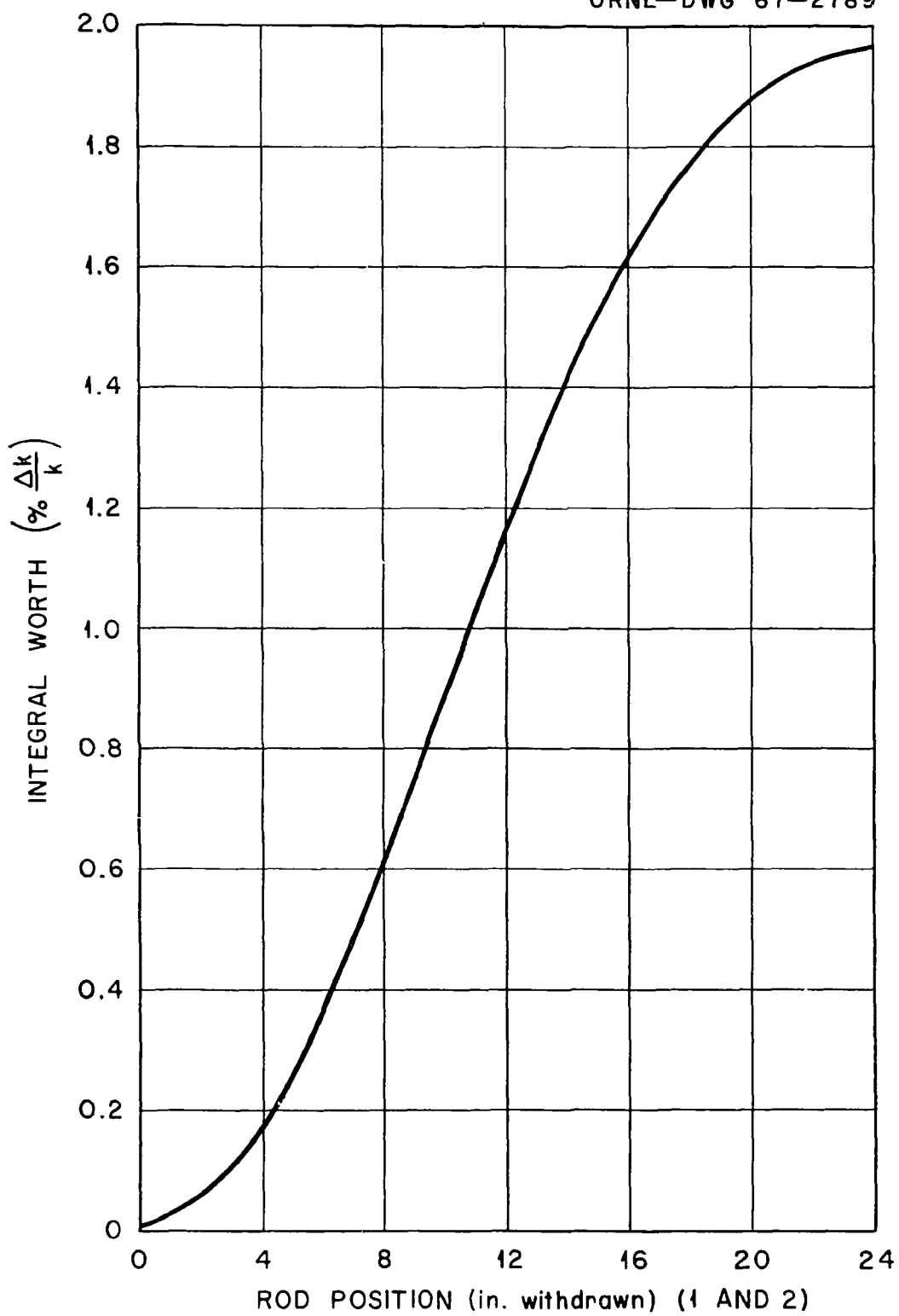
Fig. 4.16. Integral worth of shim-safety rods 5 and 6.
