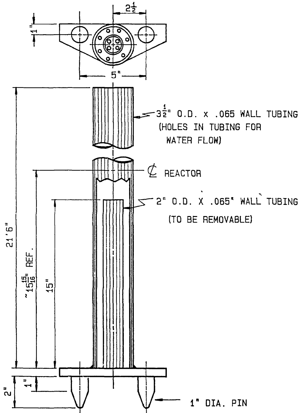
Fig. 5.5. North face irradiation facility.
