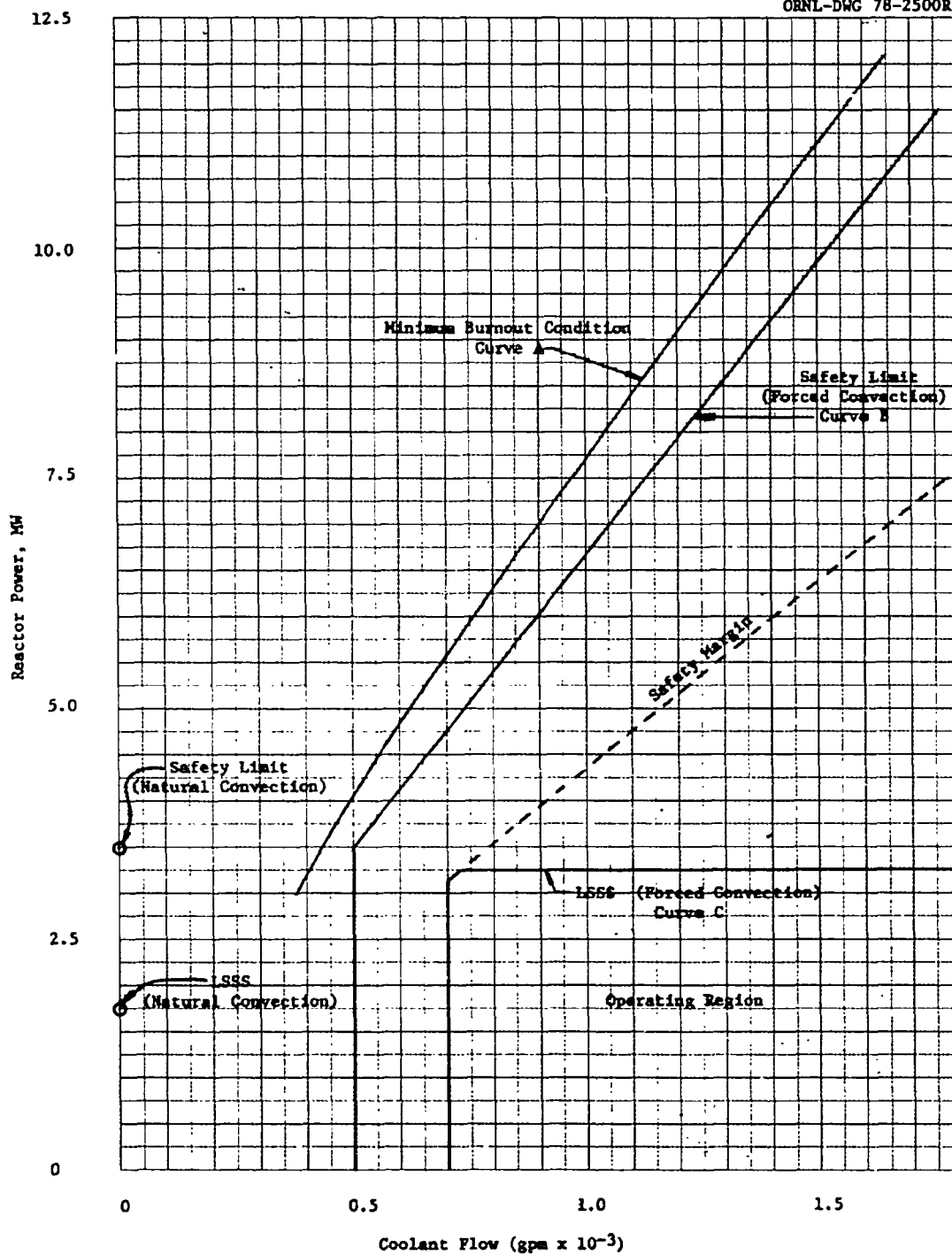
Fig. 16.1. Safety limits and limiting safety system settings for the BSR.
