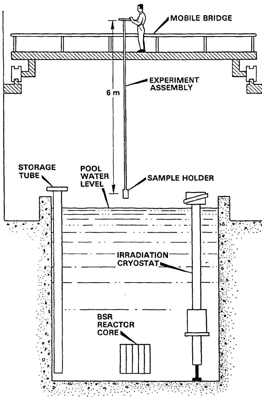
Fig. 11.4. A schematic view of the personnel bridge which is used to transfer radioactive specimens.
