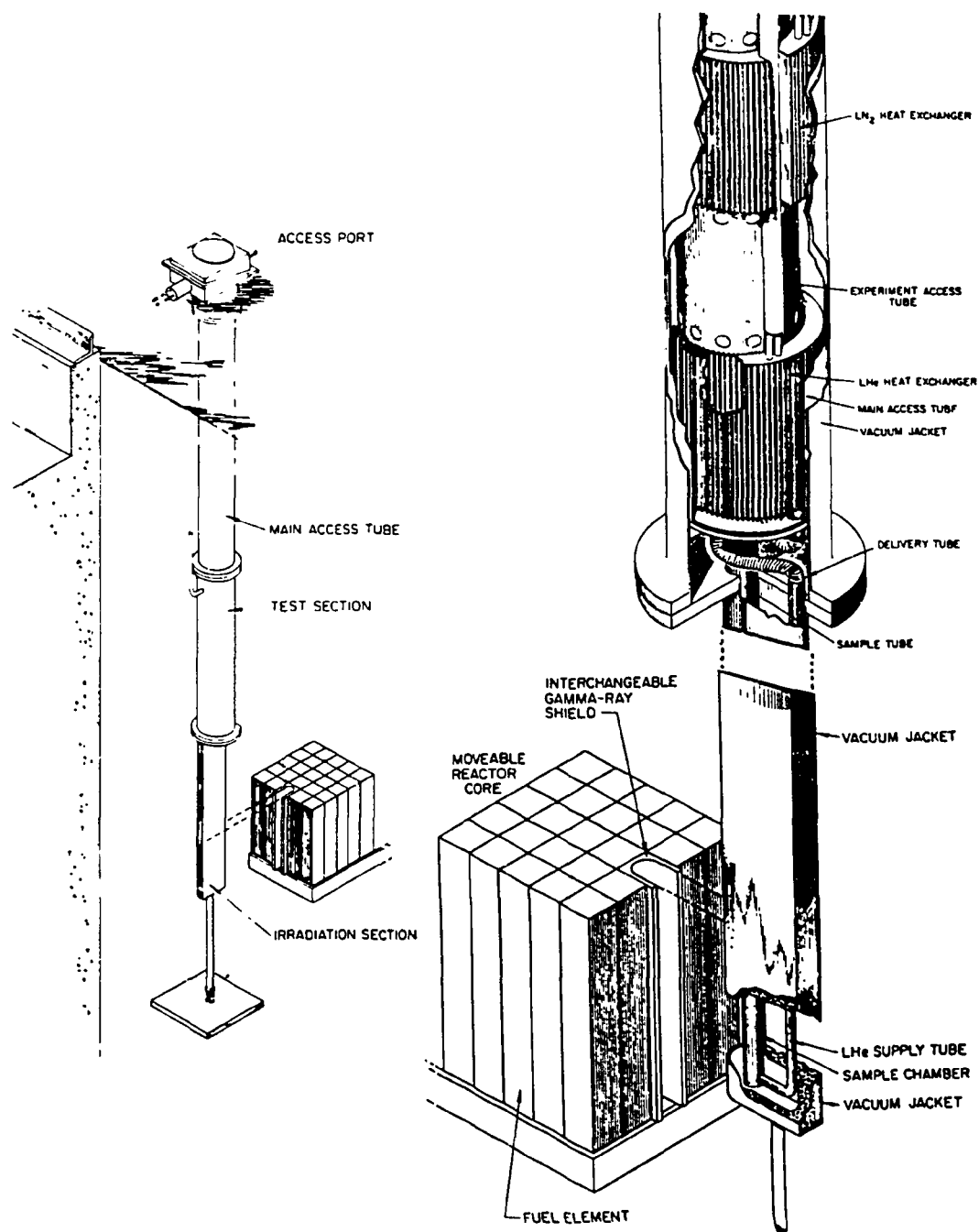
Fig. 5.8. The irradiation cryostat.
