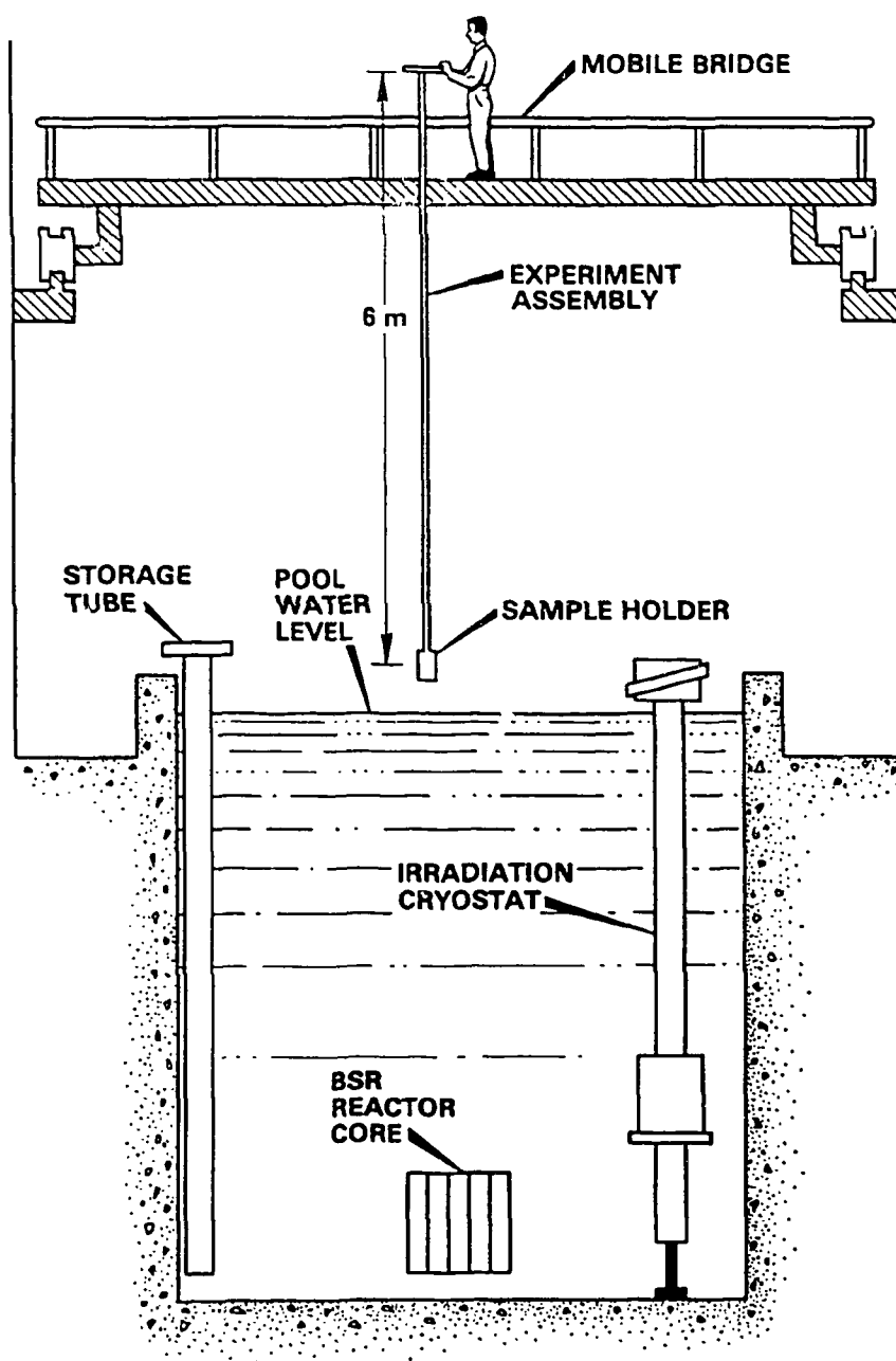
Fig. 5.9. A schematic view of the mobile catwalk bridge which is used to transfer radioactive specimens.
