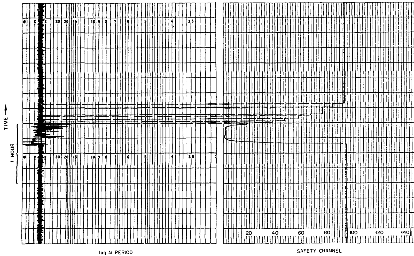
Fig. 2.10. ORR normal start-up (recorder charts of normal startup to 30 MW).
