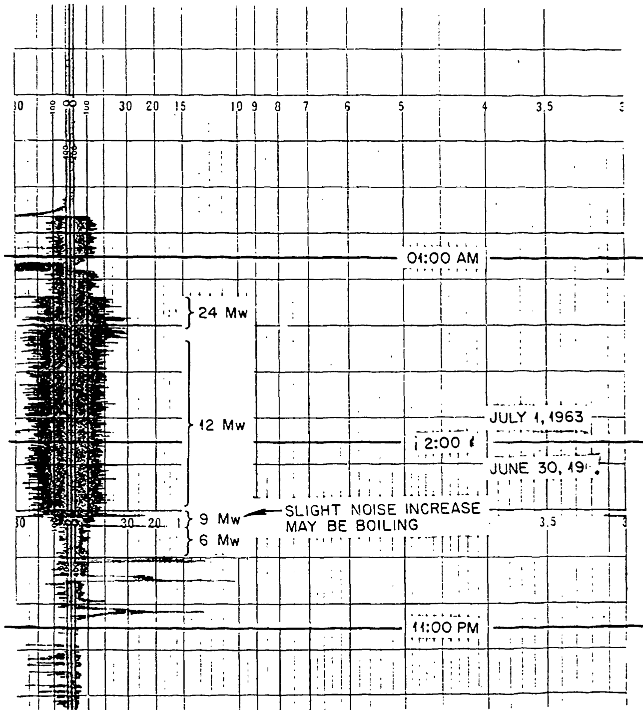
Fig. 2.8. ORR No. 1 log N period.
