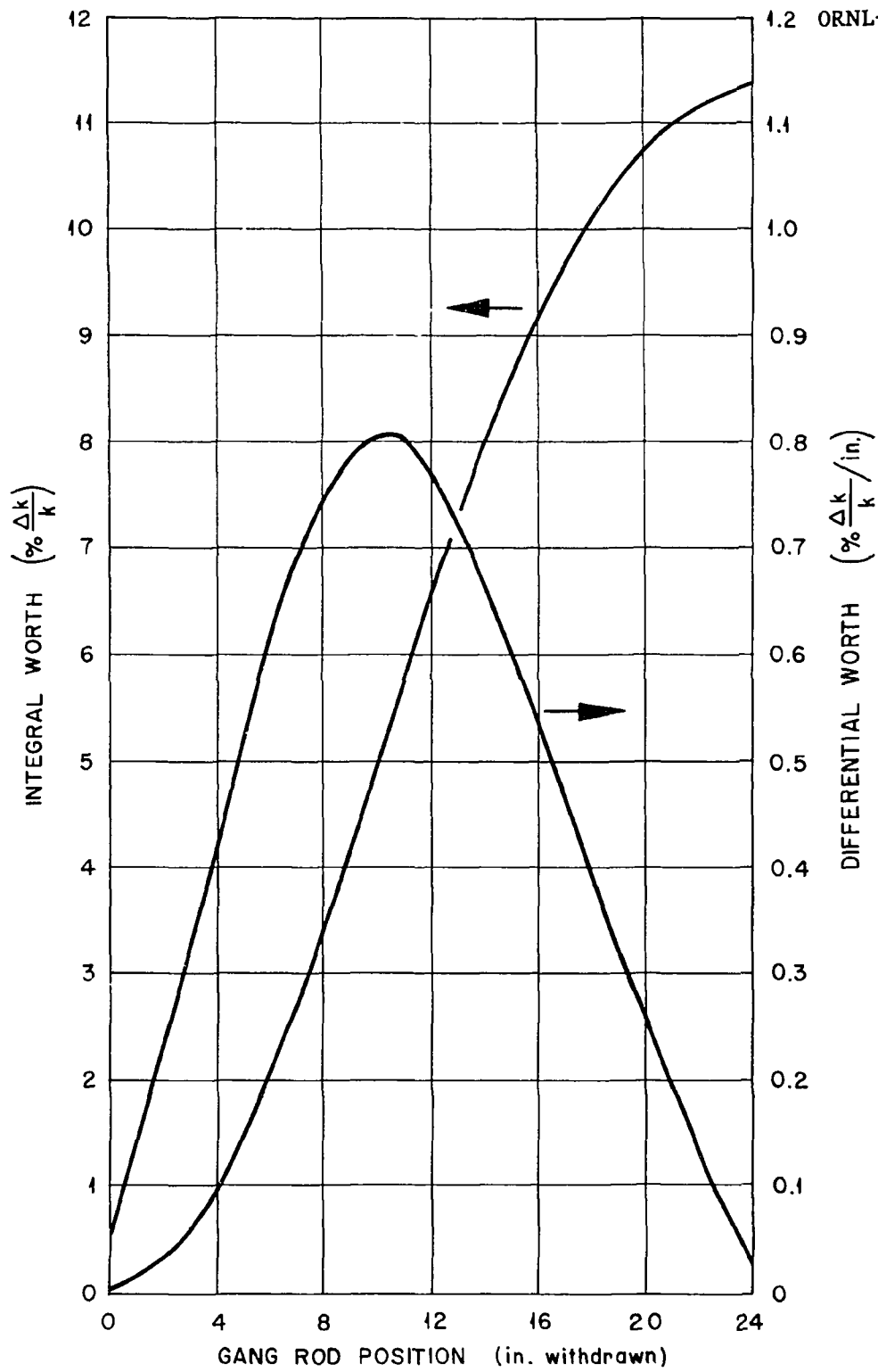
Fig. 4.14. Differential and integral worths of shim-safety rods 1 through 6.
