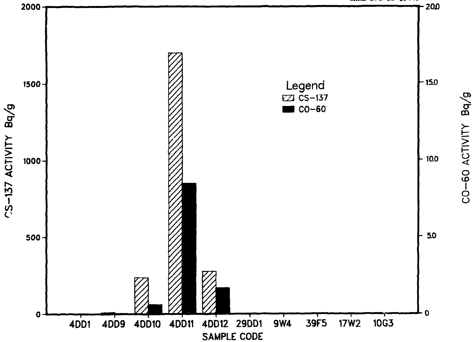
Figure 9. Gamma activities of 137 Cs and 60 Co in selected samples
