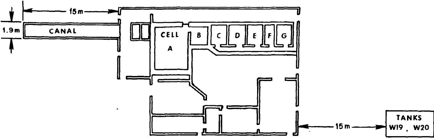
Figure 2. Building 3505 Floor Plan
