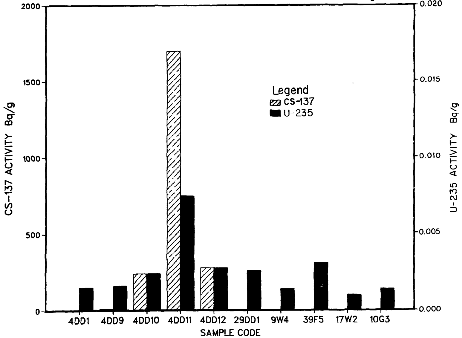
Figure 10. Gamma activities of ^{137}\text{Cs} and alpha activities of ^{235}\text{U} in selected samples
