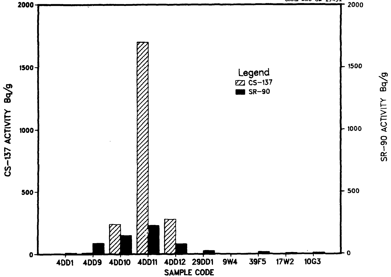
Figure 11. Gamma activities of 137 Cs and beta activities of 90 Sr in selected samples
