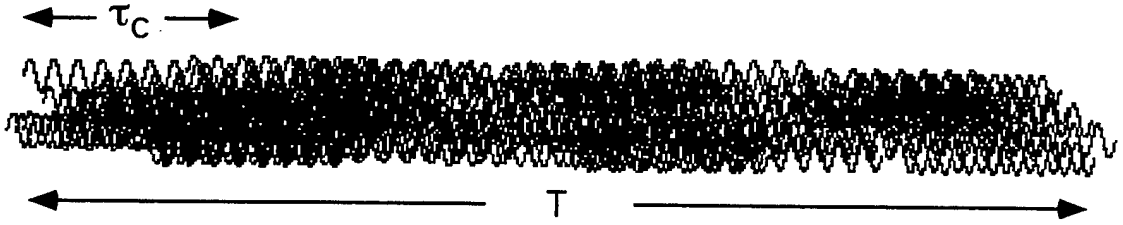
FIGURE 1. An example of chaotic light given by a random superposition of 100 sinusoidal wave packets each with six periods long. The total length of the pulse is T .
