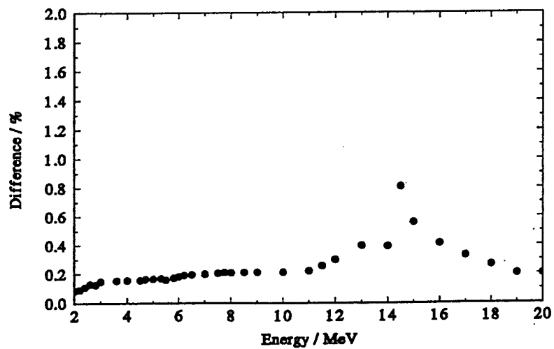
Fig. 6. Differences for ^{239}\text{Pu}(\text{n},\text{f})
