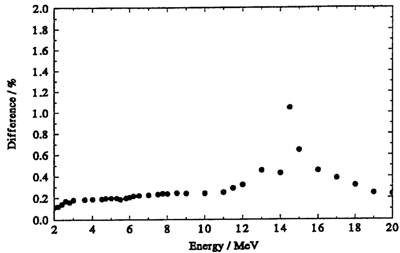
Fig. 5. Differences for ^{235}\text{U}(\text{n},\text{f})
