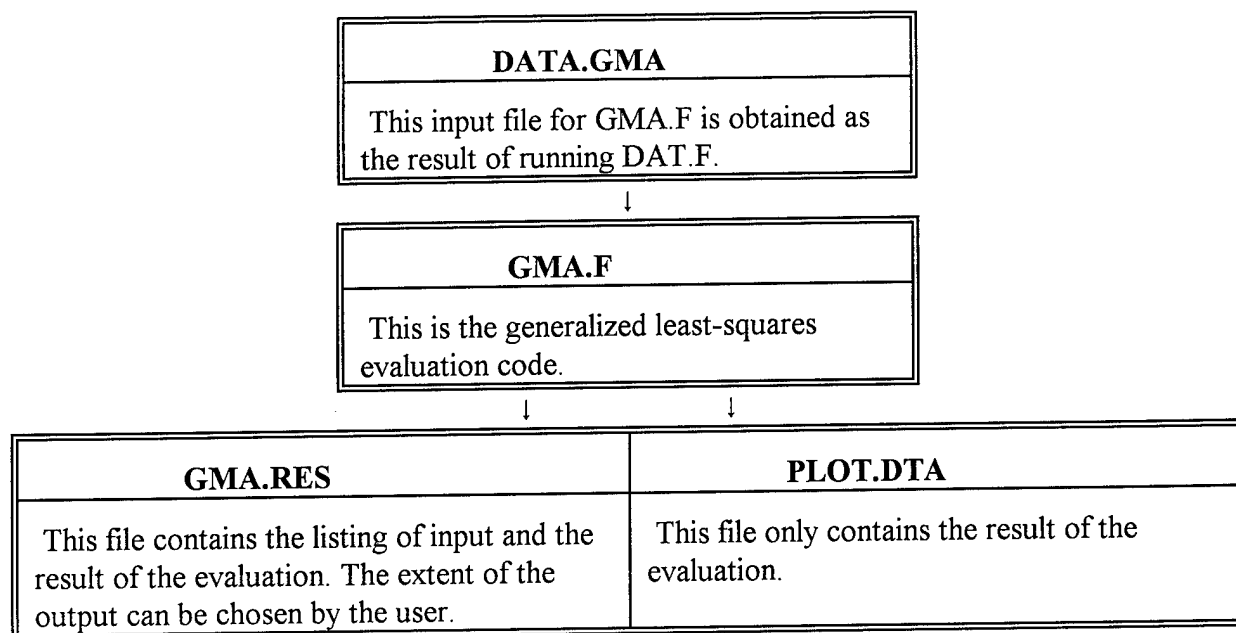
Fig. 4. The FORTRAN Code GMA.F and its Input and Output Files.
