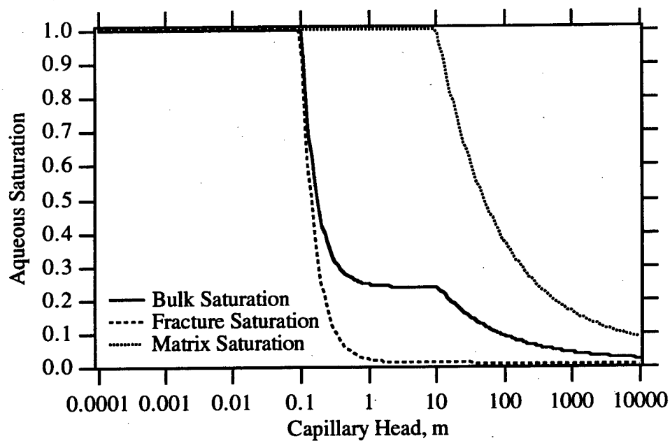
Figure 4.21. Brooks and Corey Dual Porosity Saturation Function
