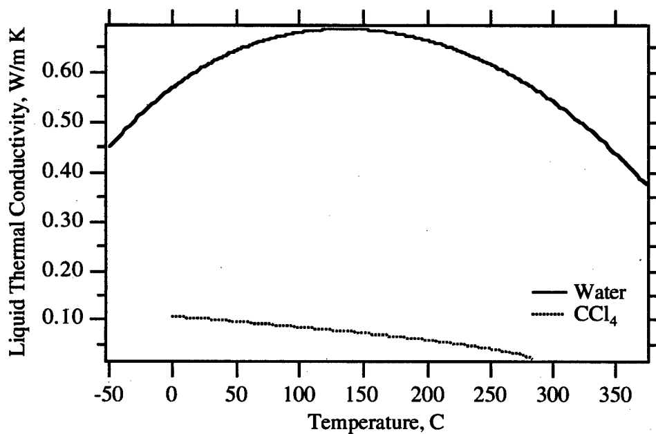
Figure 4.16. Saturated Liquid Thermal Conductivity for Water and Carbon Tetrachloride
