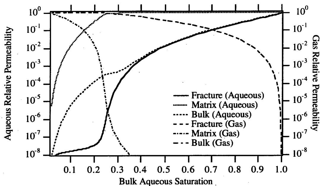
Figure 4.29. Dual Porosity Relative Permeability Function with Burdine Relative Permeability and van Genuchten Soil-Moisture Retention
