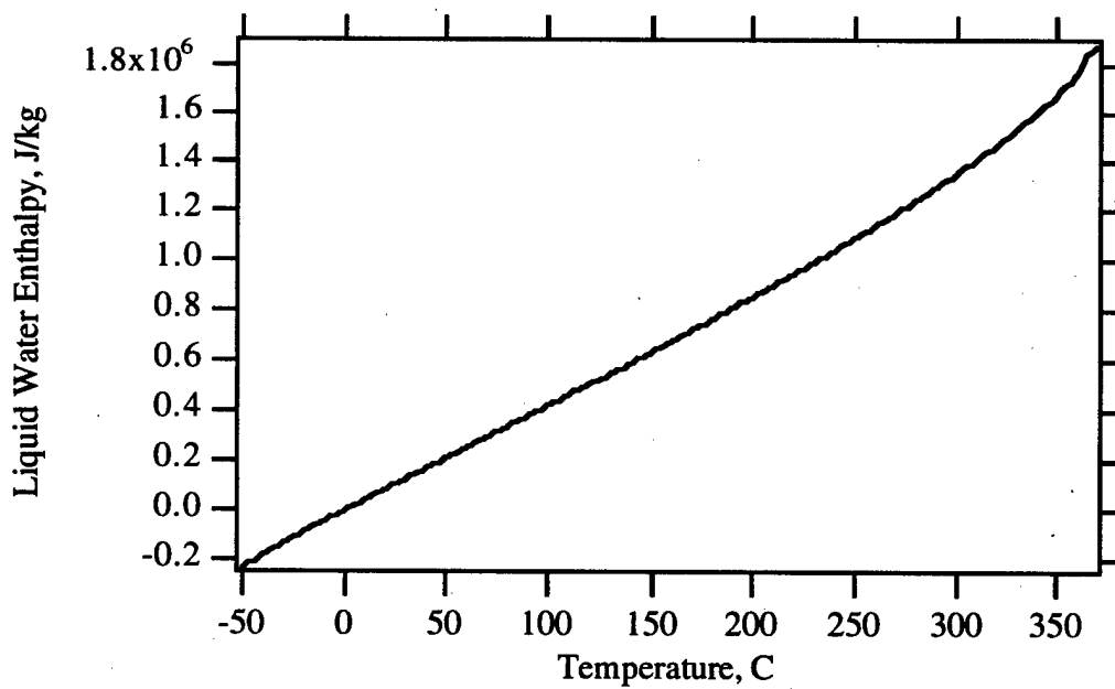
Figure 4.12. Saturated Liquid Enthalpy for Water
