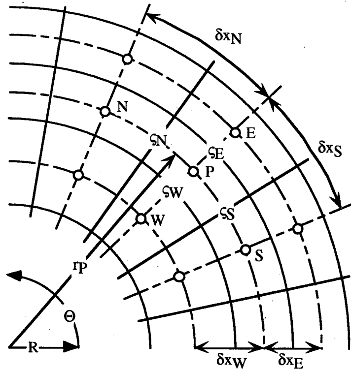
Figure 6.4. R- \Theta Coordinate Plane for Cylindrical Systems
