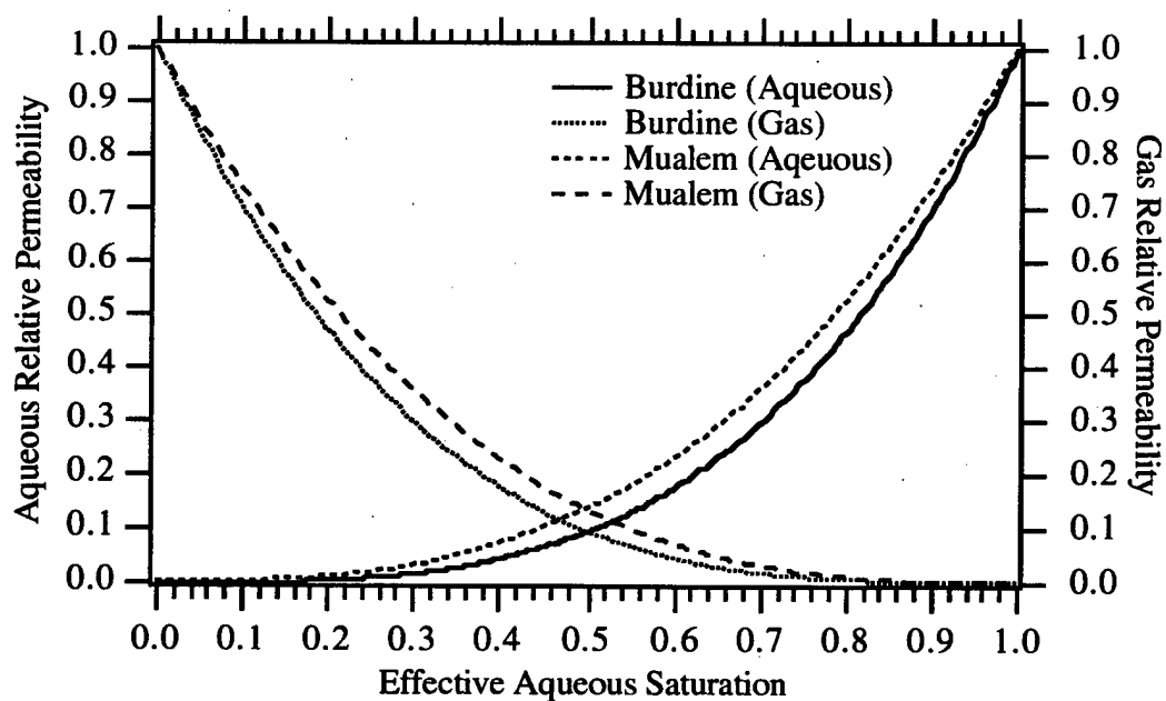
Figure 4.27. Aqueous and Gas Relative Permeability with Brooks-Corey Retention Function \lambda = 5.0
