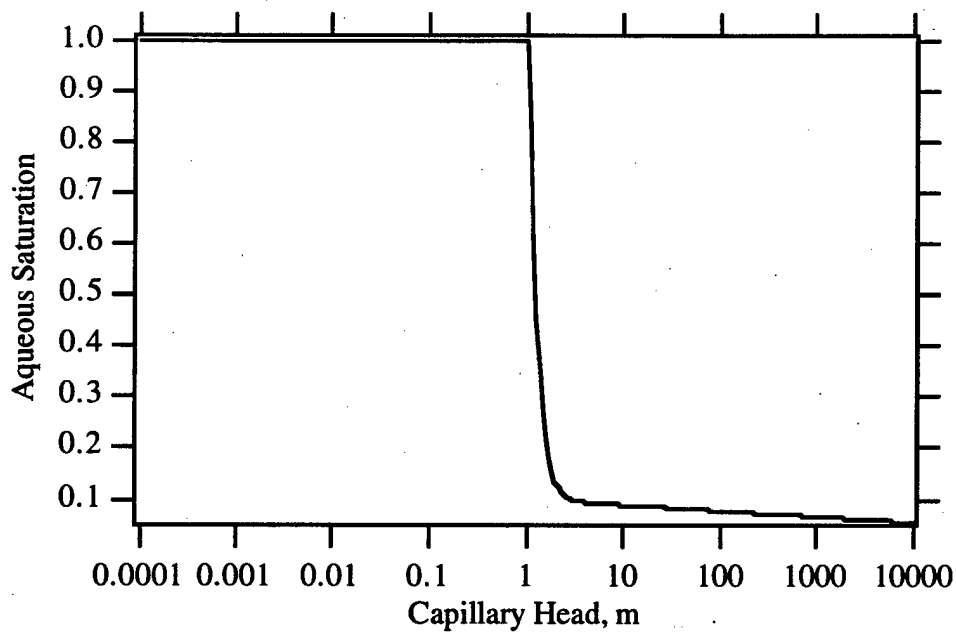
Figure 4.19. Brooks and Corey Saturation Function \psi = 1 \text{ m} , \lambda = 5 , s_m = 0.1
