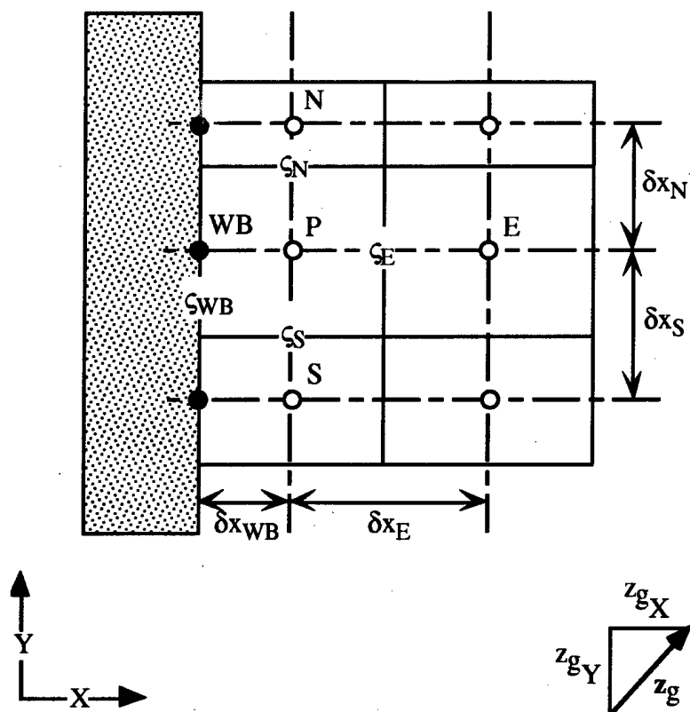
Figure 6.6. X-Y Cartesian Coordinate Plane for "West" Boundary
