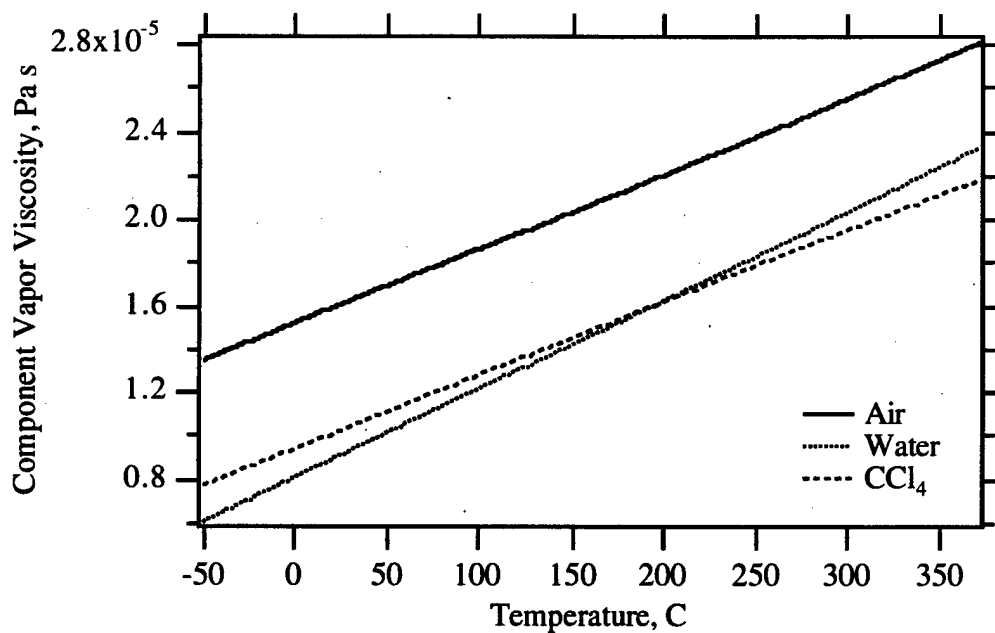
Figure 4.7. Component Vapor Viscosity for Air, Water, and Carbon Tetrachloride
