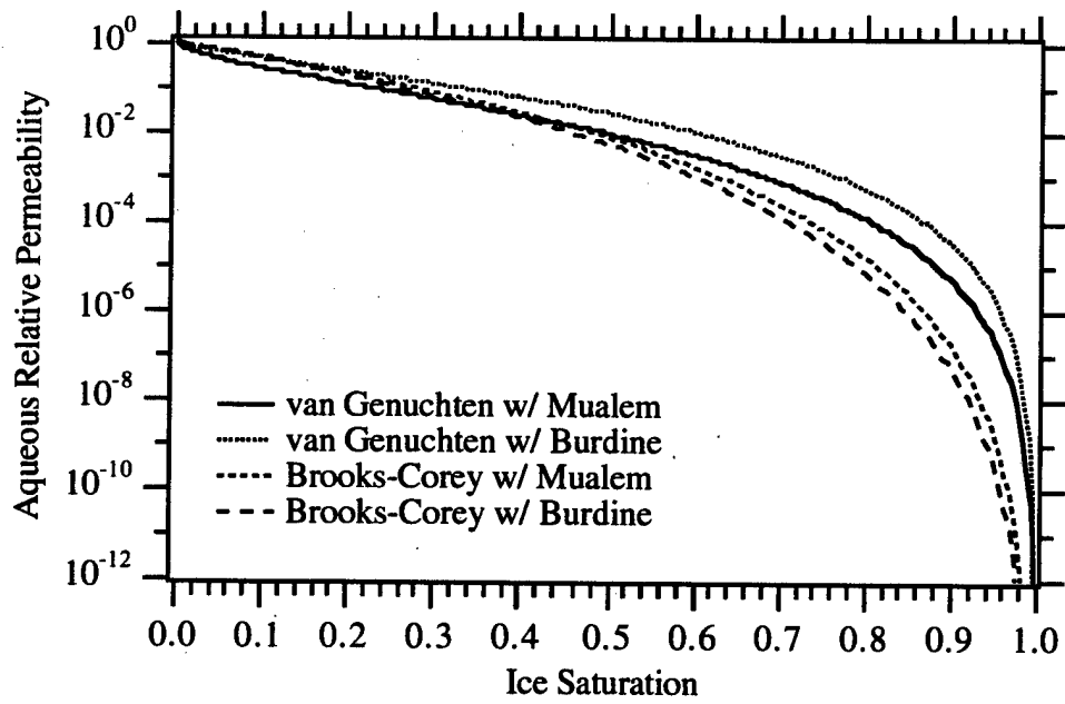
Figure 4.31. Aqueous Relative Permeability Functions Versus Ice Saturation m = 0.5 , \lambda = 0.5 , \bar{s}_\ell + \bar{s}_i = 1.0 , s_m = 0.1
