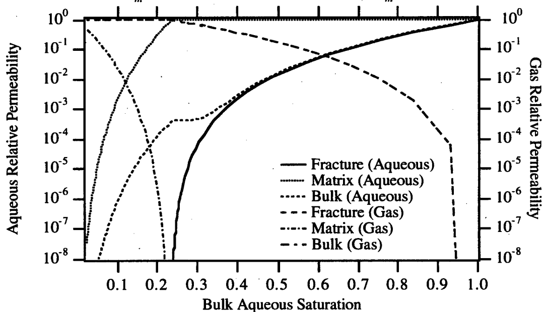
Figure 4.30. Dual Porosity Relative Permeability Function with Burdine Relative Permeability and Brooks-Corey Soil-Moisture Retention
