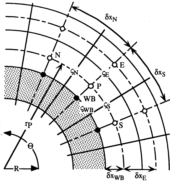
Figure 6.8. R- \theta Cylindrical Coordinate Plane for “West” Boundary
