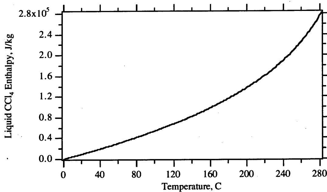
Figure 4.13. Saturated Liquid Enthalpy for Carbon Tetrachloride
