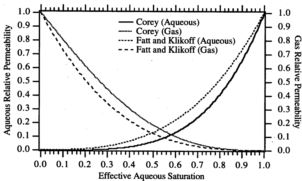
Figure 4.28. Aqueous and Gas Relative Permeability for Corey and Fatt -Klikoff Models
