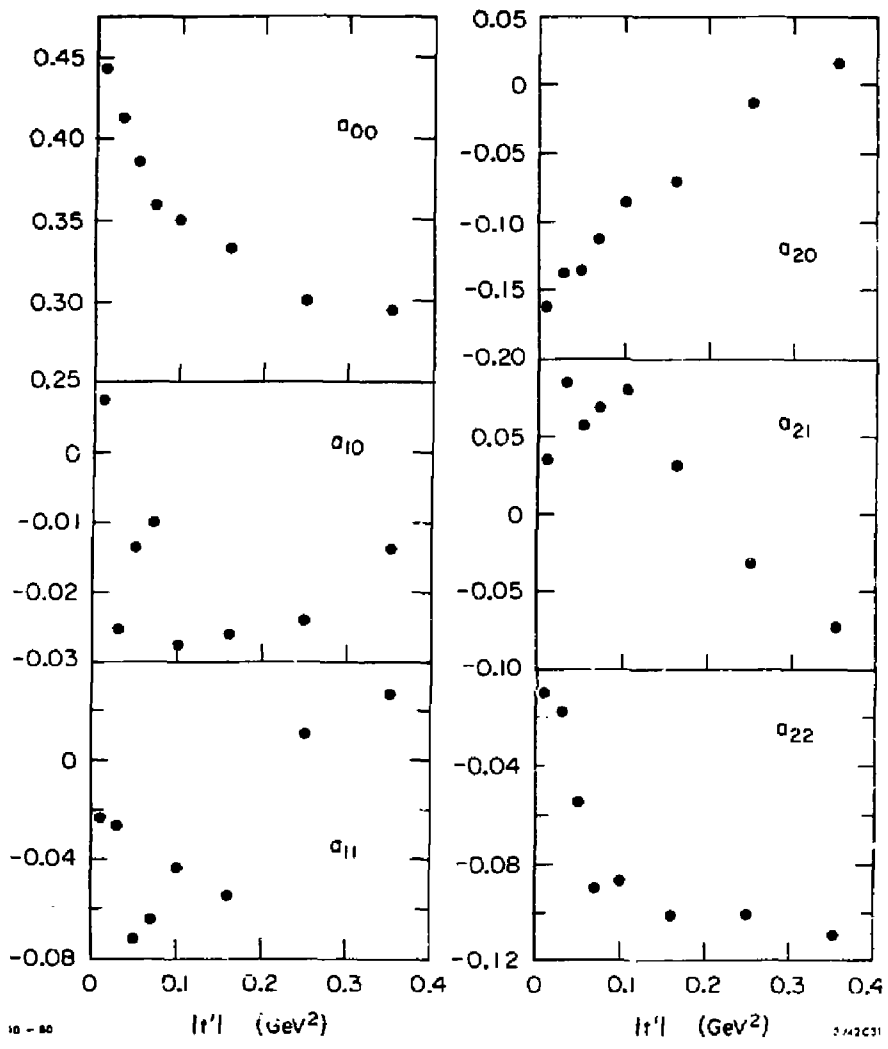
FIG. 40--The angular acceptance moments as a function of t' in the mass bin 0.90 \text{ GeV} < M(K\pi) < 0.94 \text{ GeV} .
