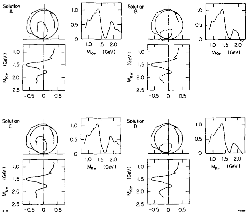
FIG. 56--Real and Imaginary projections of the S wave Argand diagrams. The diameters of these unitary circles have been normalized to one.
