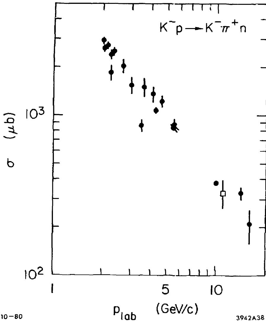
FIG. 25--A sample of total exclusive cross section measurements for the reaction K^- p \rightarrow K^- \pi^+ n versus K^- beam momentum. The cross section measured in this experiment is represented by the symbol \square
