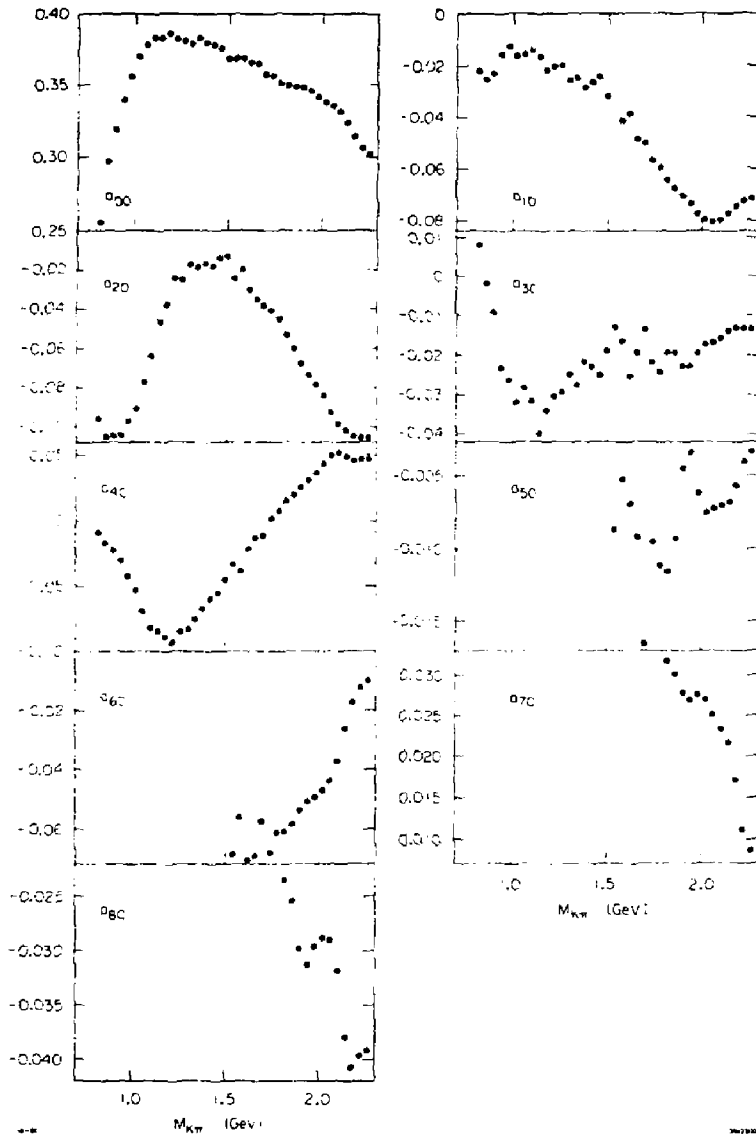
FIG. 28--The final m=0 acceptance moments as a function of mass. These moments were calculated in the t' region, |t'| < 0.2 \text{ GeV}^2 , and in 40 Mev mass bins below 1.8 GeV and 80 MeV overlapping mass bins above this mass.
