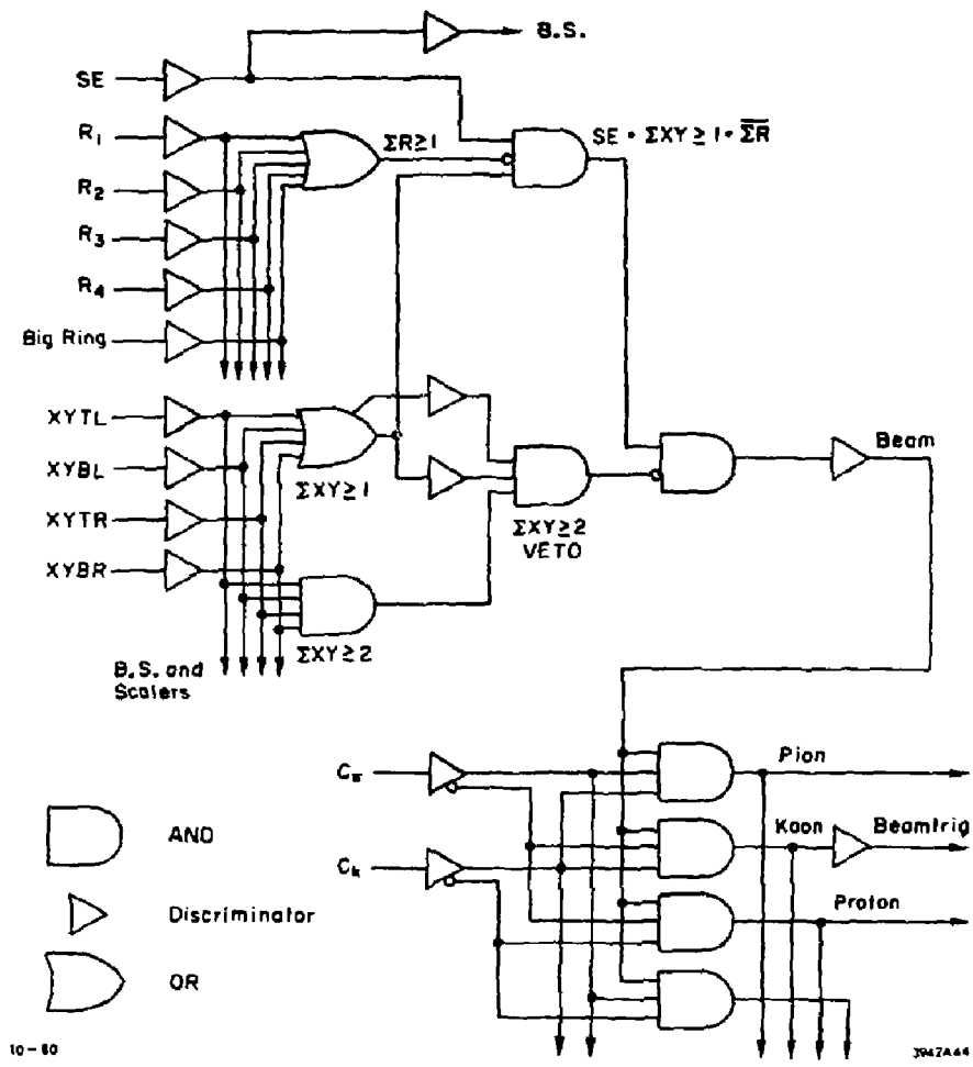
FIG. 12--Beam logic for generating the incident beam kaon (BEAMTRIG) signal.
