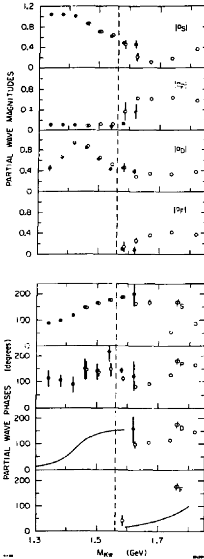
FIG. 43--The K\pi^+ elastic scattering partial waves in the 1.40 GeV- 1.60 GeV mass region with ( \bullet ) and without ( \circ ) a cut of M(\eta\pi) > 1.8 GeV imposed on the data. The overall phase has been fixed to the Breit-Wigner curves drawn on these plots.
