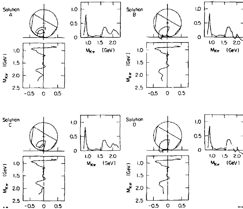
FIG. 57--Real and Imaginary projections of the P wave Argand diagrams. The diameters of these unitary circles have been normalized to one.
