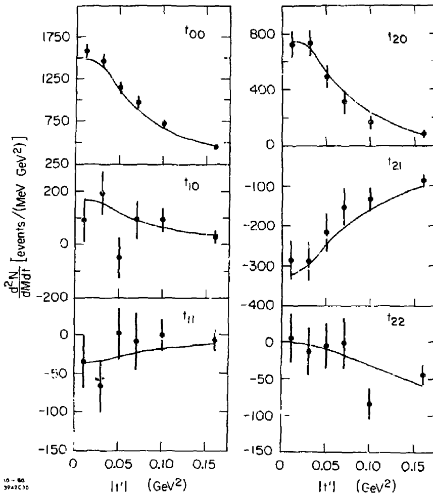
FIG. 41--The acceptance corrected angular moments as a function of t' in the mass bin 0.90 \text{ GeV} < M(K\pi) < 0.94 \text{ GeV} . The moments have been divided by the mass bin width and the t' bin width. The curves drawn through these moments represent the simple exchange model fit to these moments described in the text.
