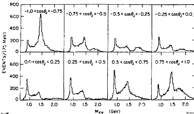
FIG. 22--Eight K^-\pi^+ invariant mass histograms in consecutive \cos\theta_j slices for the standard K^-p \rightarrow K^-\pi^+n data sample.
