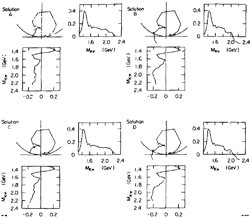
FIG. 58--Real and Imaginary projections of the D wave Argand diagrams. The diameters of these unitary circles have been normalized to one.
