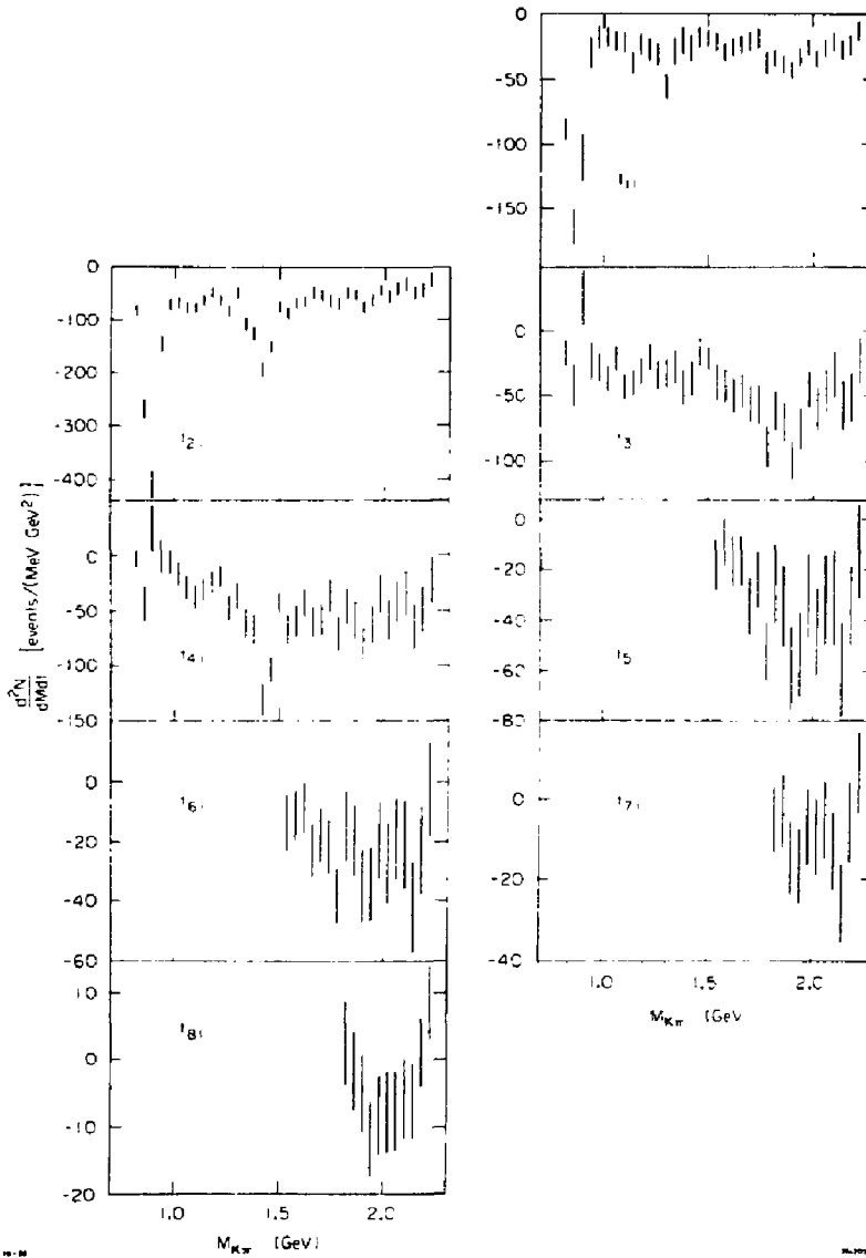
FIG. 32--The final m=1 acceptance corrected angular moments as a function of mass. These moments were calculated in 40 MeV mass bins below 1.8 GeV, and 80 MeV mass bins above this mass. The data used in performing these fits was also selected from the small t' region, |t'| < 0.2 \text{ GeV}^2 . The moments presented have been divided by the mass bin width and the t' bin width.
