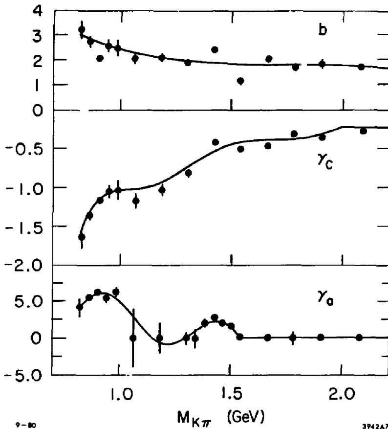
FIG. 42--The production parameters \gamma_a , \gamma_c , and b as a function of mass. The smooth curves drawn through these data points represent simple polynomial fits to the mass dependence of these parameters. These fits were used in the second step of this PWA to specify the t' dependence of the simple exchange model.
