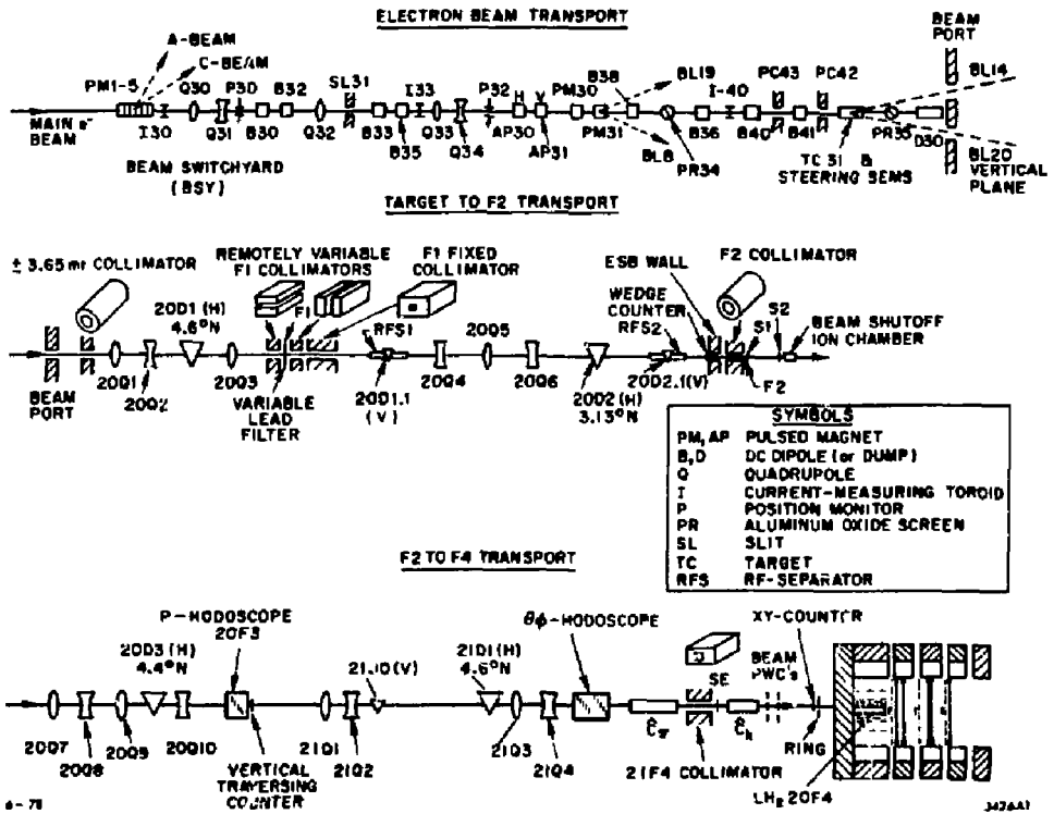
FIG. 6--A layout of the beam transport system.
