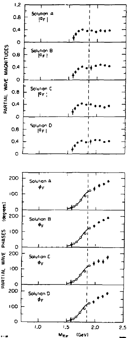
FIG. 48--The four ambiguous K^*\pi^+ elastic scattering F wave magnitudes and phases. The smooth curve drawn on the phase plots represents the F wave phase predicted by the K^*(1780) Breit-Wigner resonance fit in table 20. The overall phase in this region was fixed to the phase represented by the symbol \alpha .
