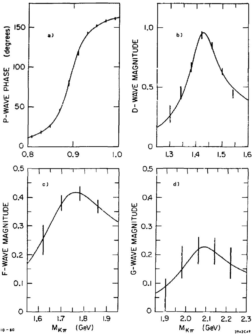
FIG. 55--Partial wave Breit-Wigner fits to the leading K^* resonances (for details see the text); a) the K^*(895) fit b) the K^*(1430) fit c) the K^*(1780) fit d) the K^*(2080) fit
