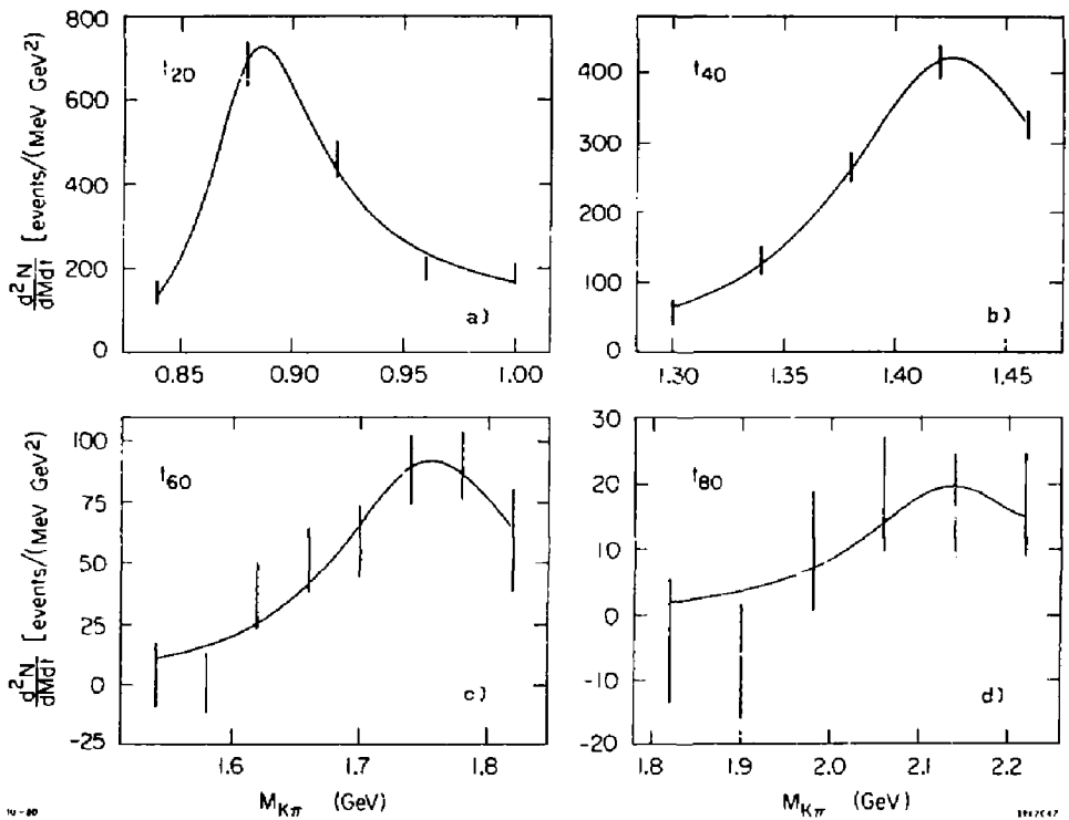
FIG. 35--Leading resonance fits to the t_{2j0} moments: a) the K^*(890) fit, b) the K^*(1430) fit, c) the K^*(1780) fit, and d) the K^*(2080) fit.
