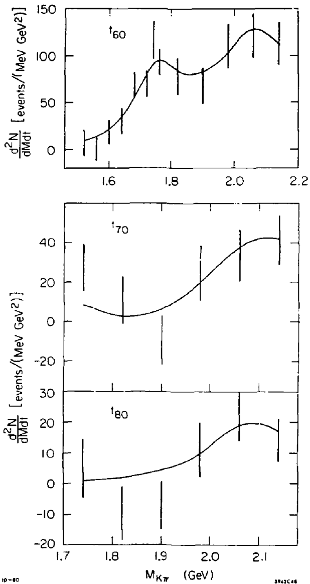
FIG. 36--The energy dependent fit (he the t_{60} , t_{70} , and t_{80} angular moments (see text for a description of this fit).
