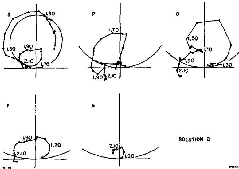
FIG. 53--Argand diagrams for the K\pi^+ elastic scattering partial waves of solution D. The phase has been fixed as in figures 45-49. The points plotted represent fits run in 40 MeV bins below 1.8 GeV and fits run in overlapping 80 MeV bins above this mass.
