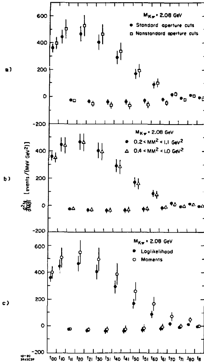
FIG. 39--Angular Moments Comparisons in the mass bin 2.04 \text{ GeV} < M(K\pi) < 2.12 \text{ GeV} ; a) tight aperture cut vs standard aperture cut b) tight missing mass cut vs standard missing mass cut c) maximum likelihood fit vs moments method fit
