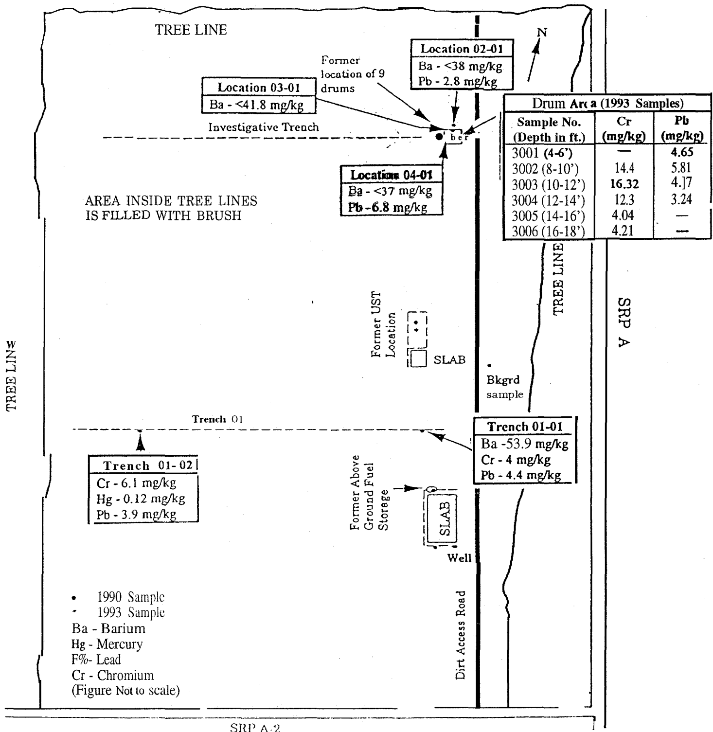
Figure 2. Layout of the Gunsite 720 Rubble Pit Unit Showing Sample Locations and Location and Concentration of Metals which Exceed the Unit-Specific Background Level
