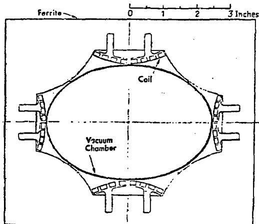
Fig. 5. Ferrite pulsed quadrupole.
