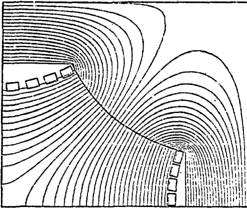
Fig. 6. Calculated magnetic field plot for pulsed quadrupoles.
