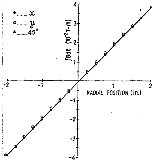
Fig. 9. Search coil pick up signal as a function of position in the pulsed quad.
