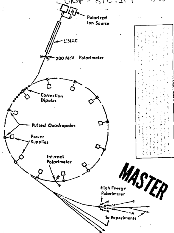
Fig. 1. AGS modifications for polarized proton acceleration.
