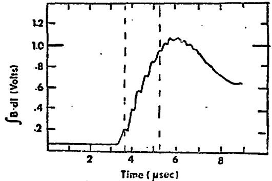
Fig. 8. Scope trace of search coil pick up signal on pulsed quad.
