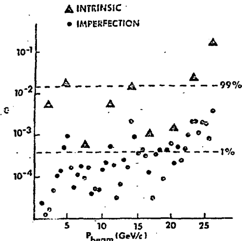
Fig. 3. ZGS depolarizing resonance strengths, \epsilon , calculated for standard acceleration and \pm 1 mm misalignments.
