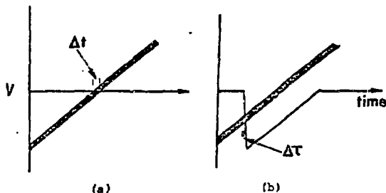
Fig. 4. a) Normal resonance crossing b) Rapid intrinsic resonance crossing by pulsing the vertical betatron frequency, v .
