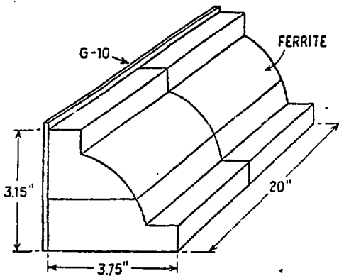
Fig. 7. Perspective view of a ferrite pole quadrant.
