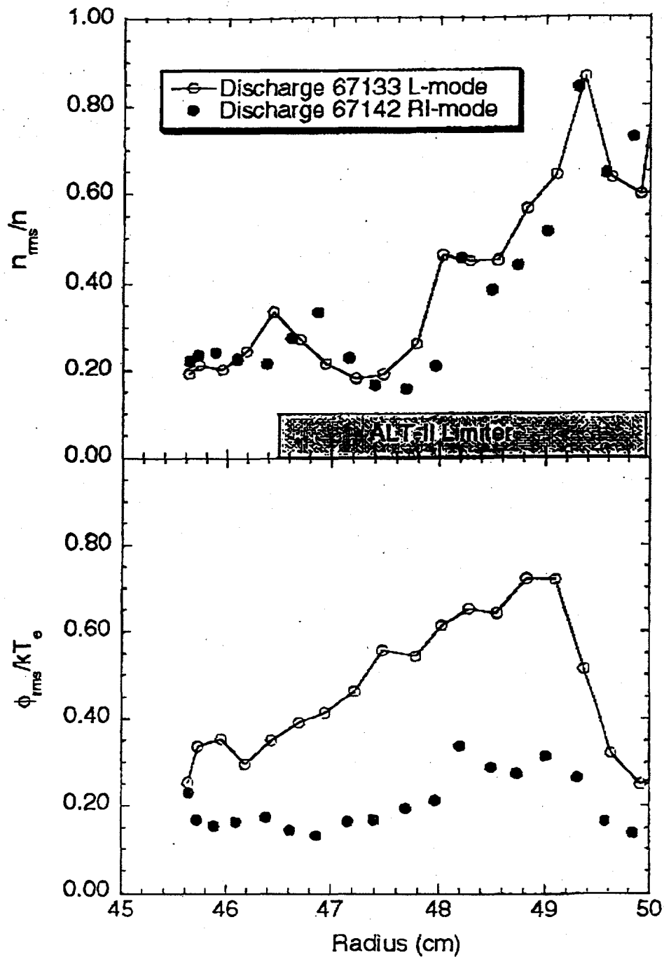
Fig. 1: Reduction of normalized potential fluctuations by factors of 2-5 is observed in the bottom panel. The normalized density fluctuation levels are not much affected by the RI-mode.
