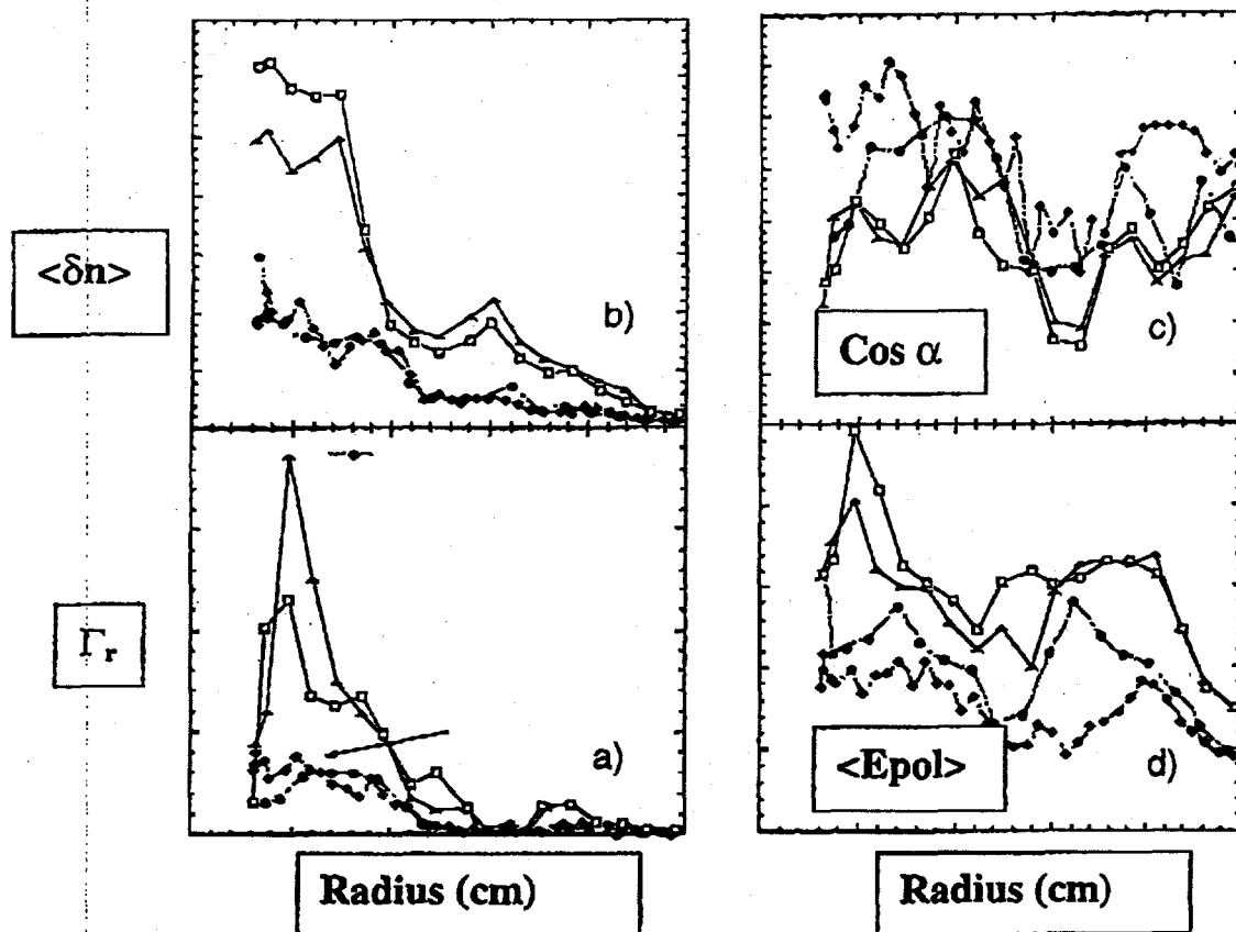
Fig. 2: Turbulent radial particle flux (a), absolute density turbulence level (b), the cosine of the phase between density and poloidal field fluctuations (c) and the poloidal field fluctuation levels (d) are shown vs. radius during RI-mode discharges in TEXTOR. The limiter and SOL are shown as a dark square.
