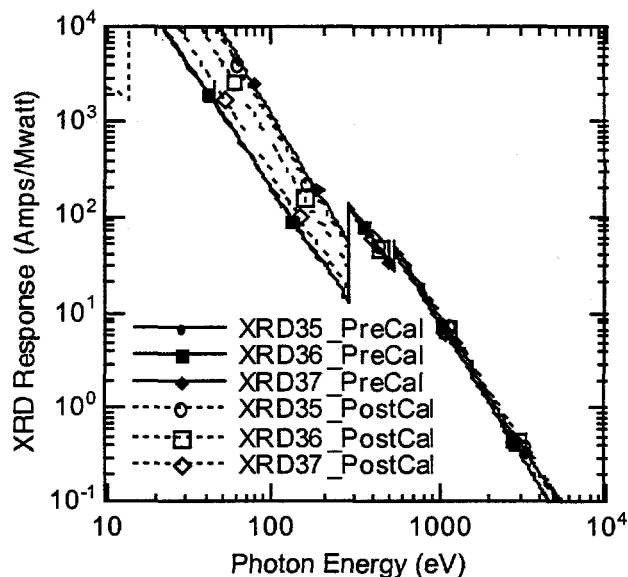
Figure 15. Pre- vs. post-calibrated carbon photocathode responses.
