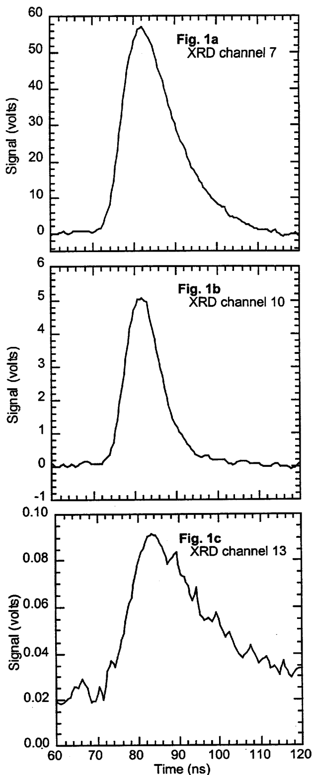
Figure 1. Three representative XRD traces from PBFA-II shot #6517.
