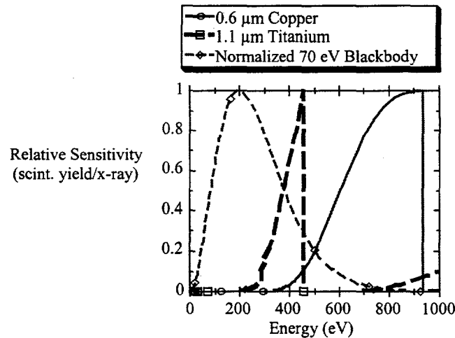
Figure 3. Estimated responses for x-ray filter coatings.
