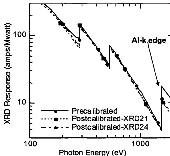
Figure 16. XRD pre- and post-calibrations.
