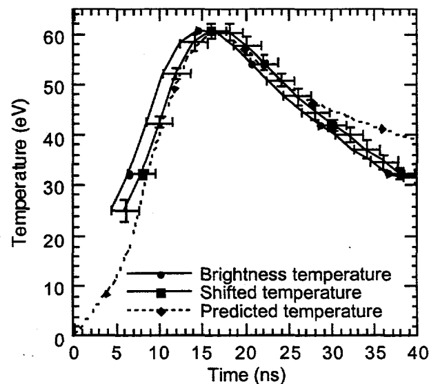
Figure 2. Unfolded, time-resolved brightness temperature for shot #2026.
