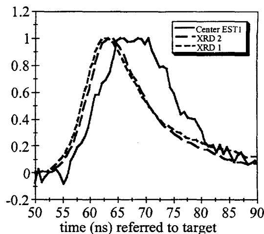
Figure 9. Time history of two XRD traces and the emission from the center of the target as obtained with the EST diagnostic. The \text{FWHM}_{\text{center}} = 17 \pm 4 ns and the \text{FWHM}_{\text{XRD}} = 13 \pm 2 ns.
