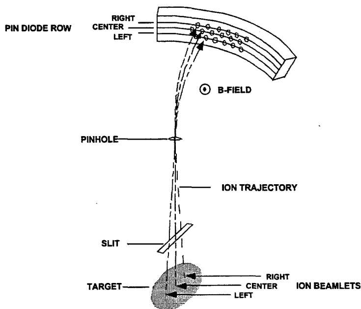
Figure 2. Artist's conception of the magnetic spectrometer.
