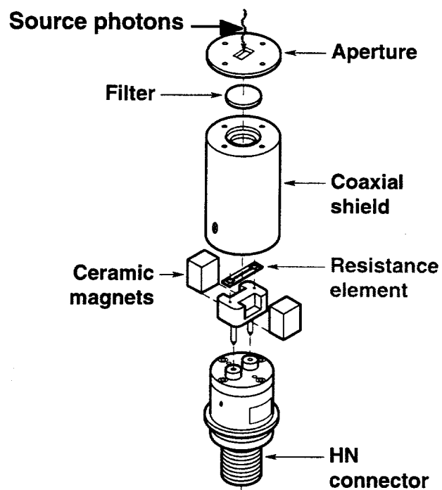
Figure 1. A bolometer detector
