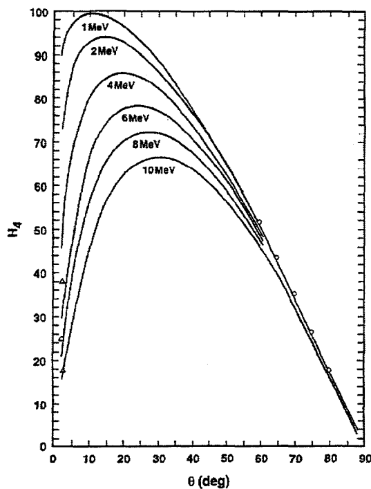
Figure 4. H_4 as a function of angle for various initial Li beam energies.
