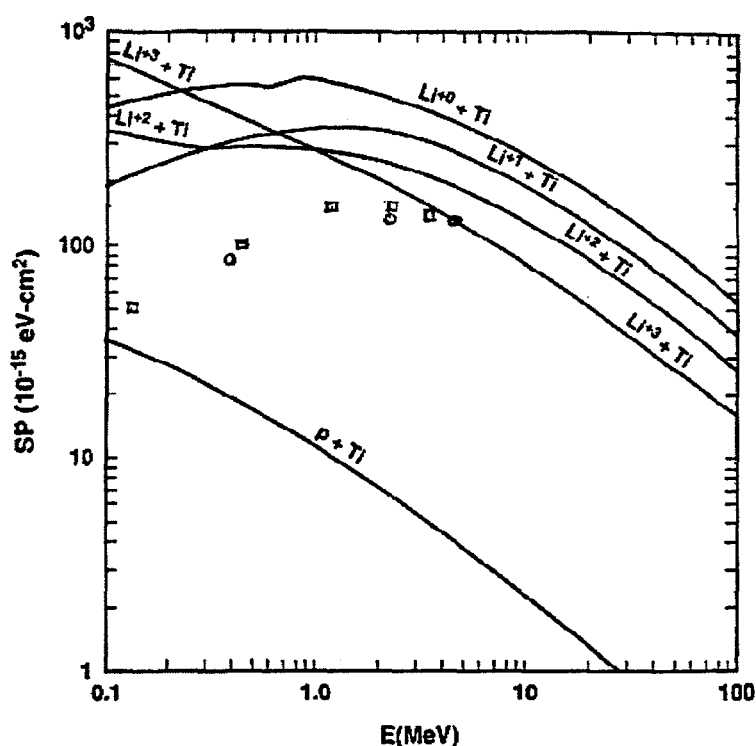
Figure 2. Comparison of calculated SP for Li on Titanium with the measurements of Teplova et al. 1 on argon (open squares) and nickel (open circles).
