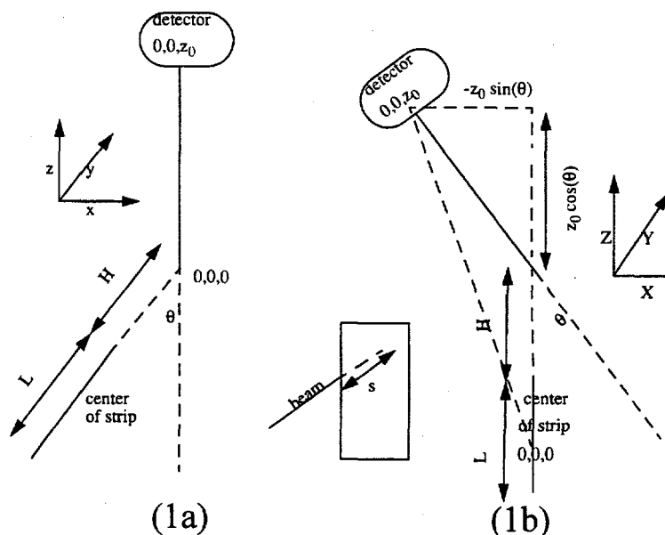
Figure 1. Coordinate systems used for the calculation inner-shell x-ray yields. (1a) Location of Ti strip with detector on-axis at (0, 0, z_0) . (1b) Off-axis detector.
