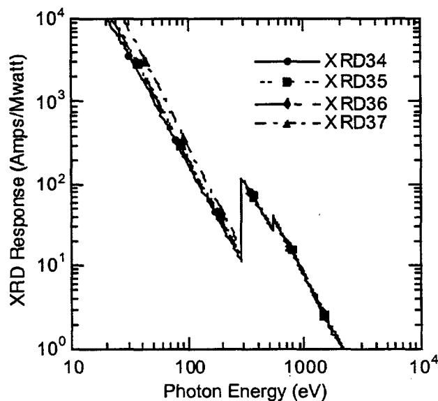
Figure 14. Responses for the carbon photocathodes.
