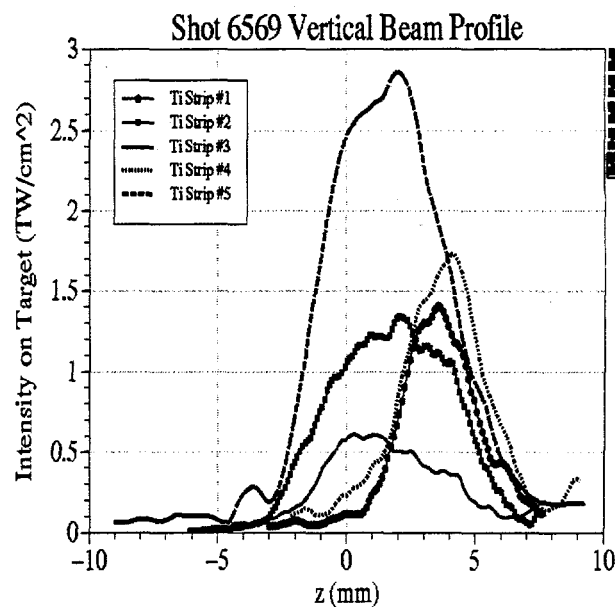
Figure 3. Vertical beam profiles from shot #6569. Strips #1 and #4 are shortened and thus only view the beam above the target. The target midplane is at z=0 .
