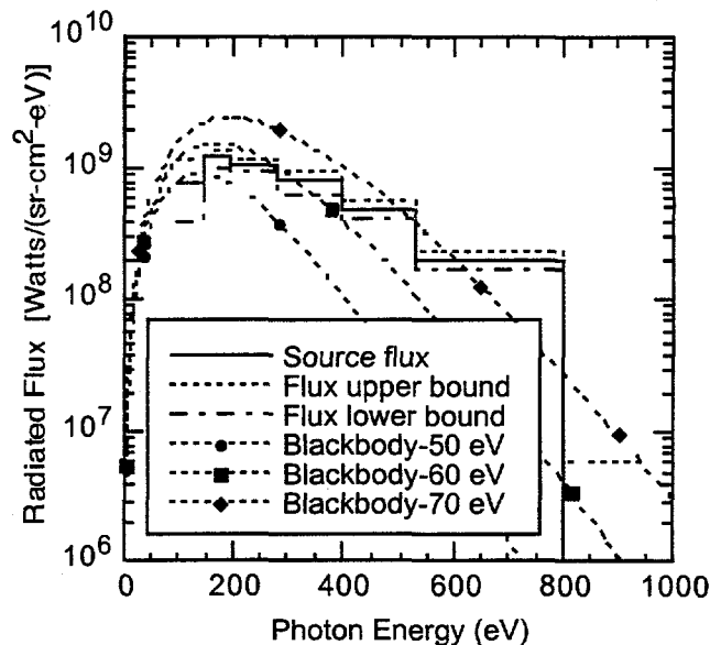
Figure 1. Time-integrate unfolded peak radiation spectrum from shot 2026.
