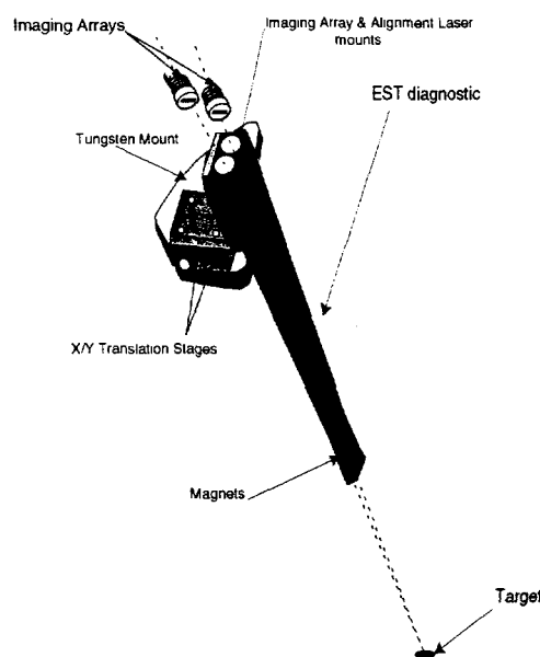
Figure 1. EST imaging assembly and alignment hardware.
