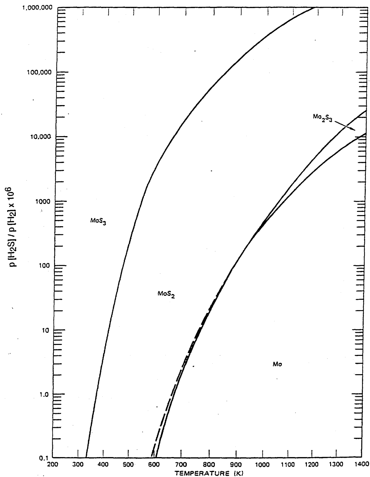
Figure 3. Stability of molybdenum sulfides in hydrogen.
