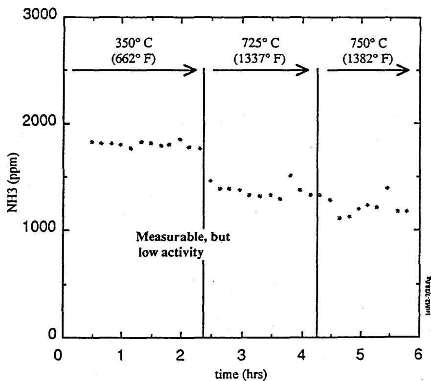
Figure 2.3.5-3 Ammonia Decomposition over L-3787M2 Previously Subjected to Ten Absorption/Regeneration Cycles
