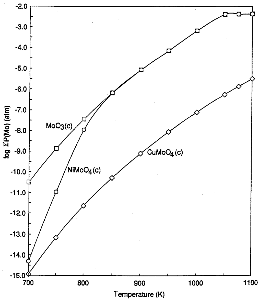
Figure 1. Plot of total Mo-containing species pressure vs temperature over \text{MoO}_3(\text{c}) and \text{NiMoO}_4(\text{c}) in presence of pure \text{O}_2 at 0.02 atm total pressure.
