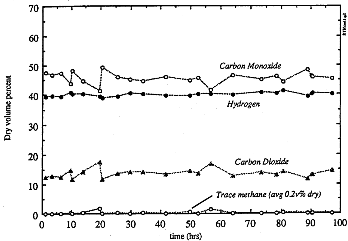
Figure 3.4-1 Reactor inlet dry gas concentrations for 100-hr run
