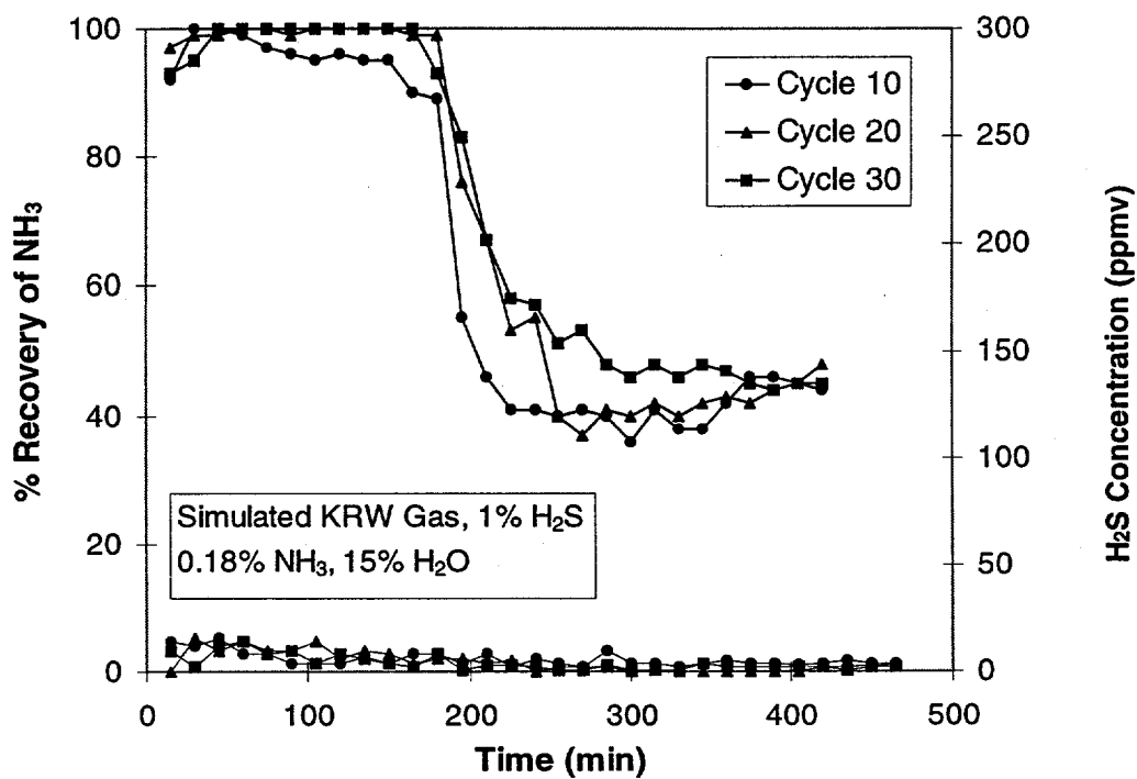
Figure 5. Multicycle \text{NH}_3 removal performance of HART-49 at 700^\circ\text{C} and 1.0 atm.
