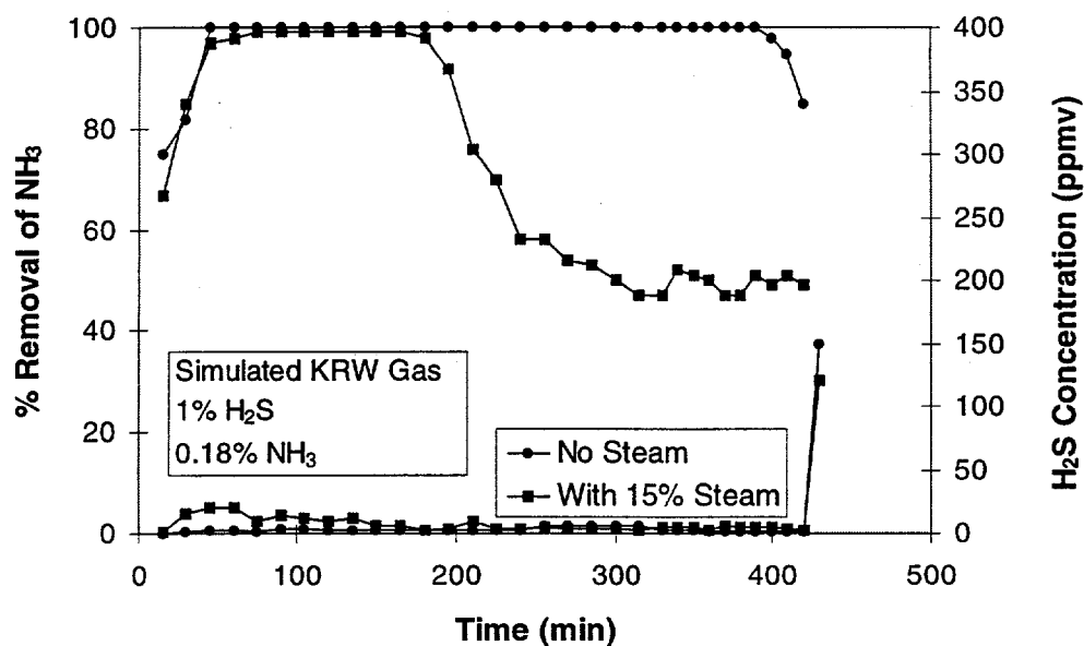
Figure 4. Simultaneous \text{H}_2\text{S} and \text{NH}_3 removal using HART-49 at 700^\circ\text{C} and 1.0 atm.
