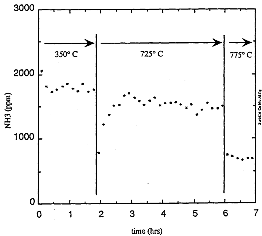
Figure 2.3.3-1 Ammonia Measurements for Co-Mo-Al-Zinc Titanate
