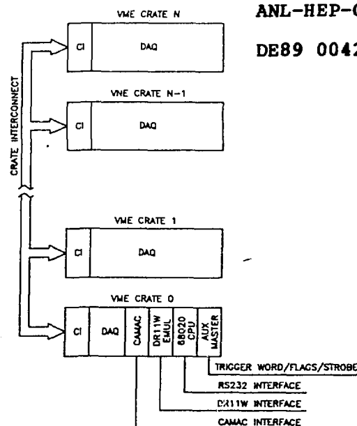
Fig. 1. A configuration of a multi-crate VME environment in which the DAQ cards reside.
