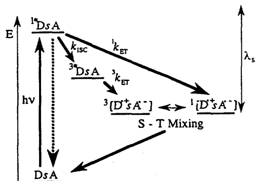
Figure 3. Energy level diagram of the IET reactions, valid for all donor-spacer- acceptor molecules. The solvent reorganization energy is represented schematically by \lambda_s .
