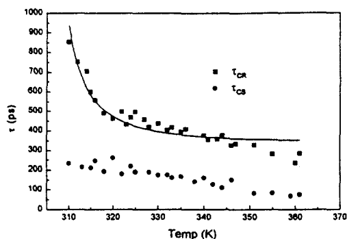
Figure 5. The temperature dependence of the time constants for charge separation ( \tau_{CS} ) and charge recombination ( \tau_{CR} ) for PNI-PI in 5CB are shown.
