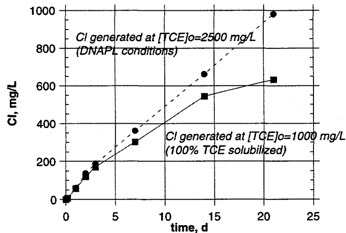
No significant DNAPL destruction at the iron surface, unless TCE is solubilized Figure L-7. TCE degradation with DNAPL present.
