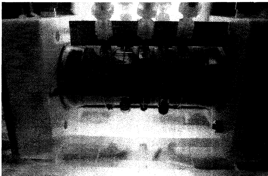
Figure I-3. Photograph of agar experiment with iron zone. Anode is on the left and cathode on the right.
