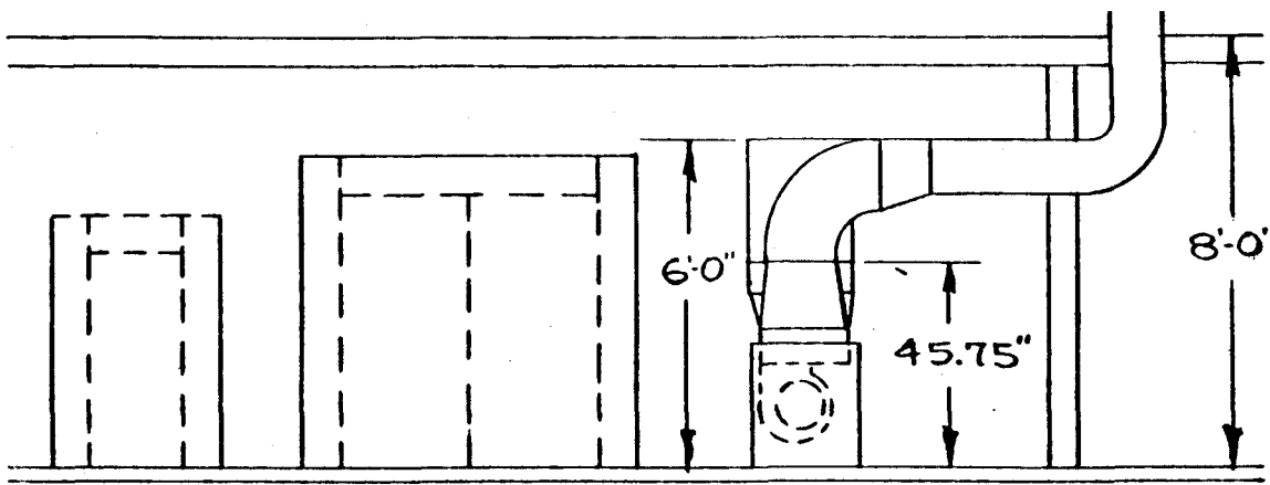
VIEW "A-A"
