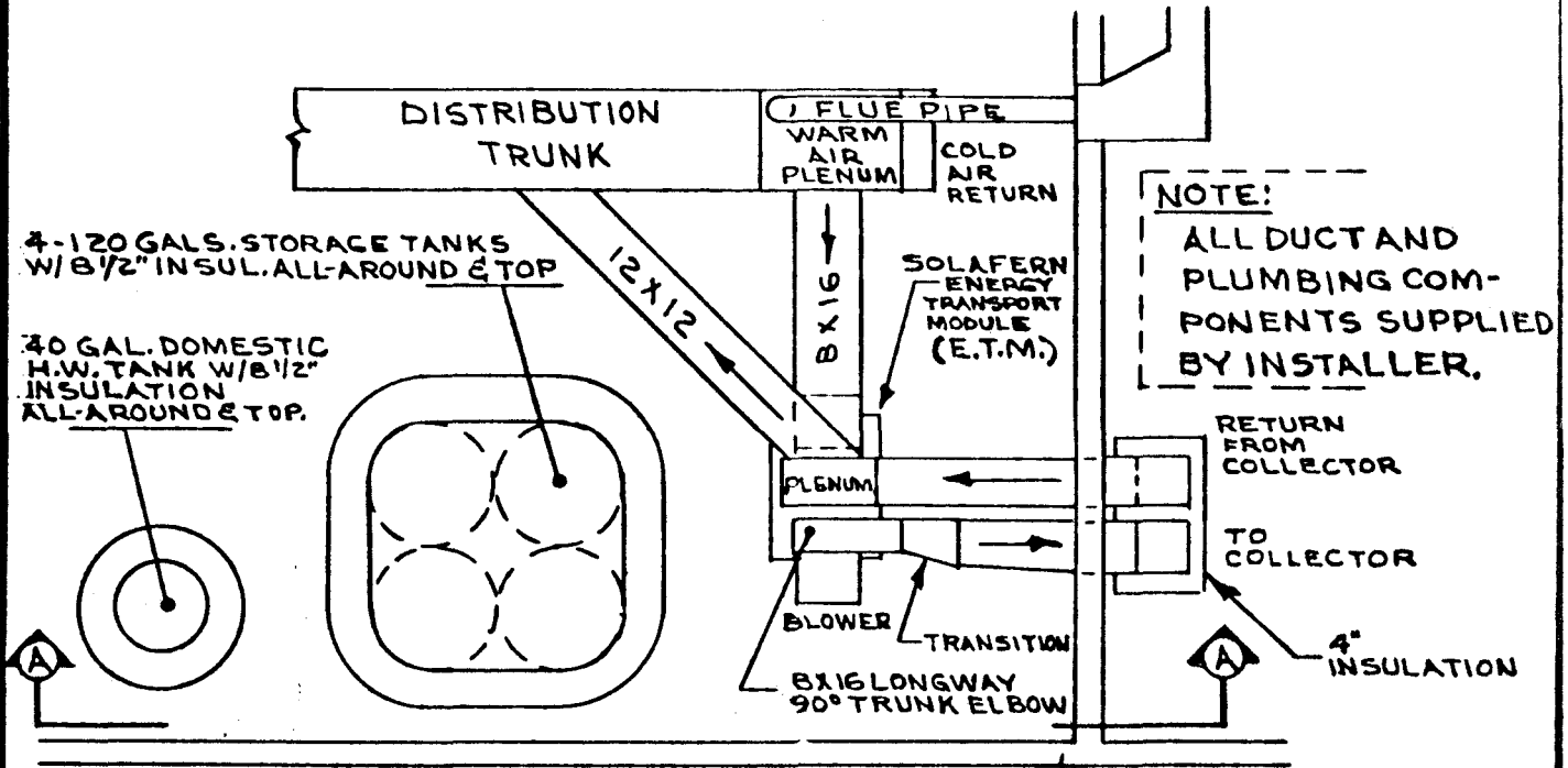
BASEMENT PLAN VIEW SCALE: 1/4" = 1.0'
