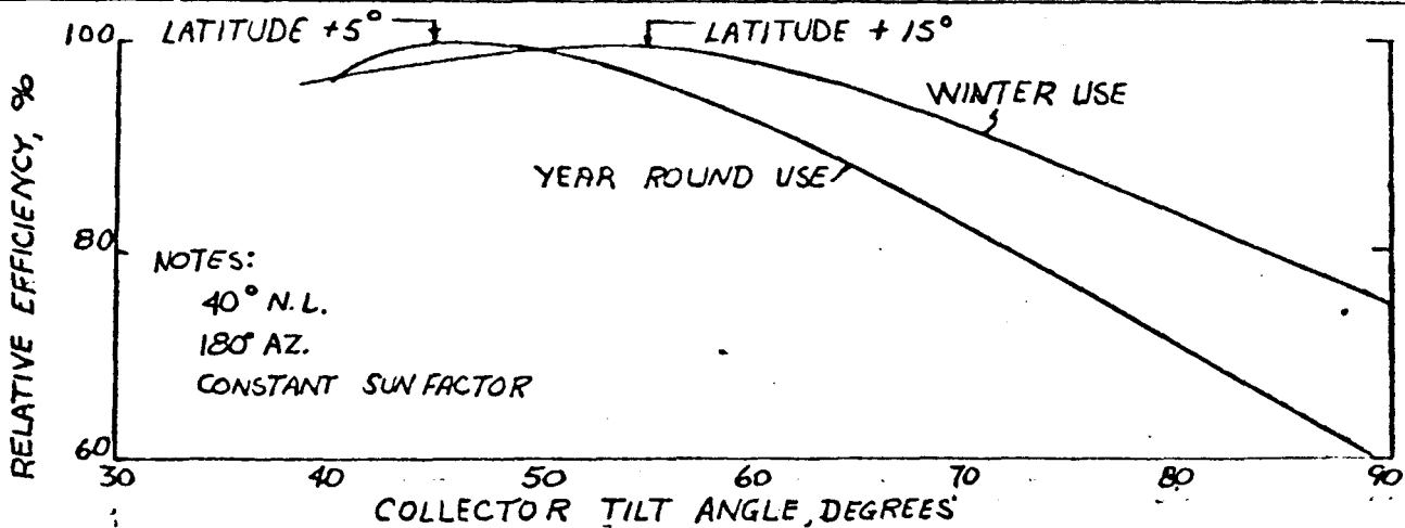
FIGURE 7 EFFECT OF COLLECTOR TILT ON SYSTEM EFFICIENCY
