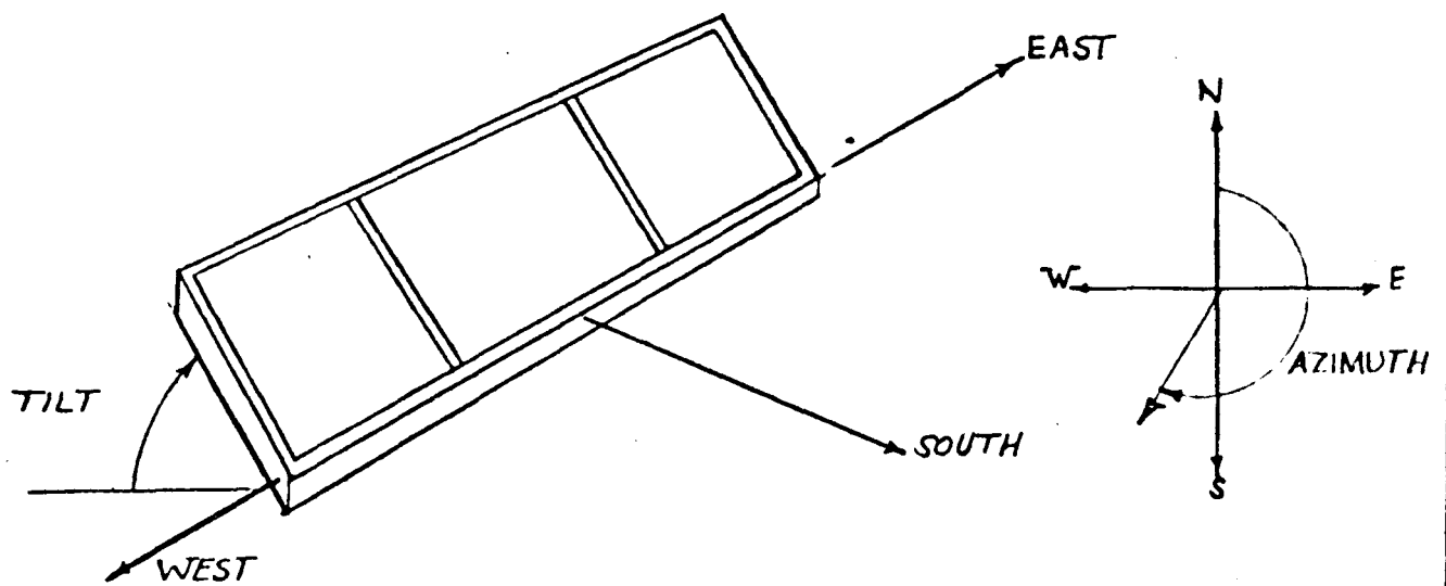
FIGURE 5 COLLECTOR TILT & AZIMUTH
