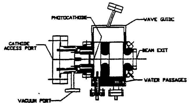
FIGURE 1 RF ELECTRON GUN SECTION
