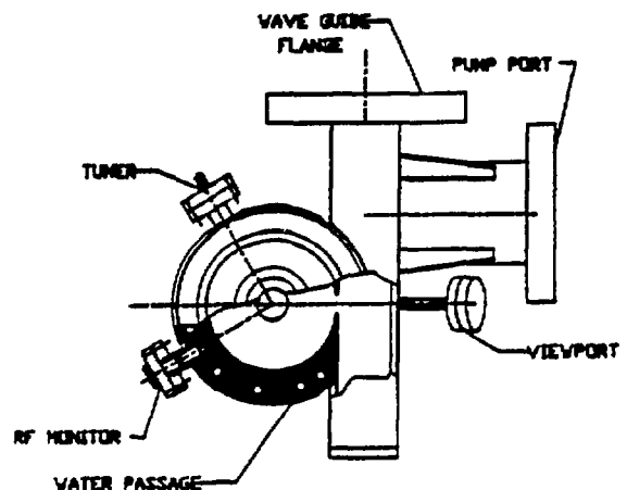
FIGURE 2 RF ELECTRON GUN END VIEW
