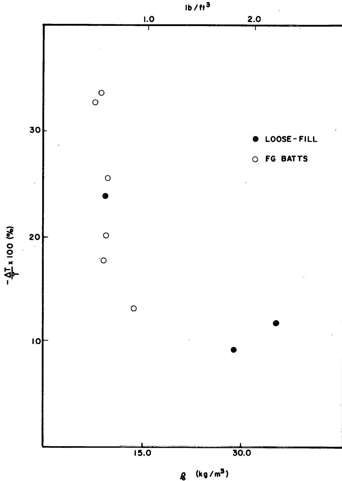
Figure 7. Compression at 4.88 \text{ kg/m}^2 ( 1.0 \text{ lb/ft}^2 ).
