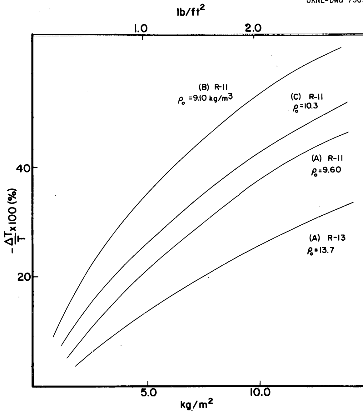
Figure 3. Compression of R-11 and R-13 Fiberglass Batts for Loads up to 13.4 \text{ kg/m}^2 ( 2.75 \text{ lb/ft}^2 ).
