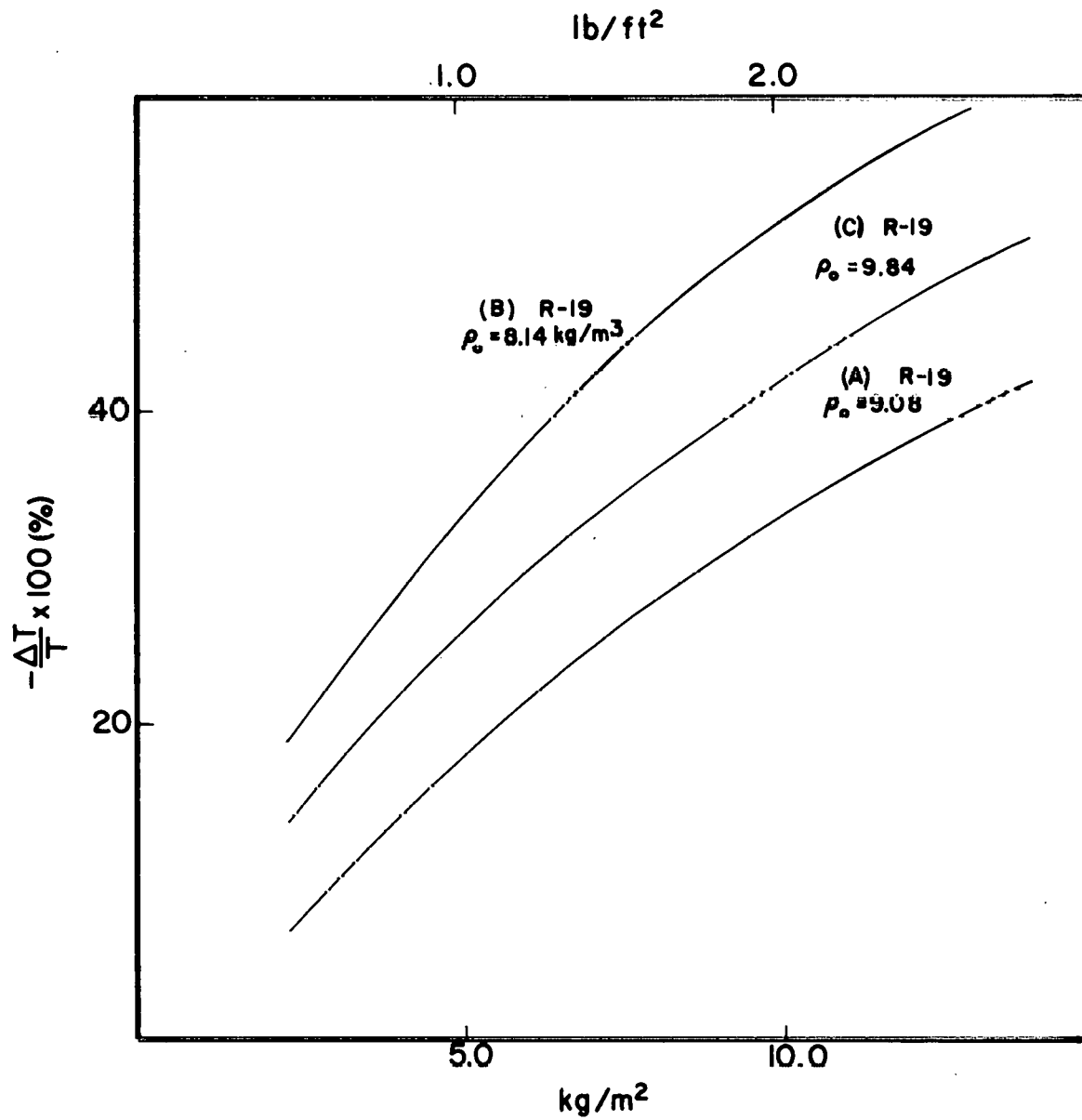
Figure 4. Compression of R-19 Fiberglass Batts for Loads up to 12.2 \text{ kg/m}^2 ( 2.5 \text{ lb/ft}^2 ).
