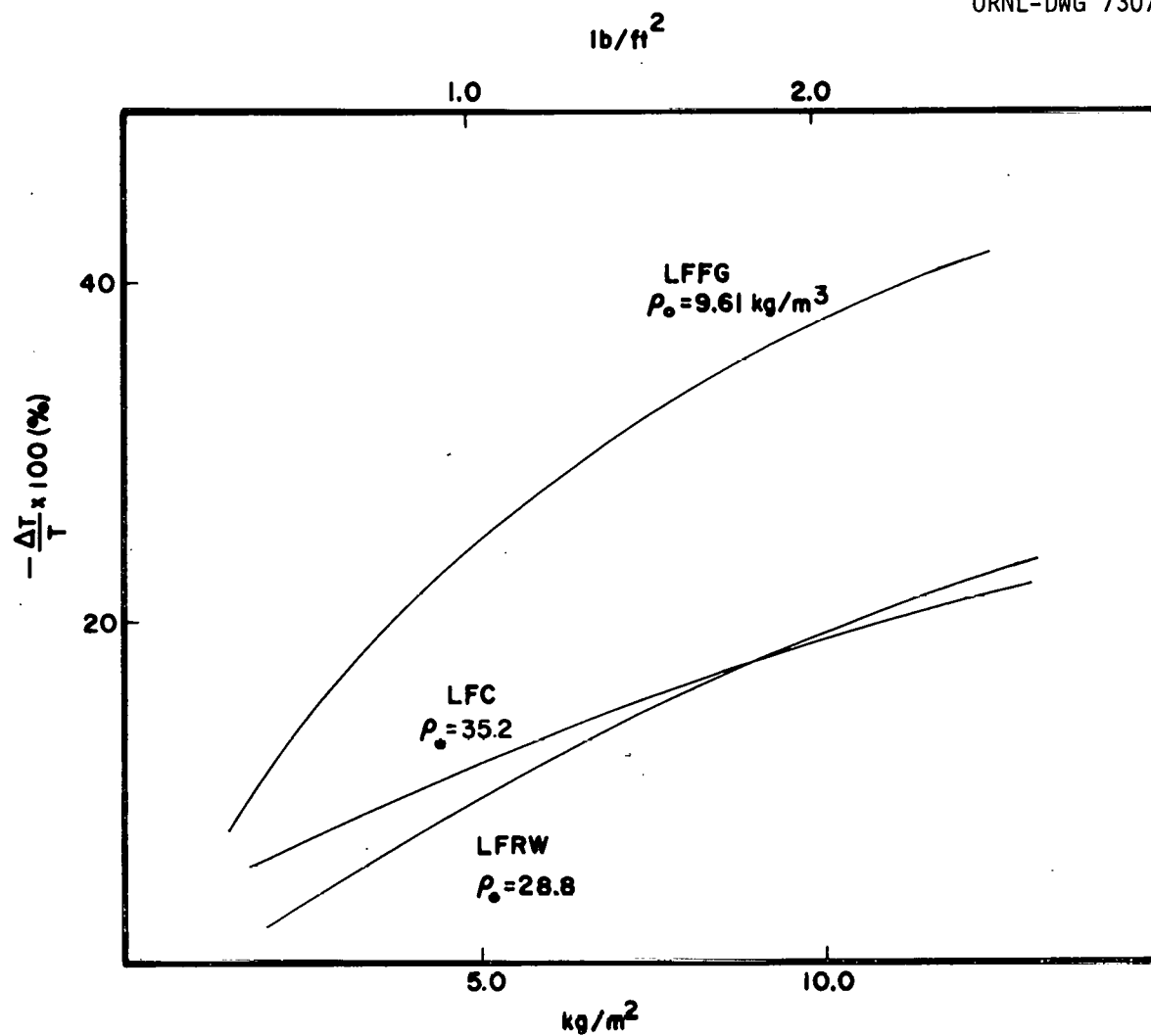
Figure 5. Compression of Loose-Fill Insulations for Loads up to 12.2 \text{ kg/m}^2 ( 2.5 \text{ lb/ft}^2 ).
