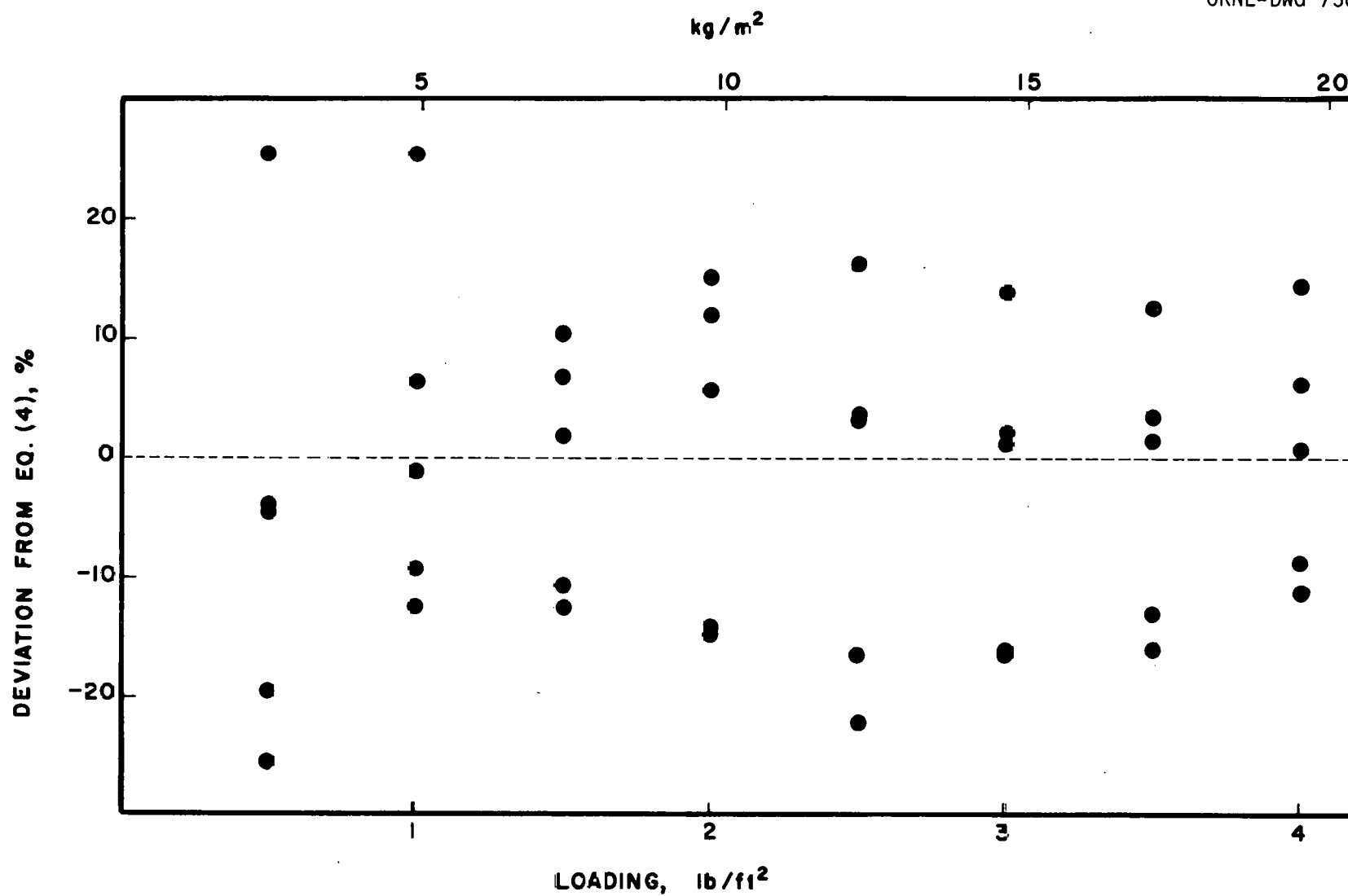
Figure 6. Deviation of Experimental Data for Compression of Product R-11 (A) from Equation (4).
