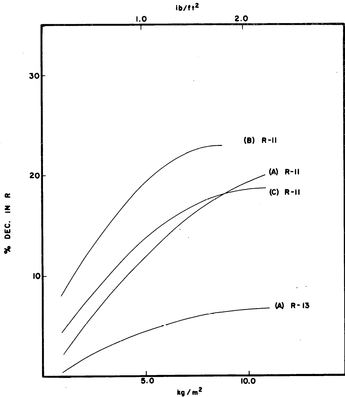
Figure 8. Percentage Decrease in R-Value of R-11 and R-13 Fiberglass Batts due to Compression.
