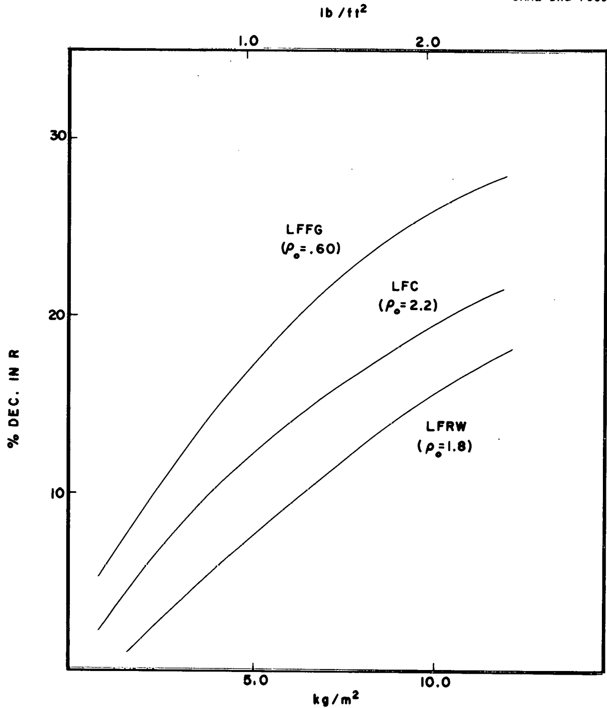
Figure 10. Percentage Decrease in R-Value of Loose-Fill Insulations due to Compression.
