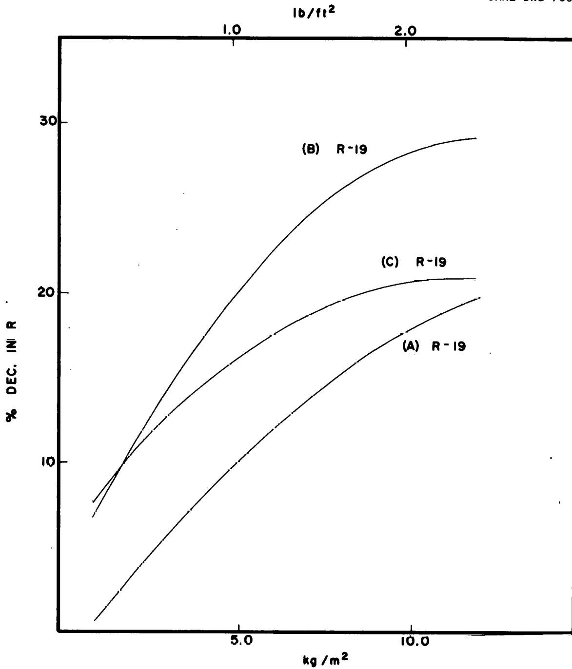
Figure 9. Percentage Decrease in R-Value of R-19 Fiberglass Batts due to Compression.
