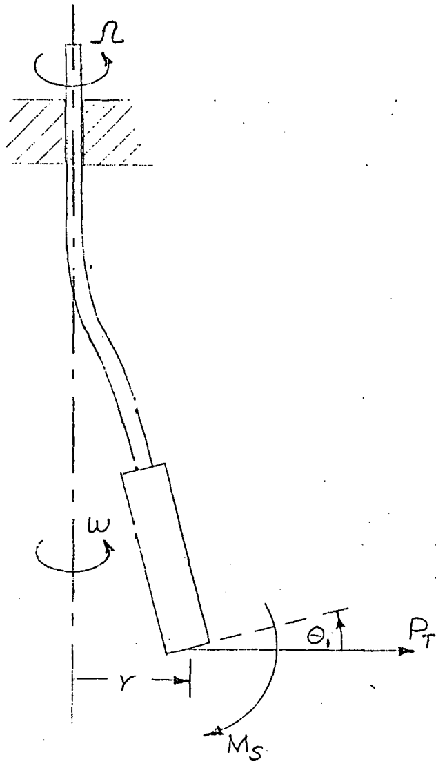
SHAFT/QUILL
