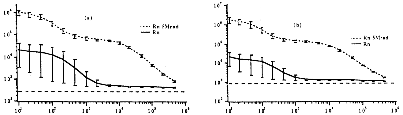
Fig. 2. Series noise resistance versus frequency for the Siliconix 2N4416A JFET at (a) I_D = 1 mA and (b) I_D = 100 \mu A [ V_{DS} = 2.5 V].
