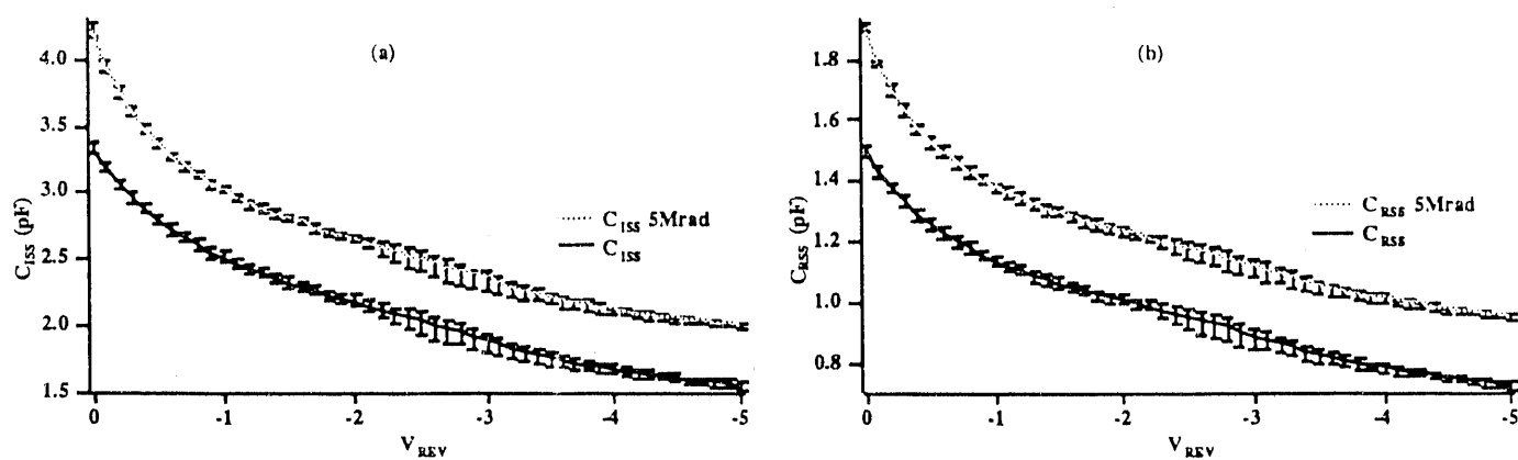
Fig. 4. Capacitance variations for the 2N4416A JFET.
