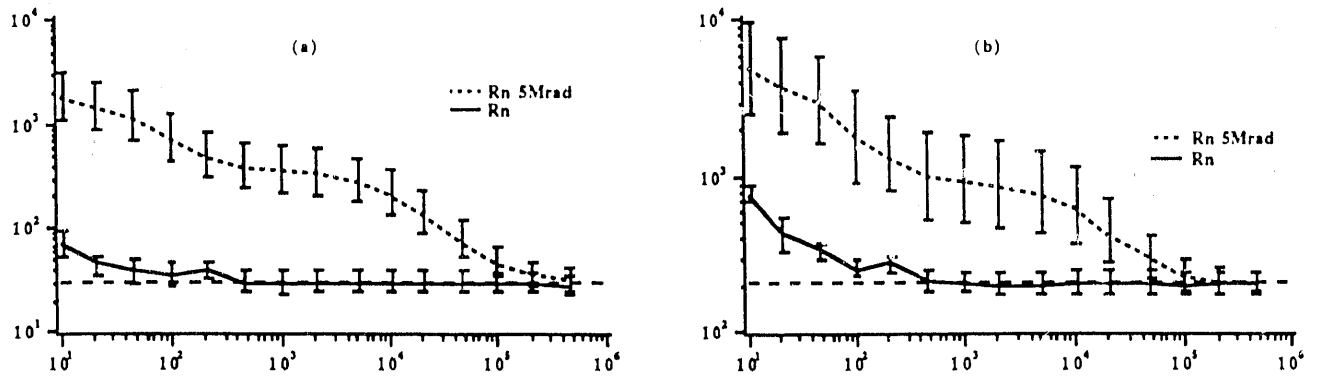
Fig. 1. Series noise resistance versus frequency for the InterFet NJ3600L at (a) I_D = 1 mA and (b) I_D = 100 \mu A [ V_{DS} = 2.5 V].
