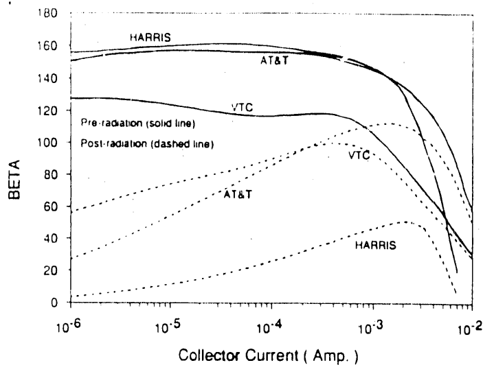
Fig. 5. Beta vs. I_C for npn high-frequency transistors. [ V_{CE} = 2.5 V]
