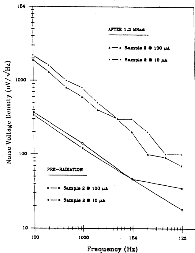
Fig. 7. Noise spectra for a MOSIS NMOS transistor with W/L = 100 \mu m/10 \mu m , both before and after a 1.3-Mrad ( ^{60}Co ) total dose.
