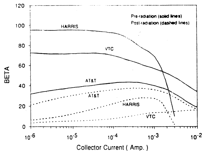
Fig. 6. Beta vs. I_C for pnp high-frequency transistors. [ V_{CE} = -2.5 V]
