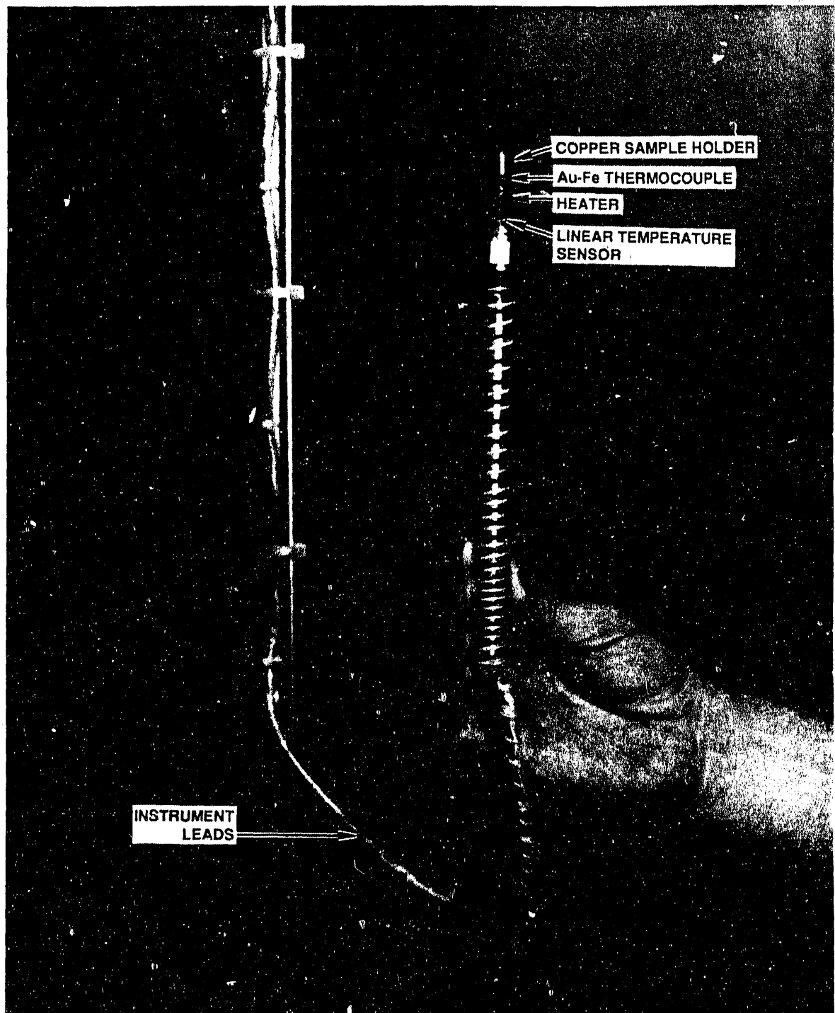
Fig. 8. Photograph of the cryostat sample holder.
