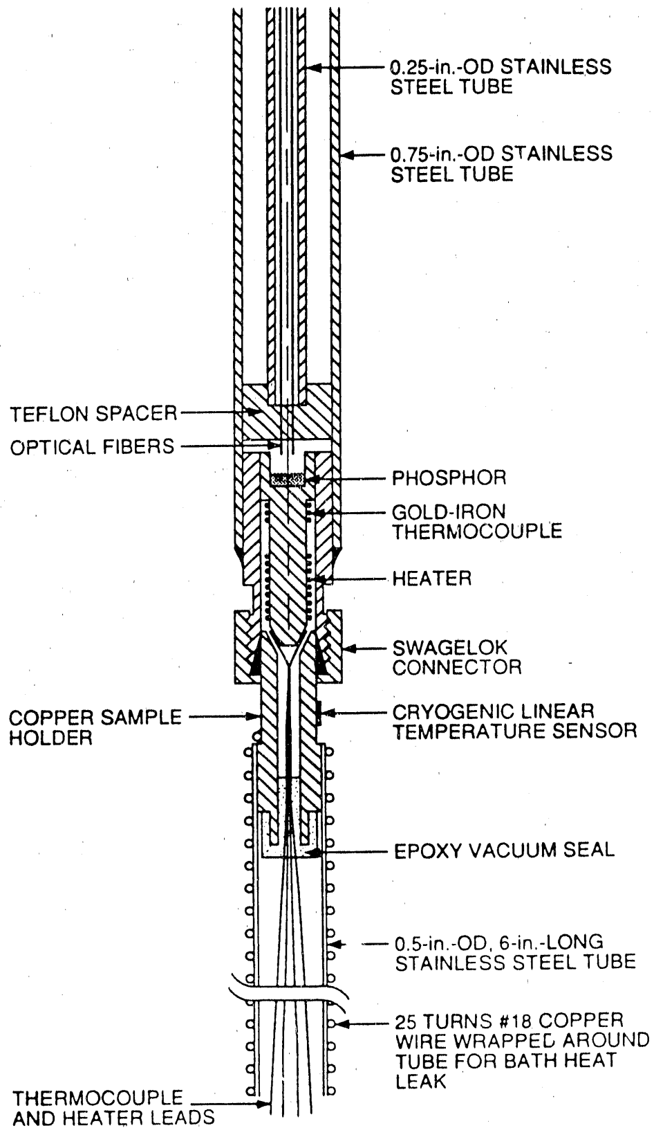
Fig. 9. Thermography sample holder.
