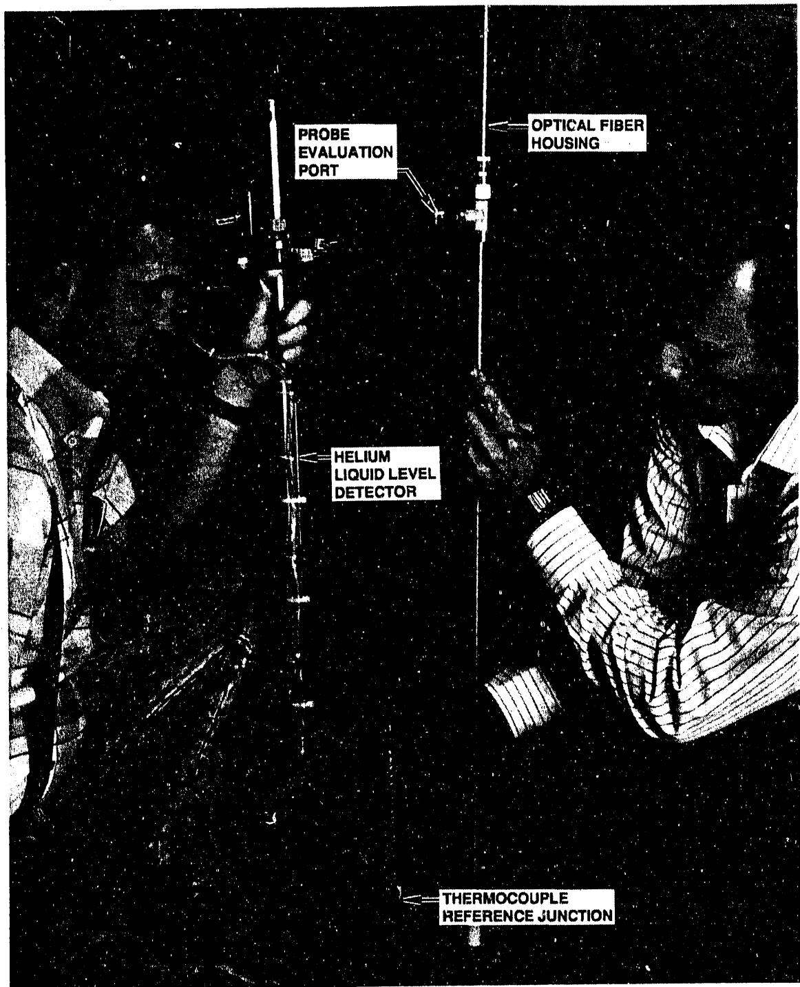
Fig. 7. Cryostat for thermographic phosphor experiments.
