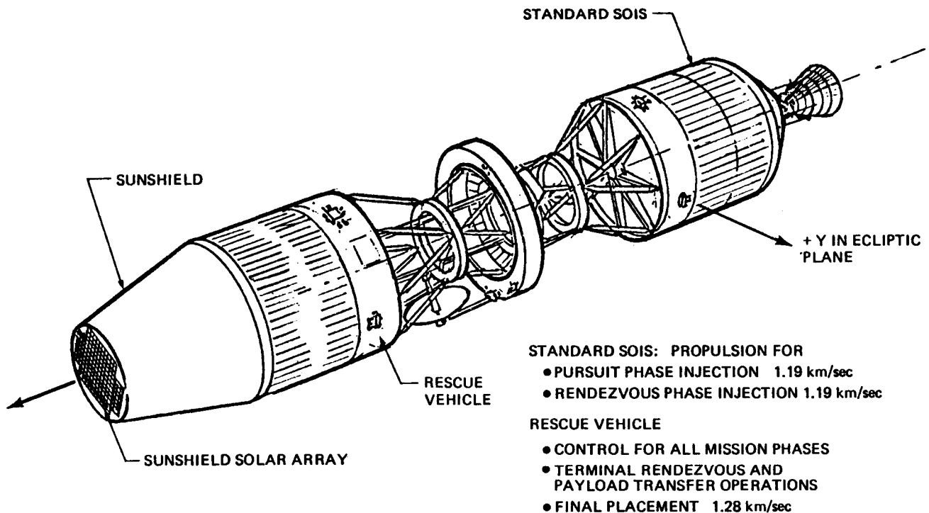
Figure 7.4.2-6. Pursuit Vehicle Configuration
