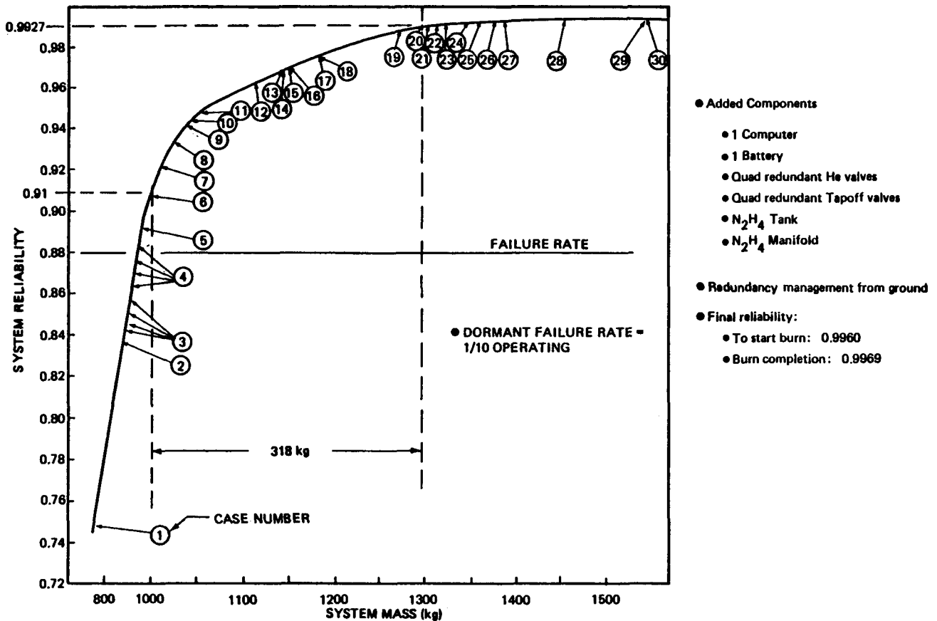
Figure 4.3-6. SOIS Mass and Reliability Optimization Study Results
