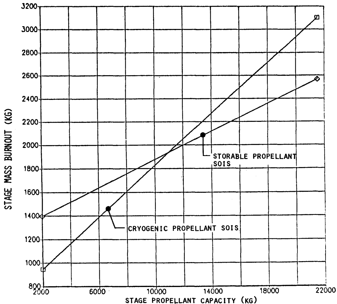
Figure 4.3-4. Parametric Mass Characterization of SOIS Configuration
