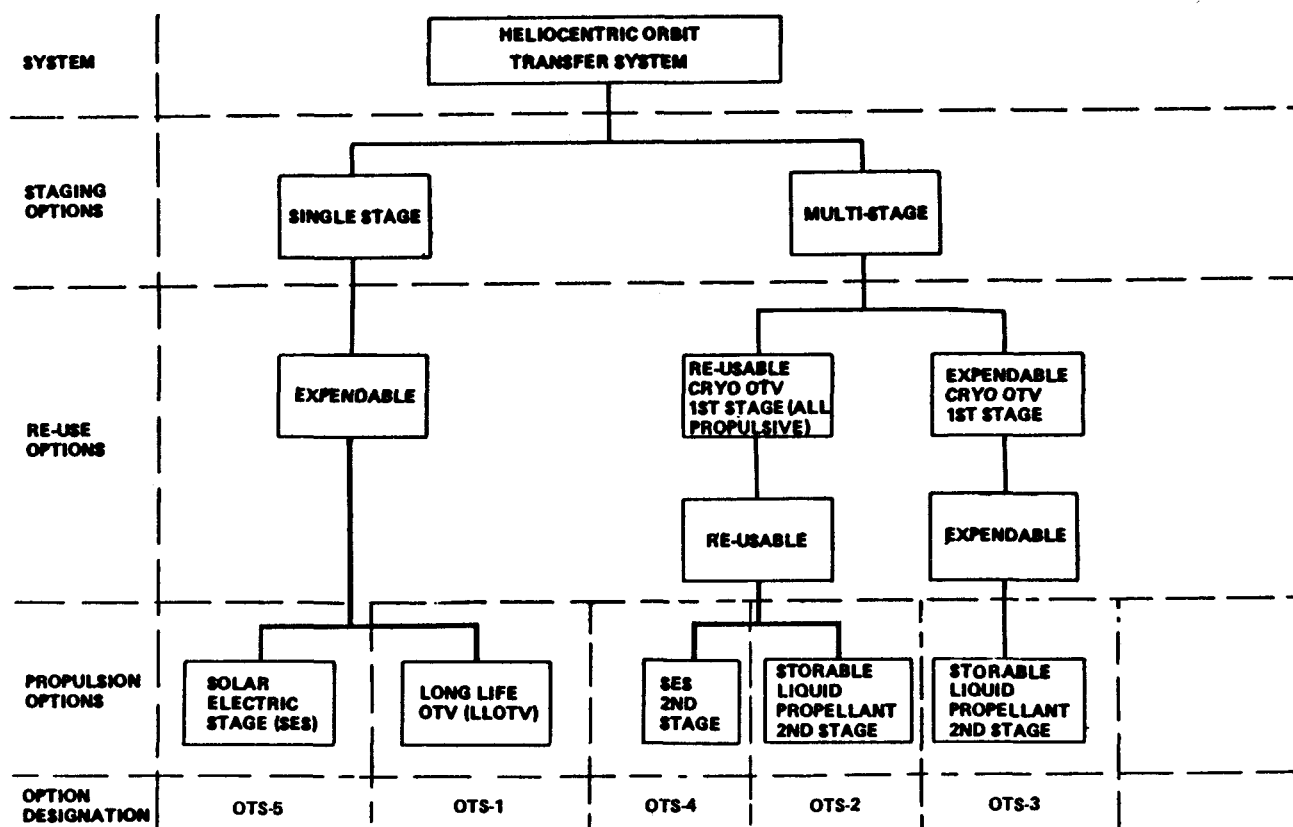
Figure 4.3-1. Orbit Transfer System for Low-Launch-Rate Systems
