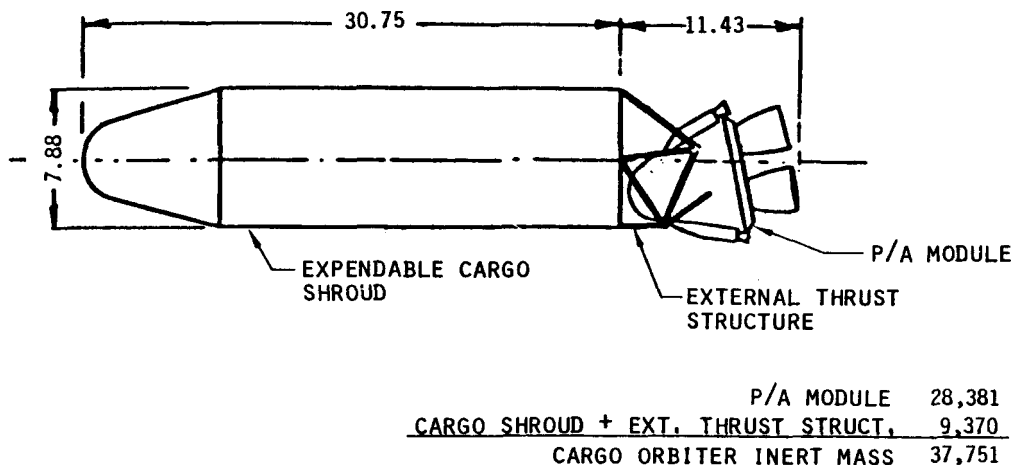
Figure 7.3.2-2. Cargo Orbiter General Arrangement
