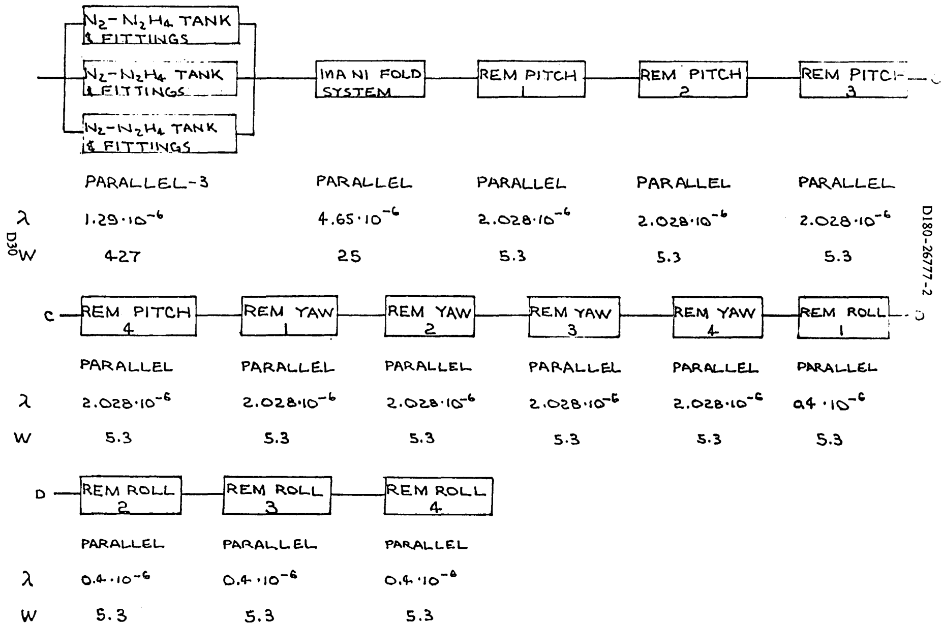
(FIG. 2.1) REACTION CONTROL SUBSYSTEM
