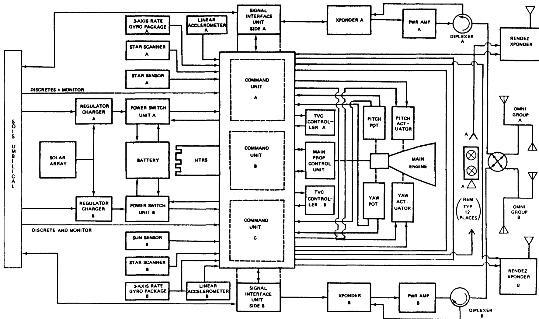
Figure 7.4.1-6. SOIS Avionics Block Diagram
