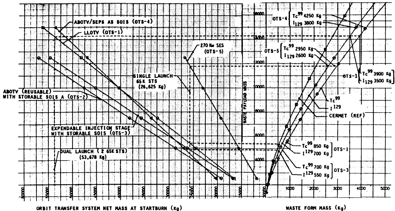
Figure 4.4-2. Parametric Performance Characteristics of Orbit Transfer Systems for Cermet, PbI_2^{129} , and Tc^{99} Waste Forms
