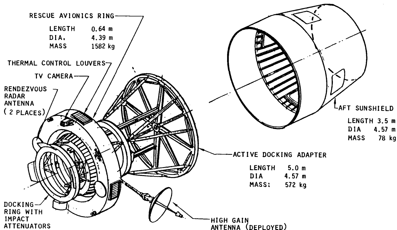
Figure 7.4.2-2. SOIS Rescue Kit
