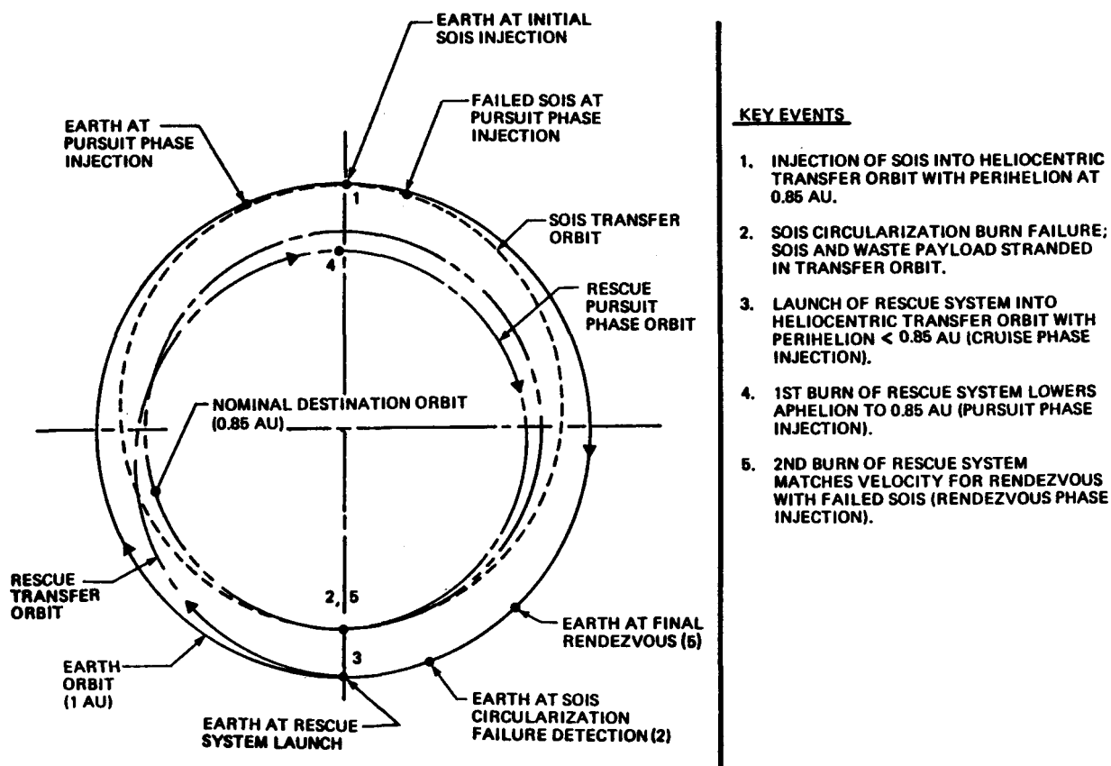
Figure 6.2-2. Deep-Space Rescue Trajectory Schematic
