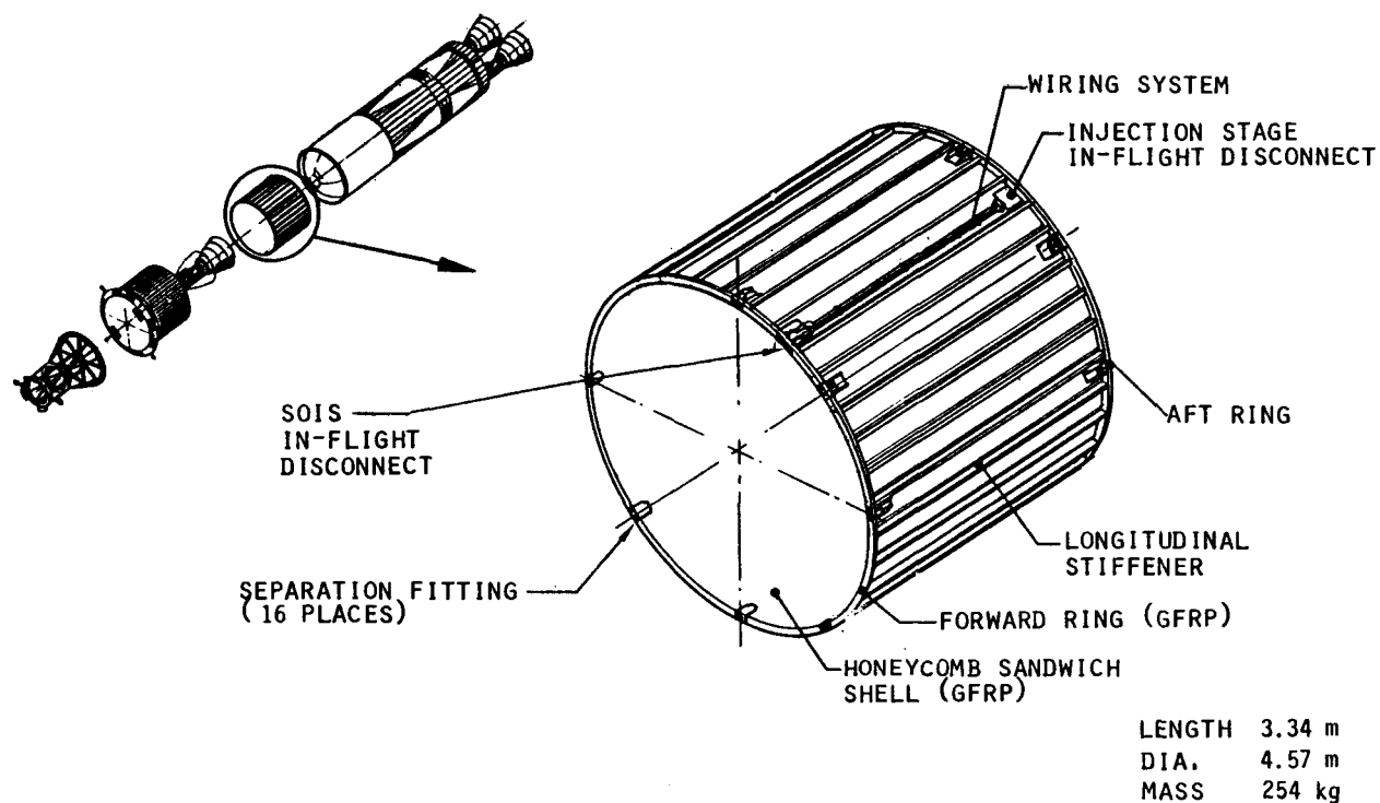
Figure 7.4.1-4. Interstage Assembly General Arrangement
