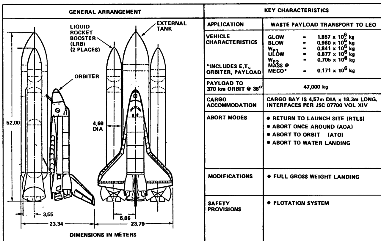
Figure 7.3.1-1. Uprated STS General Arrangement
