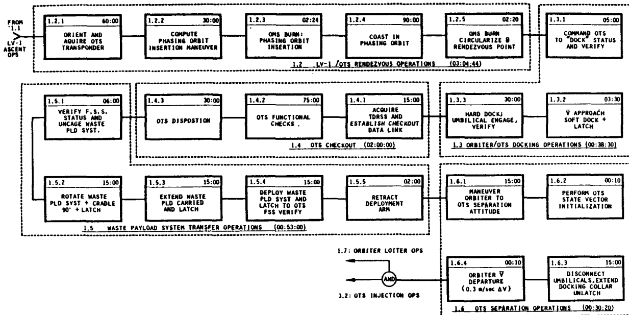
Figure 8.3-3. Orbiter Leo Operations
