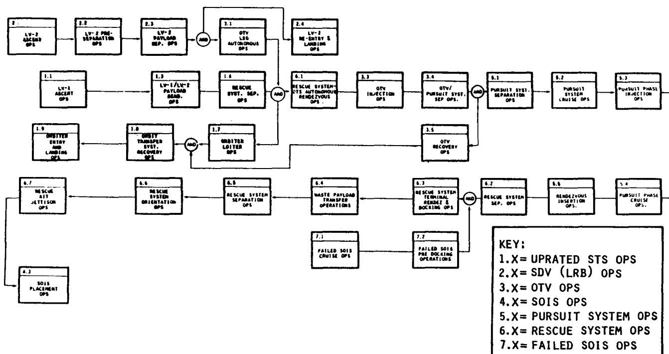
Figure 8.4-1. Nominal Deep-Space Rescue Mission Operations Flow Diagram
