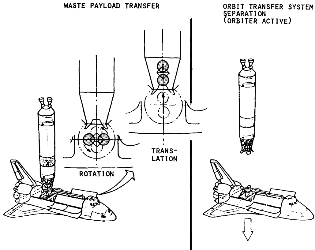
Figure 7.5-2. Flight Support System Operation Detail
