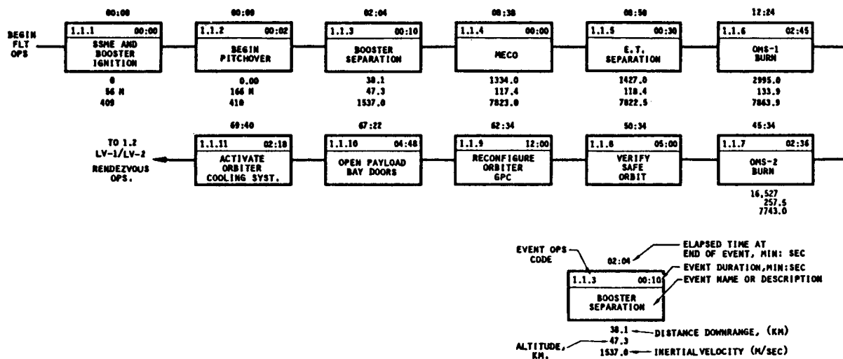
Figure 8.3-2. Orbiter Ascent Operations
