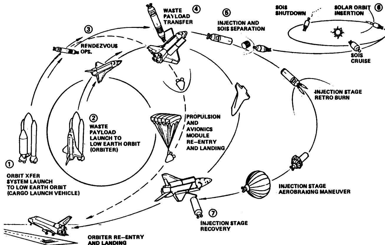
Figure 5.2-2. Reference Space System Mission Operations Summary
