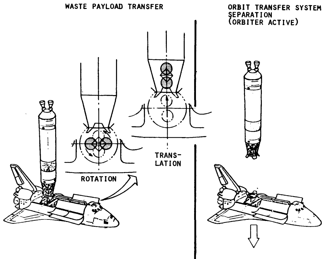
Figure 8.3-5. Waste Payload Transfer Operation Detail
