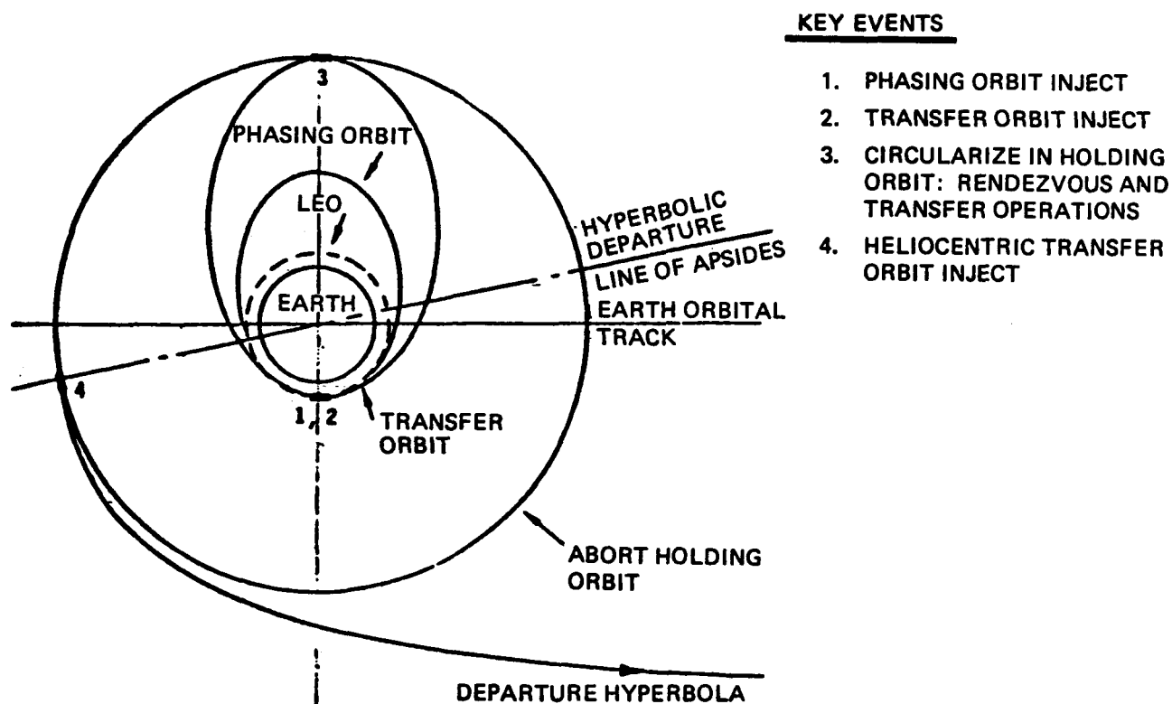
Figure 6.2-1. High Earth Orbit Rescue Trajectory Schematic
