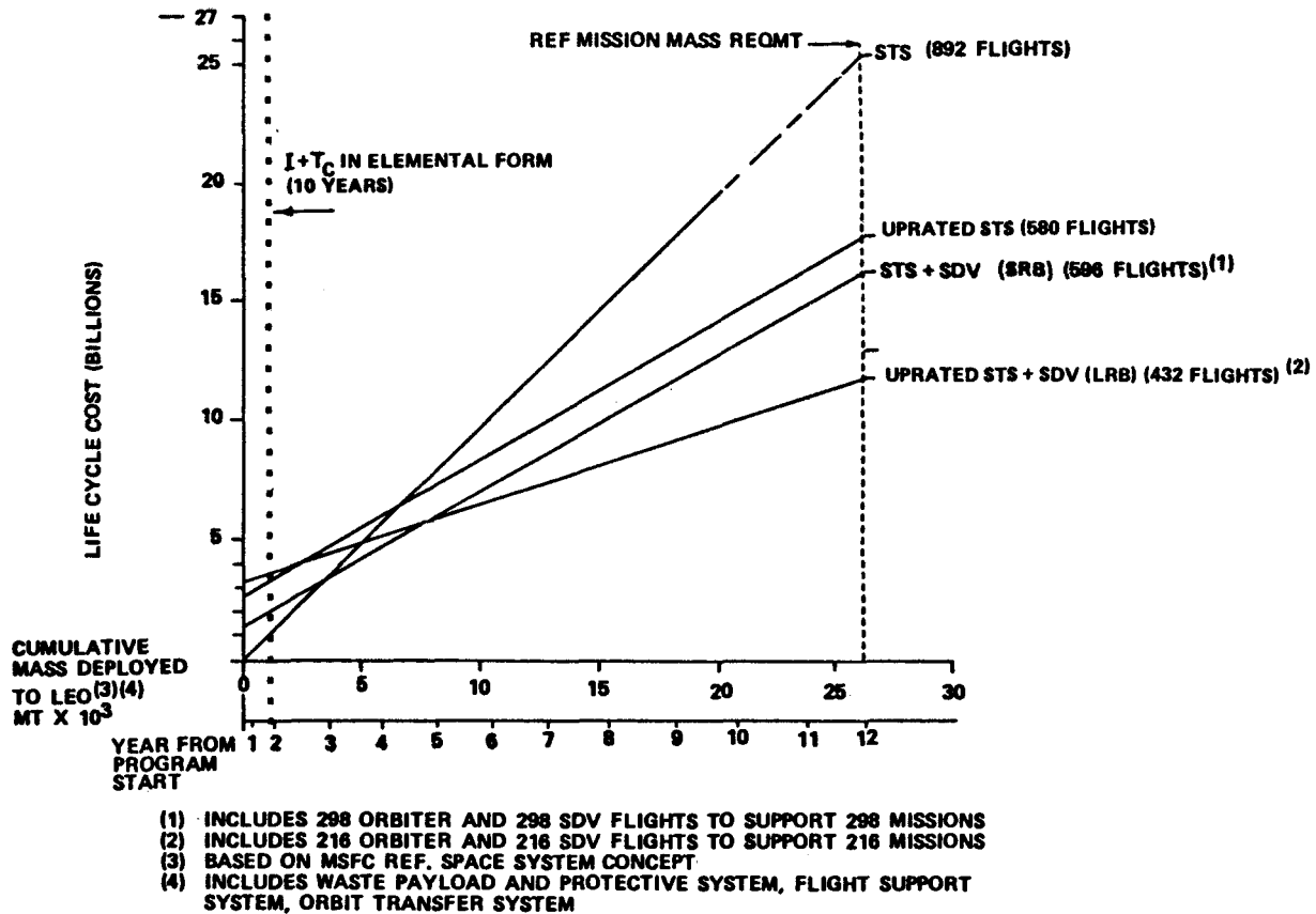
Figure 4.2-2. Launch Vehicle Life Cycle Cost Comparison
