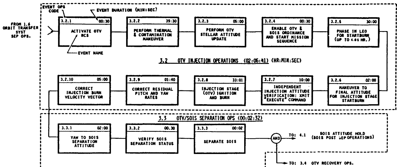
Figure 8.3-6. Nominal Delivery Mission OTV Injection Operations
