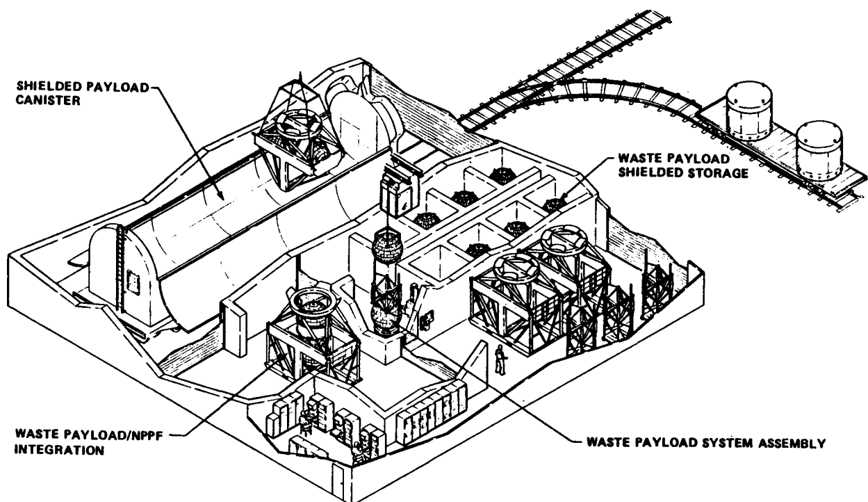
Figure 7.2.1-1. Nuclear Payload Processing Facility (NPPF)
