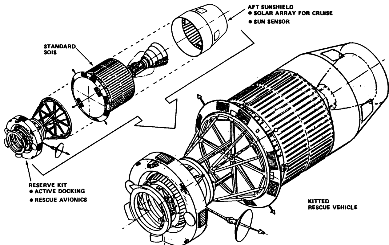
Figure 7.4.2-4. Rescue Vehicle Assembly
