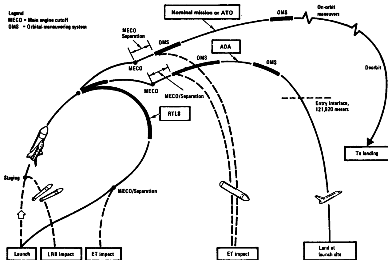
Figure 7.3.1-2. Up-rated STS Intact Abort Options
