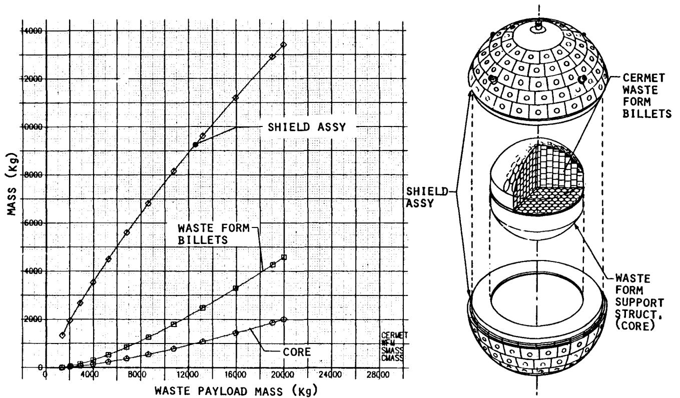
Figure 4.1-2. Waste Payload Parametric Mass Breakdown—Cermets
