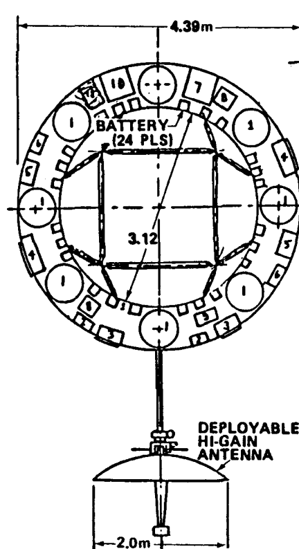
Figure 7.4.2-3. Rescue Avionics Ring
