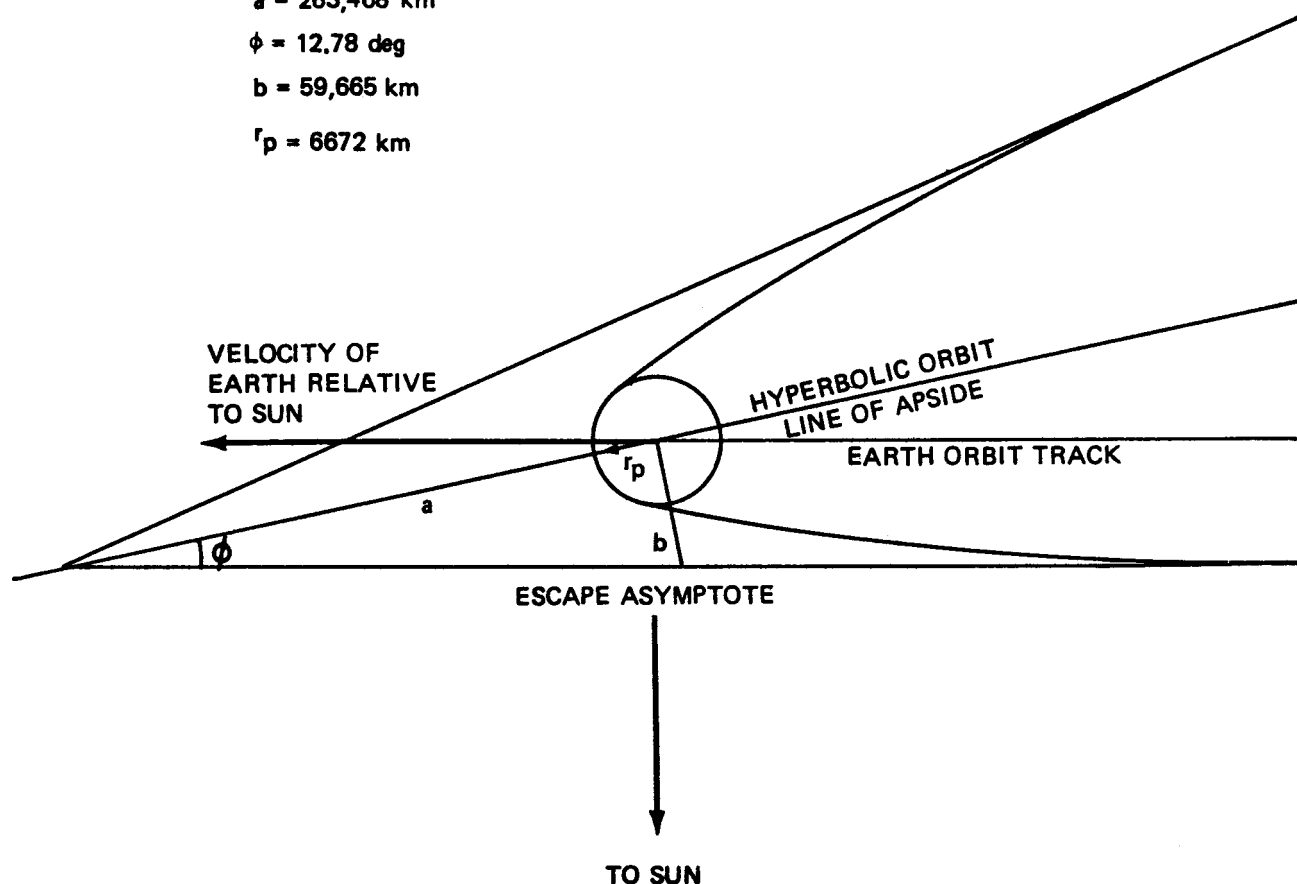
Figure 6.1-4. Reference Mission Departure Hyperbola Geometry
