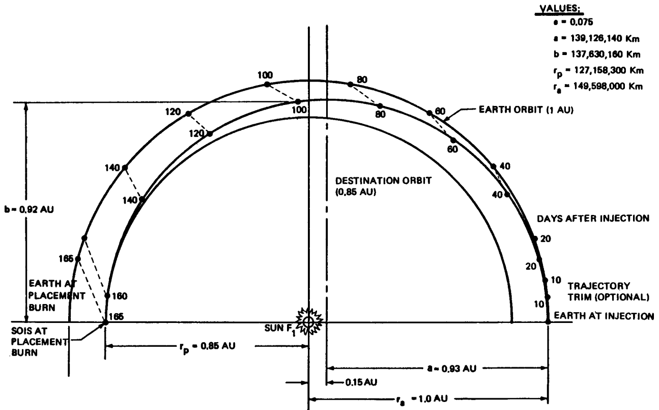
Figure 6.1-7. Placement Mission Profile
