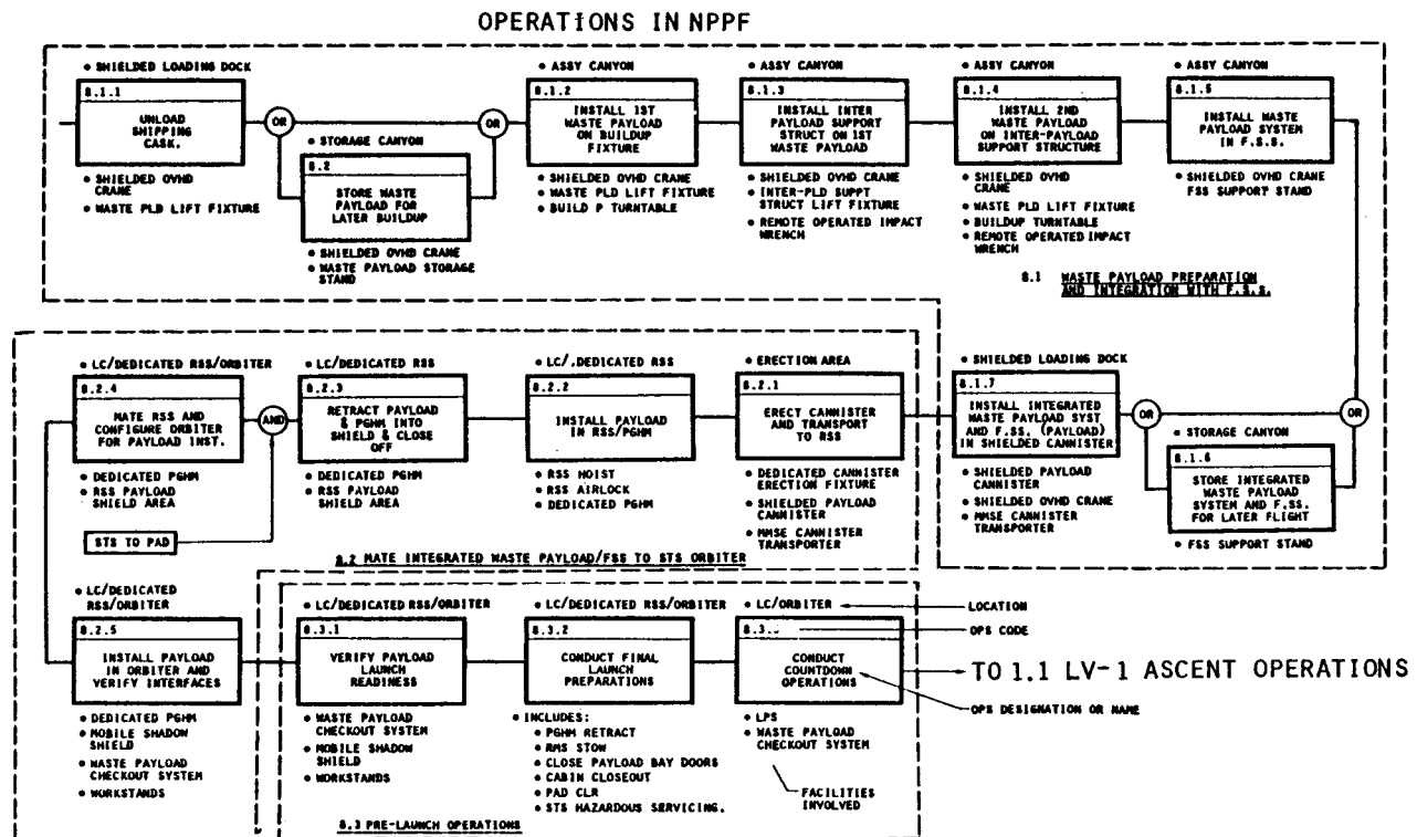
Figure 8.2-1. Launch Site Operations Flow Diagram
