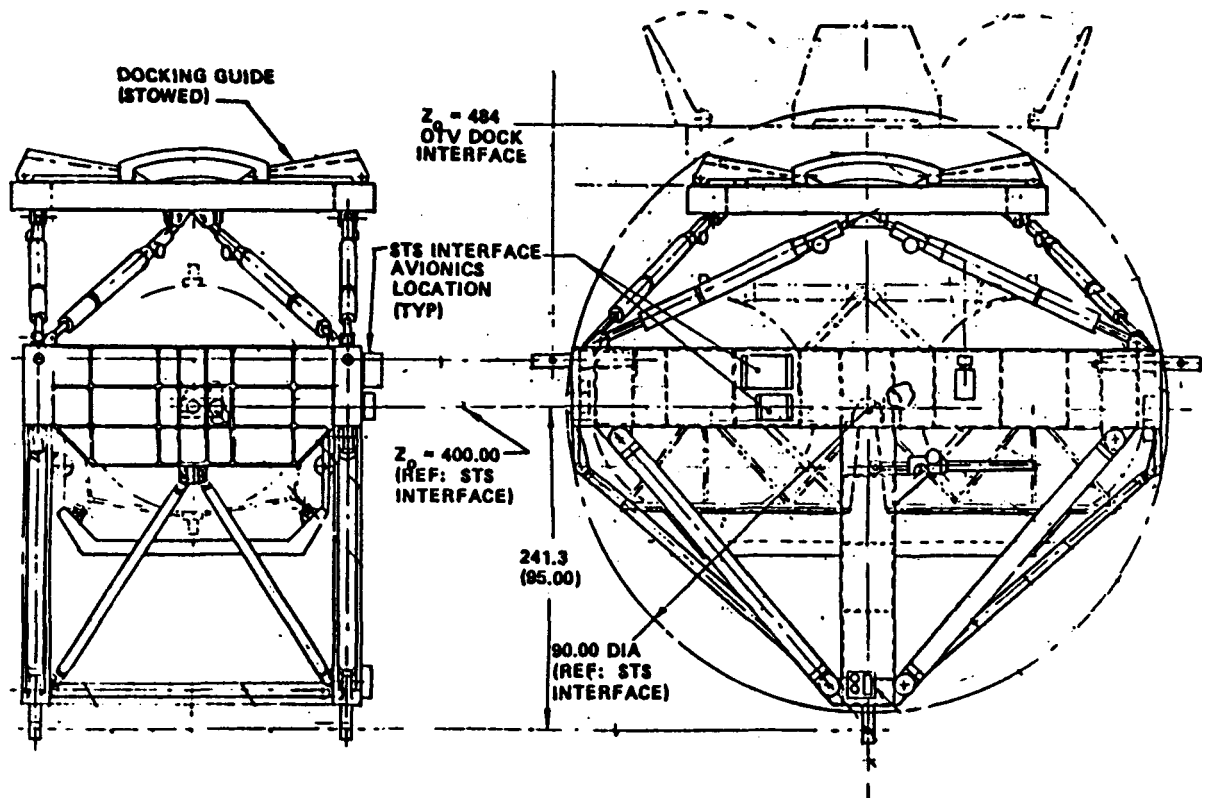
Figure 7.5-1. Flight Support System General Arrangement
