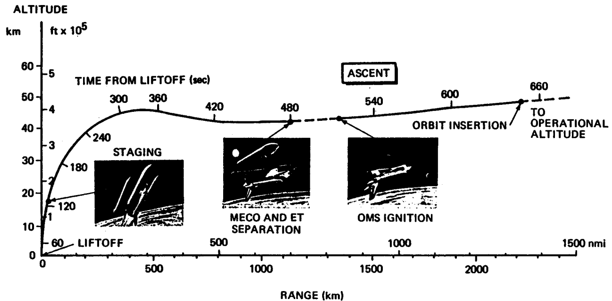
Figure 6.1-1. Uprated STS Ascent Trajectory Schematic
