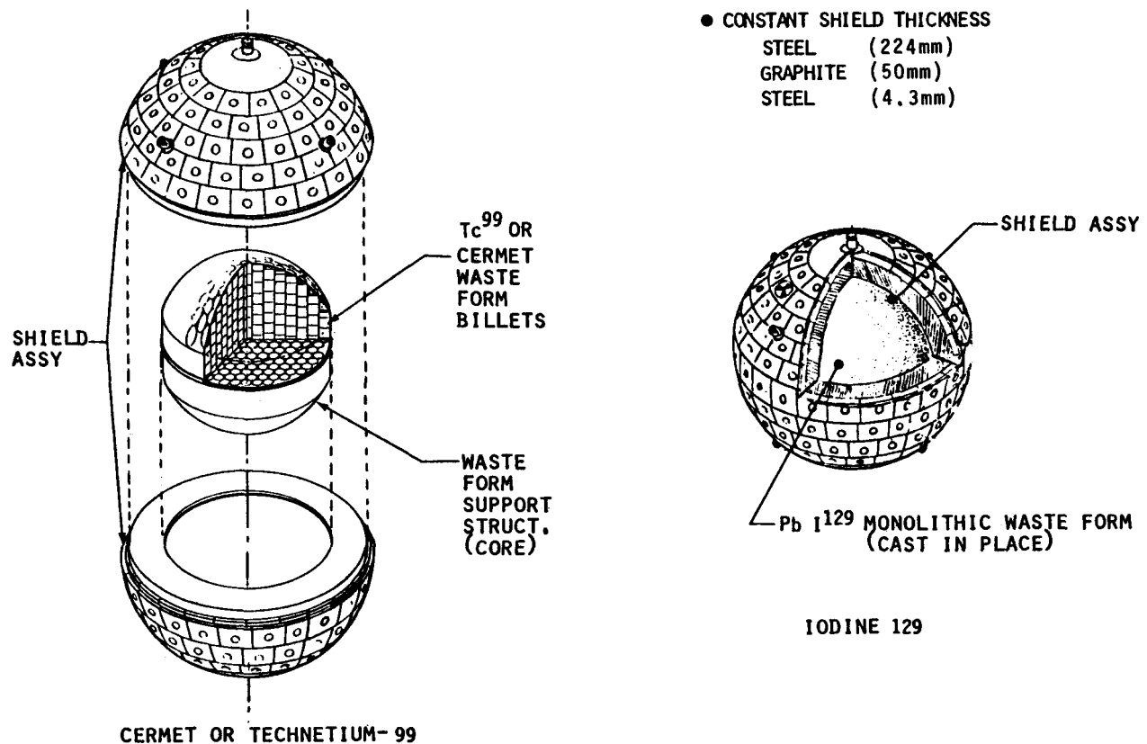
Figure 4.1-1. Waste Payload Configurations
