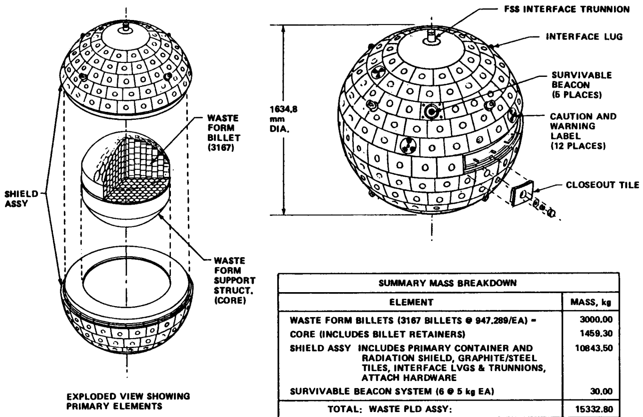
Figure 7.1.2-1. Waste Payload Assembly General Arrangement
