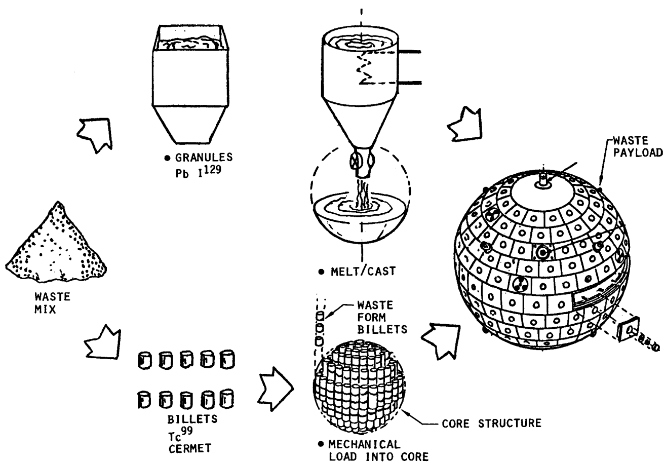
Figure 3.0-1. Waste Form Configurations
