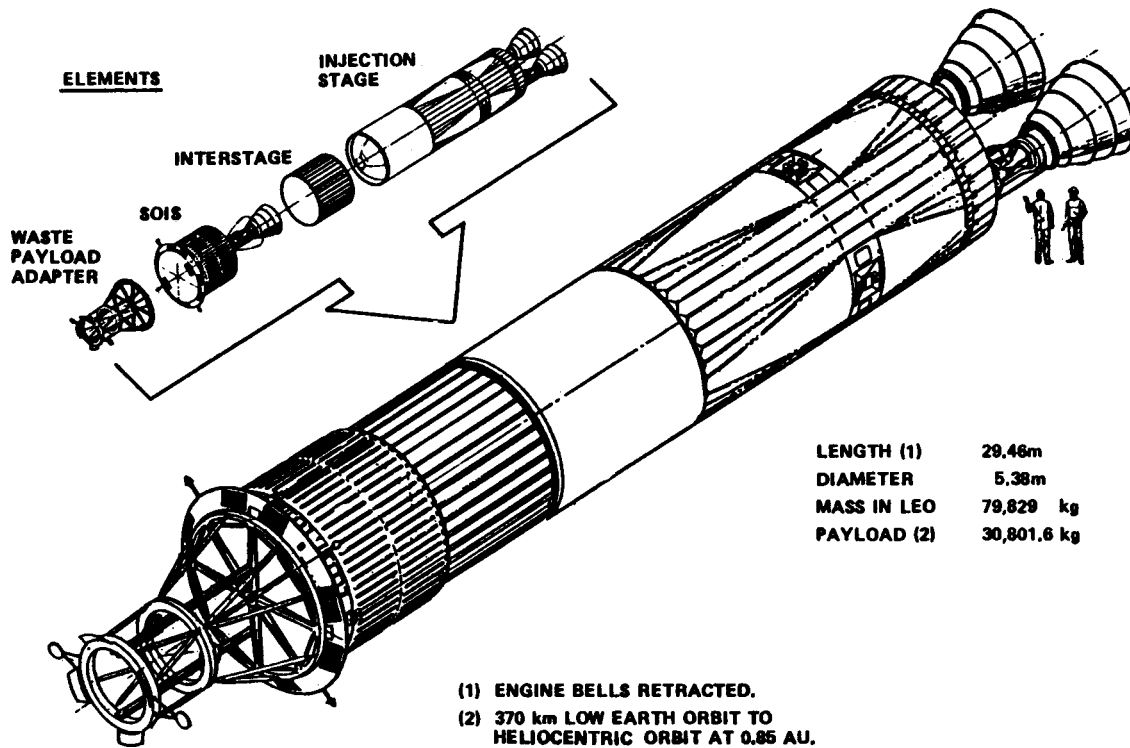
Figure 7.4.1-1. Orbit Transfer System General Arrangement
