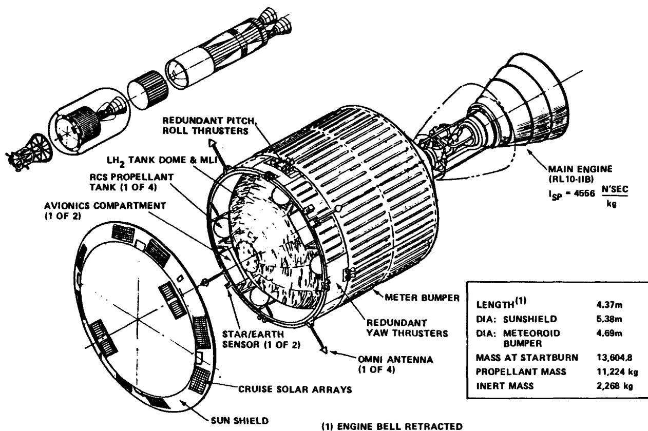
Figure 7.4.1-5. Solar Orbit Insertion Stage (SOIS) General Arrangement
