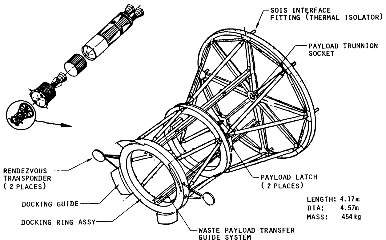
Figure 7.4.1-8. Payload Adapter Primary Elements
