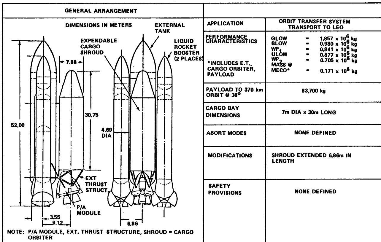
Figure 7.3.2-1. Shuttle-Derived Vehicle General Arrangement
