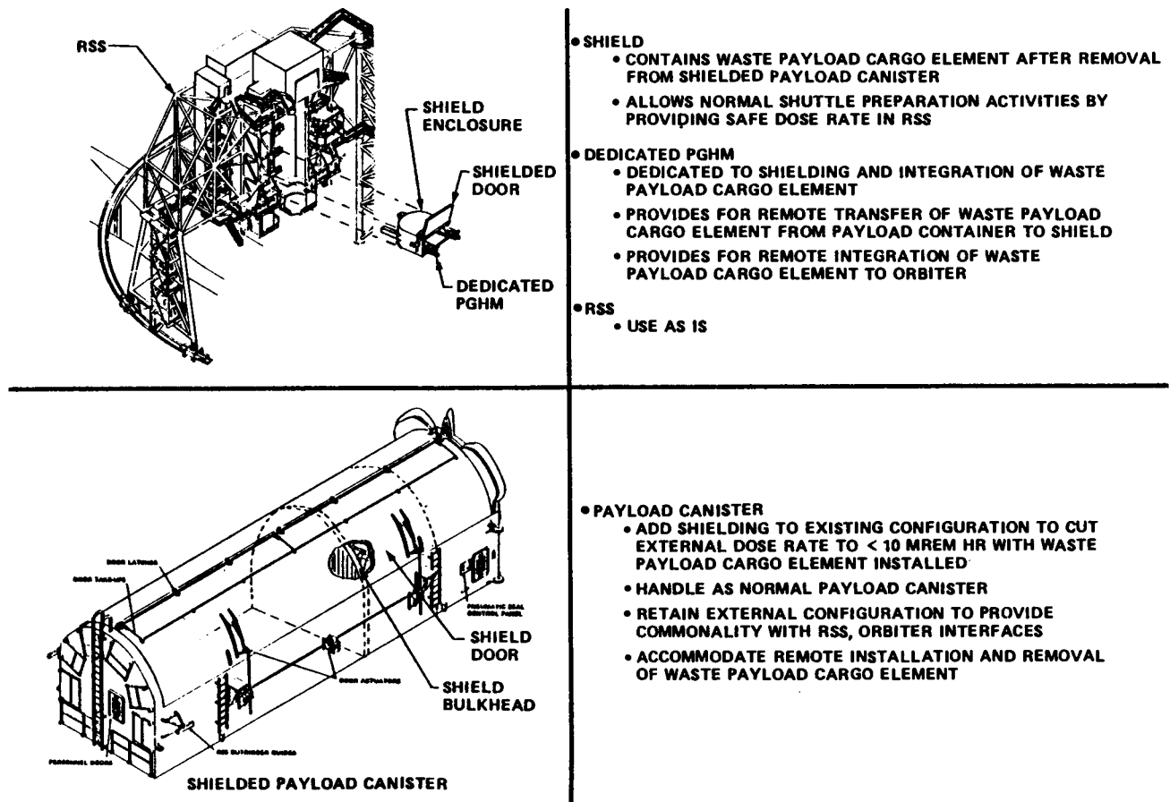
Figure 7.2.3-1. Specialized Waste Payload Cargo Integration Facilities From Modification of Existing STS Support Equipment
