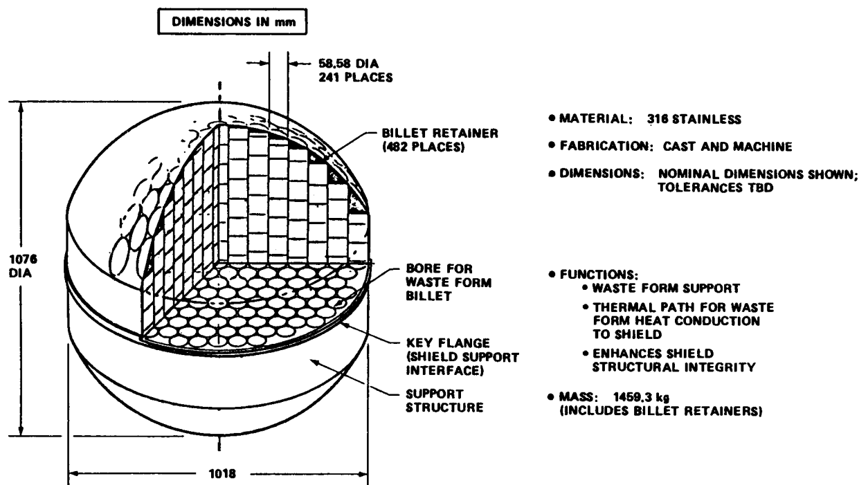
Figure 7.1.2-3. Waste Form Support Structure (Core) Configuration
