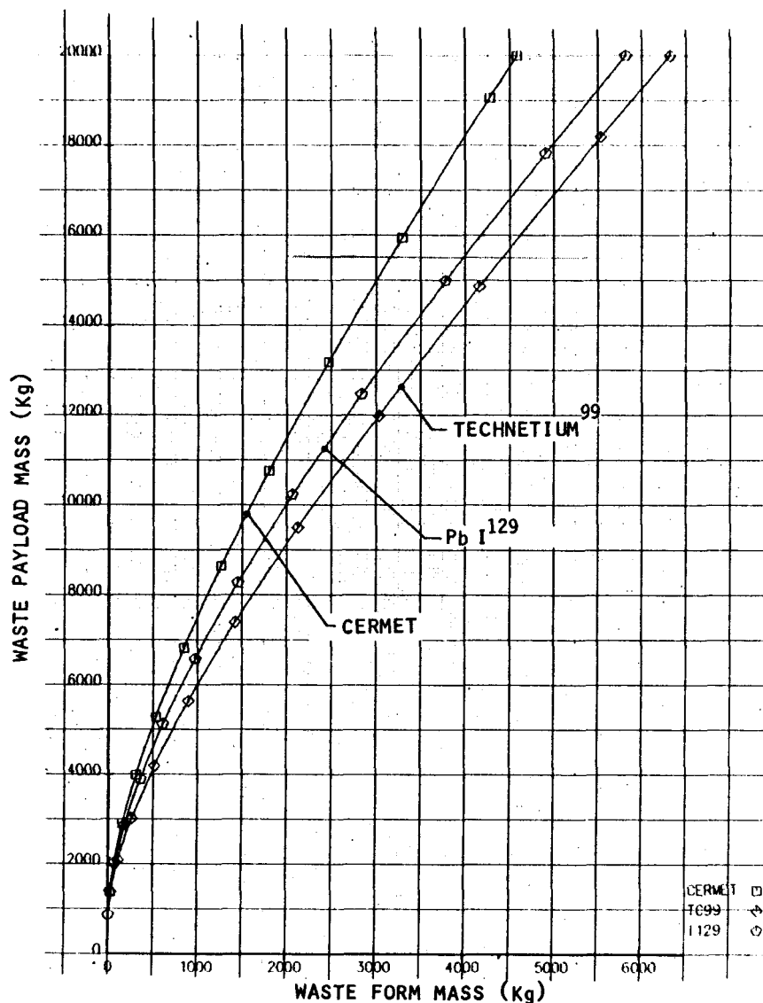
Figure 4.1-5. Complete Waste Payload Mass Versus Waste Form Mass
