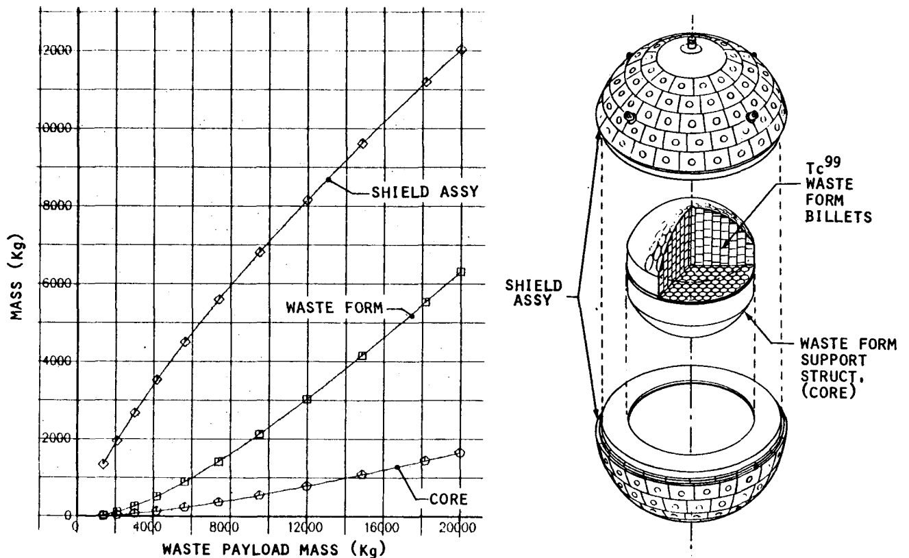
Figure 4.1-3. Waste Payload Parametric Mass Breakdown—Technetium 99
