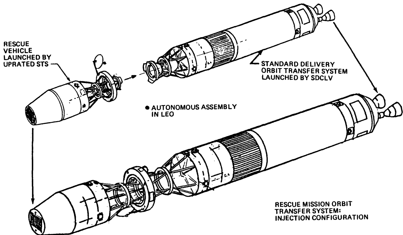
Figure 7.4.2-7. Injection Configuration of Rescue Orbit Transfer System
