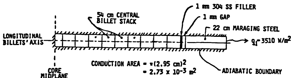
Figure 2.1. Cross-Section Depicting the Thermal Model for the Waste Core and the Maraging Shield.
