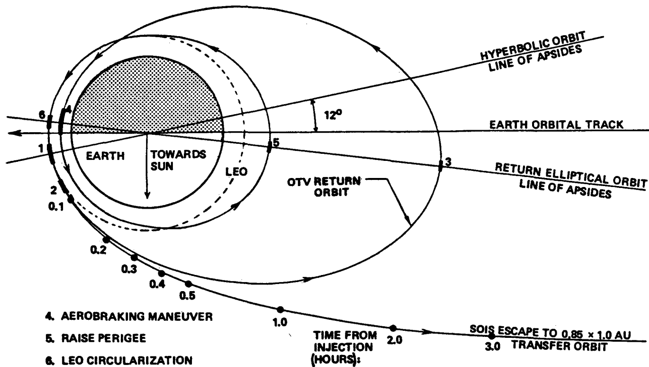
Figure 6.1-3. Injection Mission Profile Schematic
