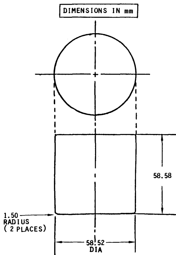
Figure 7.1.2-2. Waste Form Billet Configuration
