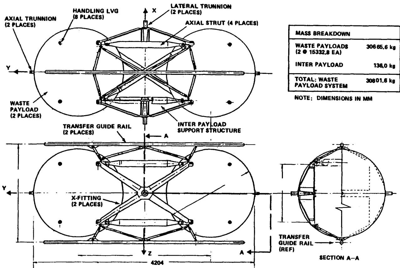
Figure 7.1-1. Waste Payload System General Arrangement
