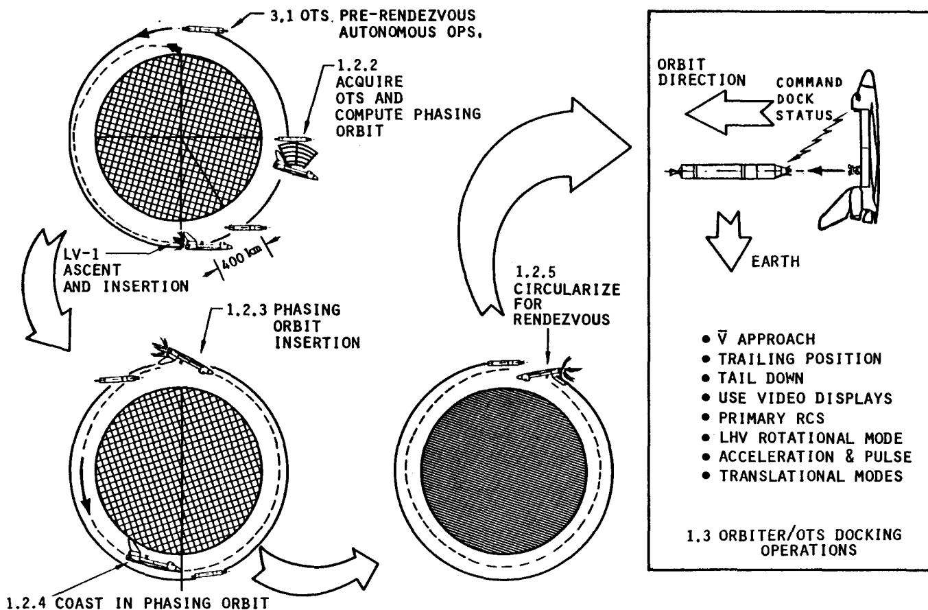
Figure 8.3-4. Leo Rendezvous and Docking Operations
