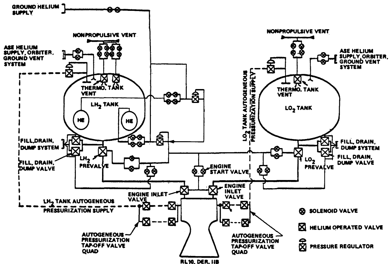
Figure 7.4.1-7. SOIS Main Propulsion System Schematic
