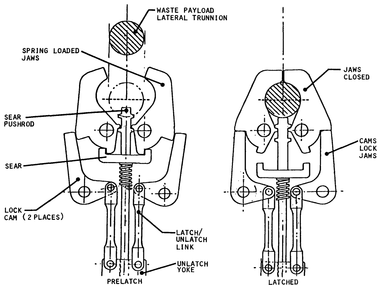
Figure 7.4.1-9. Payload Adapter Reversible Waste Payload Latch System
