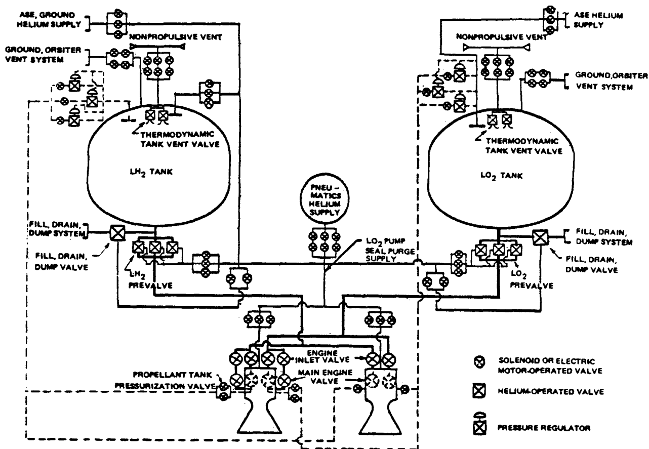
Figure 7.4.1-3. Main Engine Propulsion System Schematic
