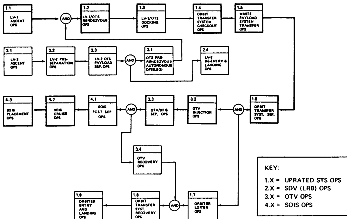
Figure 8.3-1. Nominal Waste Payload Delivery Mission Flow Diagram
