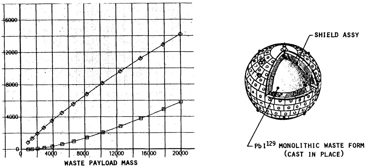
Figure 4.1-4. Waste Payload Parametric Mass Breakdown—Lead Iodide ( \text{Pb I}_2^{129} )
