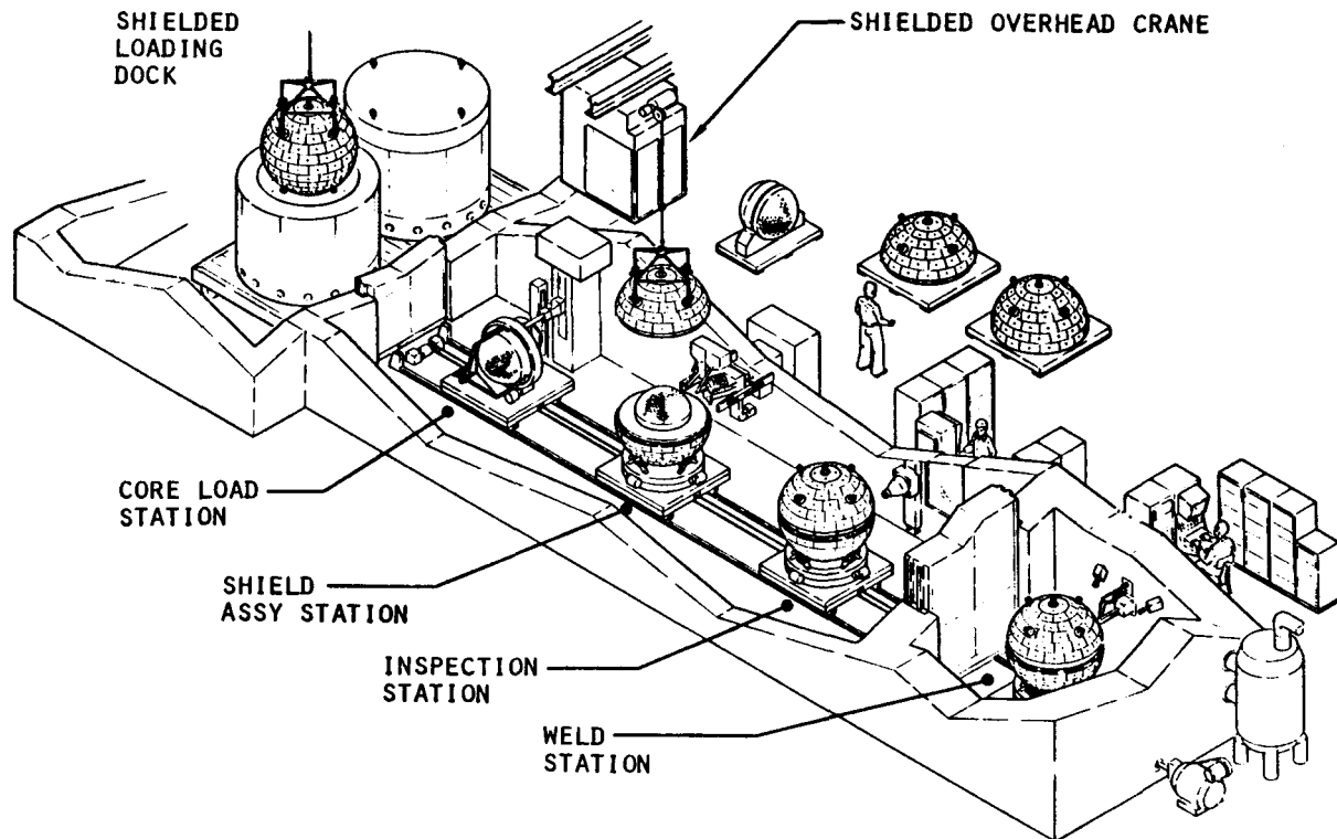
Figure 8.1-2. Conceptual Waste Payload Assembly Facility Schematic
