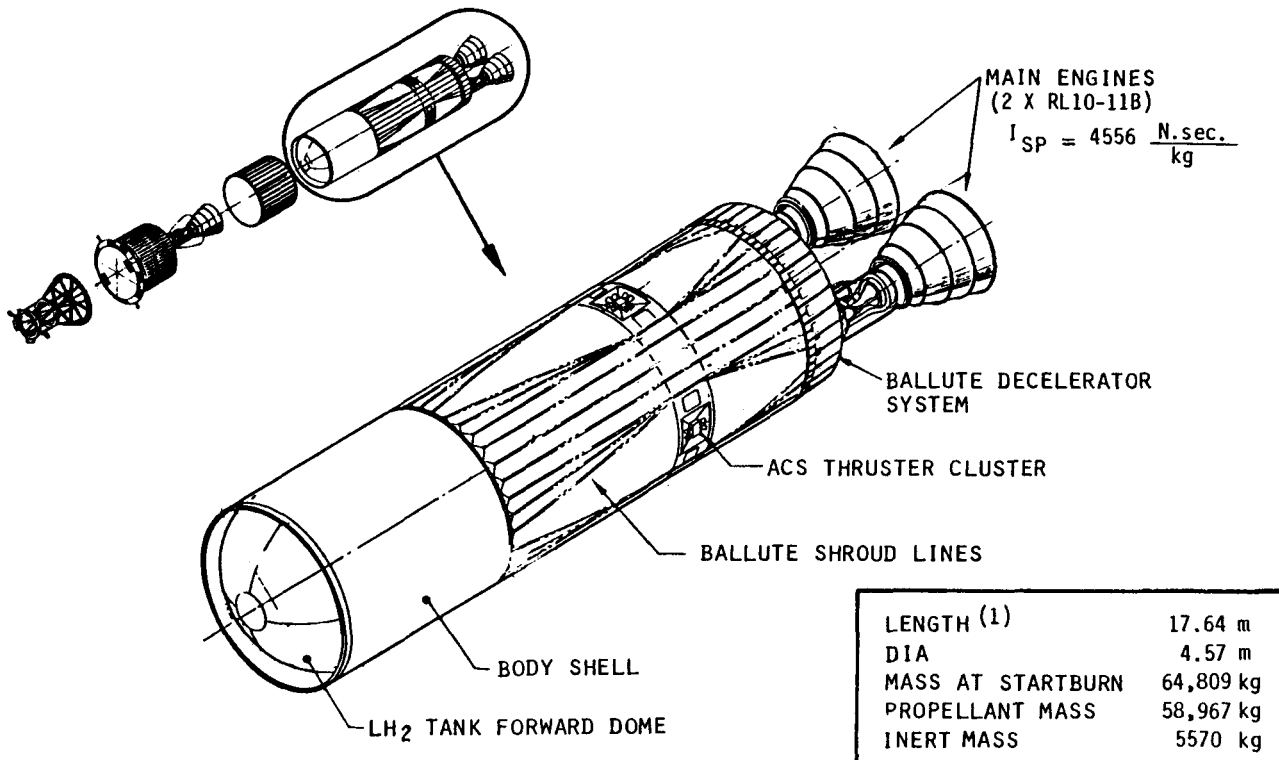
Figure 7.4.1-2. Injection Stage General Arrangement
