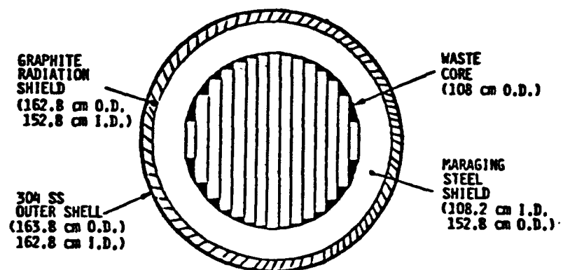
Figure 1.3. Cross-section of Nuclear Waste Disposal Vessel (waste billets not shown)
