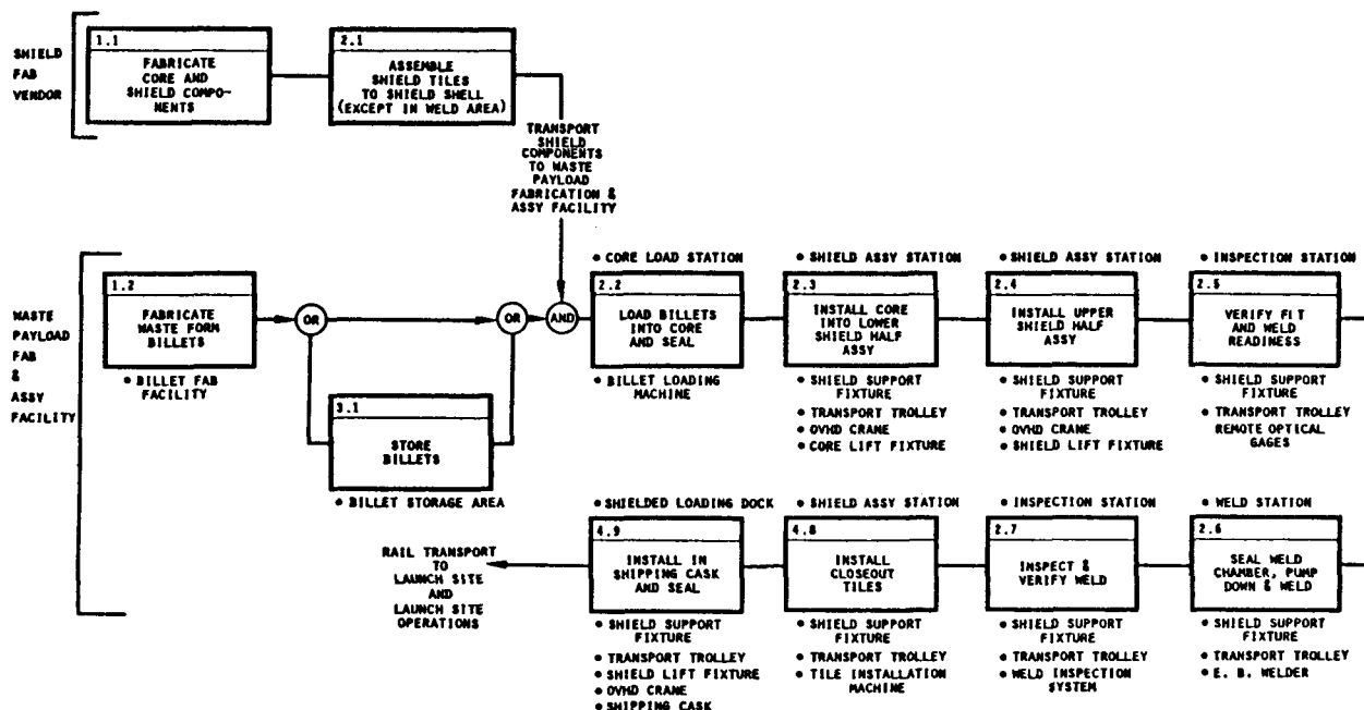
Figure 8.1-1. Waste Payload Fabrication and Assembly Flow Diagram
