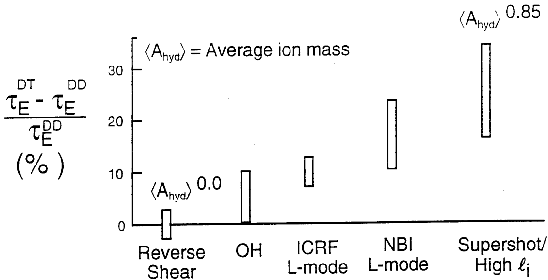
Fig.3. Comparison of the percentage increase in comparable D and D-T plasmas, for the confinement time in reverse shear, ICRF, OH L-mode, supershots and high \ell_i regimes. The results are shown for an average mass of the hydrogenic ion of 2.5.
