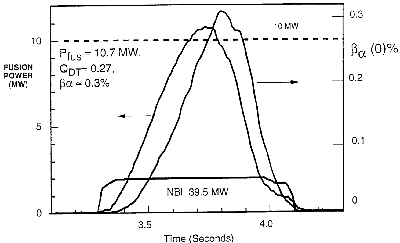
Fig. 1. Time evolution of the DT fusion power and beta alpha from a shot producing the highest instantaneous power of 10.7 MW at 39.5 MW of input power for an instantaneous Q of 0.27.
