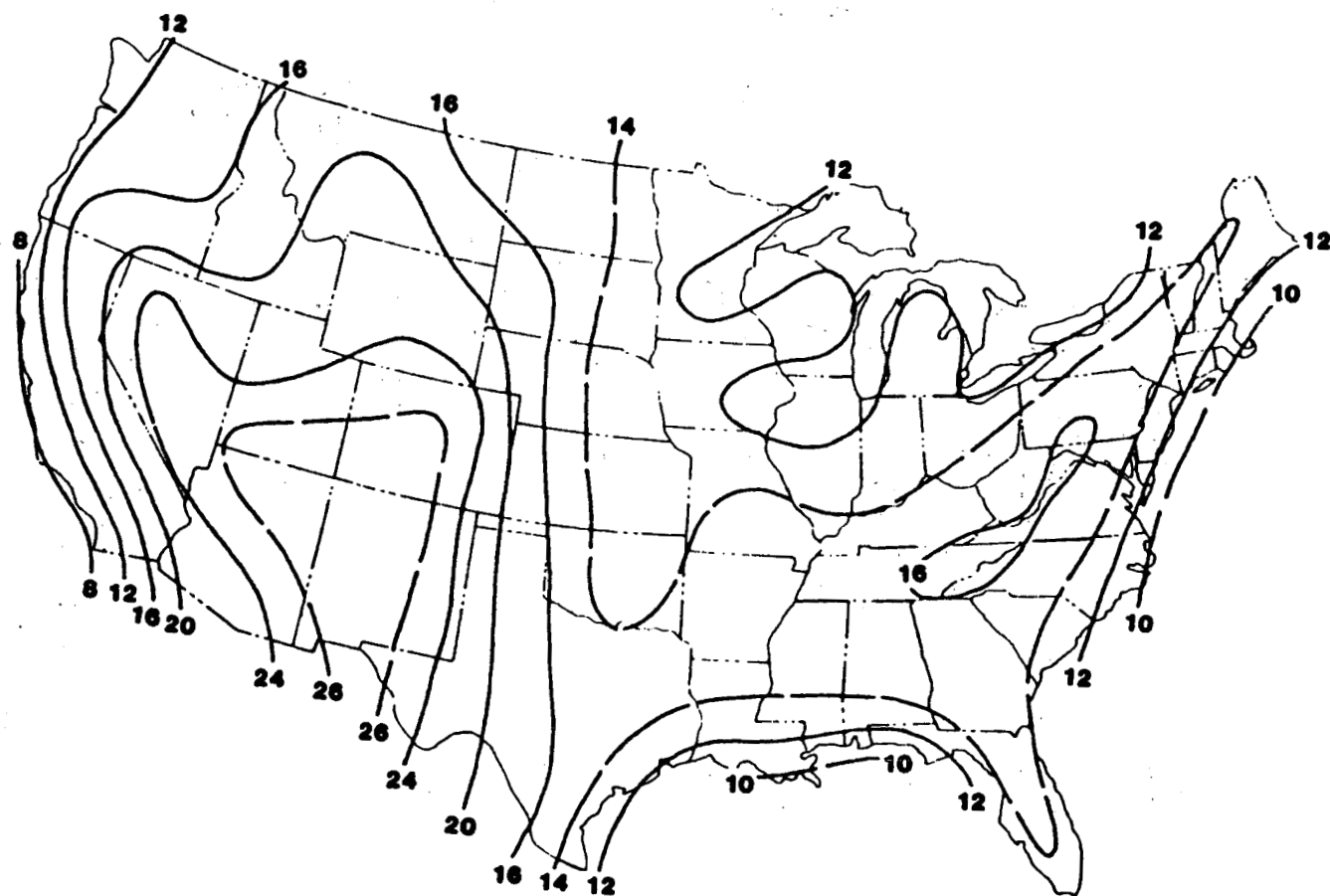
Figure A.3-1 Isopleths ( m \times 10^{-2} ) of Mean Annual Afternoon Mixing Heights. From reference [5].
