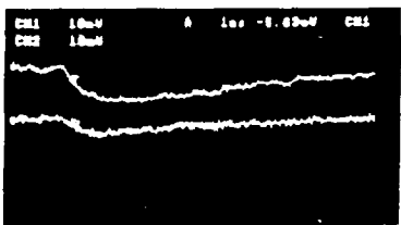
Figure 9. Simultaneous pulses from thermistors a and b. The upper trace in each photograph is from thermistor b, and the lower trace is from thermistor a. The X-rays were incident on the region between the two thermistors. The pulse height appears to be dependent on the interaction distance from the thermistor.
