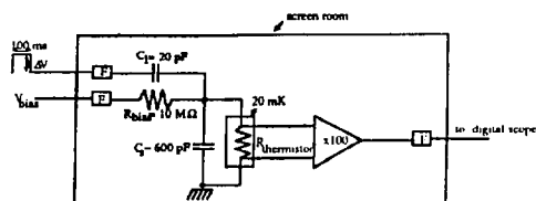
Figure 3. Equivalent electrical circuit for a thermistor in our experiment
