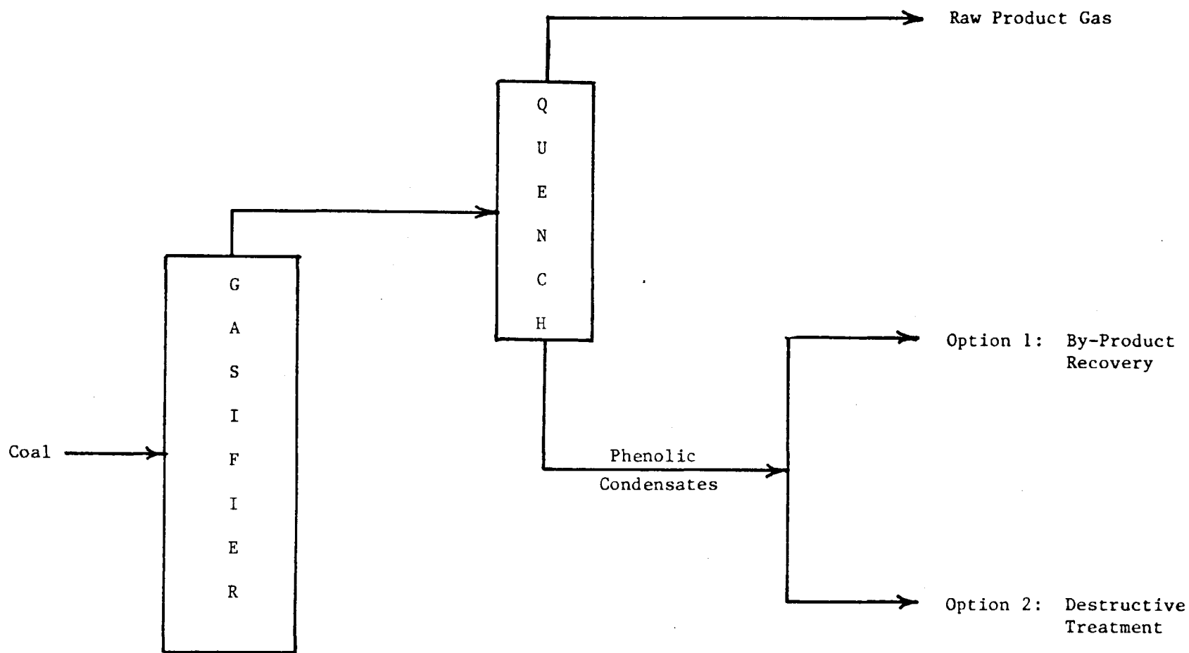
Figure 1. Basic production and processing patterns of phenols during coal gasification.
