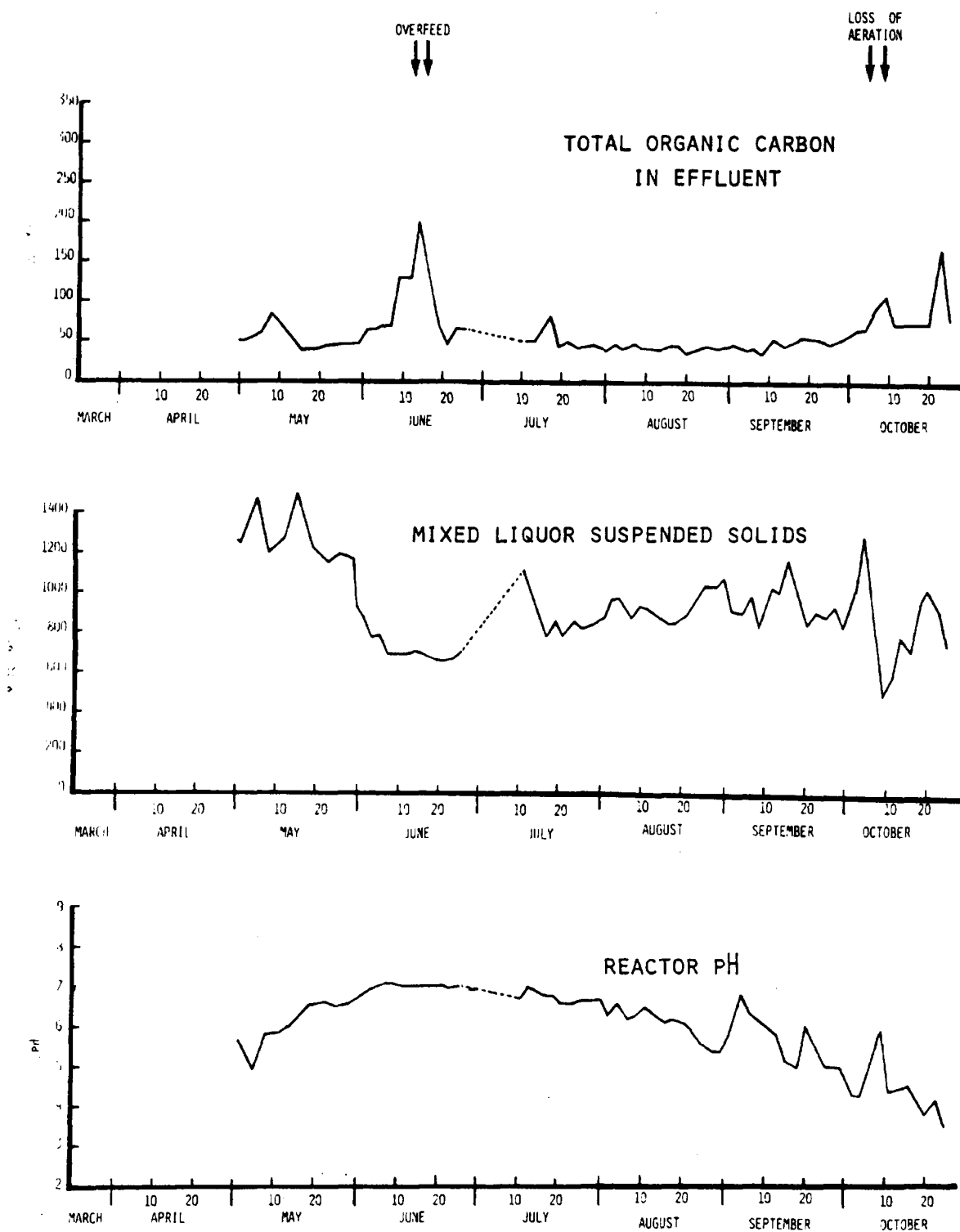
Figure 4. Performance characteristics of Reactor 3 with 20-day residence time.
