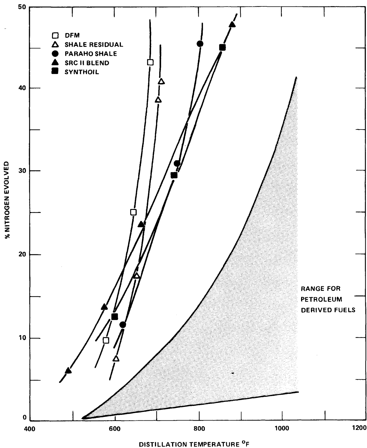
Figure 7. Fuel nitrogen volatility as determined by vacuum distillation. 16
