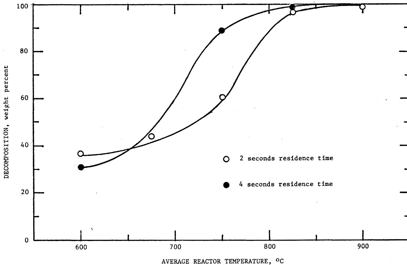
Figure 7. Measured ortho-cresol decomposition as a function of average reactor temperature for 2 and 4 s nominal residence time.
