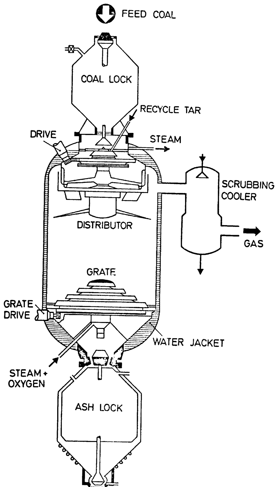
Figure A-3. Lurgi pressure gasifier.
