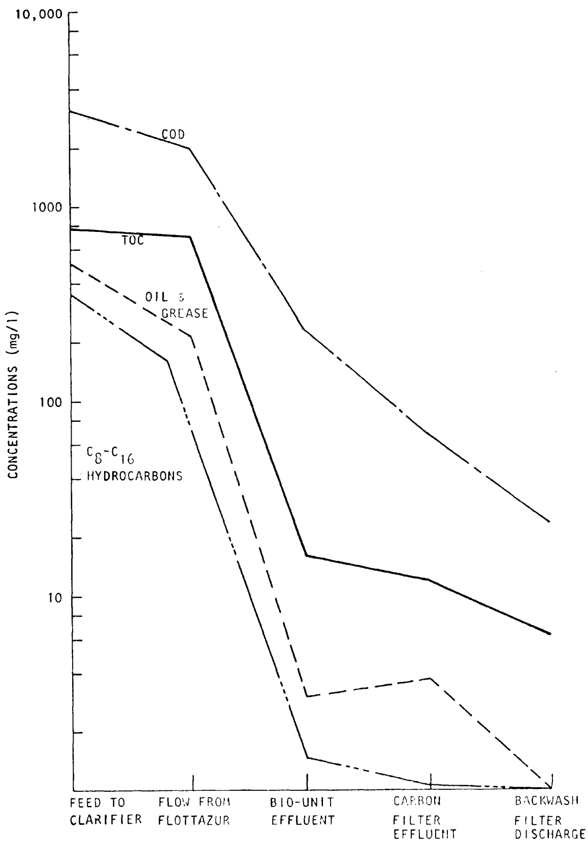
Figure 6. Effects of the wastewater treatment process on organics.
