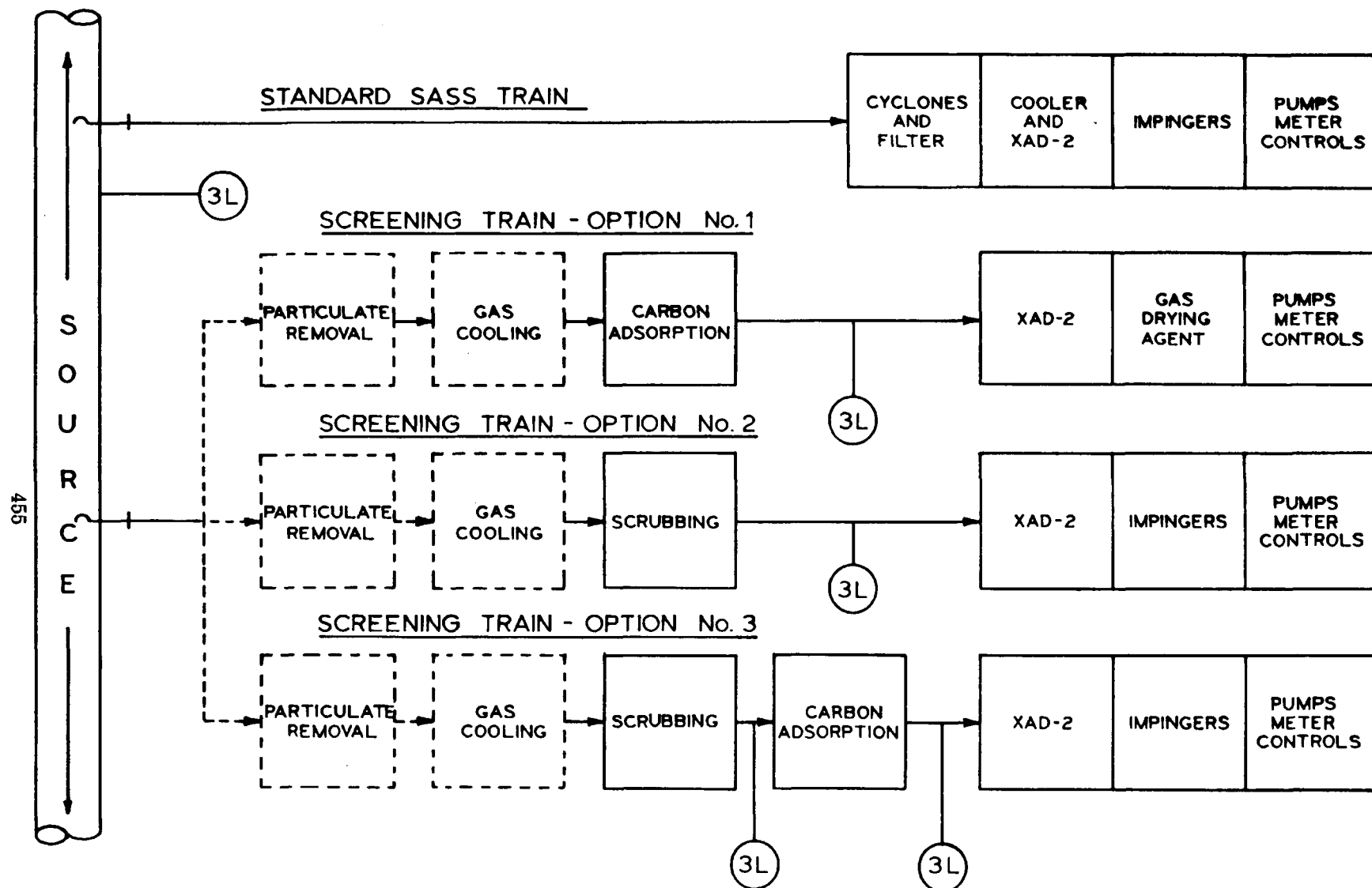
Figure 11. Screening train options.
