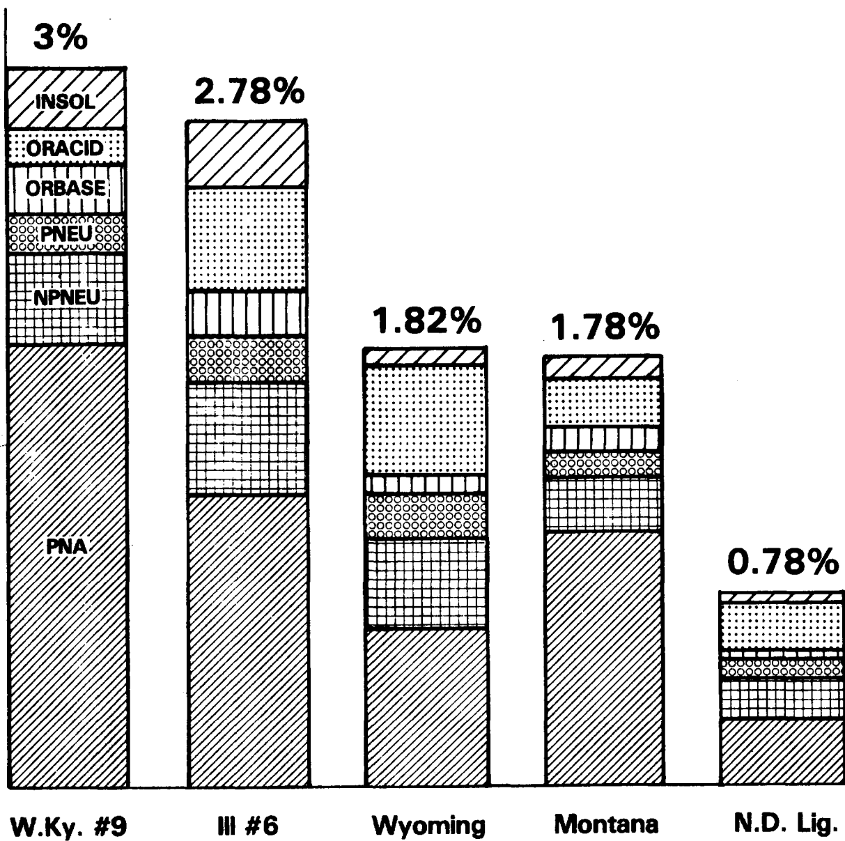
Figure 3. Tar partitions.
