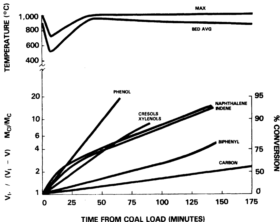
Figure 7. Pollutant kinetics.
