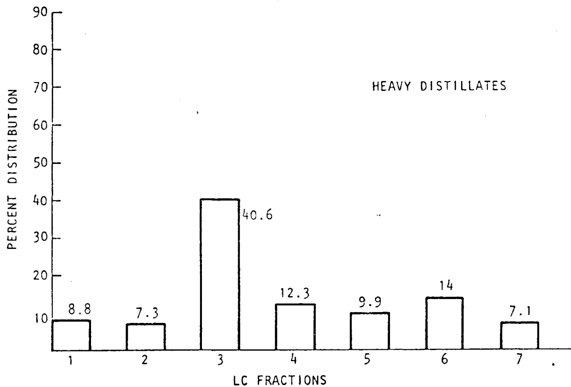
Figure 10. Relative distribution of total organics in seven LC fractions.
