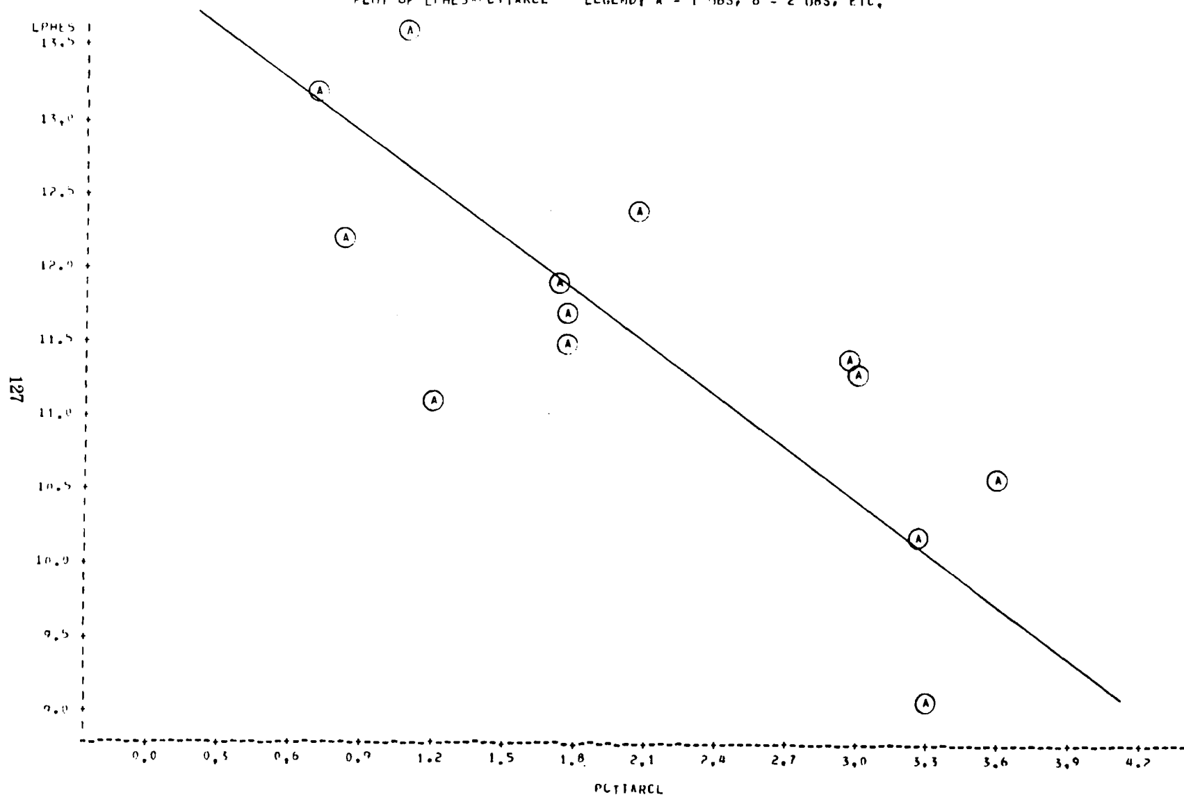
Figure 4. Tar/coal (weight percent) vs. phenol condensate concentration (log \mu\text{g/L} [MATE]).
