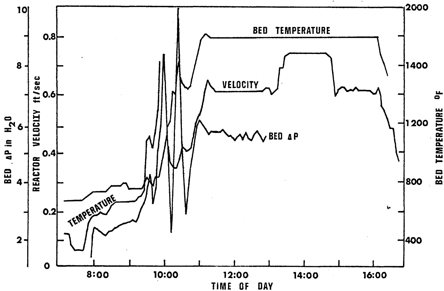
Figure 5. Startup and steady-state data for runs GO-5, GO-6, GO-7.
