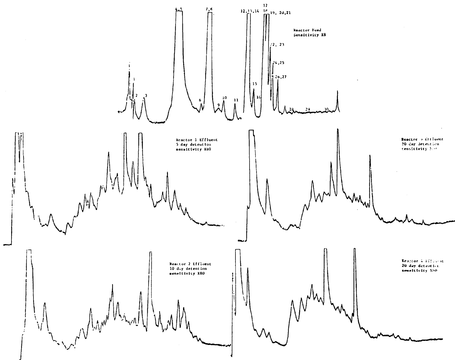
Figure 10. HPLC chromatograms of raw synthetic feed and reactor effluents.
