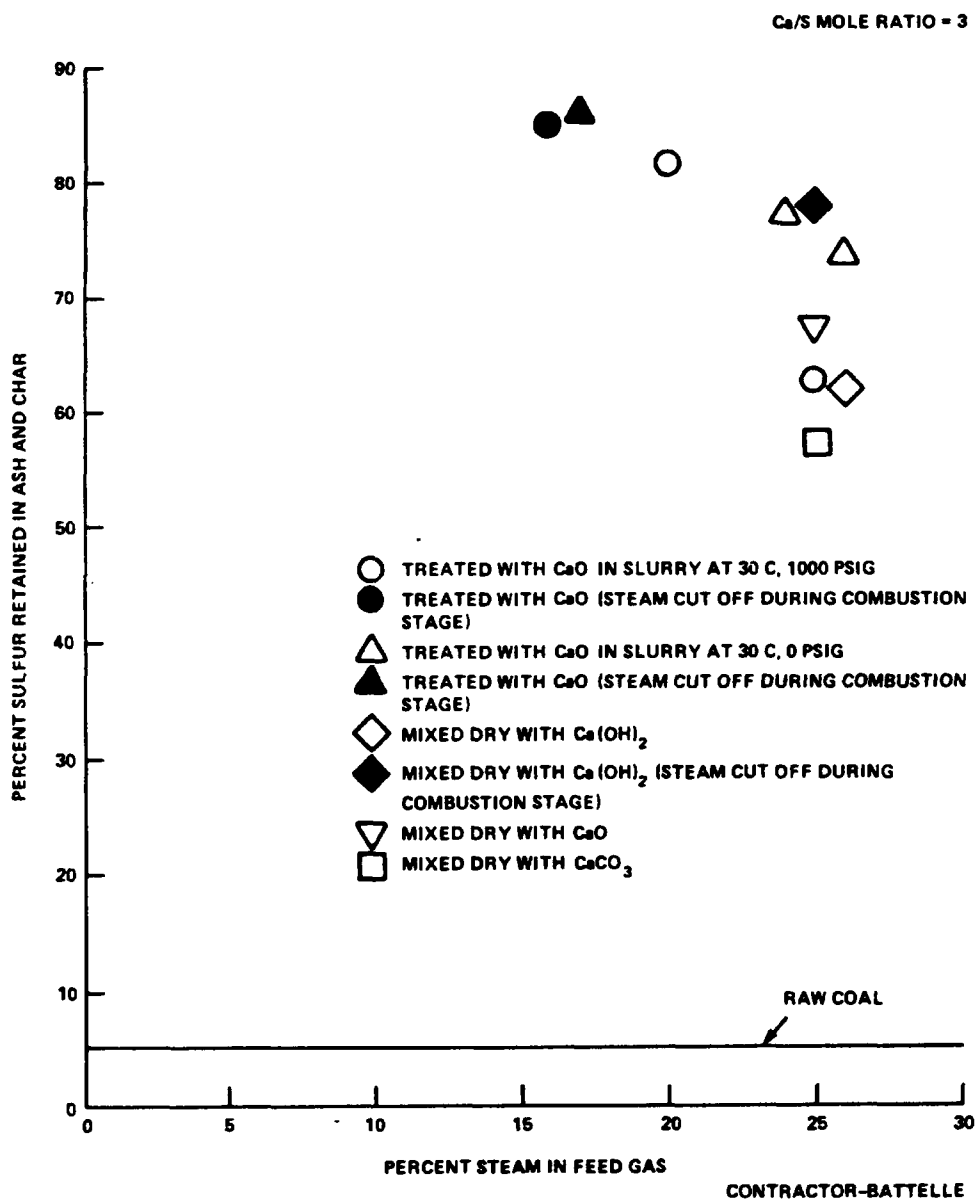
Figure 18. Laboratory screening tests-feasibility of in-gasifier sulfur scavenging (steam air gasification of treated coal in fluidized bed).
