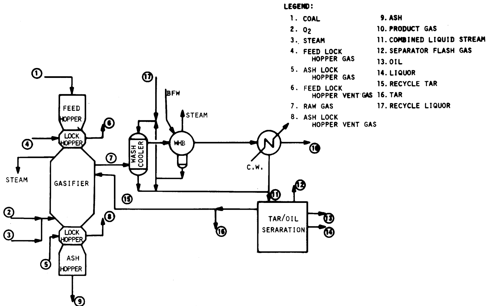
Figure A-1. Lurgi gasifier (Based on Westfield Lurgi Installation).
