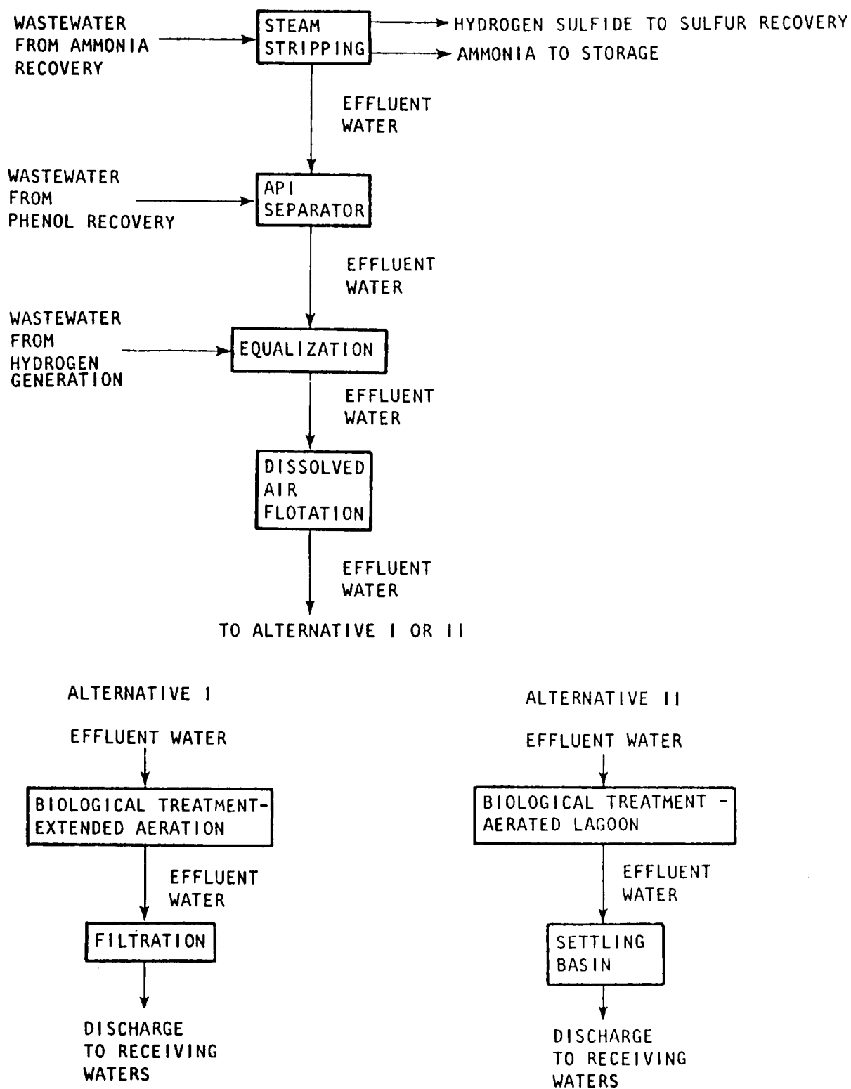
Figure 4. Two wastewater treatment alternatives applicable to SRC systems.
