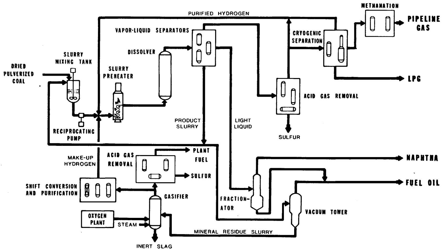
Figure 2. SRC-II process.
