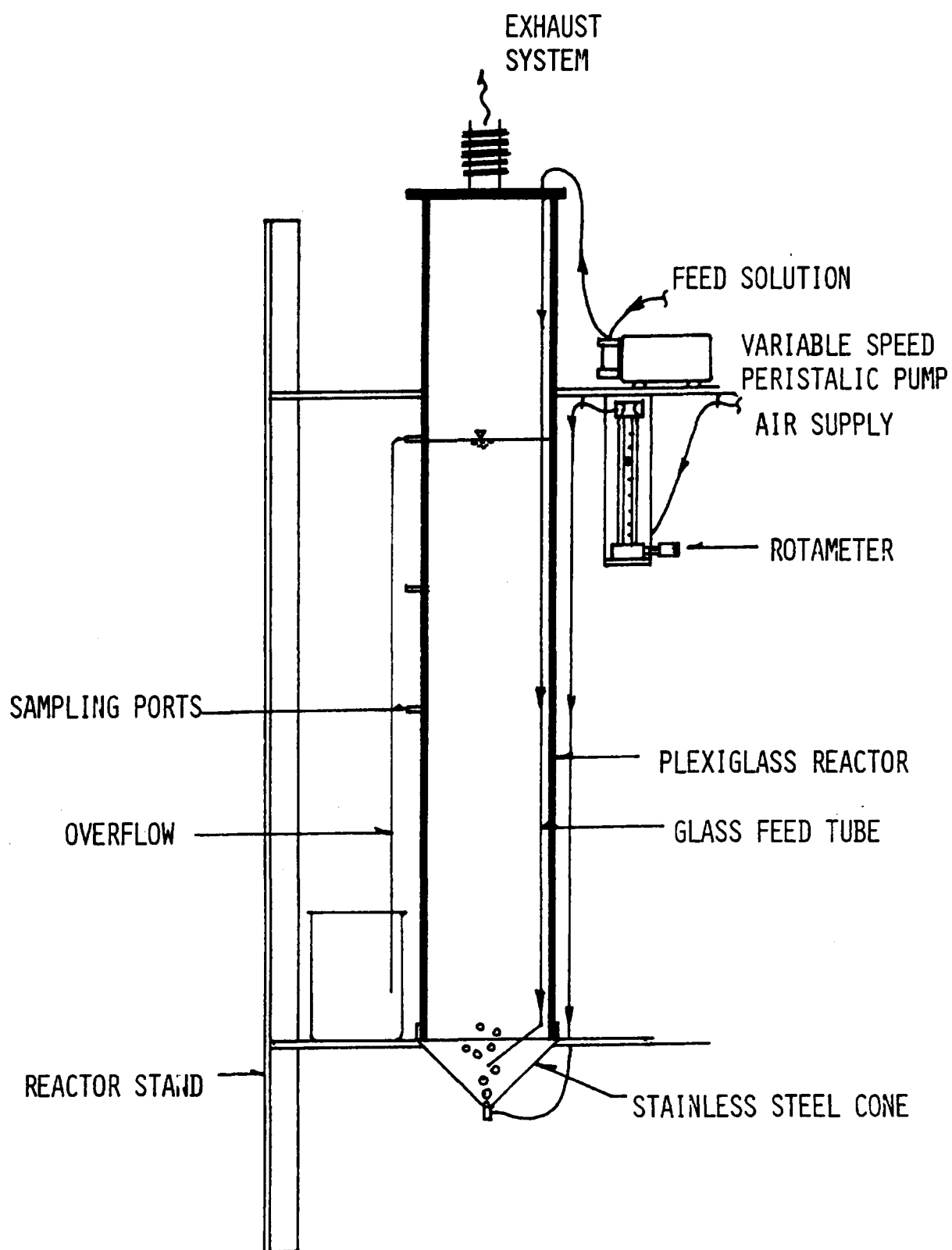
Figure 1. Schematic of experimental biological reactors.
