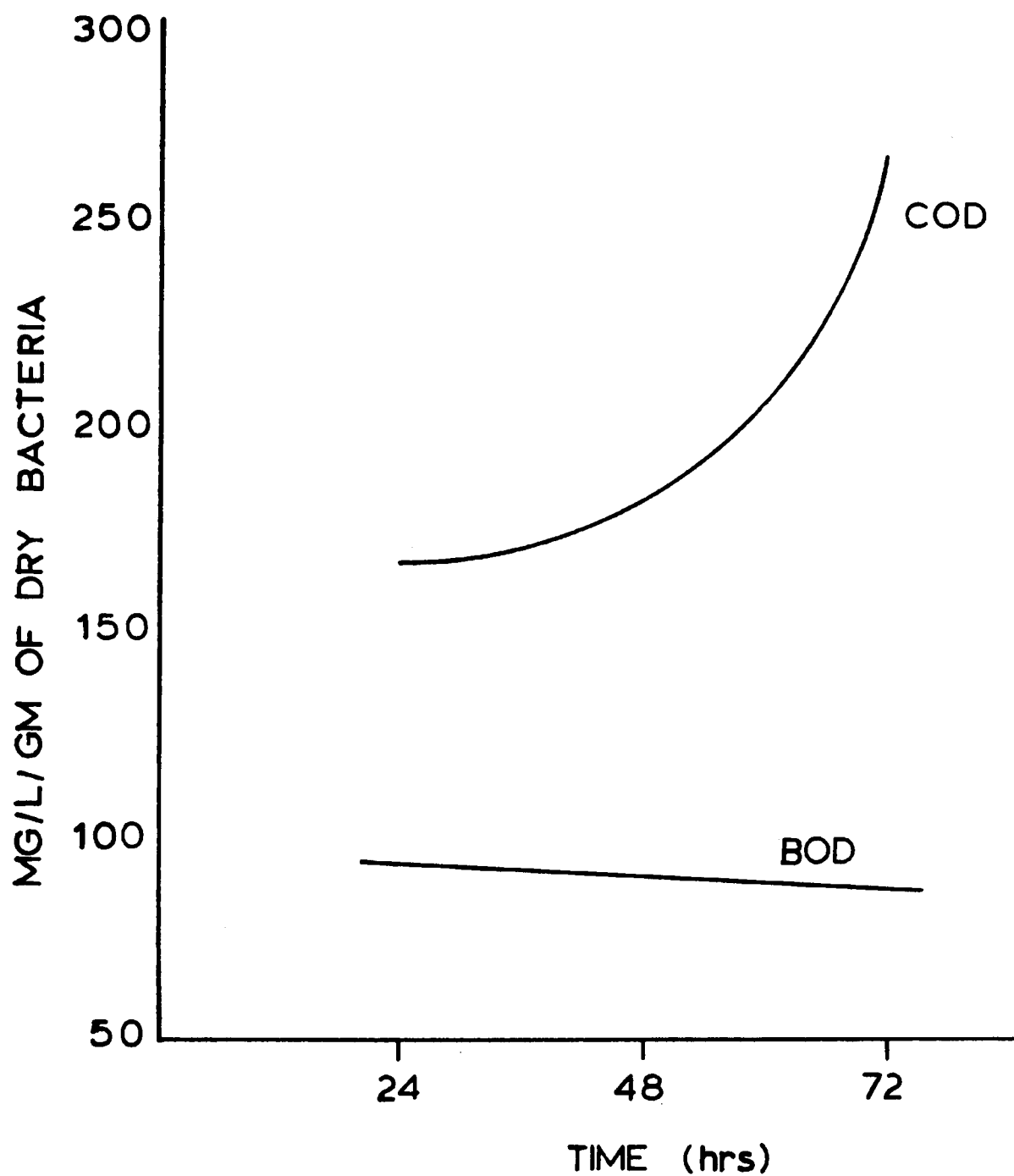
Figure 3. COD and BOD addition by dry bacteria.
