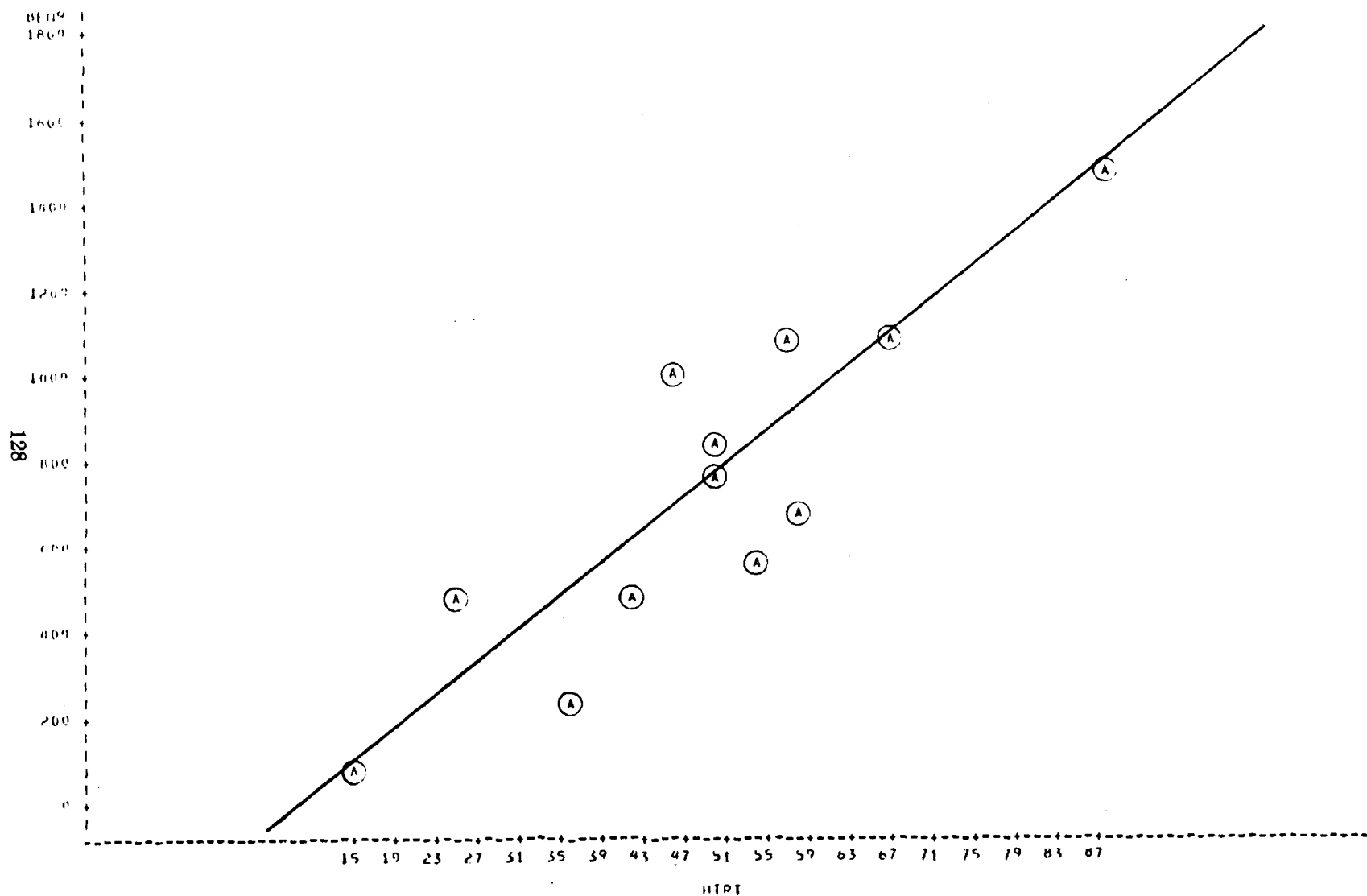
Figure 5. Devolatilization heating rate ( ^{\circ}\text{C}/\text{min} ) vs. benzene concentration in gas stream ( \mu\text{g}/\text{m}^3/[\text{MATE}] ).
