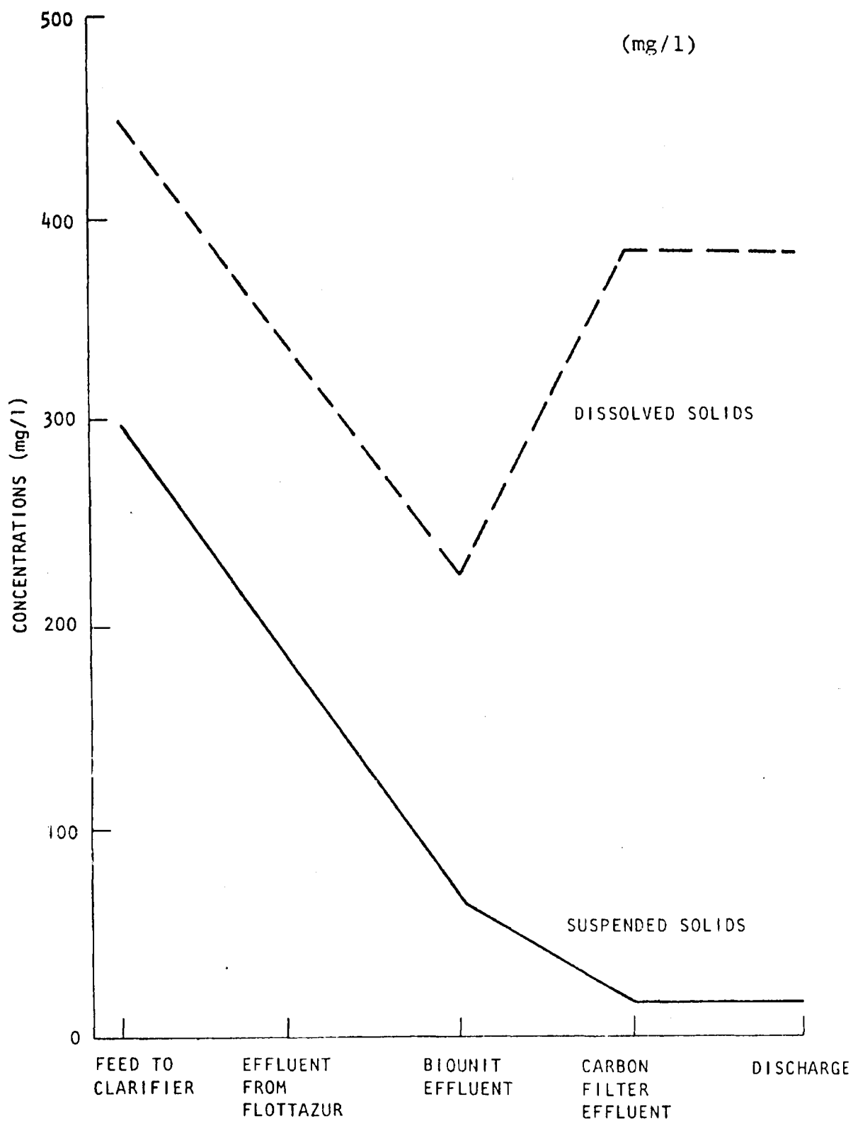
Figure 7. Distribution of dissolved and suspended solids in the wastewater treatment system.
