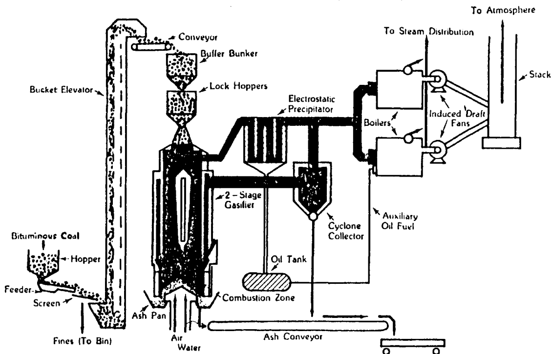
Figure 1. Schematic diagram of University of Minnesota-Duluth heating plant.
