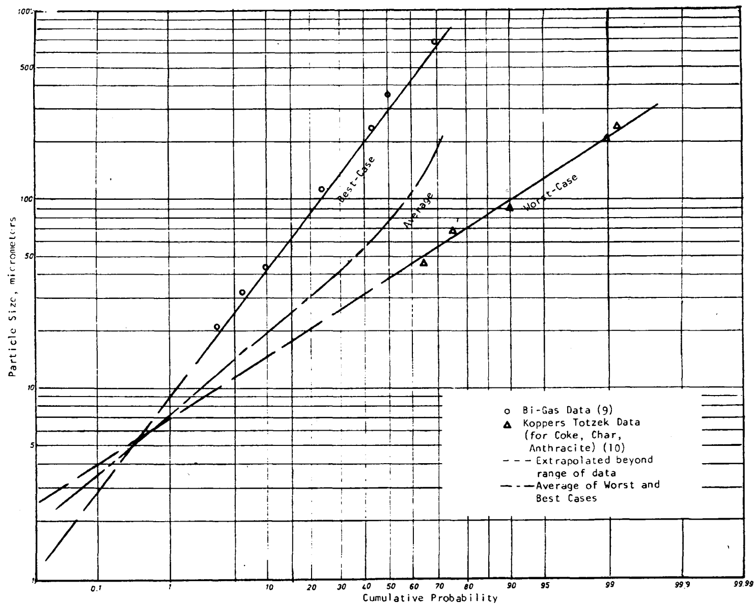
Figure 3. Particulate size distribution for entrained-bed gasifiers.
