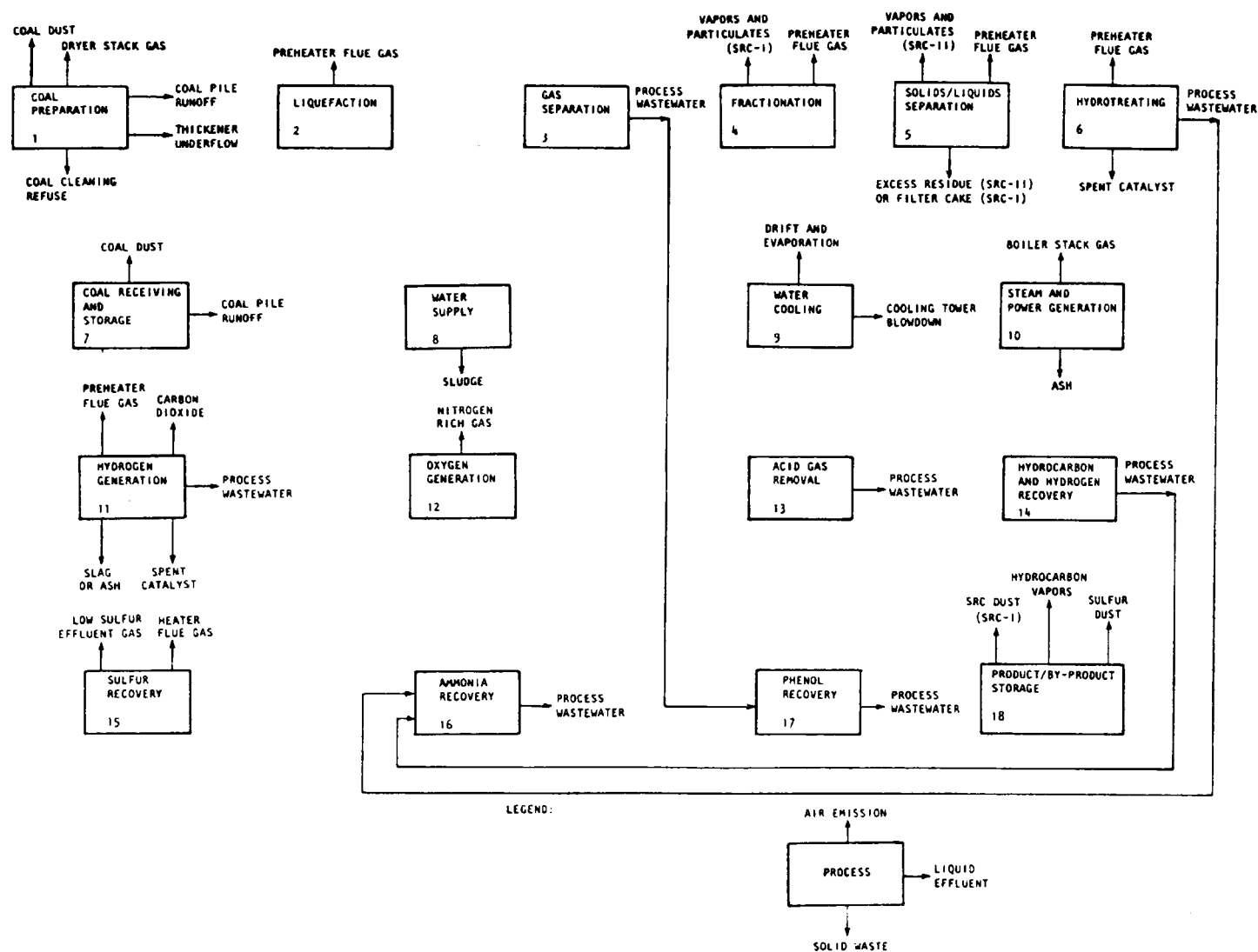
Figure 3. Source of waste discharges in SRC systems.
