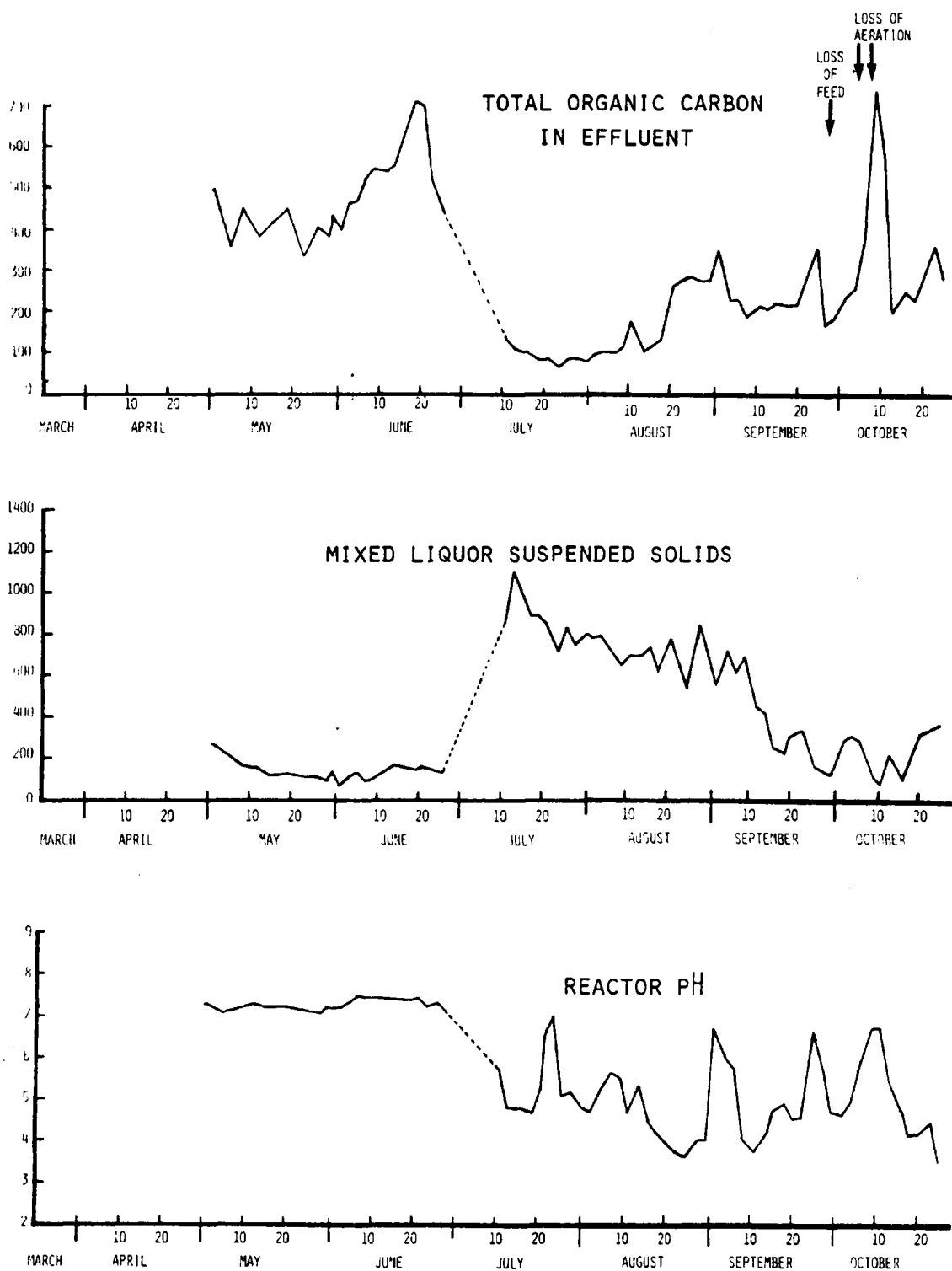
Figure 2. Performance characteristics of Reactor 1 with 5-day residence time.
