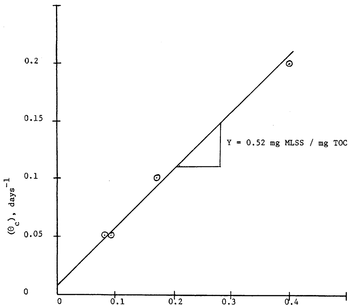
Figure 9. Effect of solids residence time on TOC loading.
