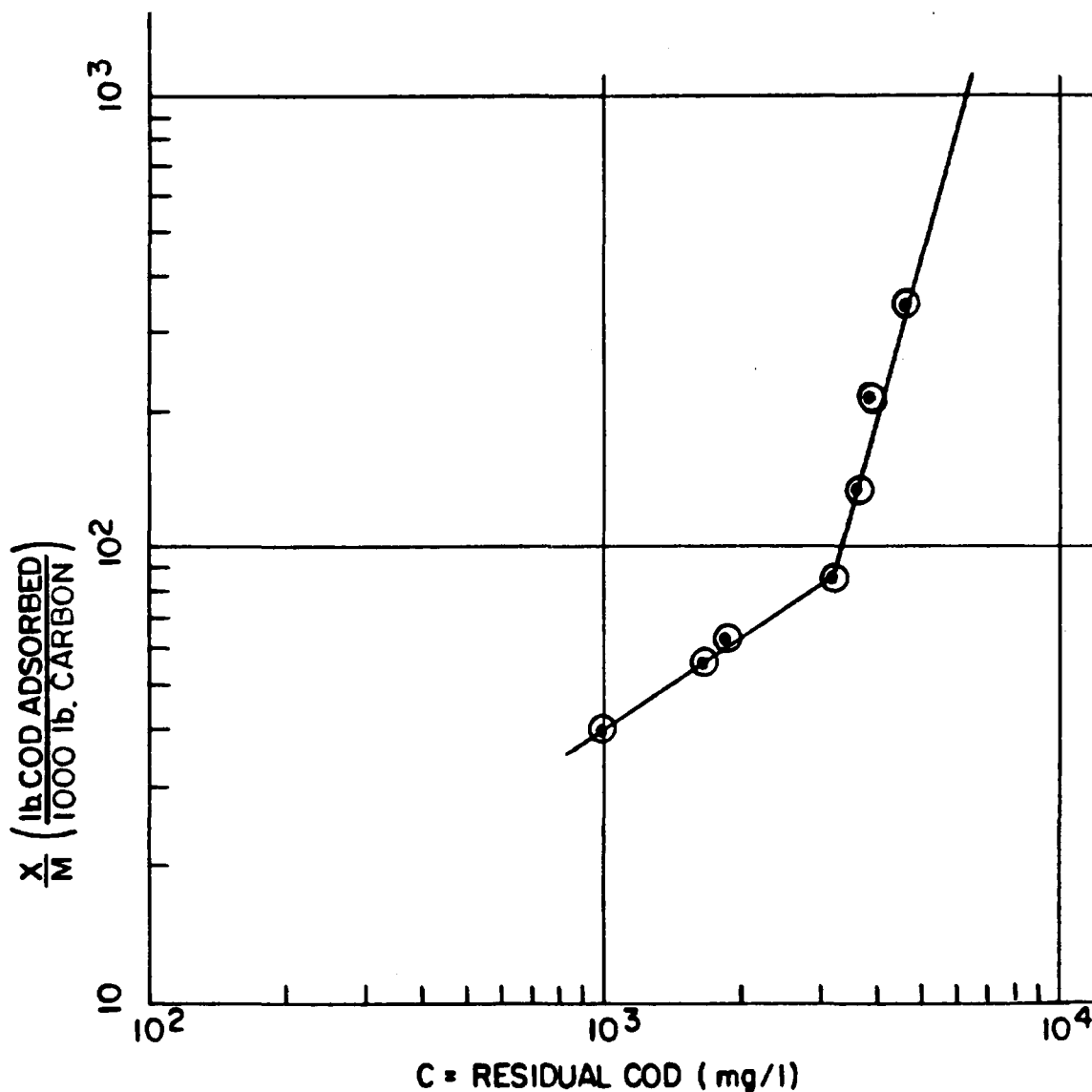
Figure 2. Carbon adsorption isotherm.
