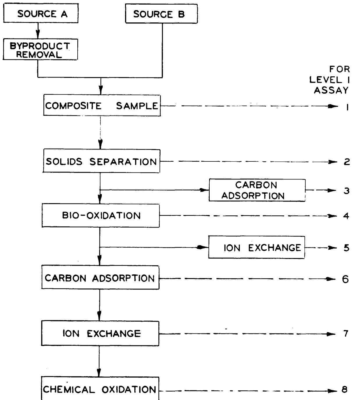
Figure 1. Preliminary wastewater test sequence.
