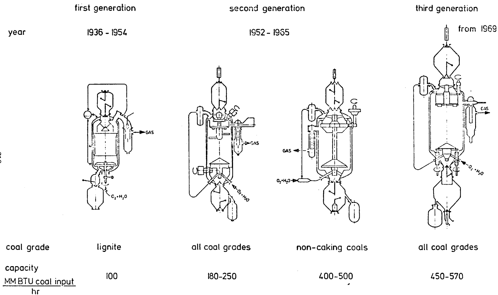
Figure A-2. Stages of Lurgi gasifier development.
