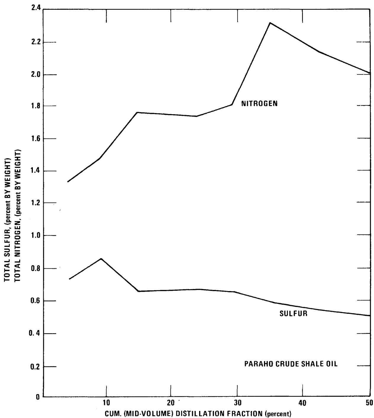
Figure 1. Total weight of nitrogen and sulfur as a function of the cumulative midvolume distillation fraction. 12
