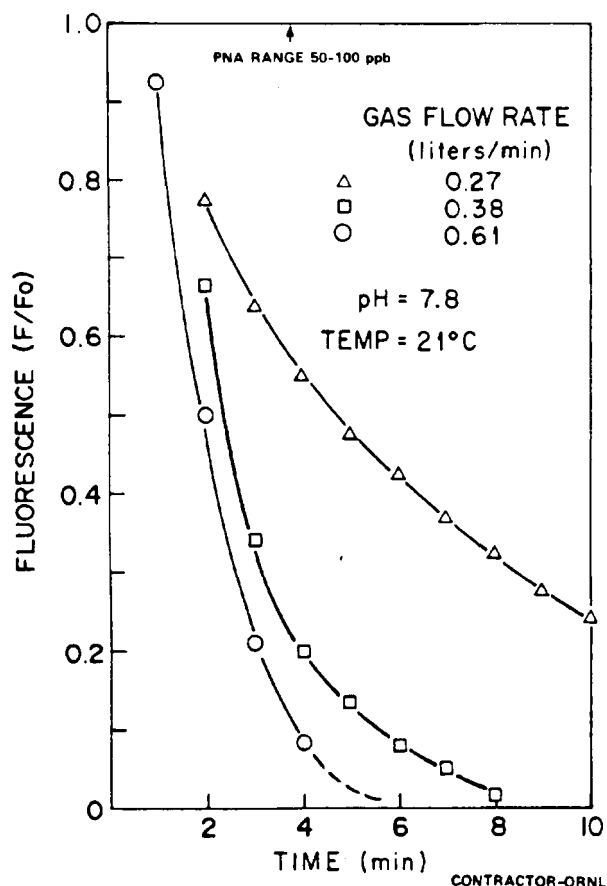
Figure 15. Screening tests—ozonation of hydrocarbonization wastewater (effect of gas flow rate).
