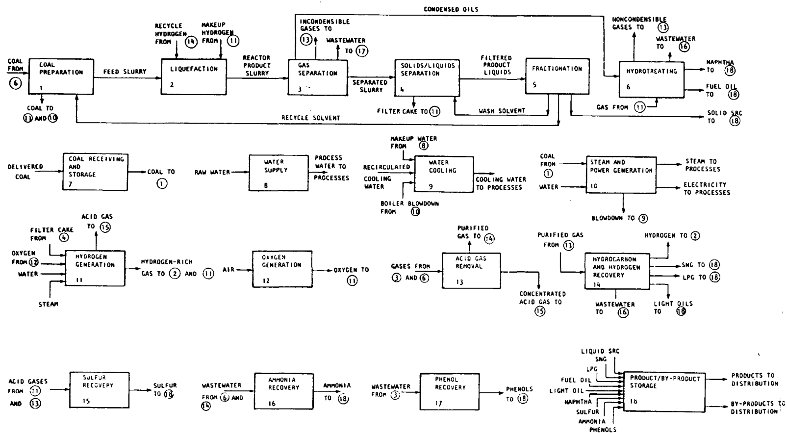
Figure 1. Flow diagram of SRC-I system.
