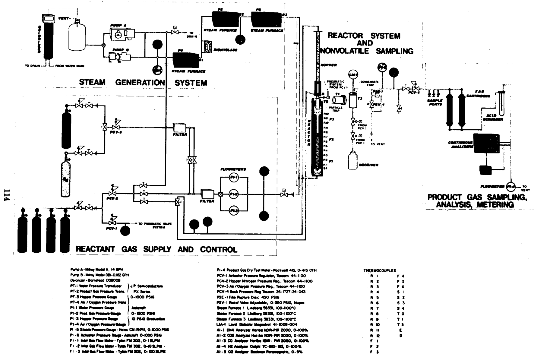
Figure 1. Reactor and sampling systems.
