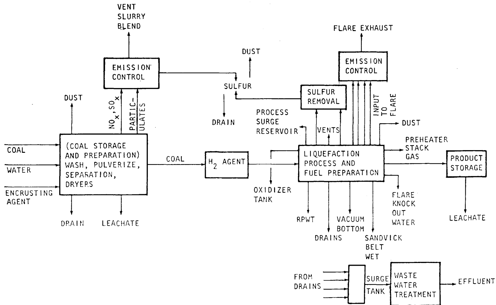
Figure 4. Pollutant streams at SRC system, Fort Lewis, Washington.
