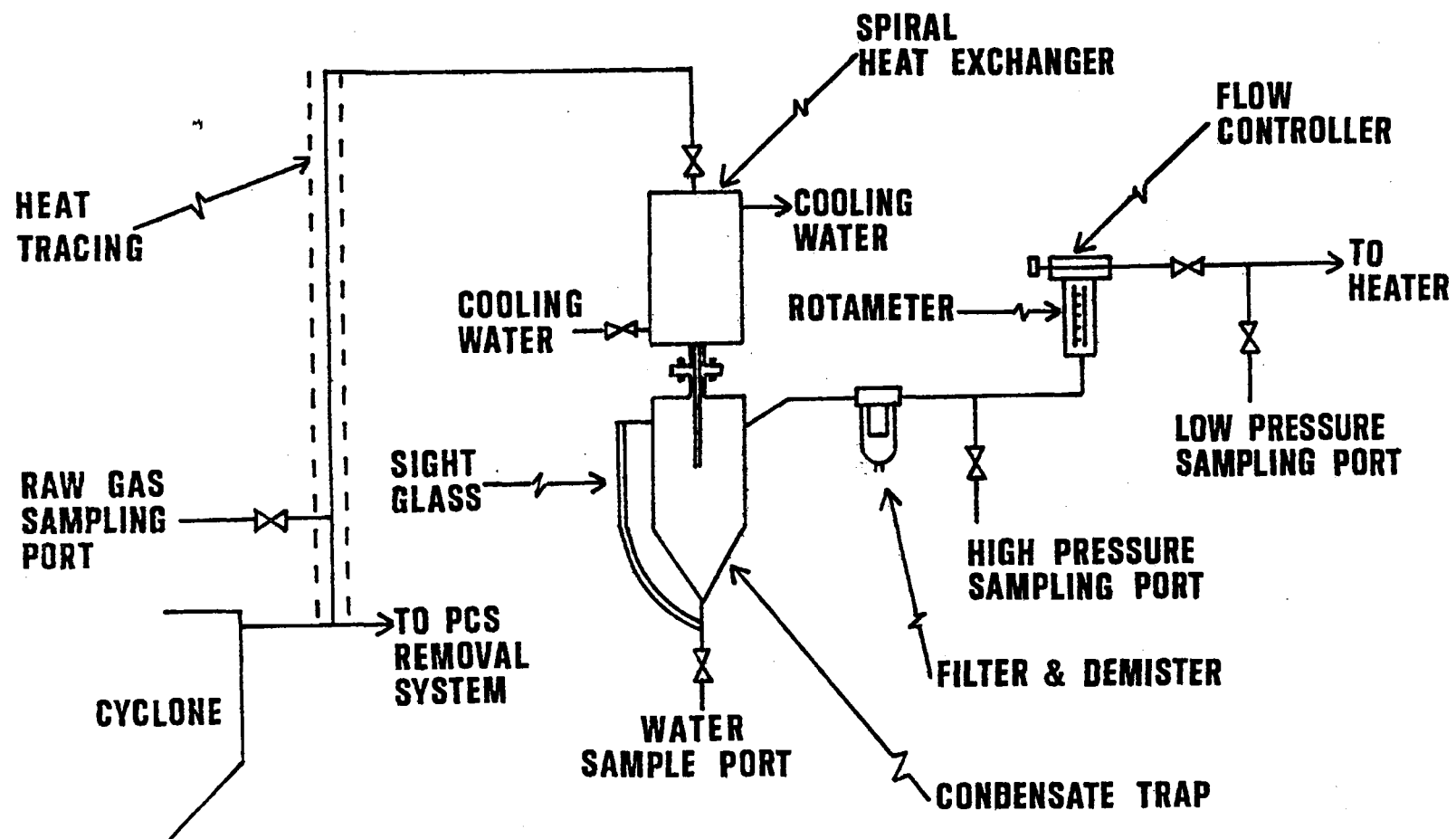
Figure 8. Sample system located at cyclone exit.
