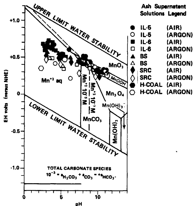
Figure 2. Stability relations of manganese oxides in water at 25° C.
