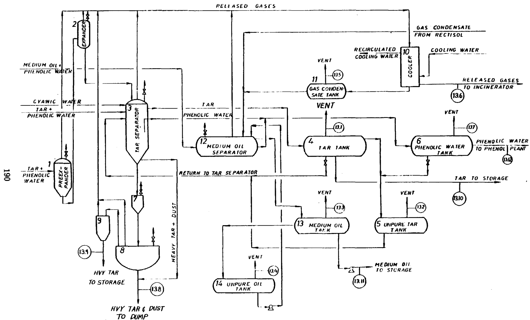
Figure 5. Process flow diagram showing sampling points in Kosovo plant tar separation section.
