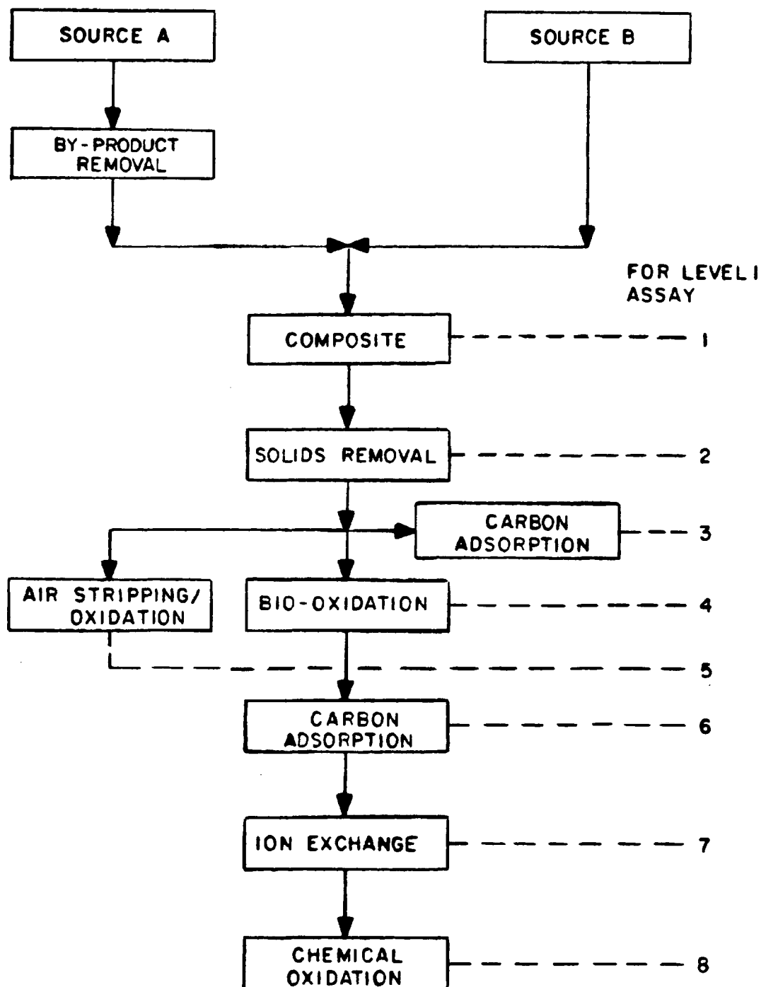
Figure 6. Final wastewater test sequence.
