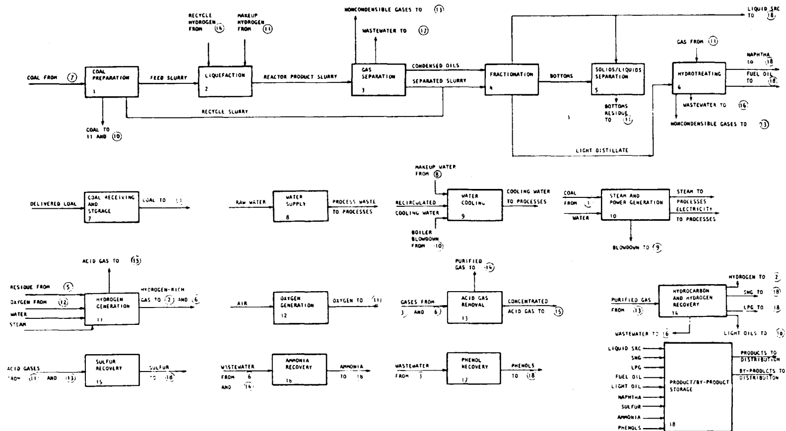
Figure 2. Flow diagram of SRC-II system.
