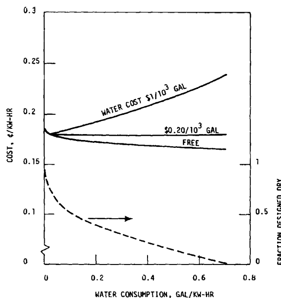
Figure 3. Cost of steam turbine condenser cooling in Farmington, New Mexico.
