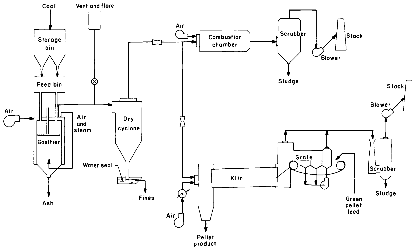
Figure 1. Process flow diagram of Bureau of Mines Gasification and Pelletizing Pilot-Plant, Twin Cities Metallurgy Research Center.
