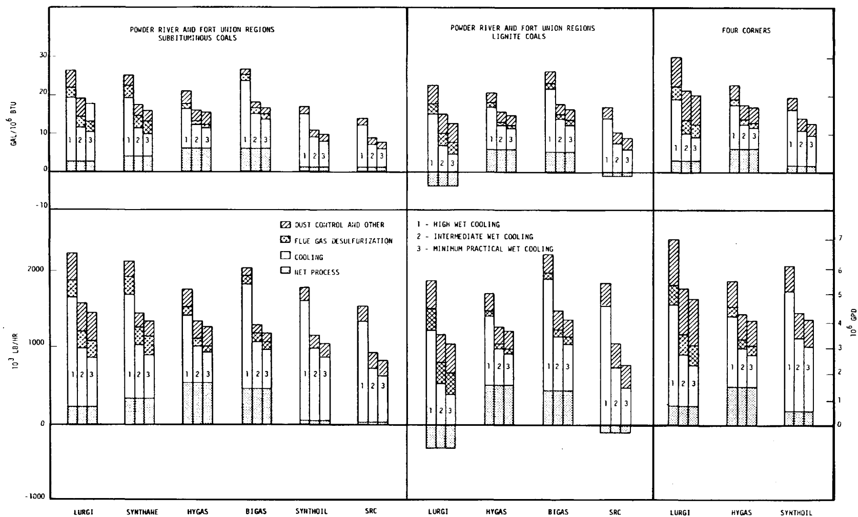
Figure 7. Summary of average net water consumed for coal conversion plants located in the Western States.
