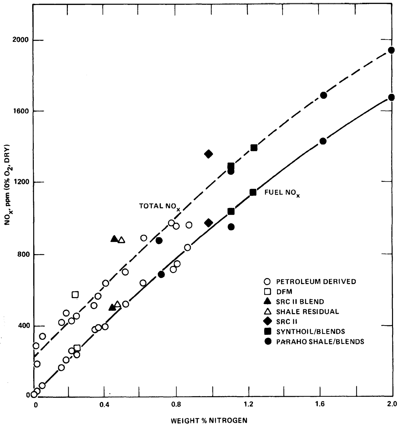
Figure 2. The effect of fuel nitrogen content on total and fuel NO x (5 percent excess oxygen). 16
