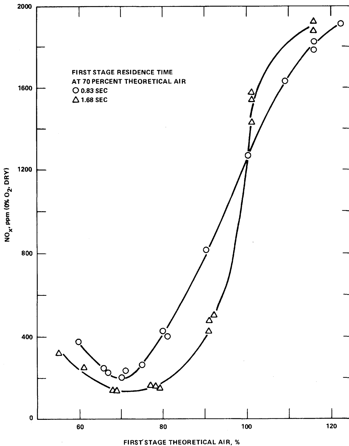
Figure 3. The influence of staged operation in the tunnel furnace on \text{NO}_x emissions from the Paraho shale oil (5 percent excess oxygen). 16
