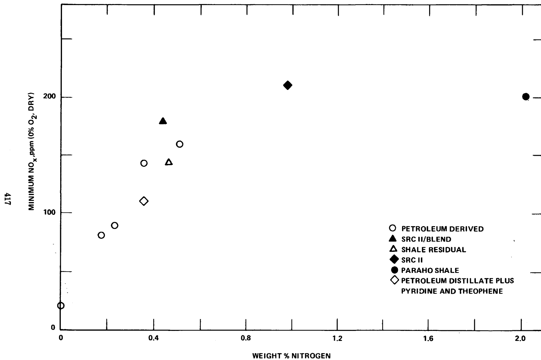
Figure 6. Minimum NO x levels obtained in the tunnel furnace as a function of fuel-bound nitrogen content. 16
