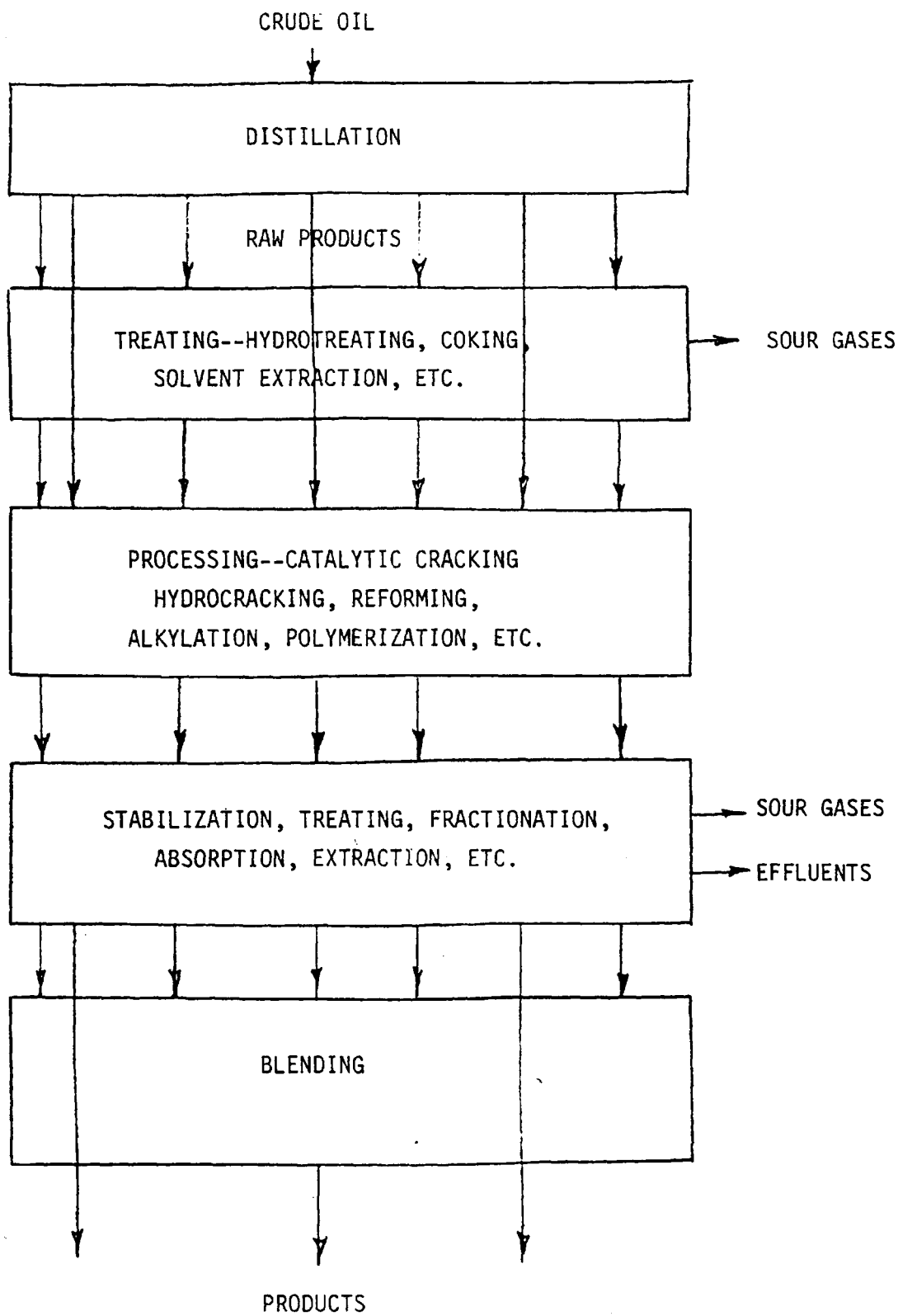
Figure 2. Petroleum refinery.
