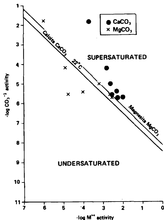
Figure 4. Calcium and magnesium carbonate equilibria of alkaline ( \text{pH} > 7.6 ) leachates from five coal conversion solid wastes in contact with air.
