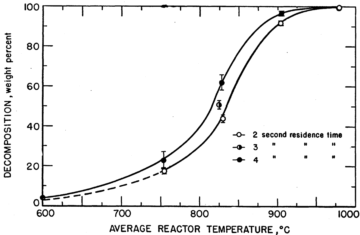
Figure 6. Measured phenol decomposition as a function of average temperature for 2, 3, and 4 s nominal residence times.
