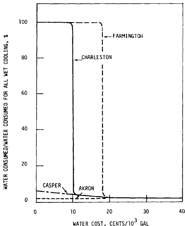
Figure 4. The effect of water cost on water consumed for cooling turbine condensers.
