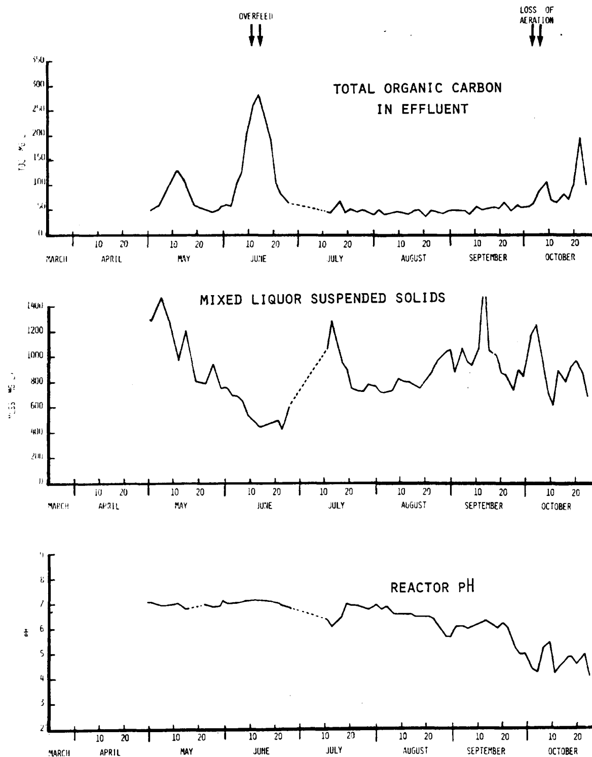
Figure 5. Performance characteristics of Reactor 4 with 20-day residence time.
