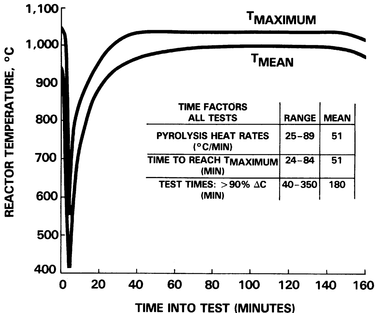
Figure 6. Reactor heating.
