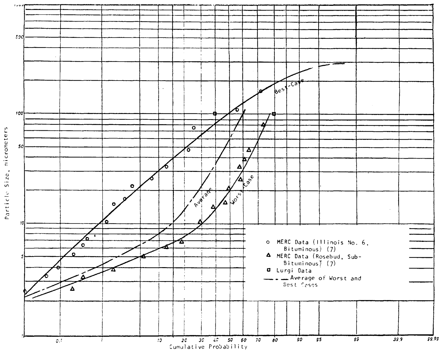
Figure 1. Particle size distribution for fixed-bed gasifiers.
