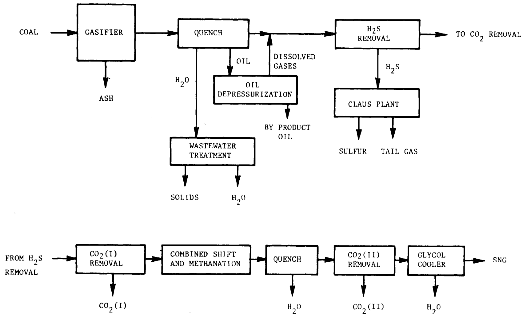
Figure 4. Typical gas producing configuration for producing SNG.
