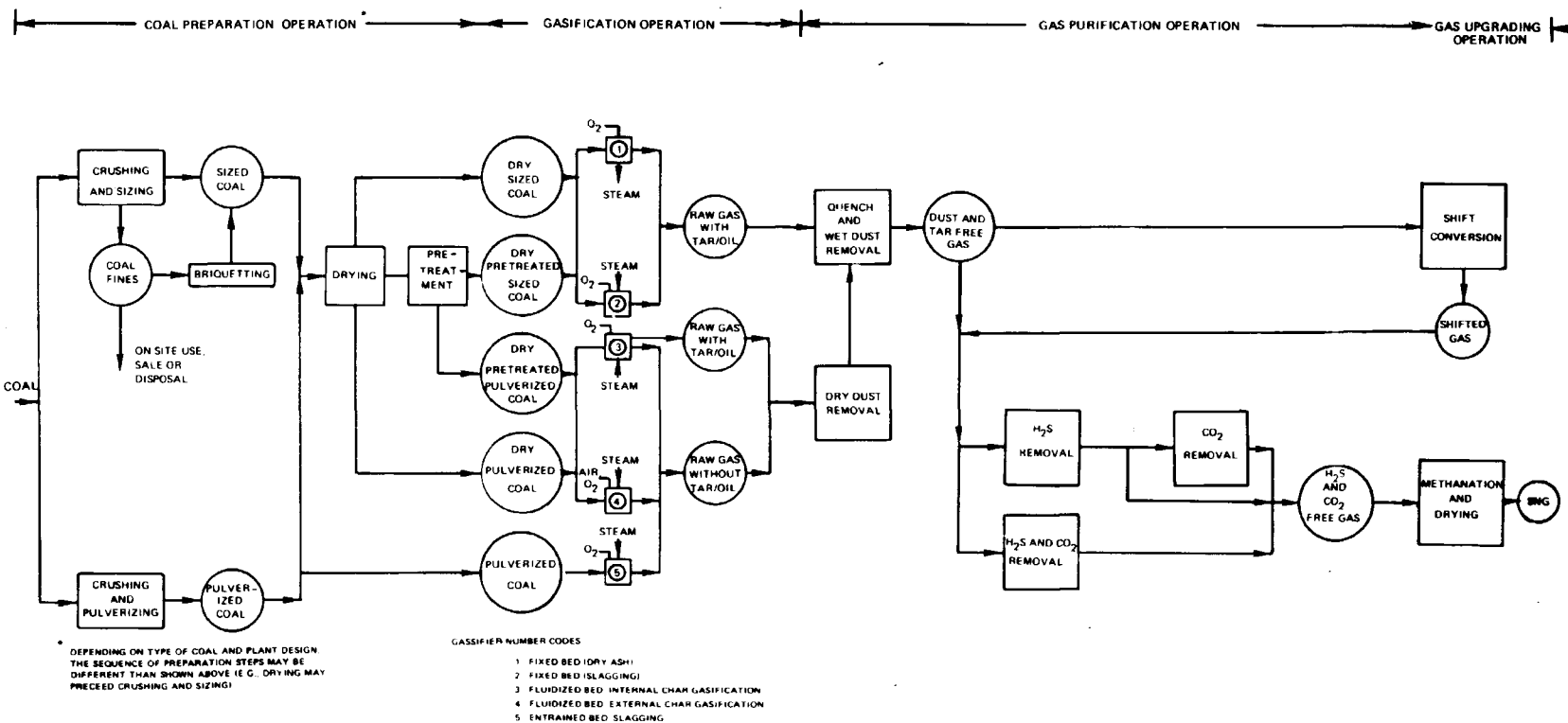
Figure 1. High-Btu gasification operations and process modules.
