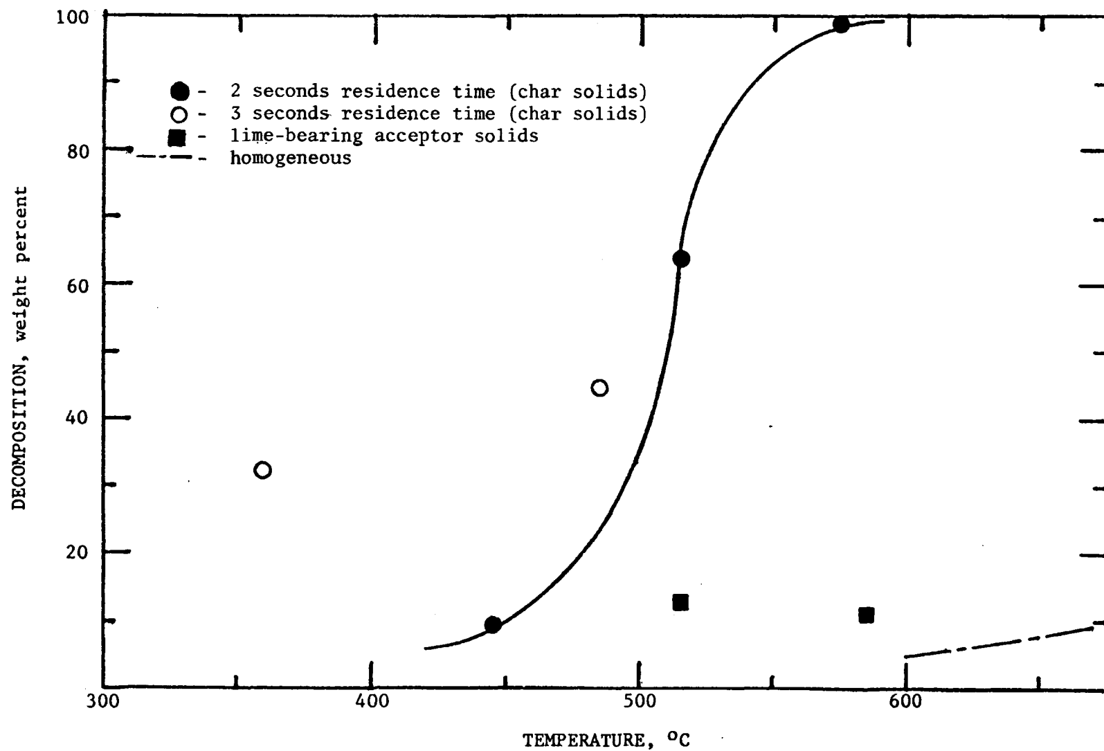
Figure 8. Measured phenol decomposition in the presence of lignite char and limestone acceptor solids as a function of temperature.
