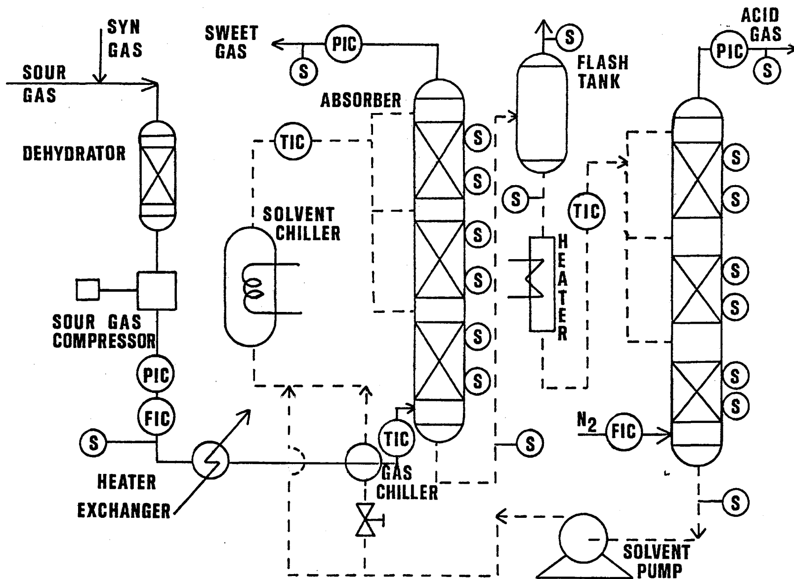
Figure 3. Acid-gas removal system.
