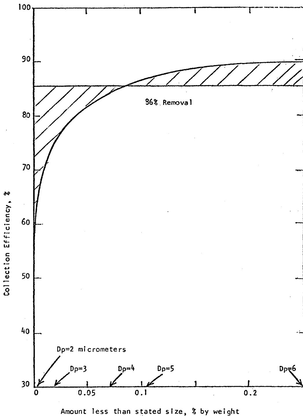
Figure 5. Graphical procedure for estimating overall collection efficiency for particulates up to 6 \mu\text{m} in diameter.
