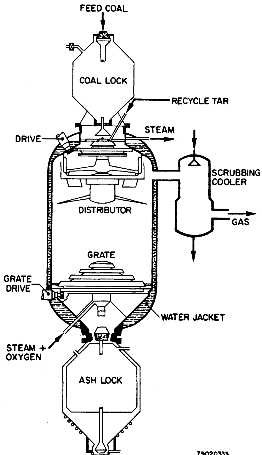
Figure 2. Lurgi pressure gasifier.
