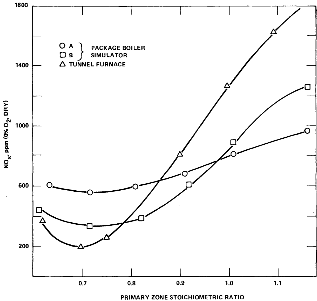
Figure 5. NO x emissions staged—Paraho shale (5 percent overall excess oxygen). 16
