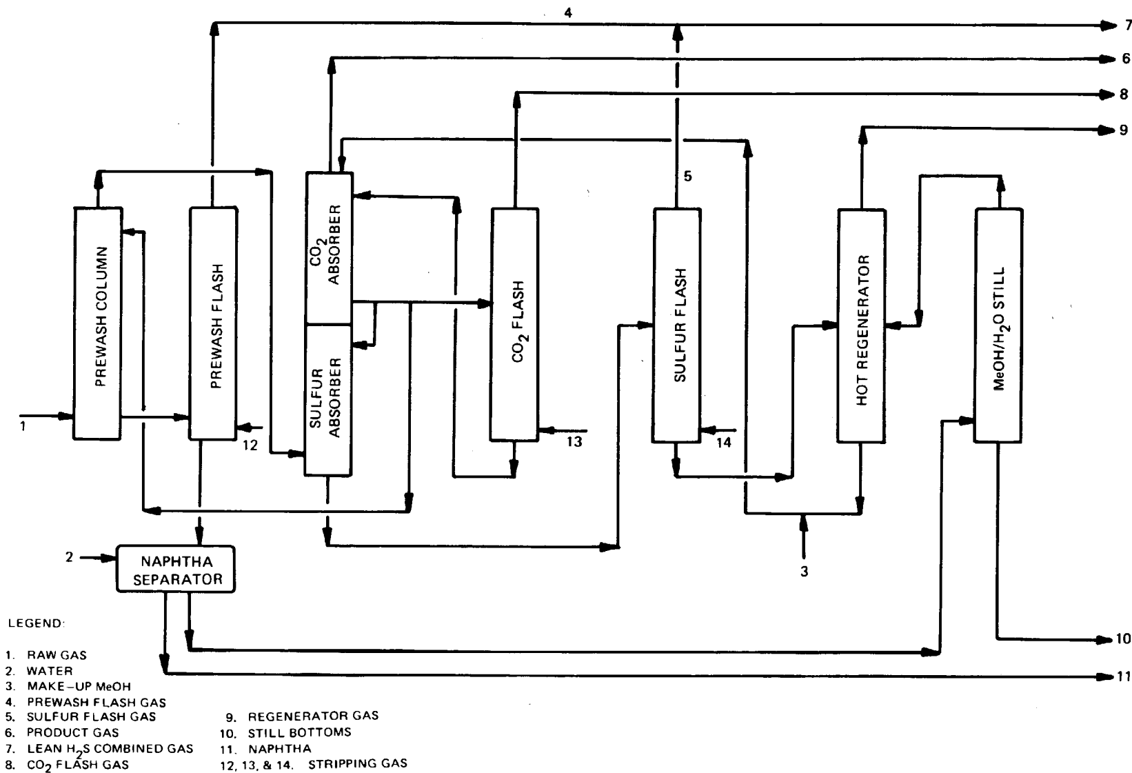
Figure B-2. Rectisol type B 3 (removal of CO_2 and H_2S with separate recovery).
