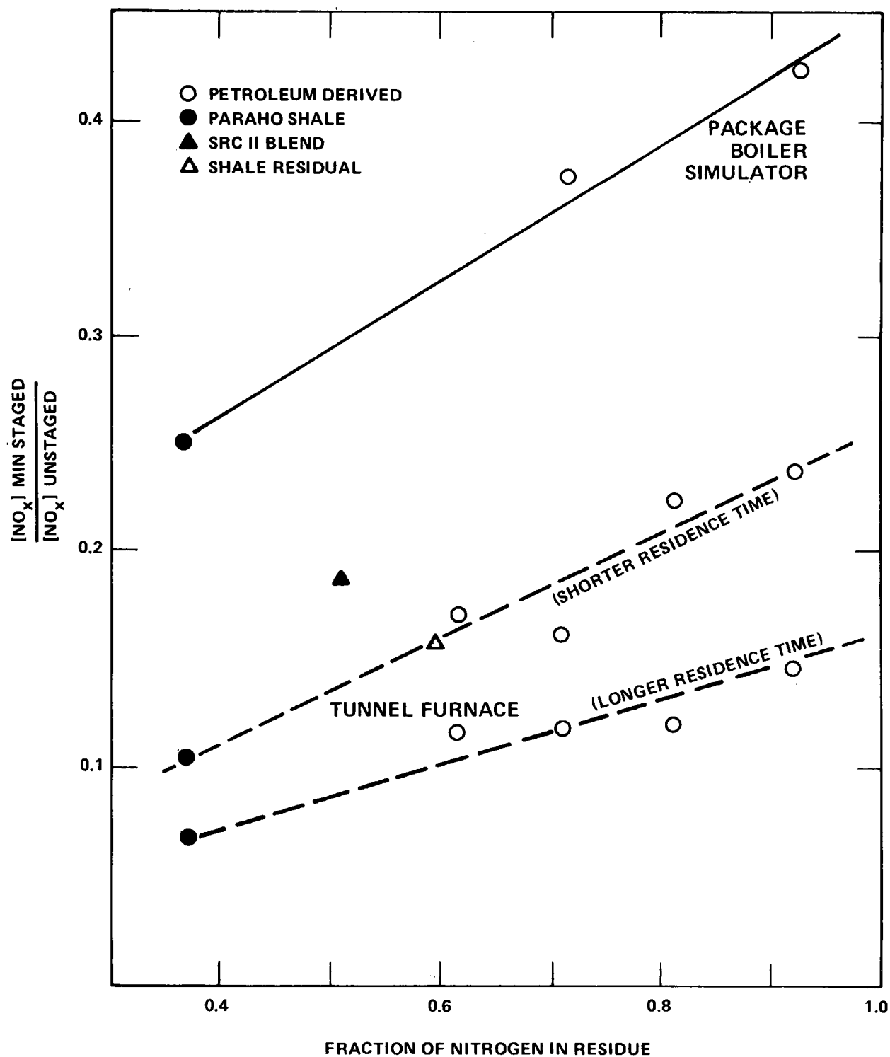
Figure 8. The influence of volatile fuel nitrogen on staging effectiveness (reference 16).
