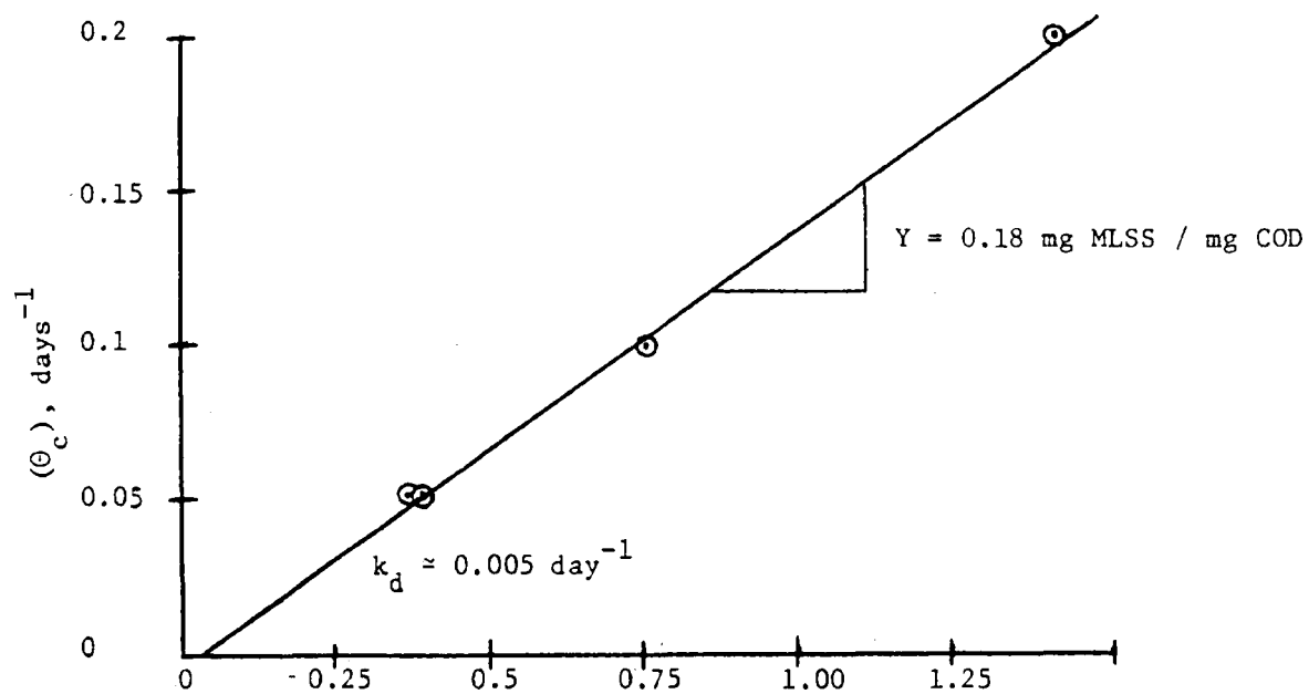
Figure 8. Effect of solids residence time on COD loading.
