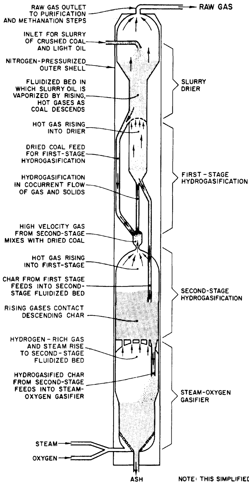
Figure 3. Hygas gasifier with steam/O 2 gasification.
