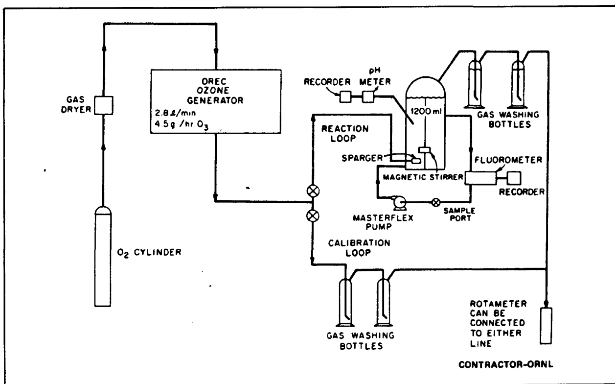
Figure 14. Schematic drawing of batch ozonation system.
