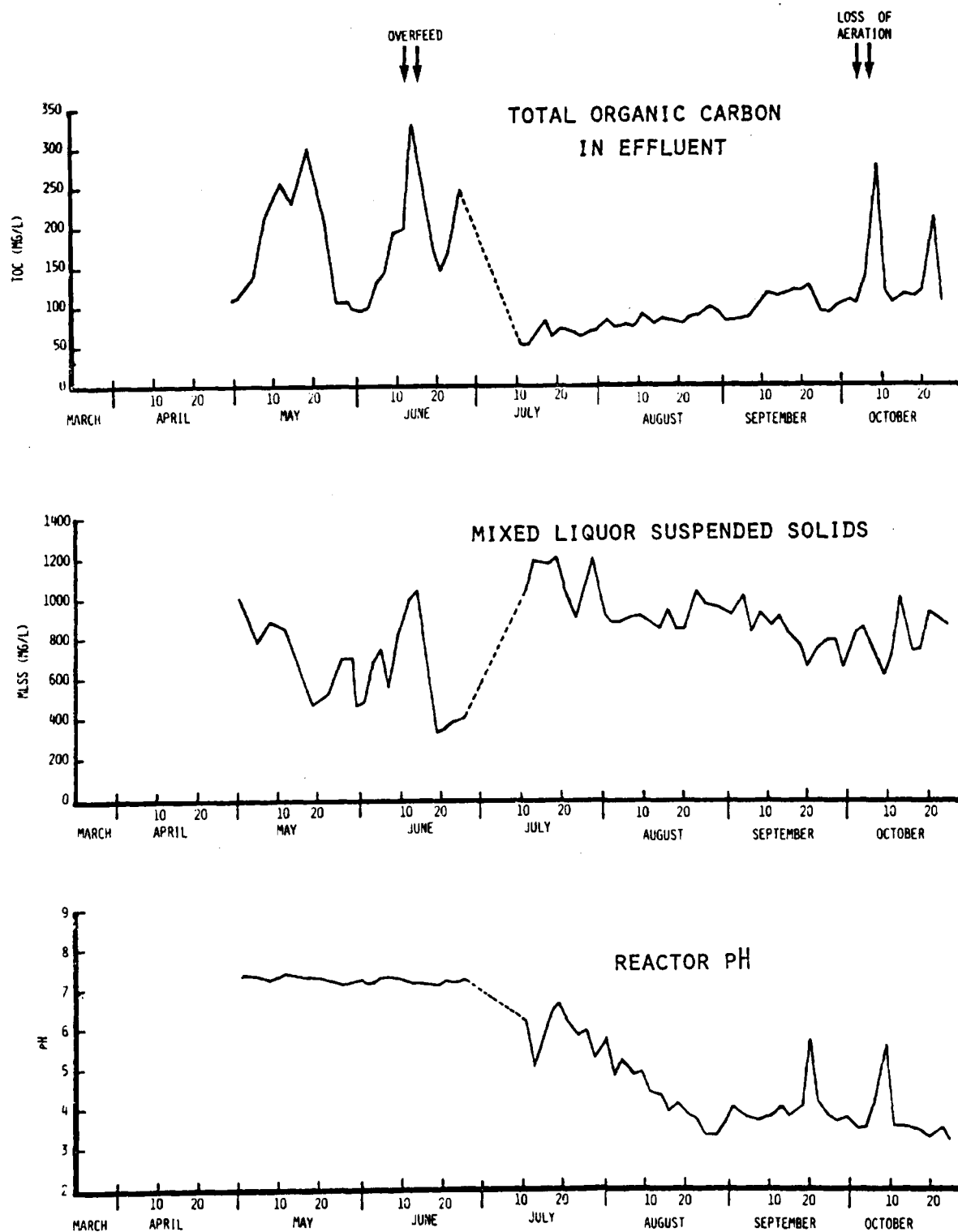
Figure 3. Performance characteristics of Reactor 2 with 10-day residence time.
