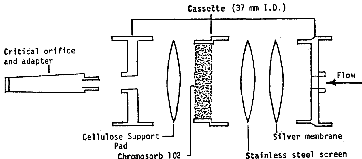
Figure 1. High-volume sampling device for PNA.
