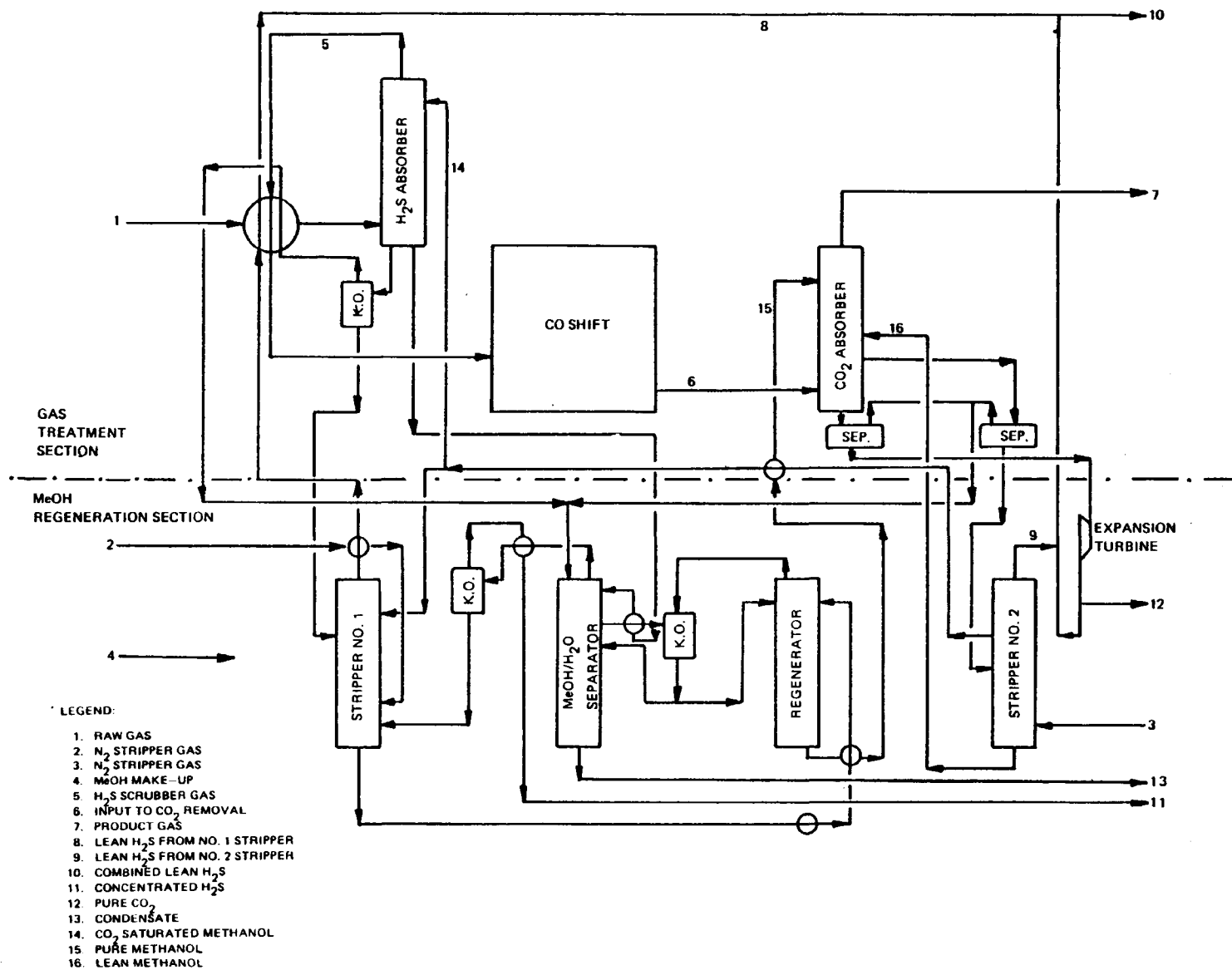
Figure B-4. Rectisol—dual-absorption flow diagram (as installed at Modderfontein, South Africa).
