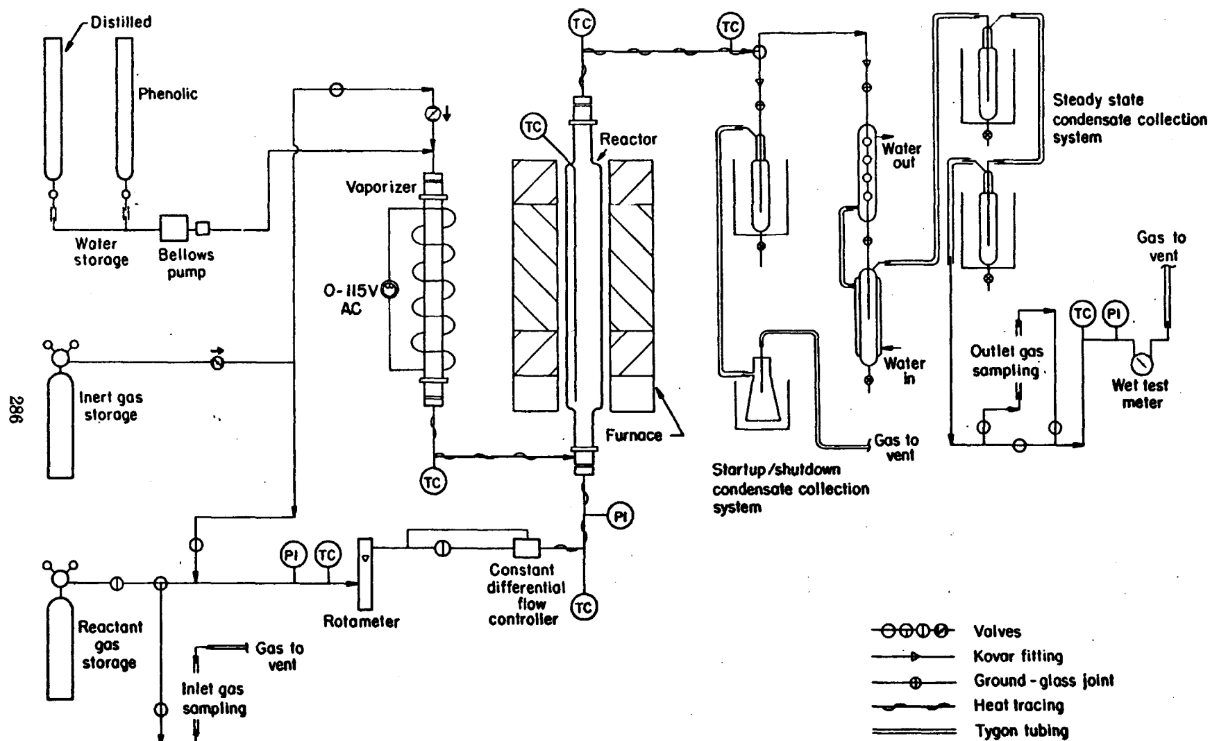
Figure 3. Thermal decomposition reactor—basic bench-scale equipment train.
