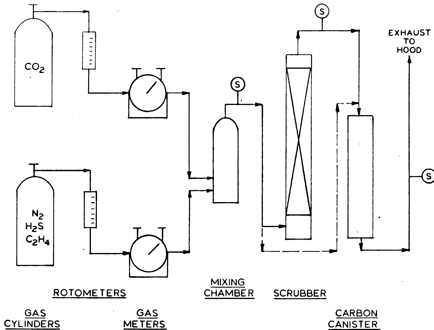
Figure 10. Pilot scrubber and carbon adsorber test apparatus.
