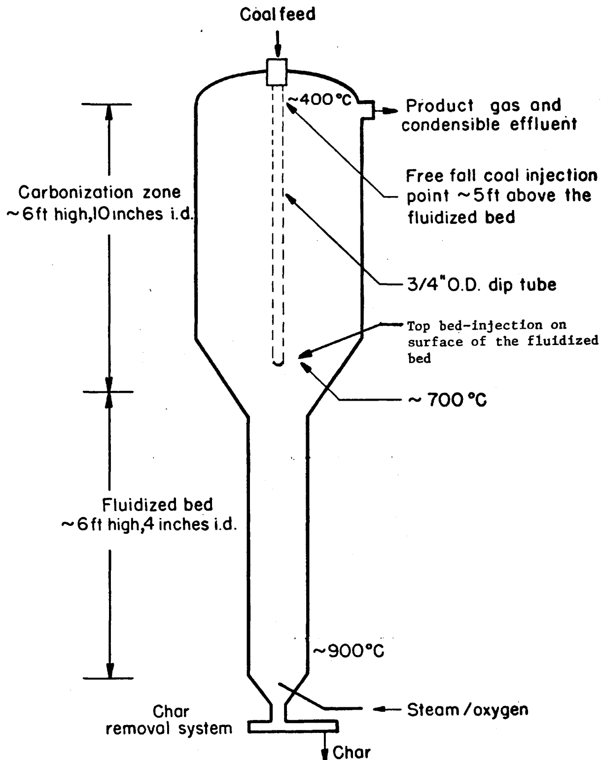
Figure 4. Basic configuration and coal feed locations of the Synthane PDU gasifier.
