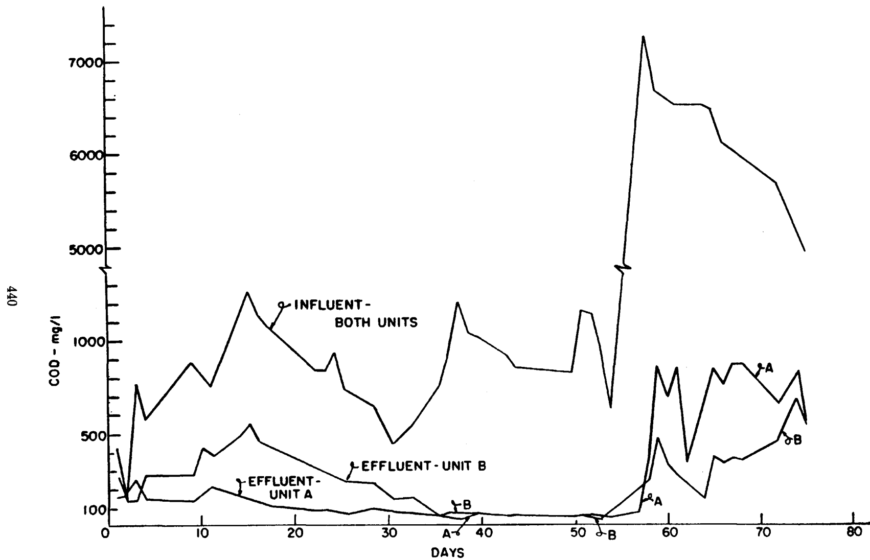
Figure 4. Continuous biological reactor results.
