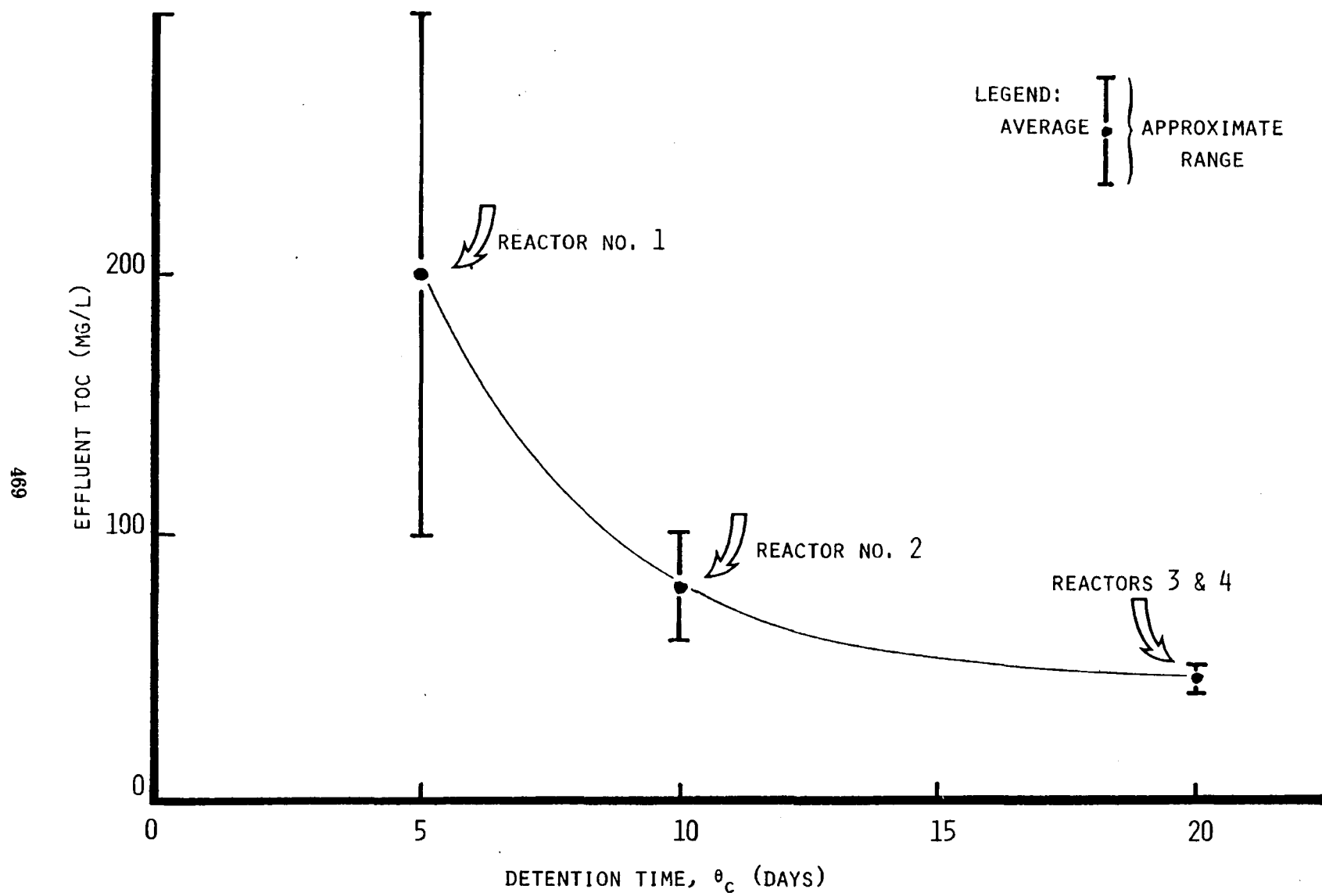
Figure 6. Effect of residence time on reactor performance and stability.
