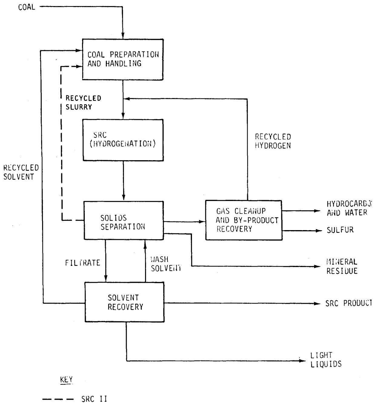
Figure 1. Solvent refined coal system. 6
