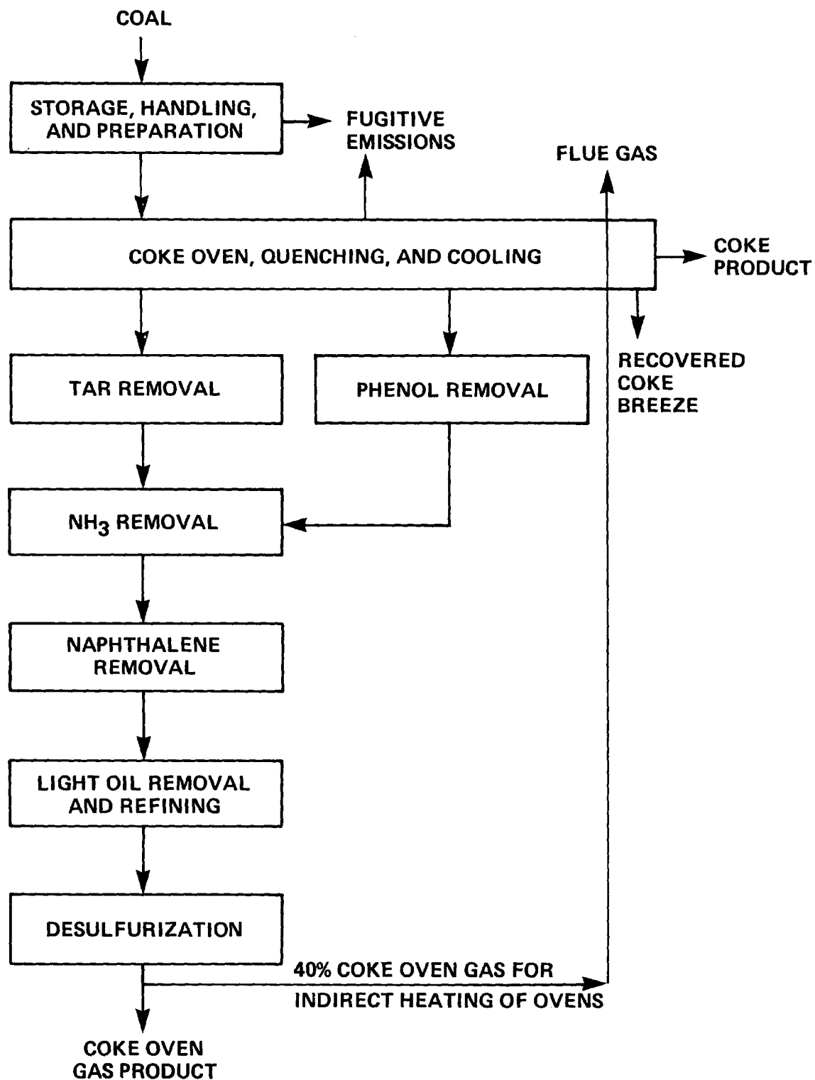
Figure 3. Byproduct coke oven process.
