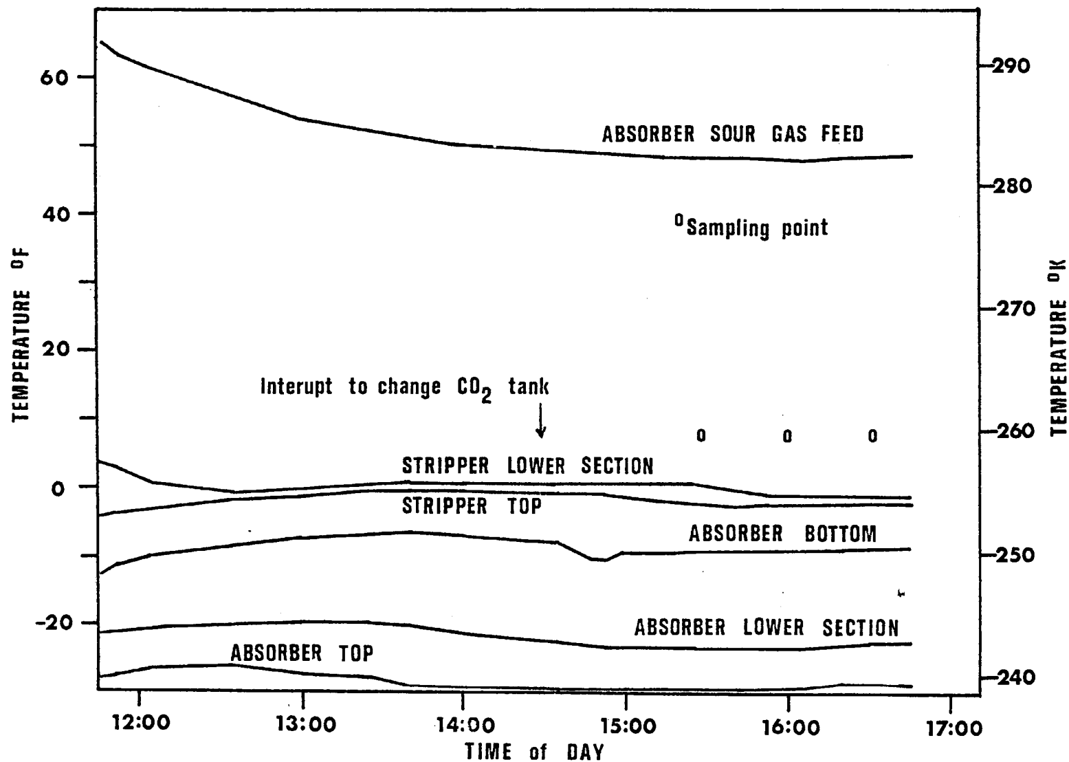
Figure 10. Run AM-4 steady-state temperature data.
