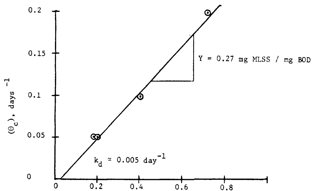
Figure 7. Effect of solids residence time on BOD loading.
