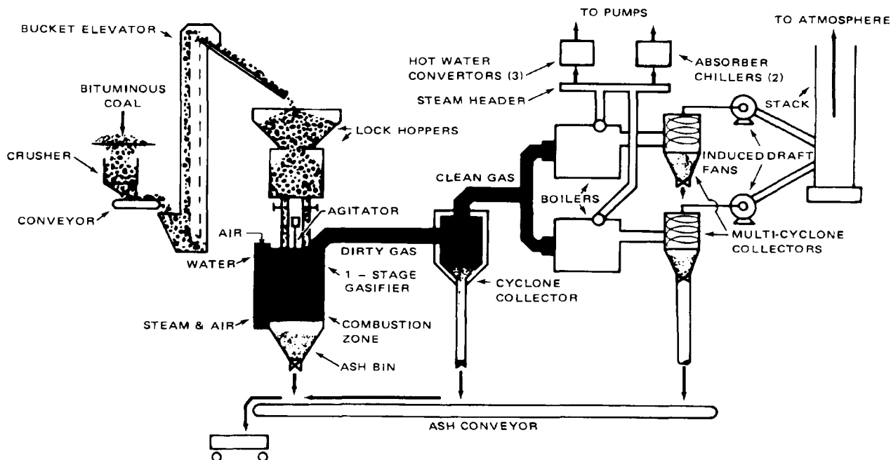
Figure 3. Schematic diagram of Pike County coal gasification facility.
