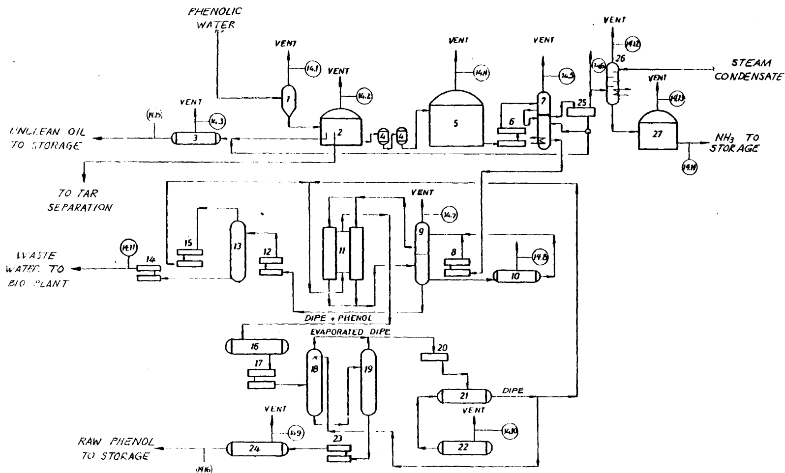
Figure 7. Process flow diagram showing sampling points in Kosovo plant phenosolvan section.
