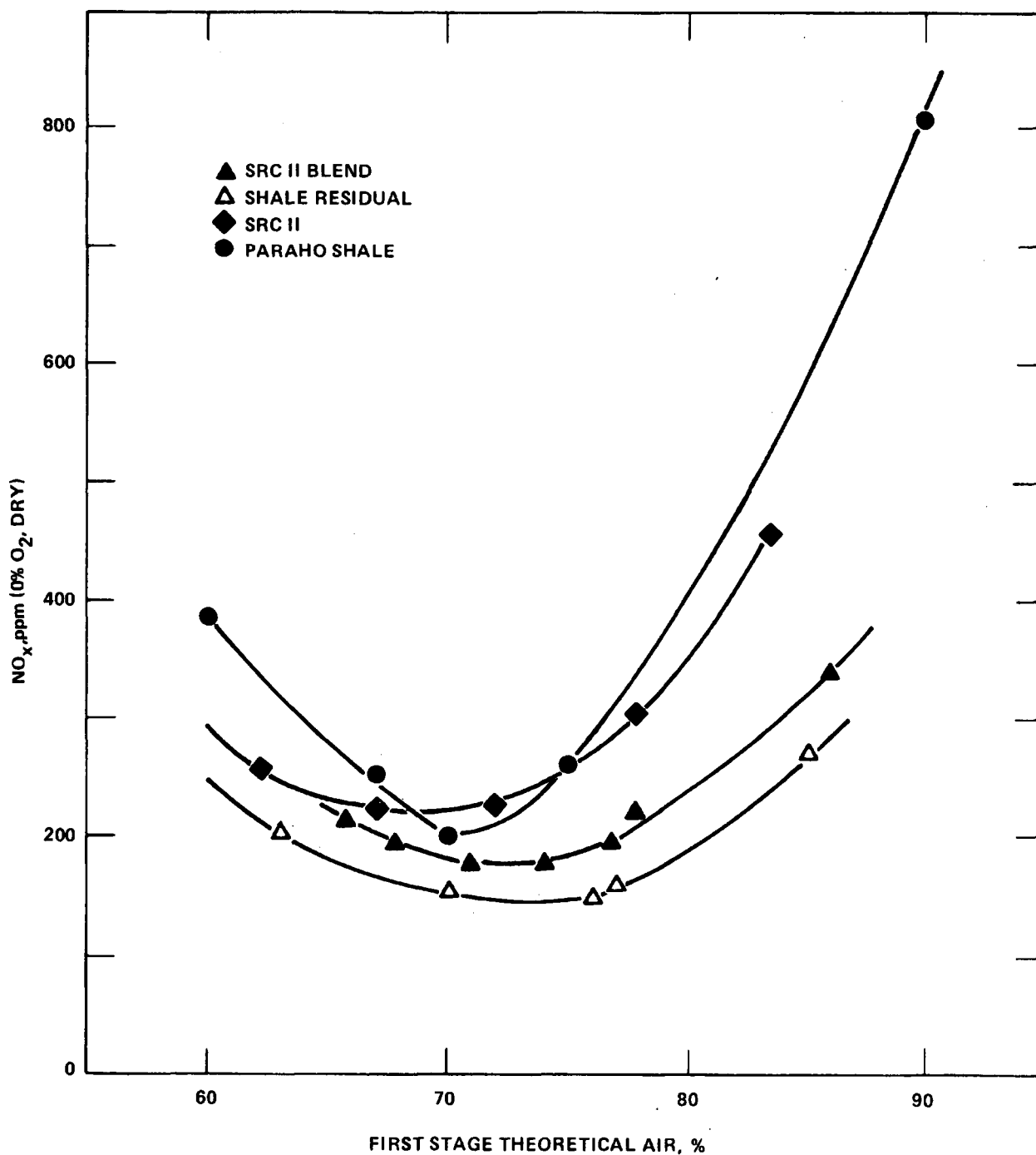
Figure 4. Minimum \text{NO}_x levels achieved with alternative fuels (tunnel furnace primary zone residence time 0.83 sec). 16
