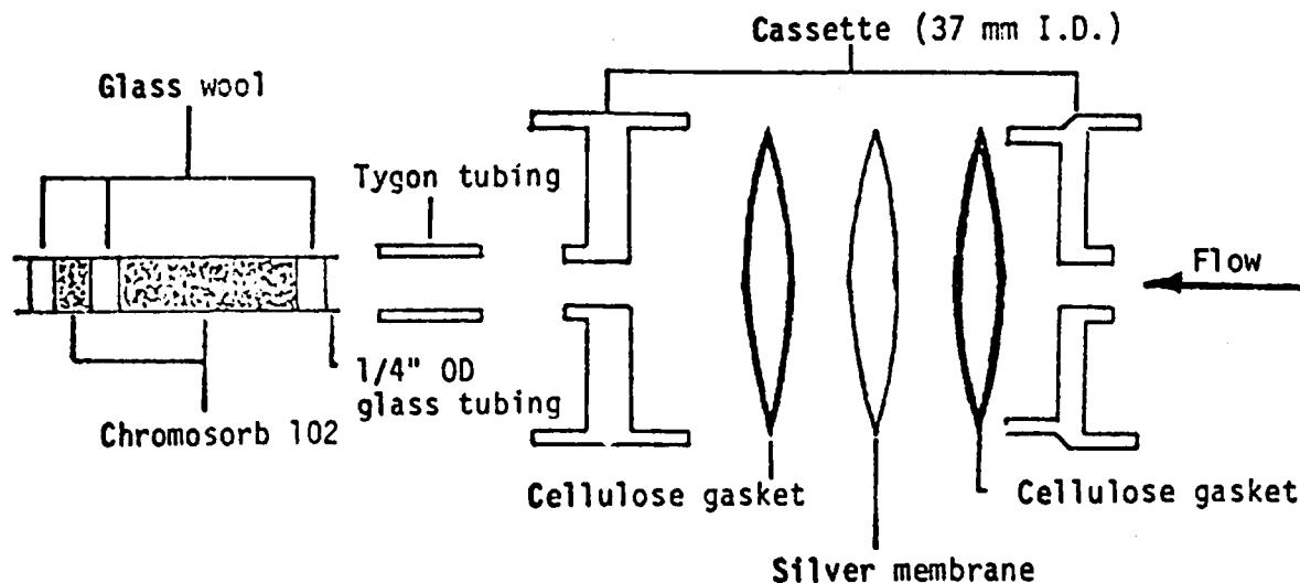
Figure 2. Personal monitoring device for PNA.
