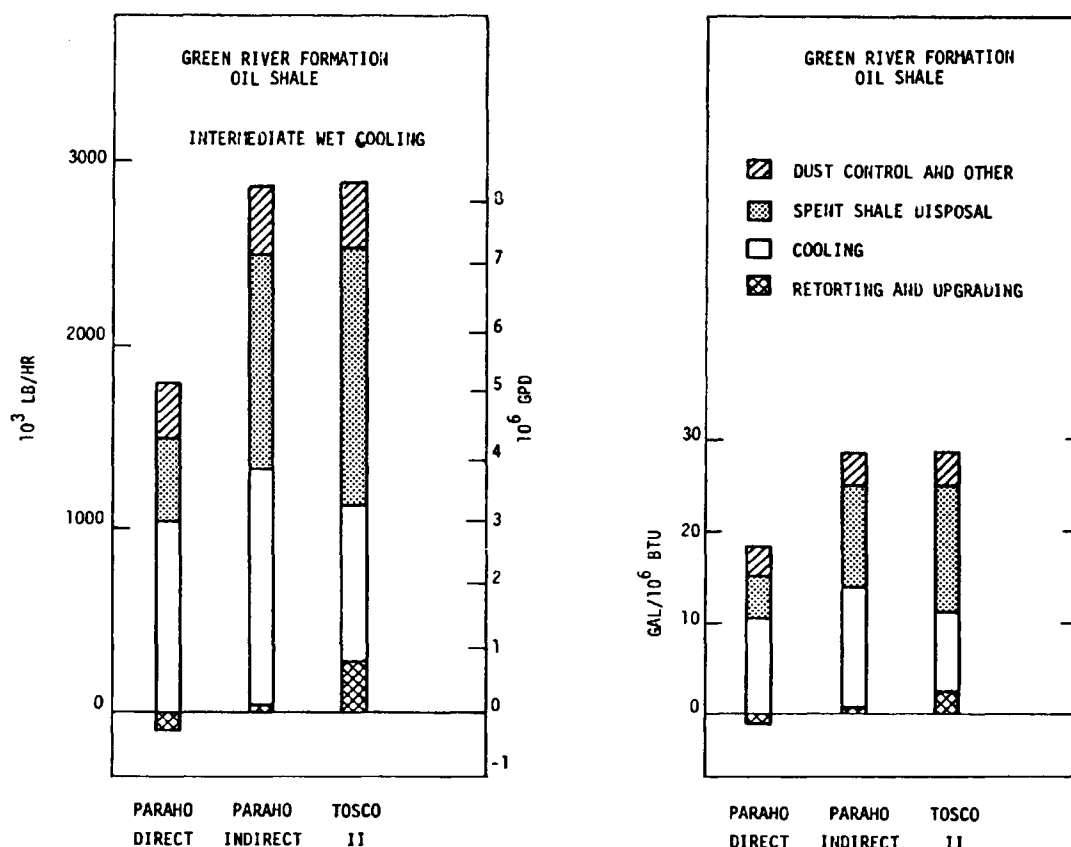
Figure 8. Summary of net water consumed for oil shale conversion plants located in the Western States.
