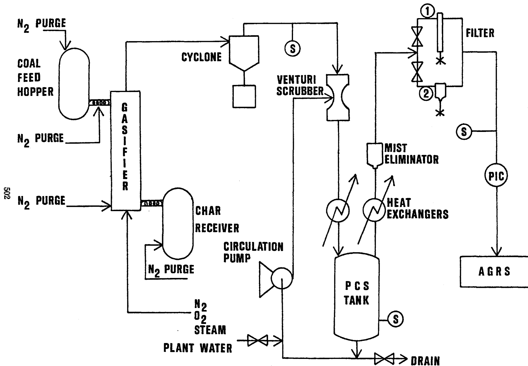
Figure 2. Gasifier-PCS system.
