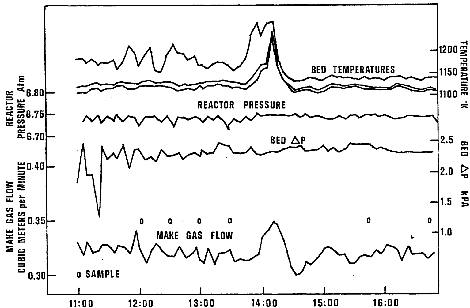
Figure 6. Run GO-13 steady state.
