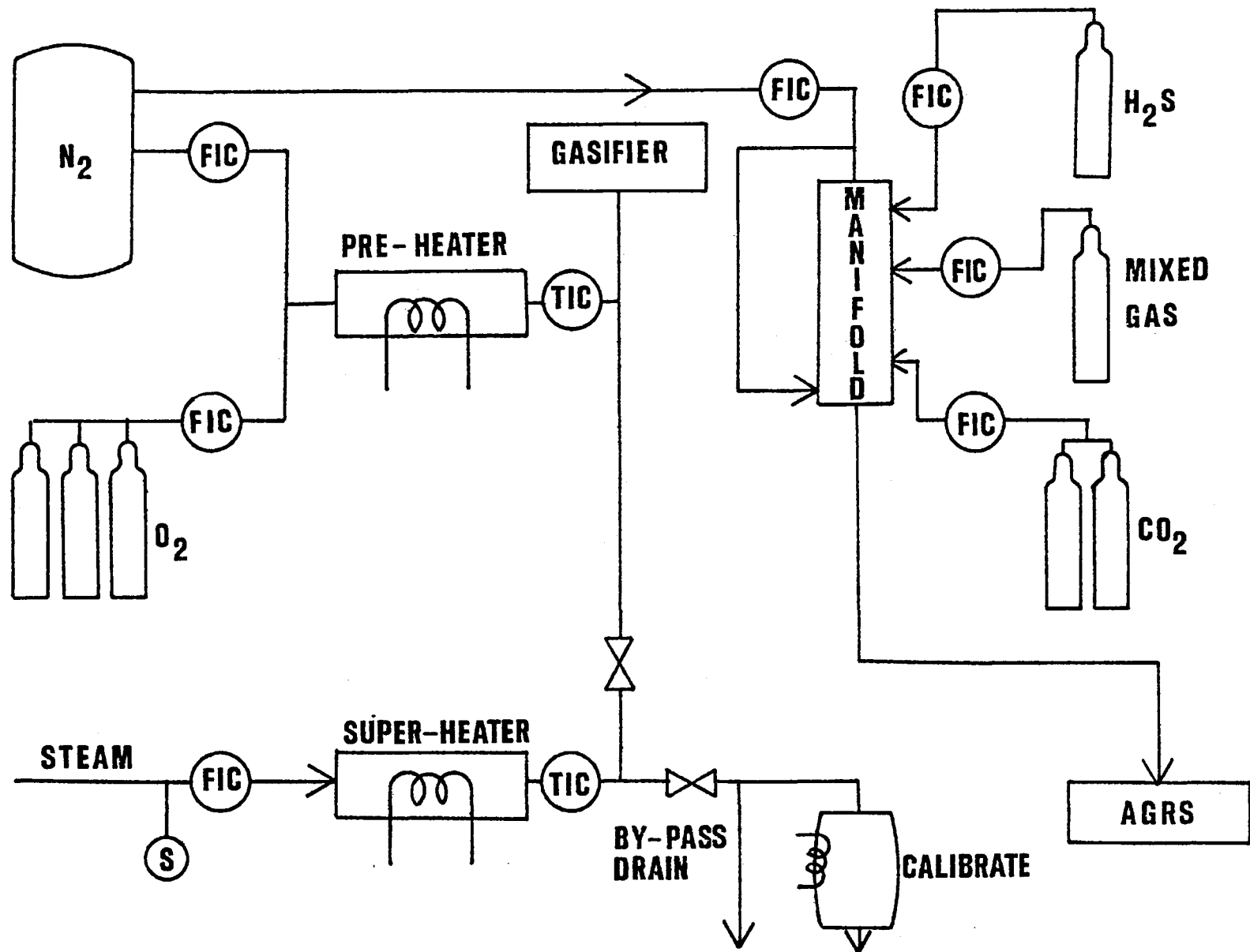
Figure 1. Utilities system.
