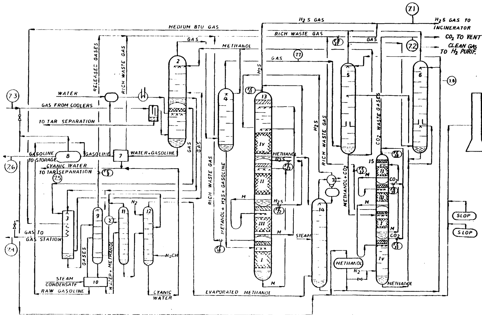
Figure 6. Process flow diagram showing sampling points in Kosovo plant Rectisol section.
