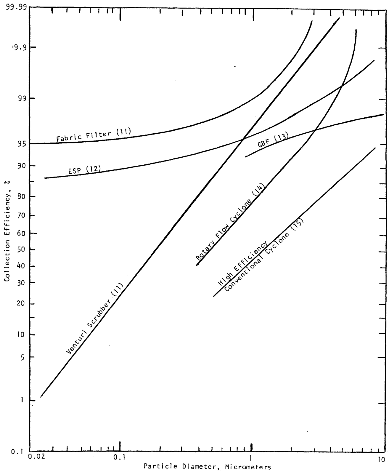
Figure 4. Typical collection efficiencies of control devices.
