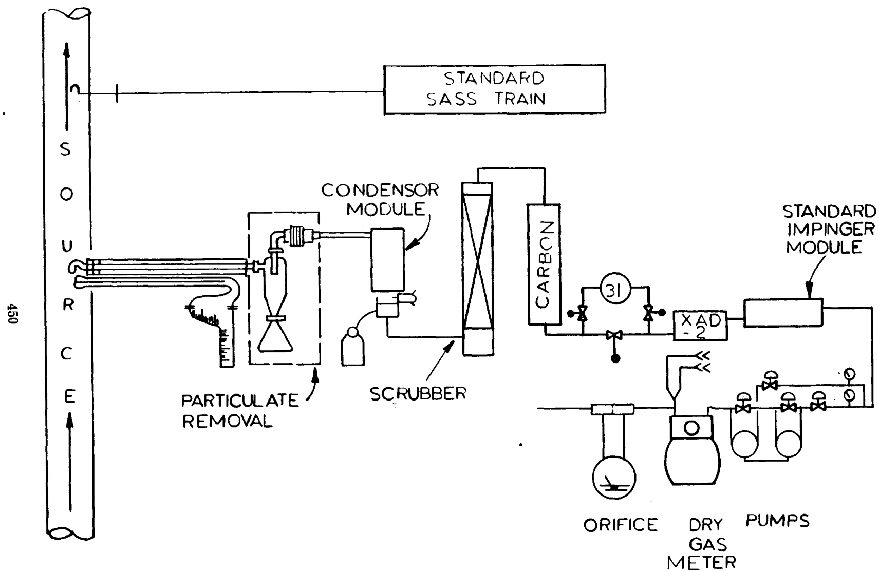
Figure 9. Combined screening train.
