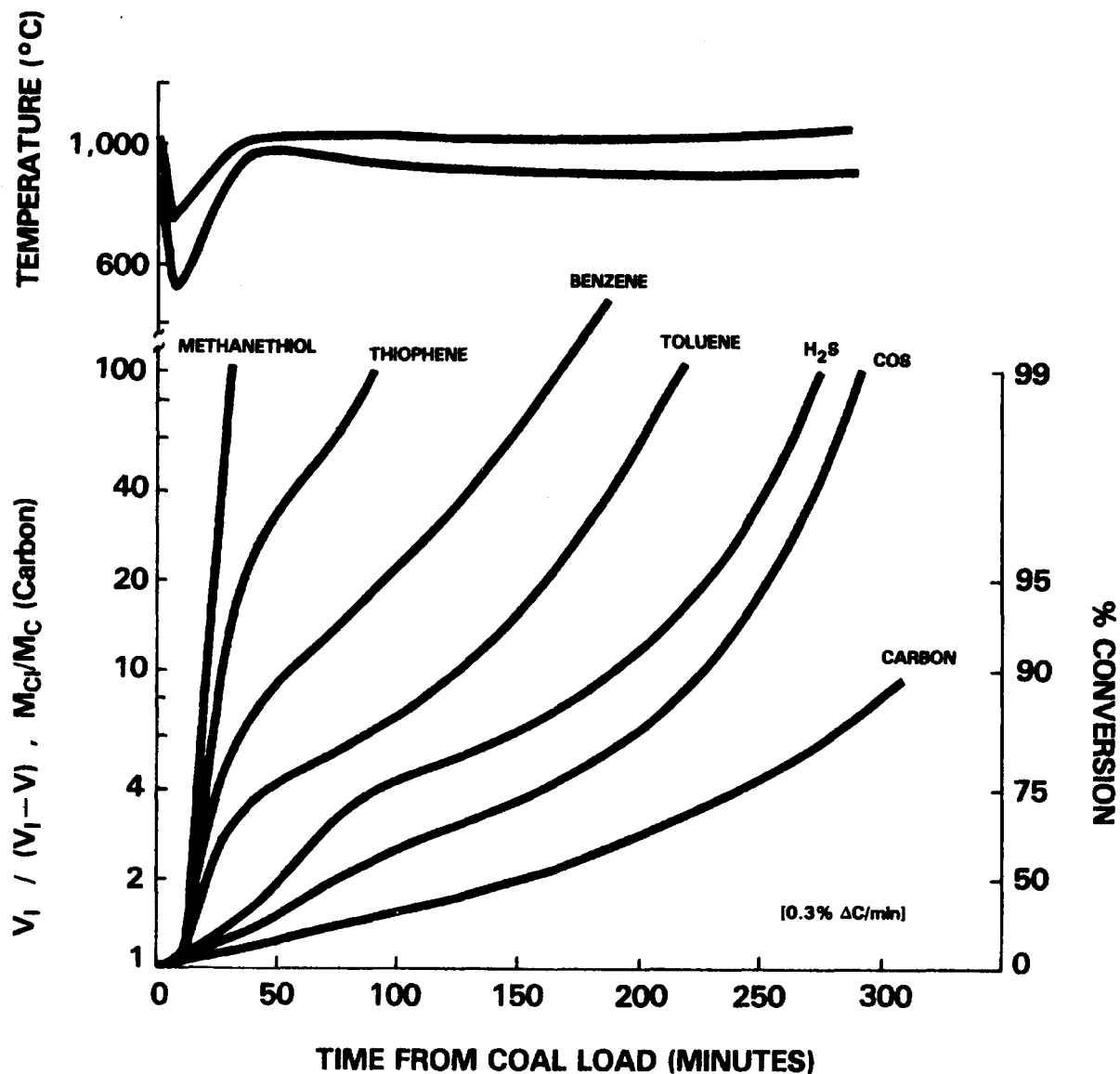
Figure 8. Pollutant kinetics.
