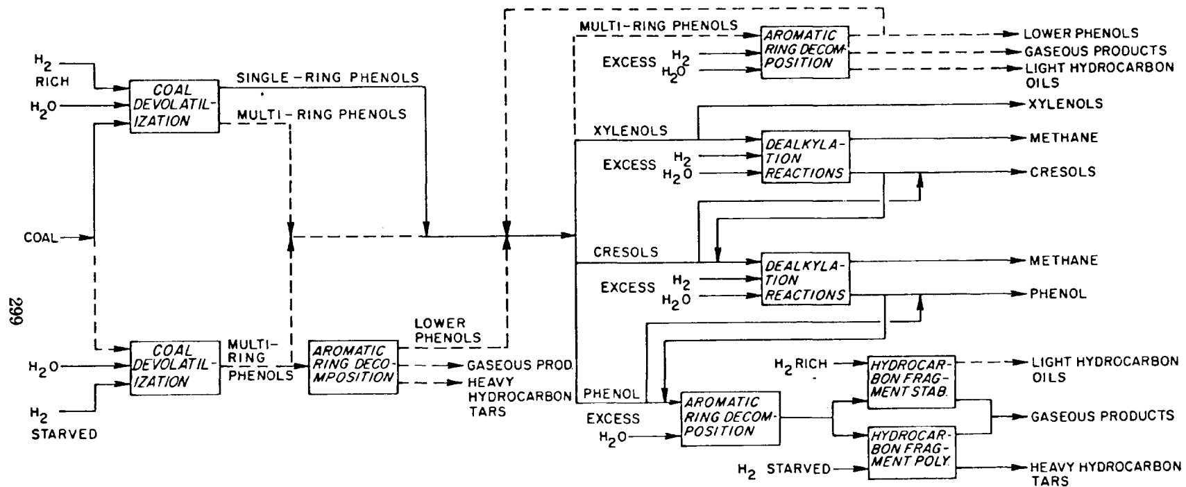
Figure 9. Pattern of phenolic compound production in coal gasification processing.
