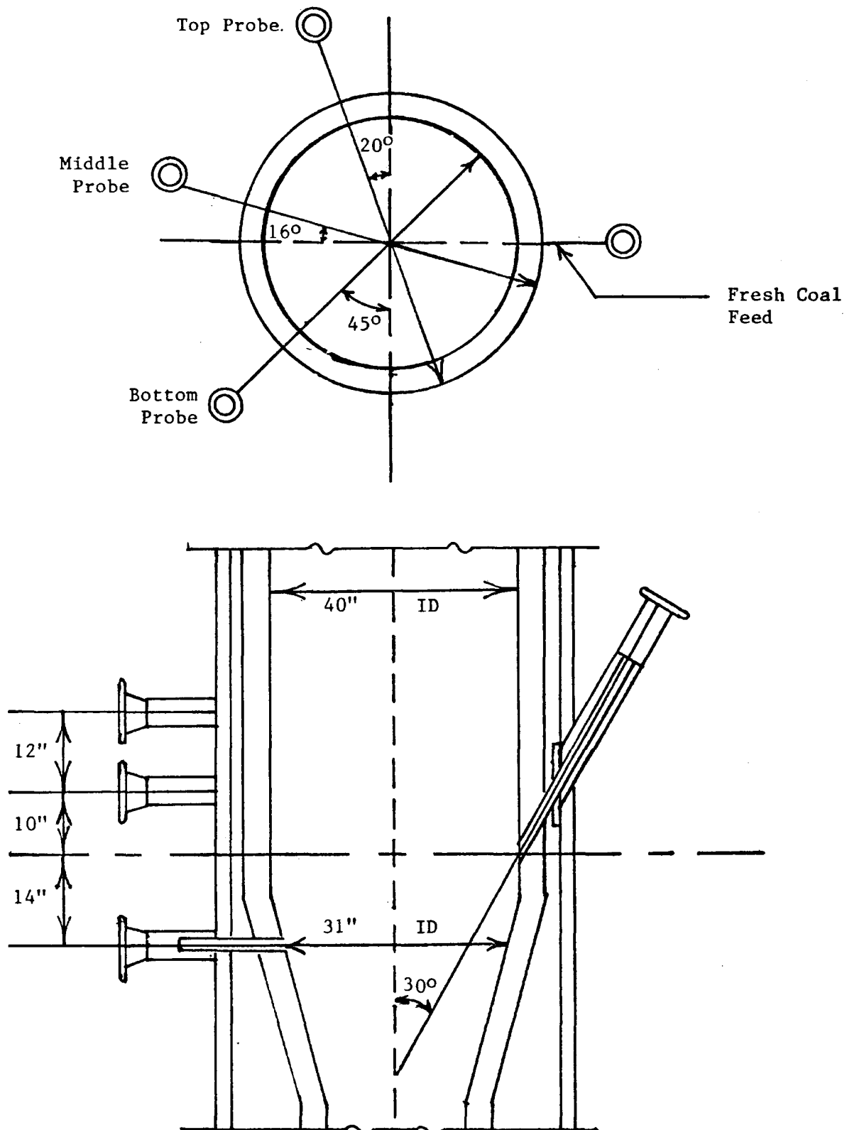
Figure 5. Radial and longitudinal probe orientations in the \text{CO}_2 -acceptor gasifier bed.
