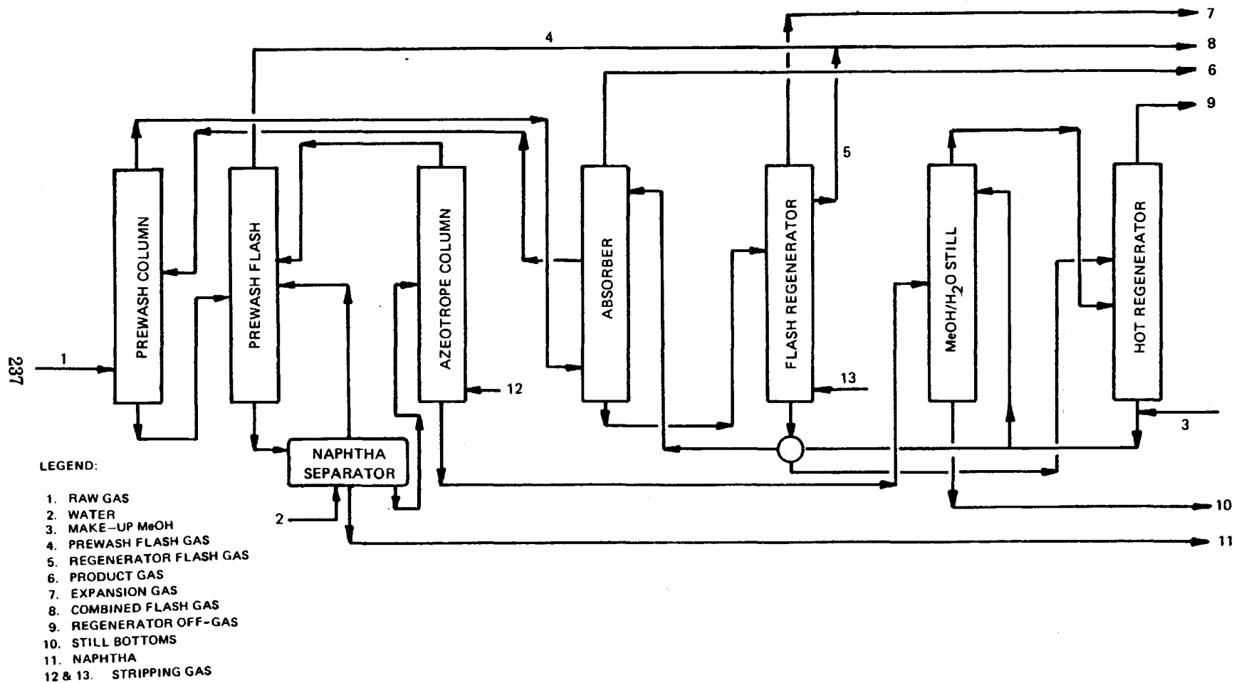
Figure B-1. Rectisol type A 3 (removal of CO 2 from gas mixtures containing little or no H 2 S).
