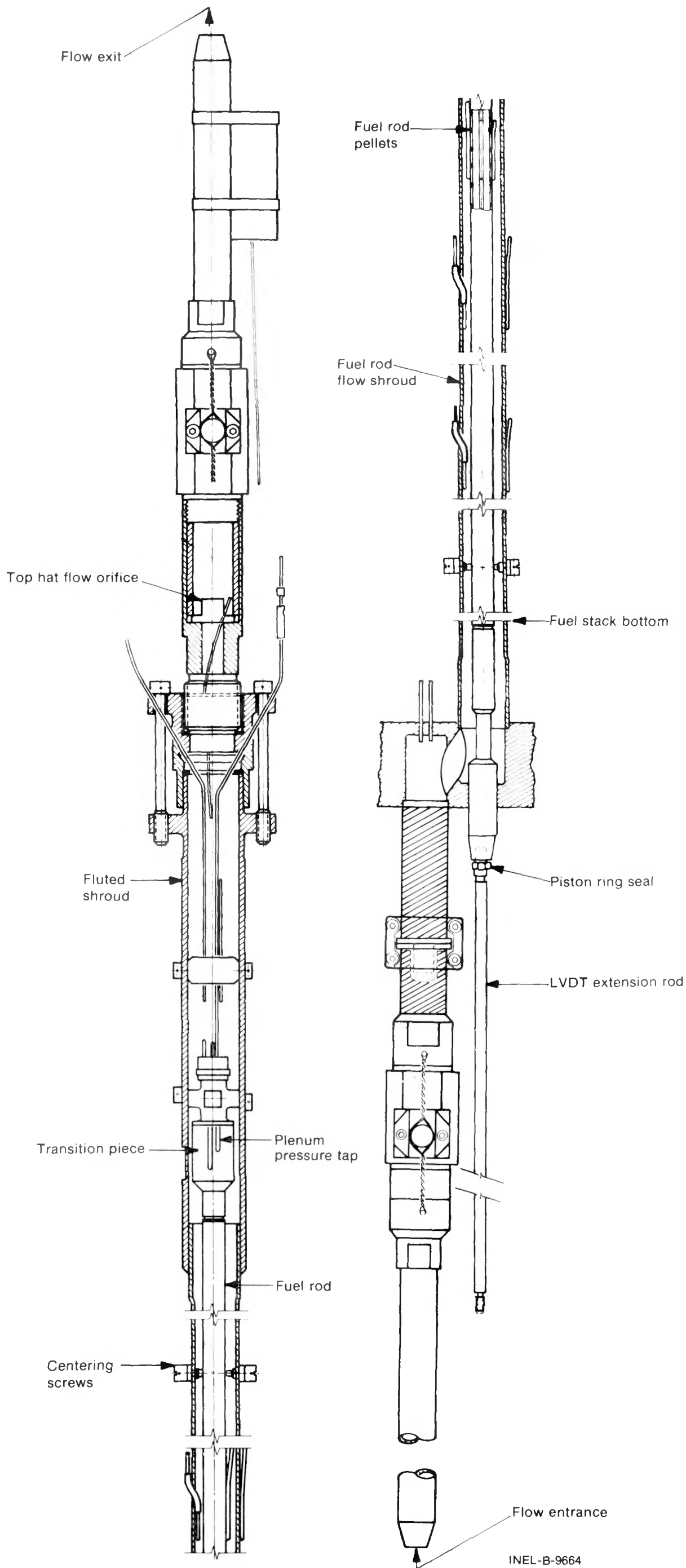
Fig. 5 LOC-11 fuel rod assembly configuration.
