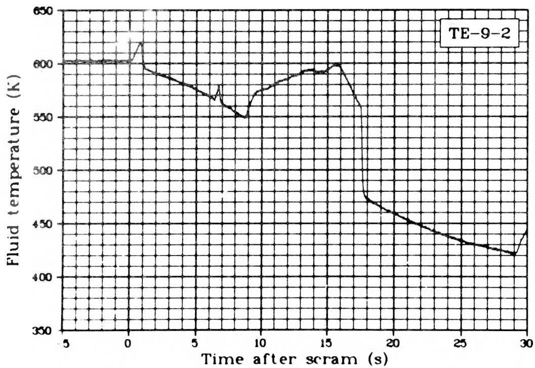
Fig. 48 Fluid temperature of Rod 2, 0.46 m above bottom of fuel stack (TE-9-2), Test LOC-11B.
