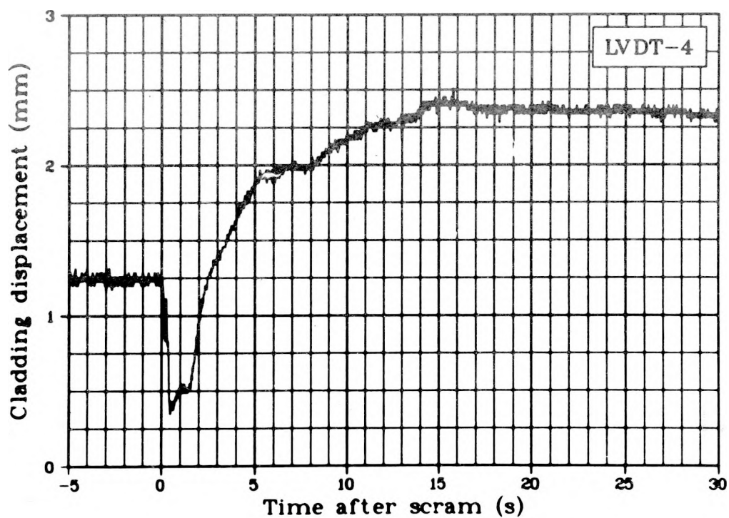
Fig. 218 Cladding displacement of Rod 4 (LVDT-4), Test LOC-11C.
