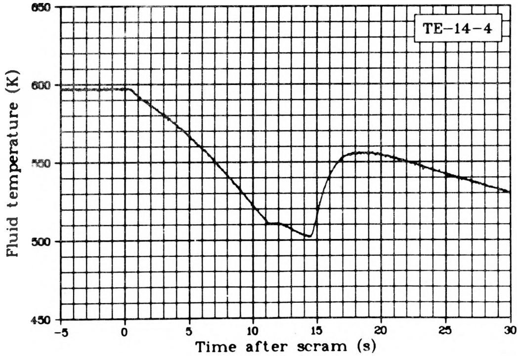
Fig. 161 Fluid temperature of Rod 4 inlet coolant (TE-14-4), Test LOC-11C.
