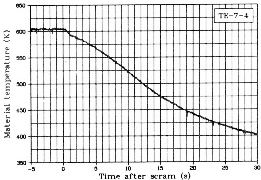
Fig. 183 Material temperature Rod 4, 0.46 m above fuel stack bottom (TE-7-4), Test LOC-11C.
