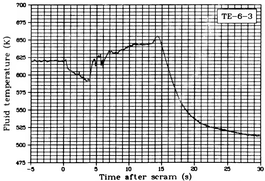
Fig. 150 Fluid temperature of Rod 3, 0.61 m above bottom of fuel stack (TE-6-3), Test LOC-11C.
