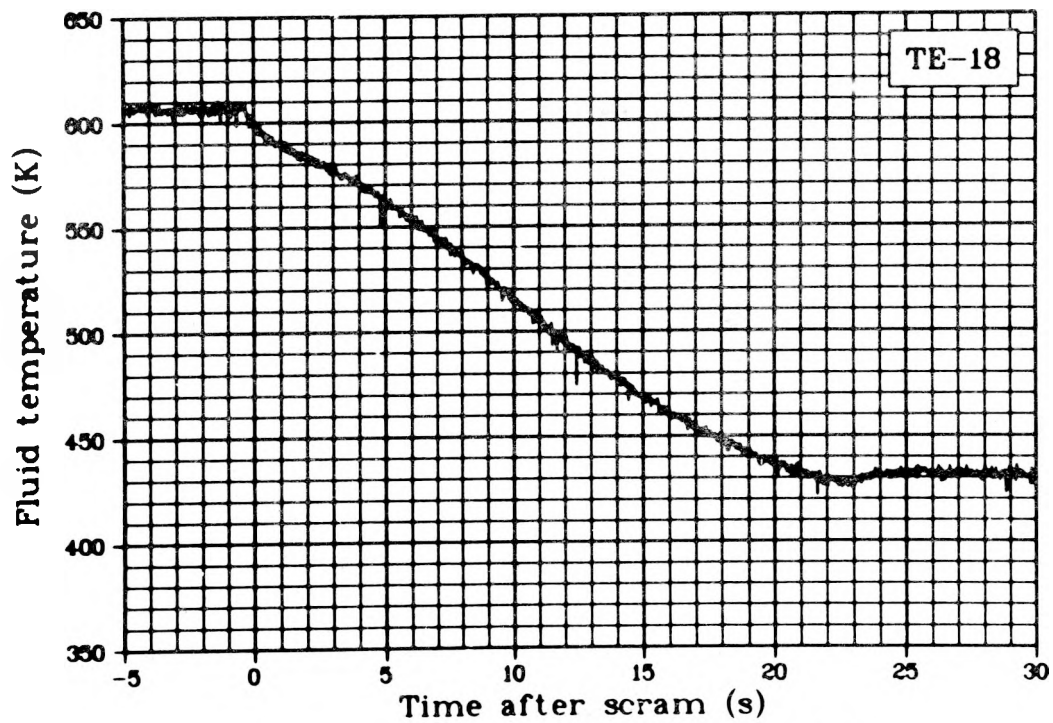
Fig. 165 Fluid temperature in upper plenum exit (TE-18), Test LOC-11C.
