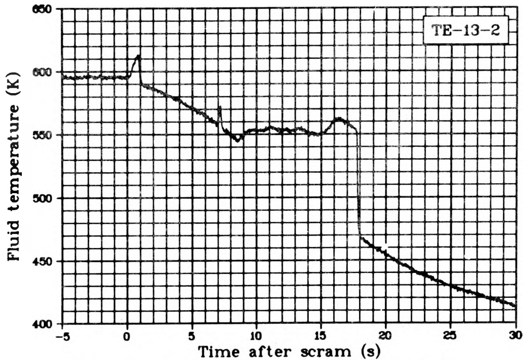
Fig. 52 Fluid temperature of Rod 2, 0.30 m above fuel stack bottom (TE-13-2), Test LOC-11B.
