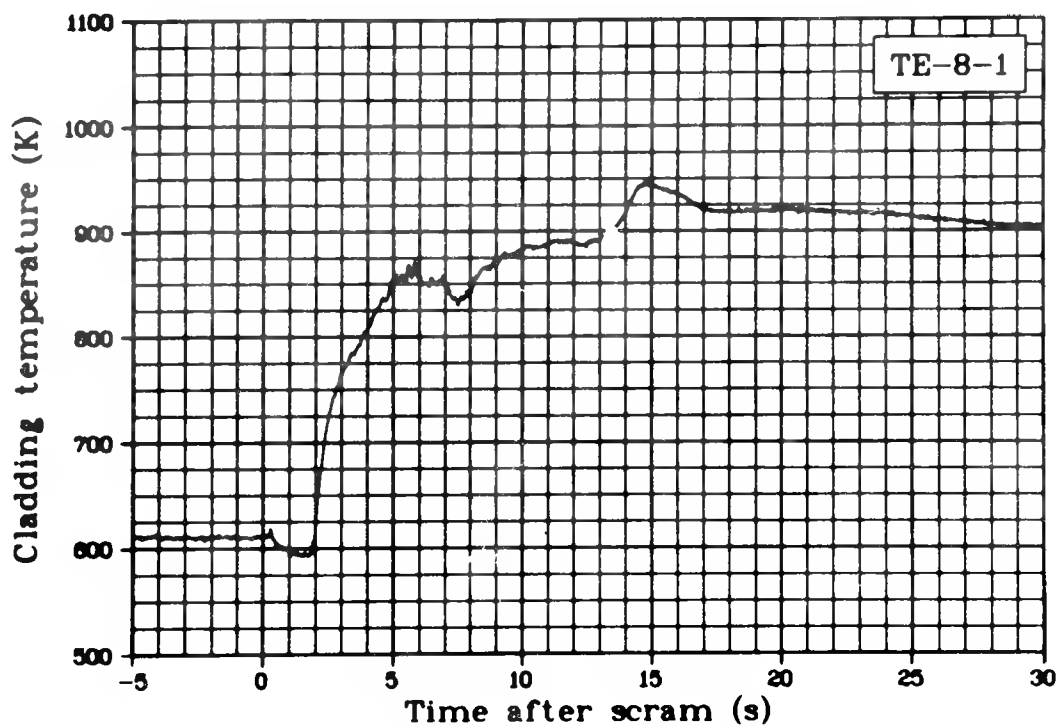
Fig. 129 Cladding temperature Rod 1, 0.61 m above bottom of fuel stack (TE-8-1), Test LOC-11C.
