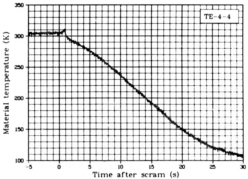
Fig. 75 Material temperature Rod 4, 0.61 m above fuel stack bottom (TE-4-4), Test LOC-11B.
