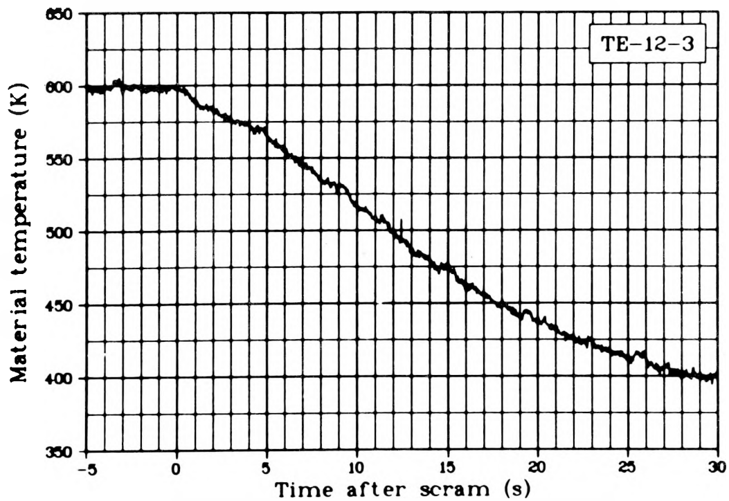
Fig. 186 Material temperature Rod 3, 0.30 m above fuel stack bottom (TE-12-3), Test LOC-11C.
