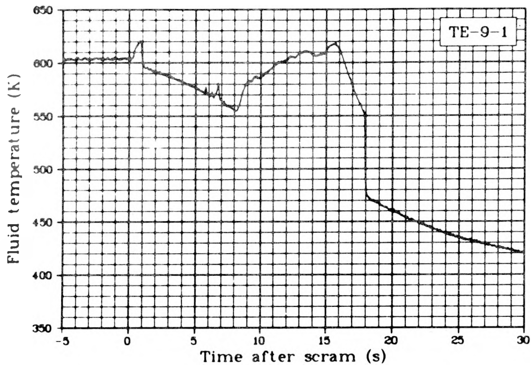
Fig. 47 Fluid temperature of Rod 1, 0.46 m above bottom of fuel stack (TE-9-1), Test LOC-11B.
