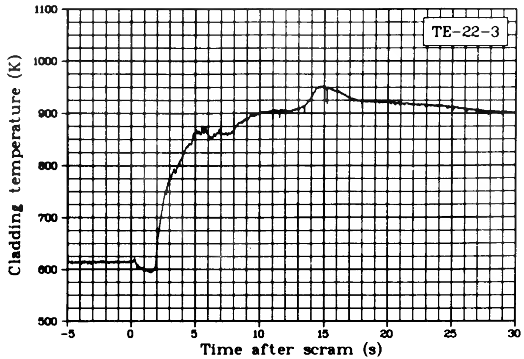
Fig. 139 Cladding temperature Rod 3, 0.61 m above bottom of fuel stack (TE-22-3), Test LOC-11C.
