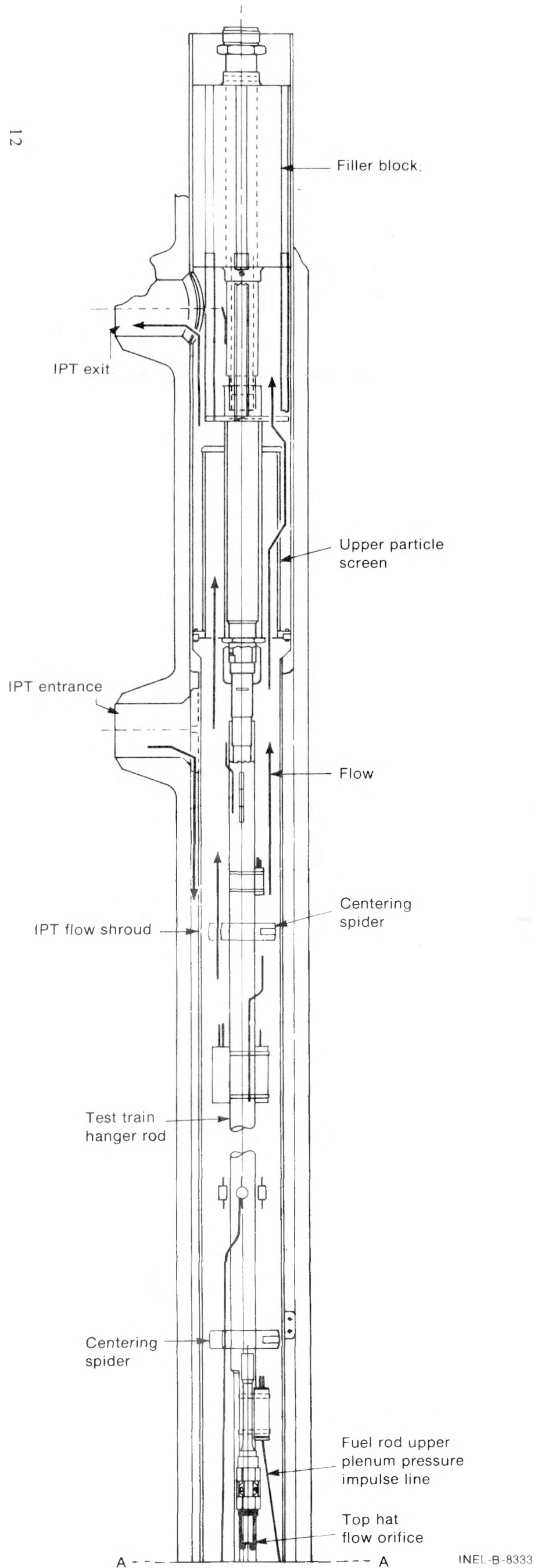
Fig. 7 Test train schematic for LOC-11 tests.
