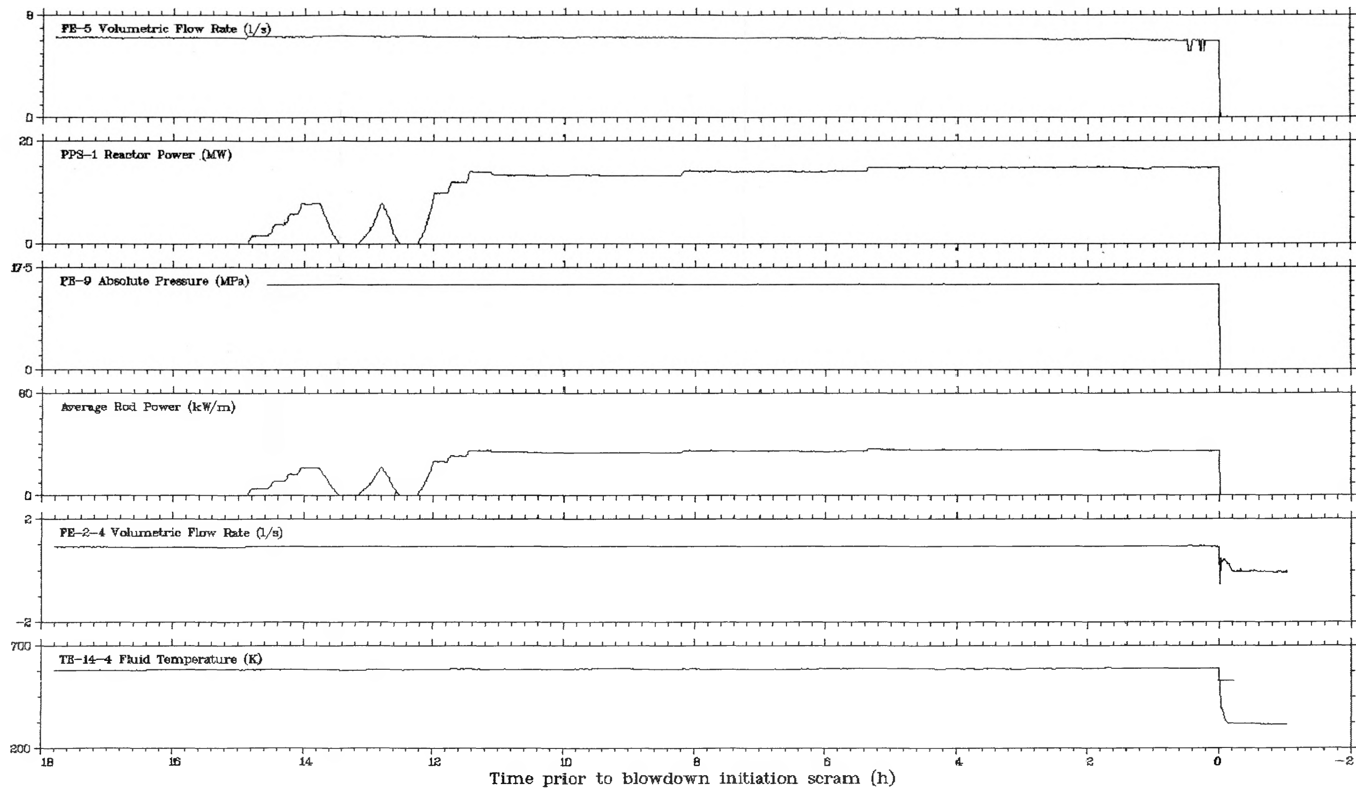
Fig. 8 Operating sequence of nuclear operation for Test LOC-11B.
