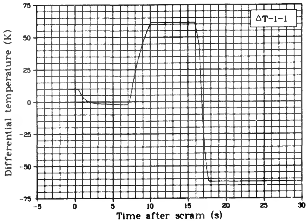
Fig. 172 Differential temperature at fuel inlet and outlet Rod 1 ( \Delta T-1-1 ), Test LOC-11C.
