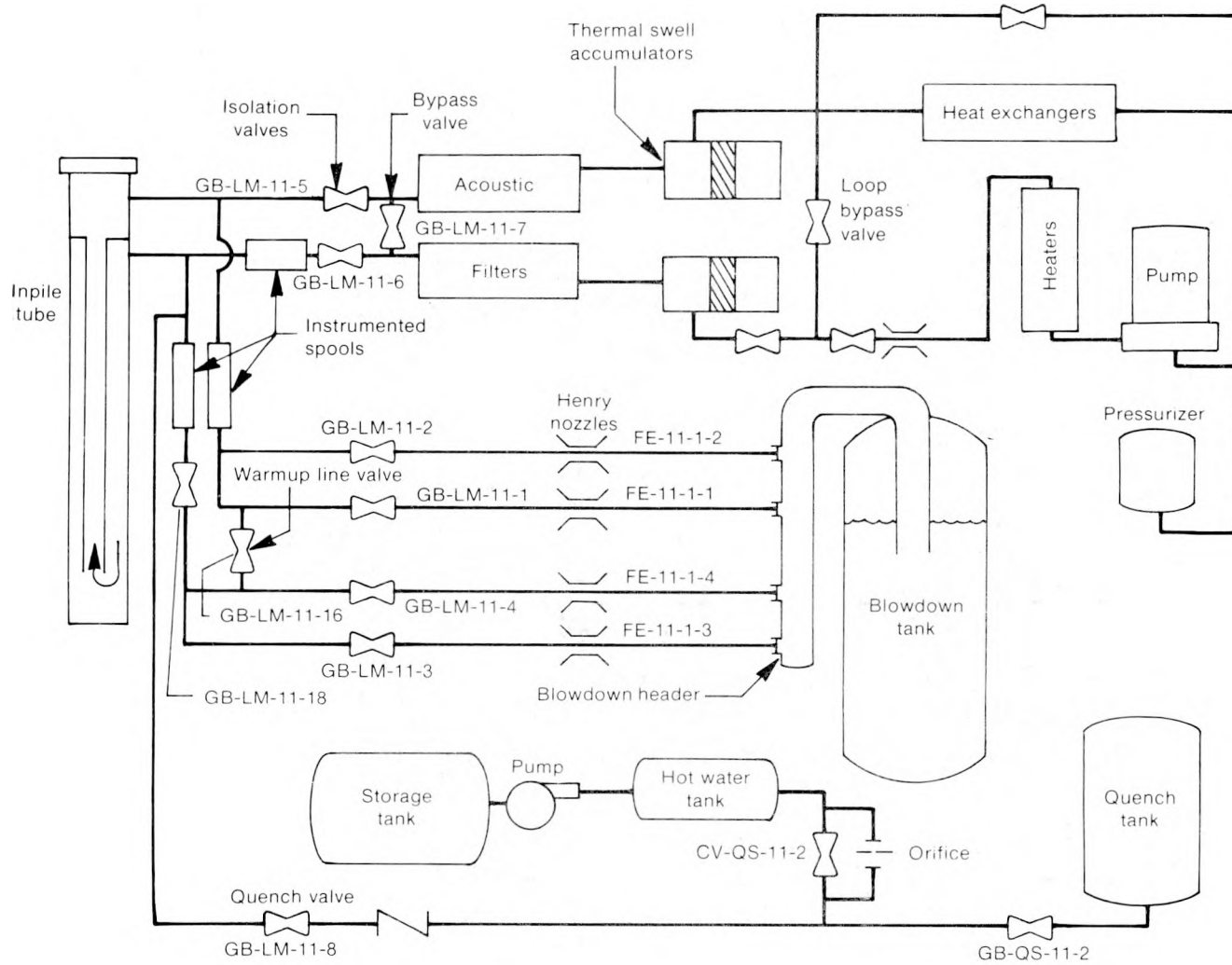
Fig. 3 PBF-LOCA modification system – schematic.
