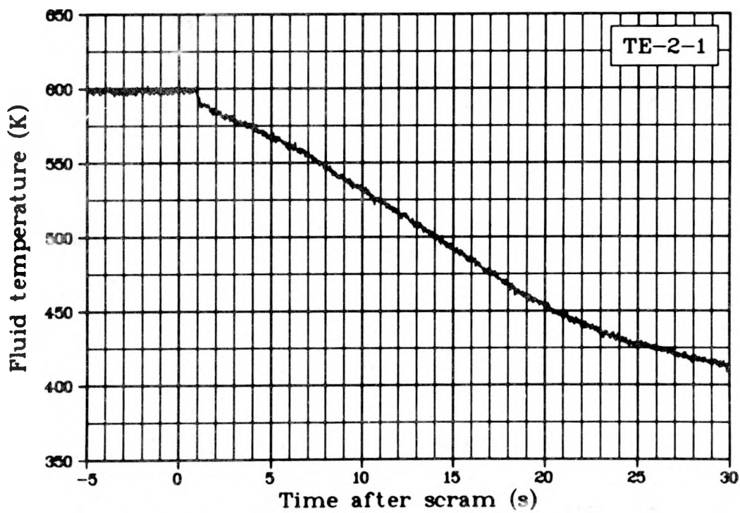
Fig. 41 Fluid temperature of Rod 1 coolant outlet (TE-2-1), Test LOC-11B.
