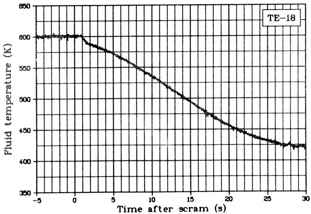
Fig. 60 Fluid temperature in upper plenum exit (TE-18), Test LOC-11B.
