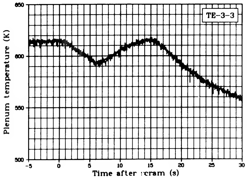
Fig. 124 Plenum temperature in fuel Rod 3 (TE-3-3), Test LOC-11C.
