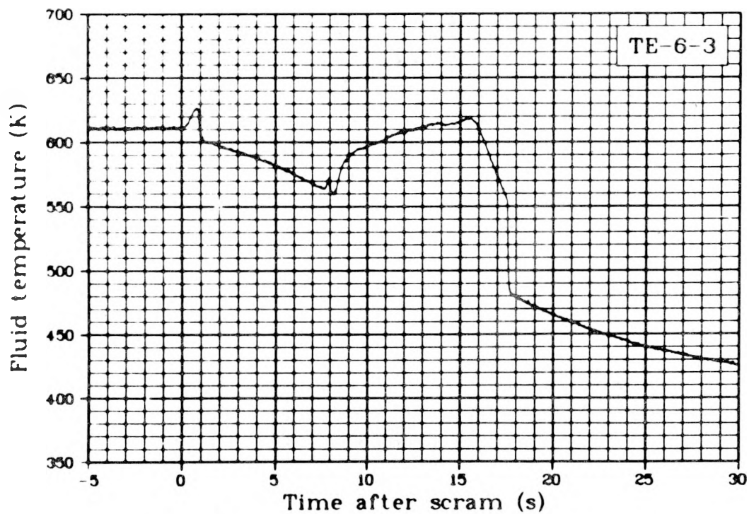
Fig. 45 Fluid temperature of Rod 3, 0.61 m above bottom of fuel stack (TE-6-3), Test LOC-11B.
