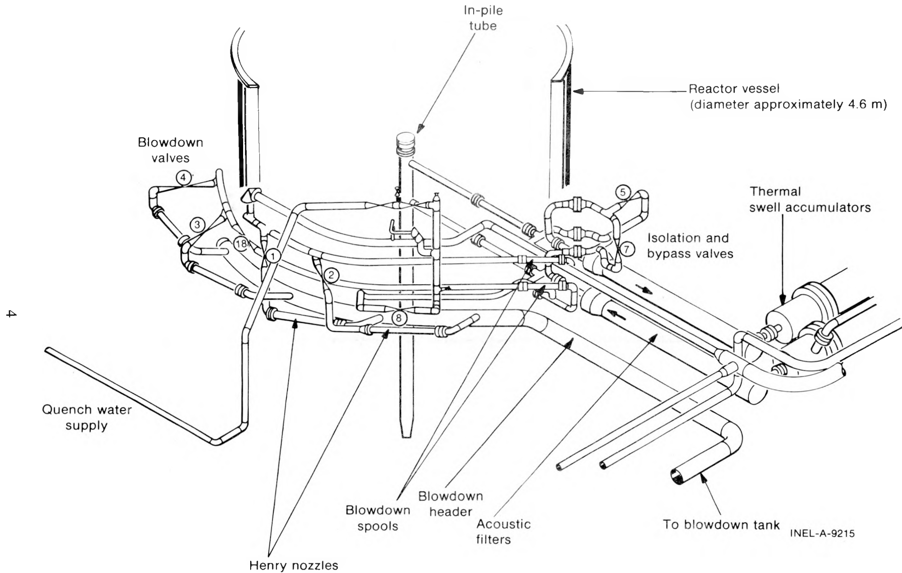
Fig. 1 PBF LOCA system – isometric.
