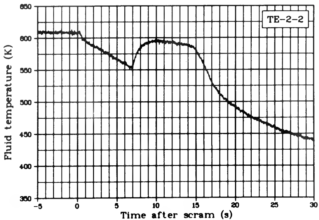
Fig. 147 Fluid temperature of Rod 2 coolant outlet (TE-2-2), Test LOC-11C.
