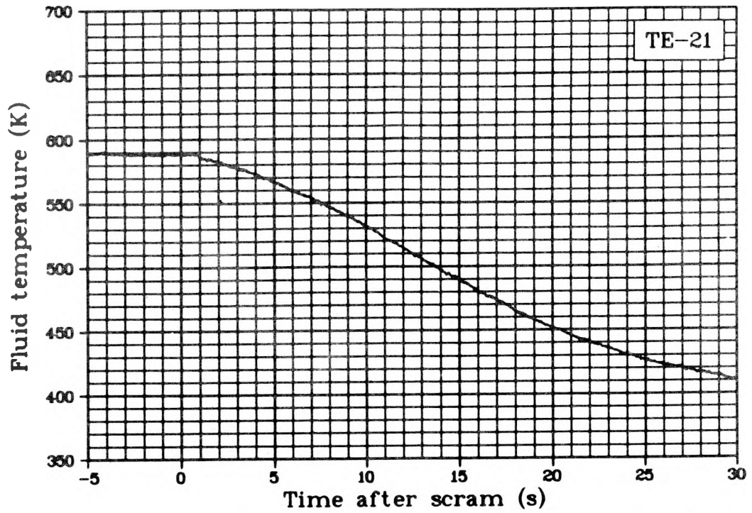
Fig. 63 Fluid temperature inlet spool (TE-21), Test LOC-11B.
