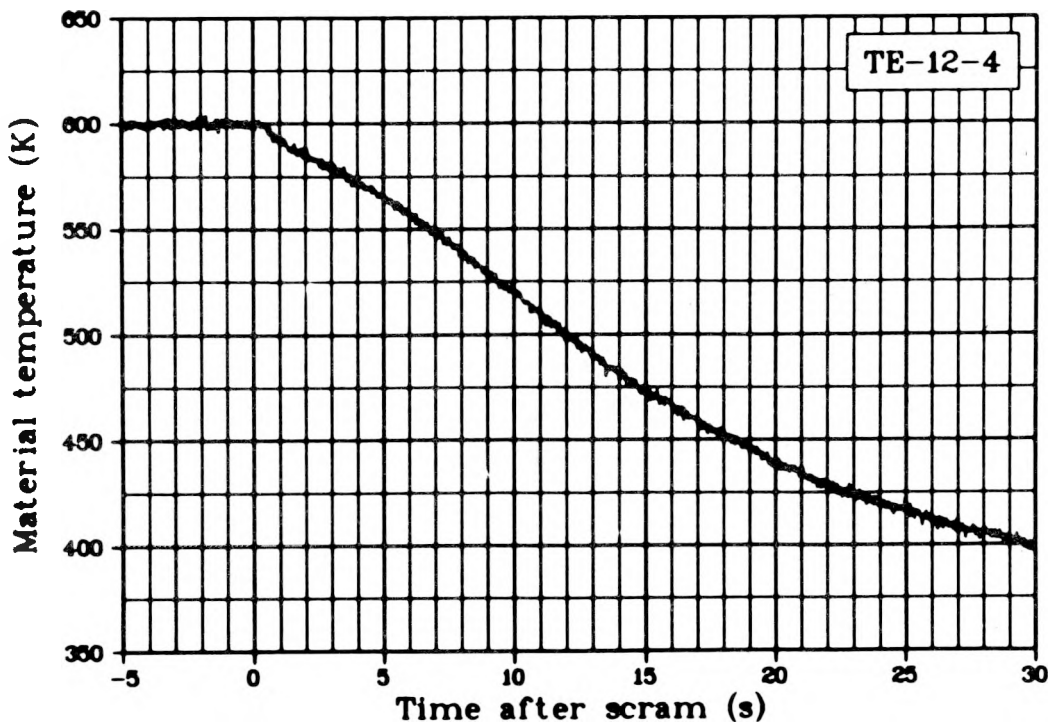
Fig. 187 Material temperature Rod 4, 0.30 m above fuel stack bottom (TE-12-4), Test LOC-11C.
