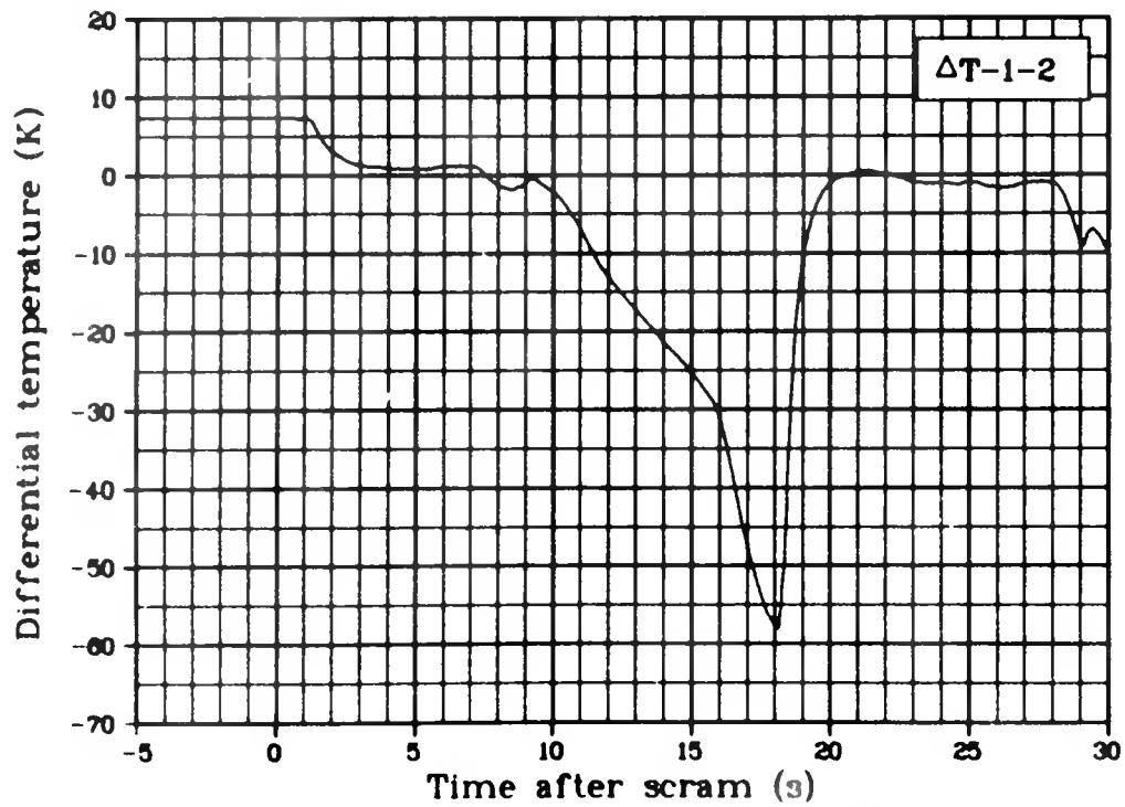
Fig. 69 Differential temperature at fuel inlet and outlet Rod 2 ( \Delta T-1-2 ), Test LOC-11B.
