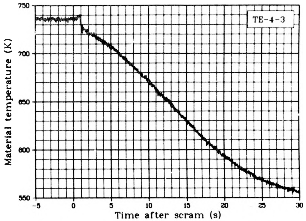
Fig. 74 Material temperature Rod 3, 0.61 m above fuel stack bottom (TE-4-3), Test LOC-11B.
