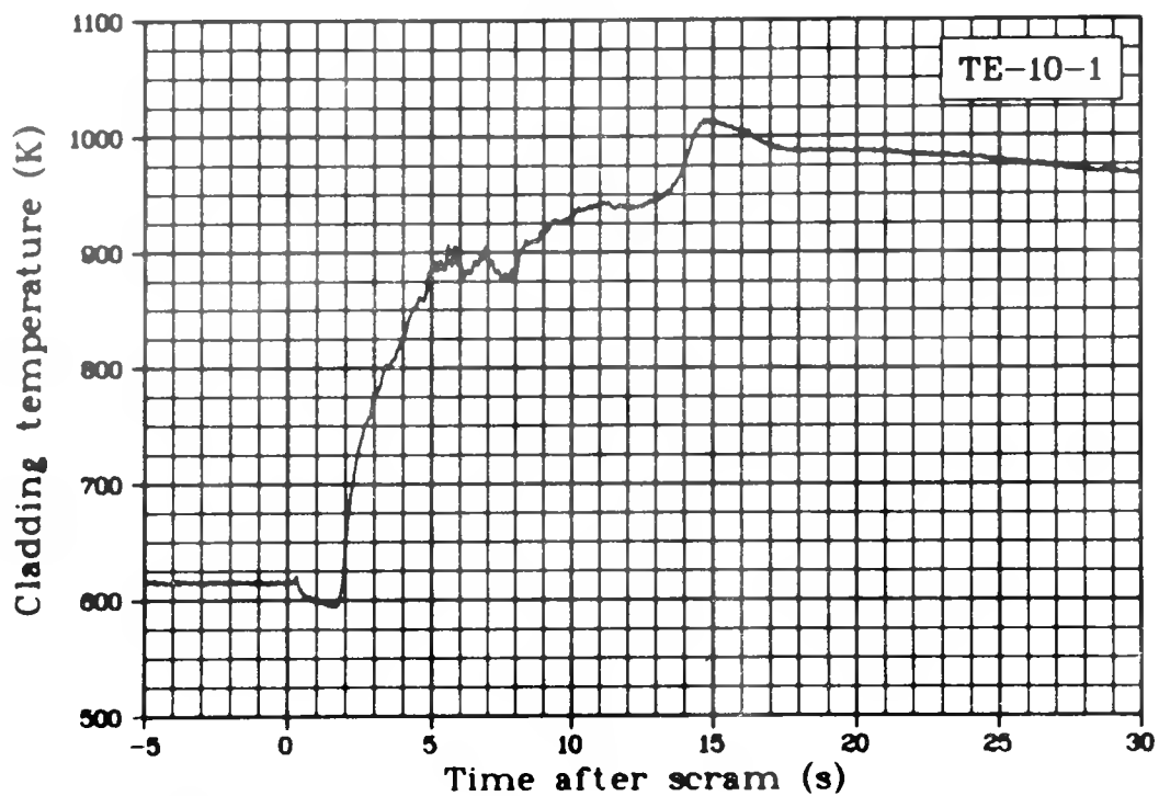
Fig. 133 Cladding temperature Rod 1, 0.53 m above bottom of fuel stack (TE-10-1), Test LOC-11C.
