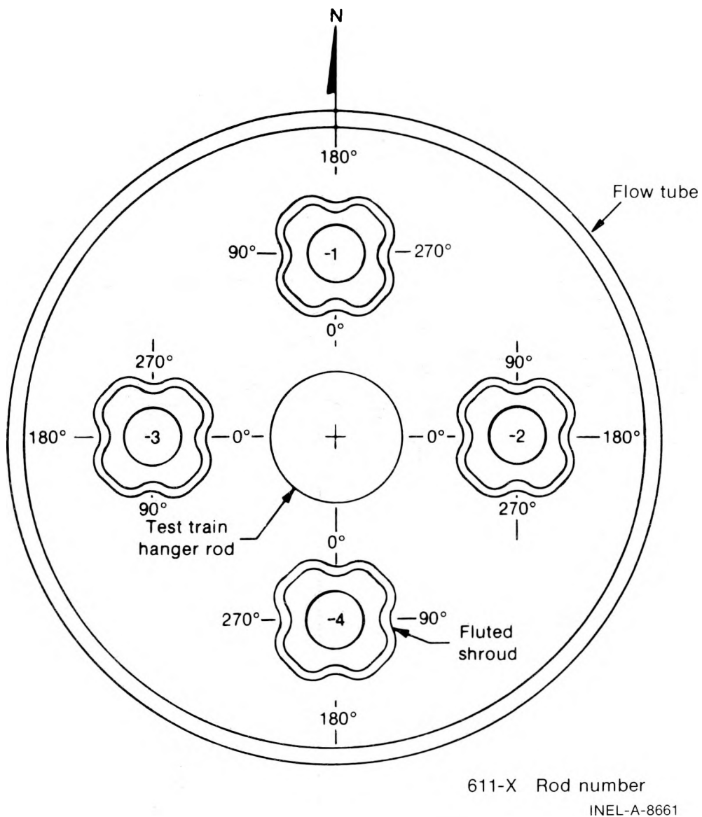
Fig. 6 Orientation of fuel rods for LOC-11 tests.
