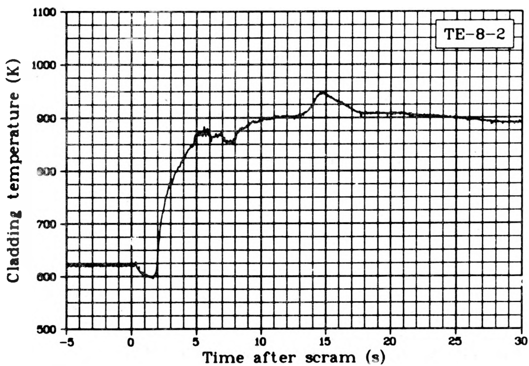
Fig. 130 Cladding temperature Rod 2, 0.61 m above bottom of fuel stack (TE-8-2), Test LOC-11C.
