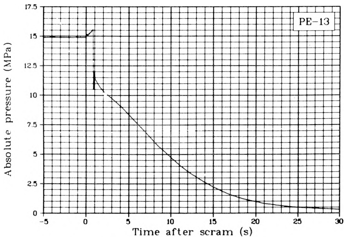
Fig. 91 Absolute pressure in hot leg blowdown spool (PE-13), Test LOC-11B.
