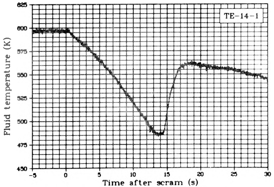
Fig. 159 Fluid temperature of Rod 1 inlet coolant (TE-14-1), Test LOC-11C.
