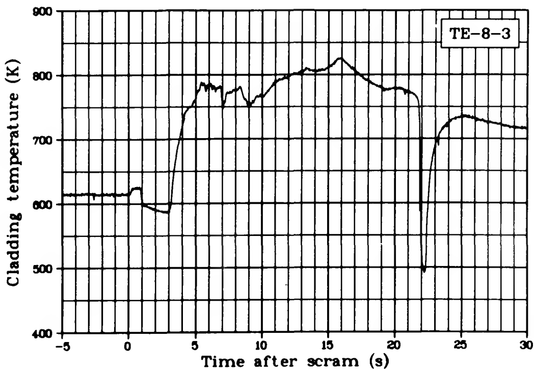
Fig. 26 Cladding temperature Rod 3, 0.61 m above bottom of fuel stack (TE-8-3), Test LOC-11B.
