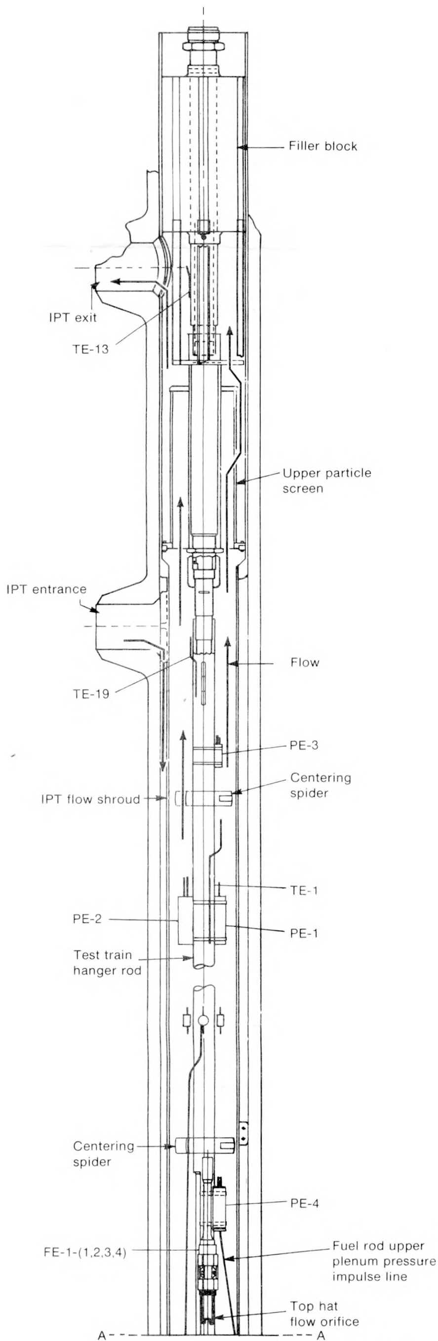
Fig. 12 LOC-11 test train assembly with instrumentation.
