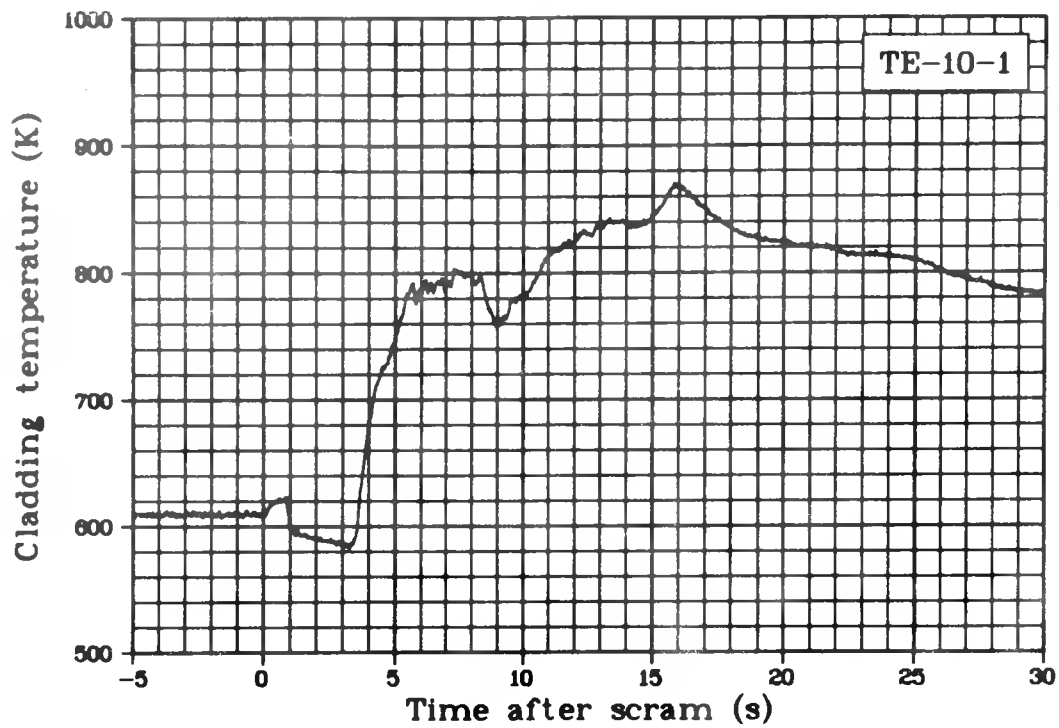
Fig. 28 Cladding temperature Rod 1, 0.53 m above bottom of fuel stack (TE-10-1), Test LOC-11B.
