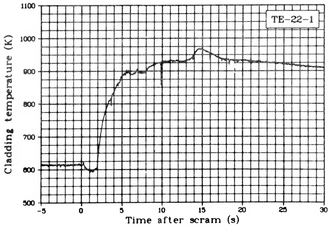
Fig. 137 Cladding temperature Rod 1, 0.61 m above bottom of fuel stack (TE-22-1), Test LOC-11C.
