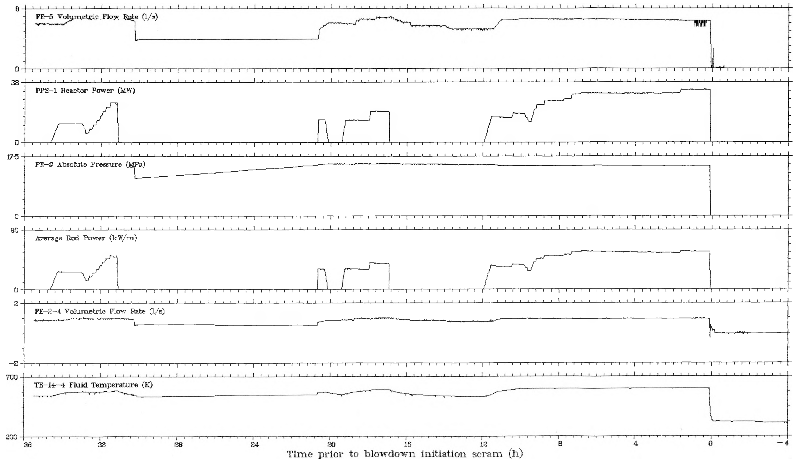
Fig. 9 Operating sequence of nuclear operation for Test LOC-11C.
