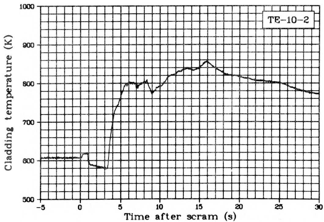
Fig. 29 Cladding temperature Rod 2, 0.53 m above bottom of fuel stack (TE-10-2), Test LOC-11B.
