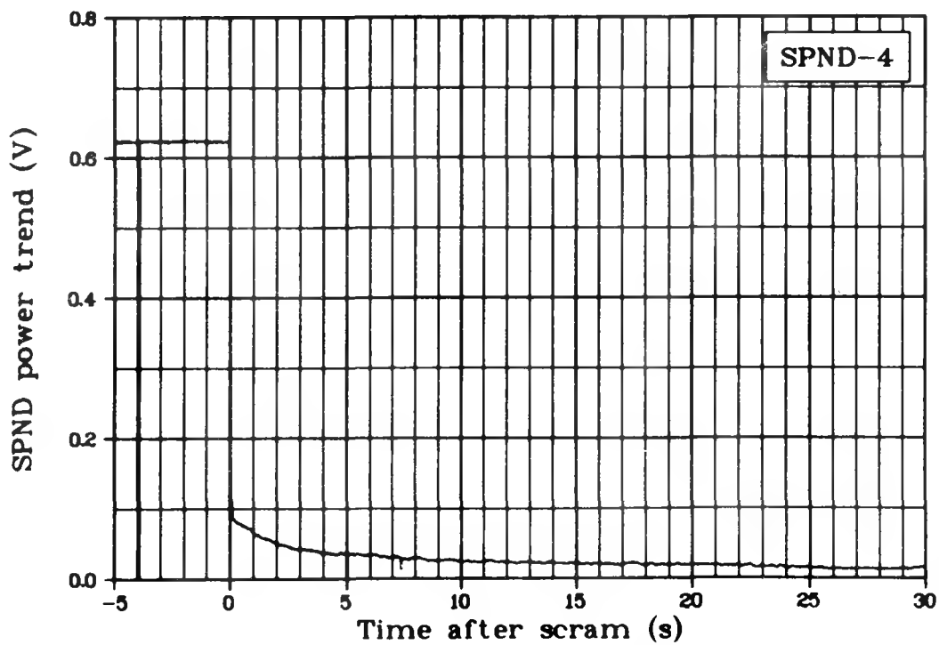
Fig. 120 SPND power trend 0.30 m above fuel stack bottom (SPND-4), Test LOC-11B.
