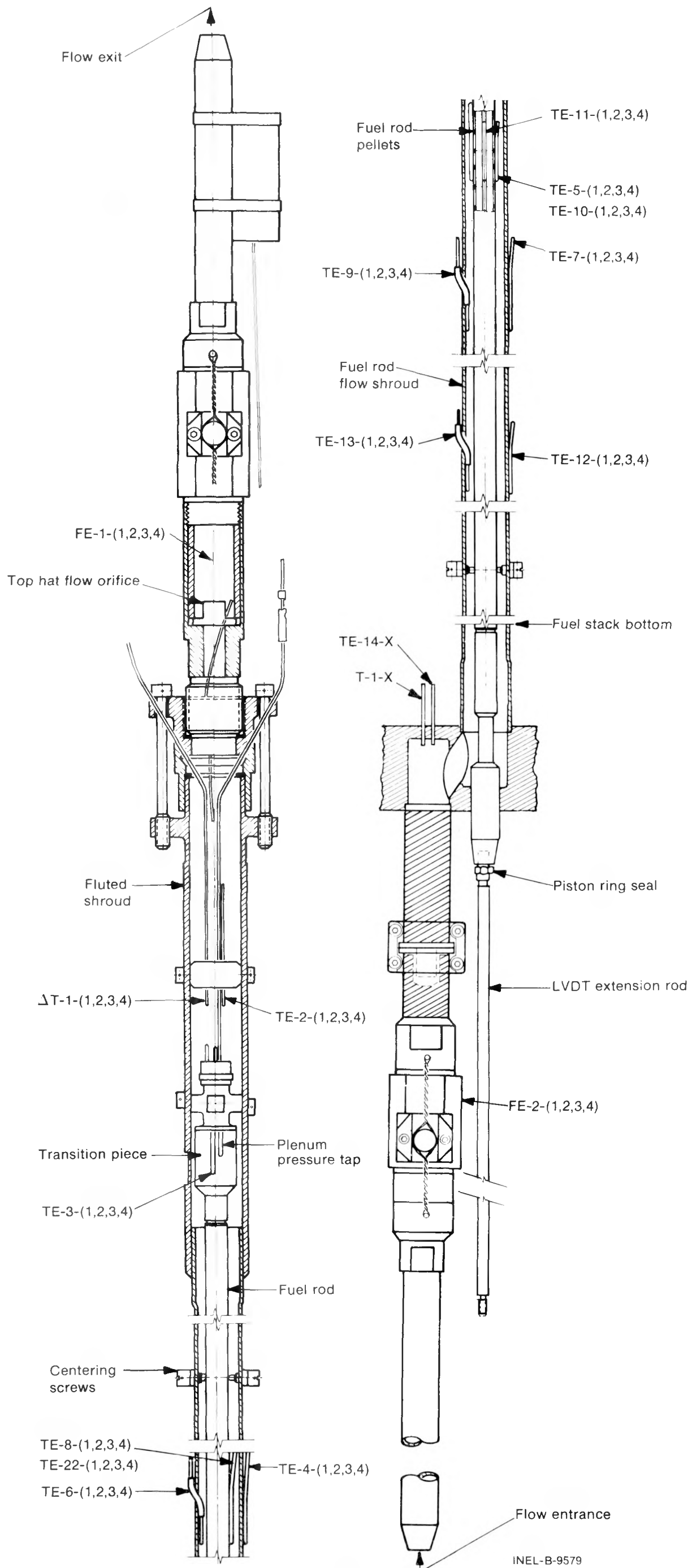
Fig. 11 LOC-11 fuel rod assembly with instrumentation.
