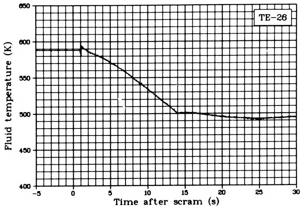
Fig. 67 Fluid temperature in hot leg blowdown spool (TE-26), Test LOC-11B.
