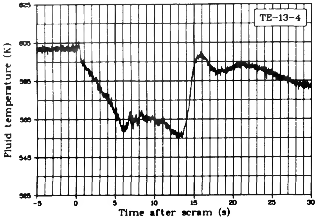
Fig. 158 Fluid temperature of Rod 4, 0.30 m above fuel stack bottom (TE-13-4), Test LOC-11C.
