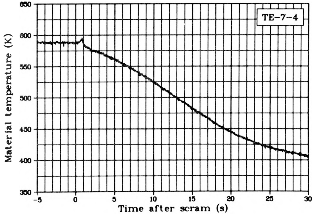
Fig. 79 Material temperature Rod 4, 0.46 m above fuel stack bottom (TE-7-4), Test LOC-11B.
