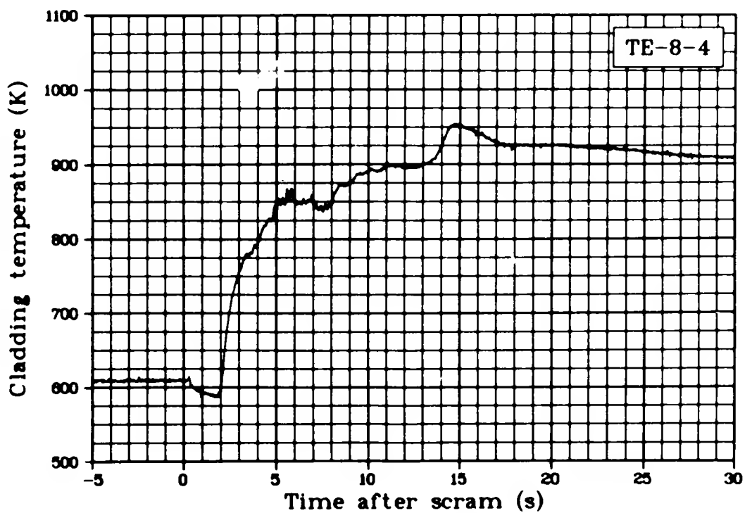
Fig. 132 Cladding temperature Rod 4, 0.61 m above bottom of fuel stack (TE-8-4), Test LOC-11C.
