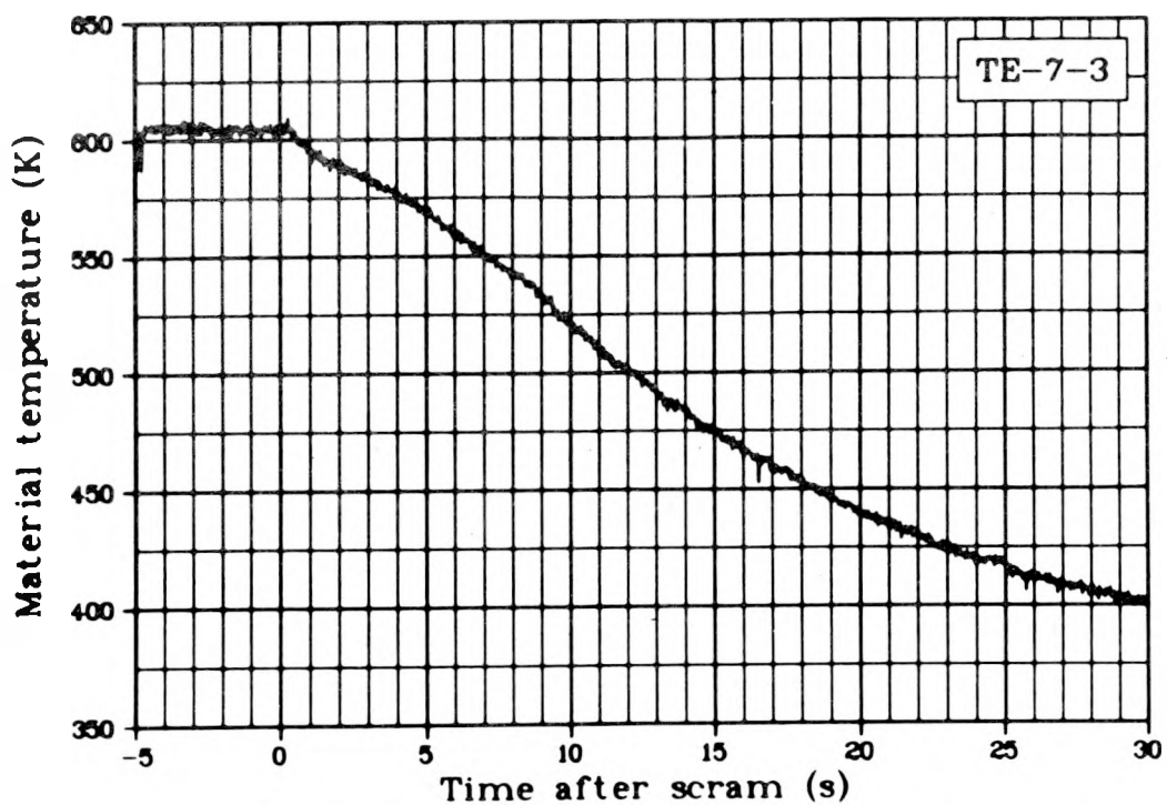
Fig. 182 Material temperature Rod 3, 0.46 m above fuel stack bottom (TE-7-3), Test LOC-11C.
