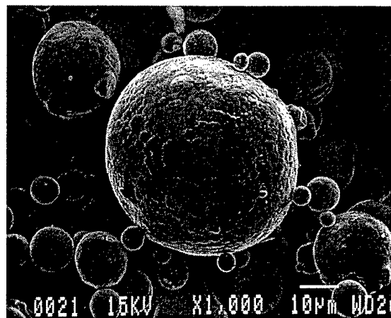
(b) Fe-15Al-2.8Si
