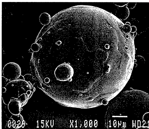
(a) Fe-15Al
