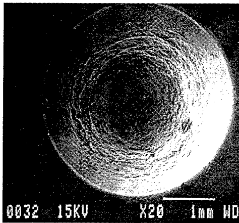
Figure 3.35 - SEM fracture of as-extruded Fe-15Al tested at 25°C
