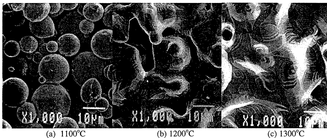
Figure 3.16 - SEM of Surface Topology for Vacuum Sintered Fe-15Al-2.8Si
