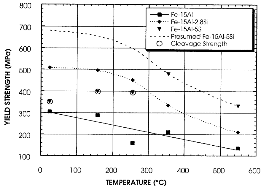
Figure 3.29 - Yield strength as a function of temperature for extruded Fe-15Al-xSi alloys (heat treatment: 600°C/7 days/WQ)
