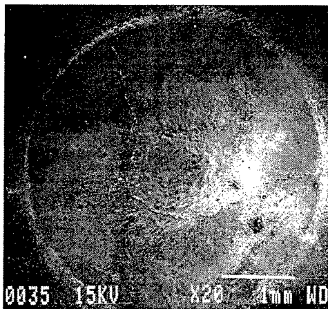
Figure 3.36 - SEM fracture of as-extruded Fe-15Al-2.8Si tested at 25°C
