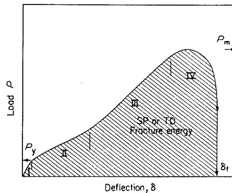
Figure 2.3 - Load-Displacement curve for small punch test
