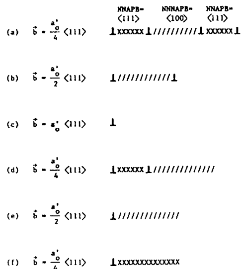
Figure 1.6 - Superdislocations which can exist in \text{DO}_3 and B2 Superlattices [22]
