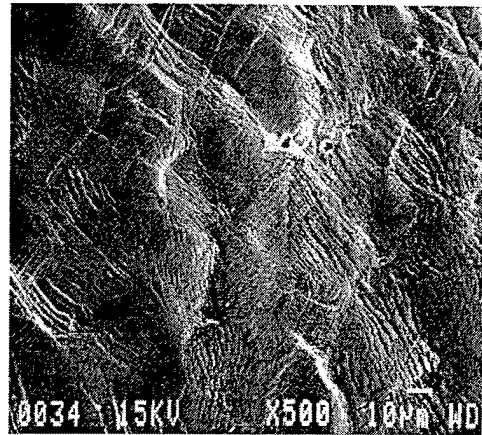
Figure 3.35 - SEM fracture of as-extruded Fe-15Al tested at 25°C
