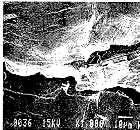
Figure 3.36 - SEM fracture of as-extruded Fe-15Al-2.8Si tested at 25°C
