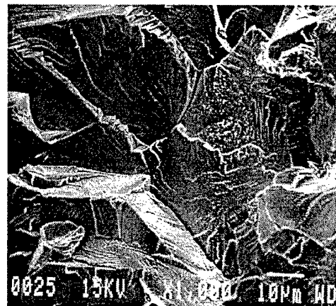
Figure 3.37 - SEM Fracture of as-extruded Fe-15Al-5Si tested at 25°C
