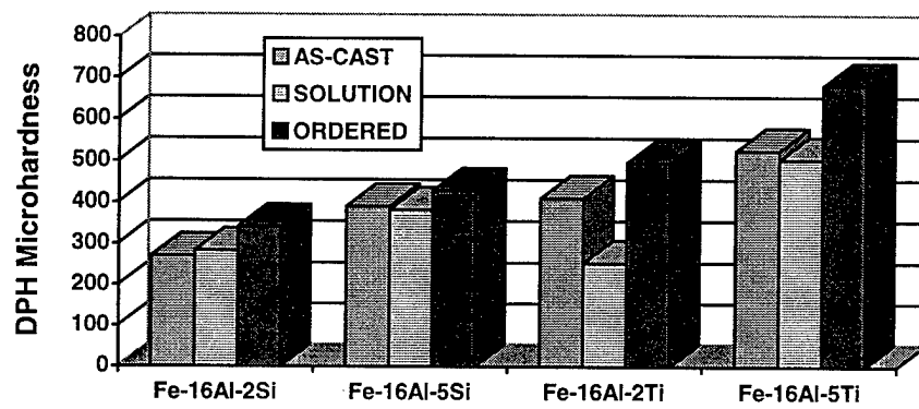
Figure 3.2 - Microhardness of Fe-Al-(Si,Ti) arc melted buttons
