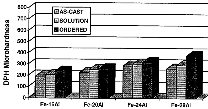
Figure 3.1 - Microhardness of Fe-Al arc melted buttons
