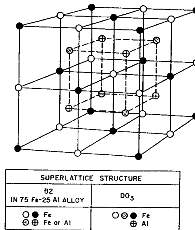
Figure 1.3 - Crystal structure of FeAl (B2) and Fe 3 Al (DO 3 ) [21]
