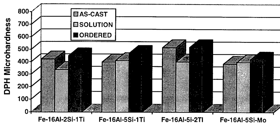
Figure 3.3 - Microhardness of Fe-16Al-Si-Ti arc melted buttons
