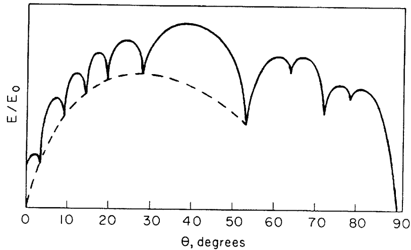
Figure 1.11 - Low energy grain boundary configurations for CLS boundaries [41]
