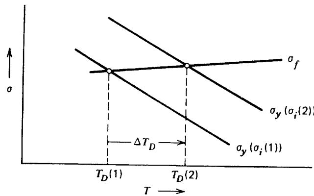
Figure 1.12 - Fracture strength and yield strength as a function of temperature [49]
