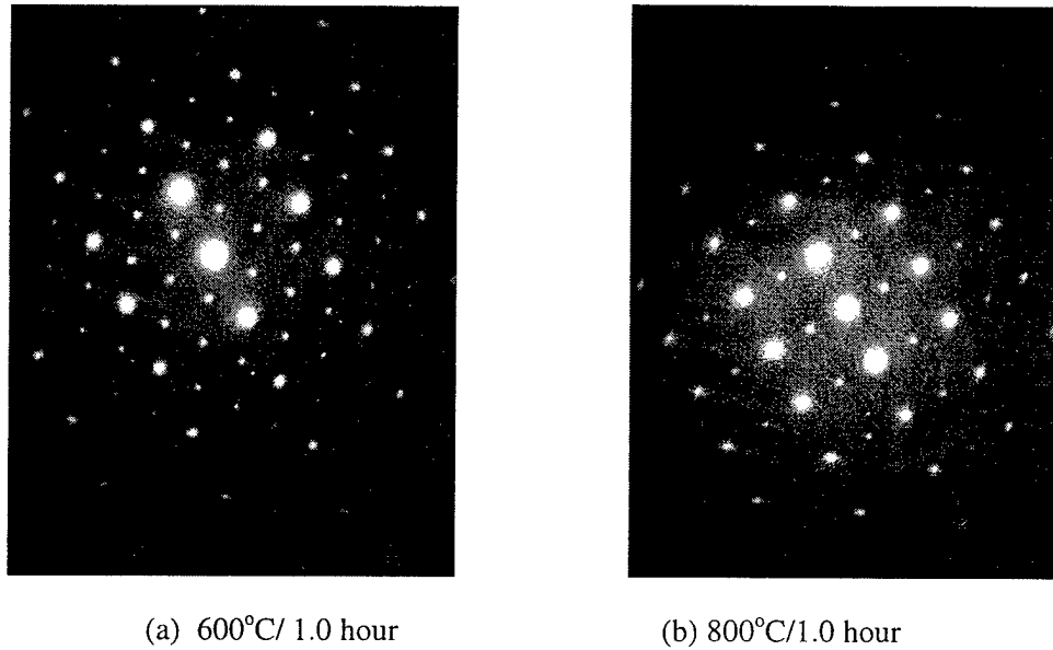
Figure 3.28 - SAD patterns of 110 zone axis for Fe-15Al-5Si indicating \text{DO}_3 \rightarrow \text{B2} transition
