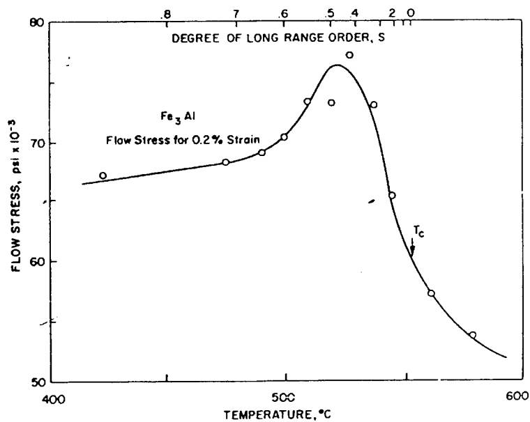
Figure 1.7- Flow stress of \text{Fe}_3\text{Al} at test temperature [23]
