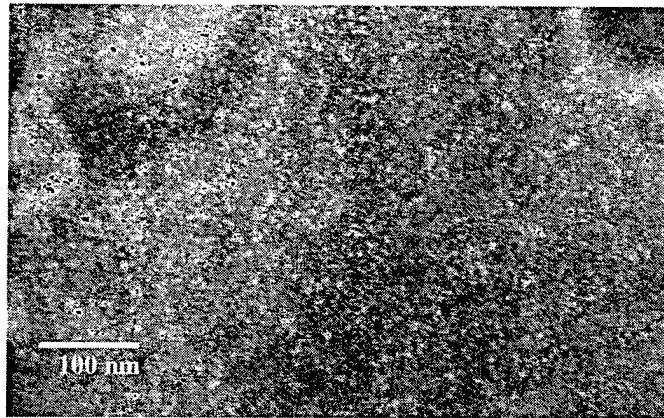
Figure 3.25 - TEM dark field image ( g = 111 ) \text{DO}_3 regions in as-extruded Fe-15Al-2.8Si
