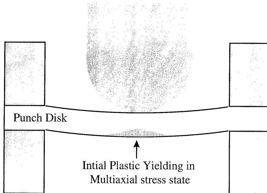
Figure 4.6 - Punch disk volume plastically deformed at yield strength
