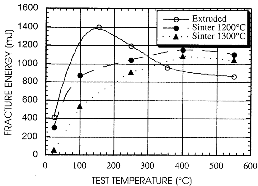
Figure 3.34 - Effect of processing on fracture energy Fe-15Al-2.8 Si powders (HT: 600°C)
