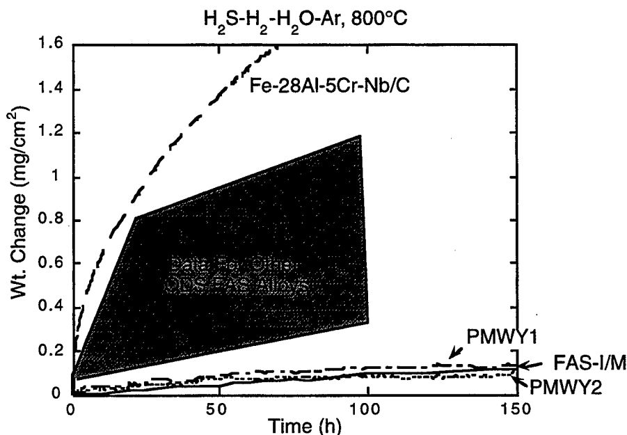
Fig. 7. Weight change versus time for specimens isothermally exposed to \text{H}_2\text{S-H}_2\text{-H}_2\text{O-Ar} at 800^\circ\text{C} . The PMWY alloys are FAS- \text{Y}_2\text{O}_3 produced from commercially prepared powders and were exposed in the as-recrystallized condition. The specimen designated FAS-I/M was produced by ingot metallurgy processing and represents the benchmark behavior in this environment. The \text{Fe}_3\text{Al} - 5\% \text{Cr} alloy was also produced by ingot metallurgy and contains 1% Nb and 0.2% C. The shaded area represents the range of data reported previously (see ref. 9) for as-extruded FAS and FAS- \text{Y}_2\text{O}_3 prepared from laboratory-produced powder mixtures.
