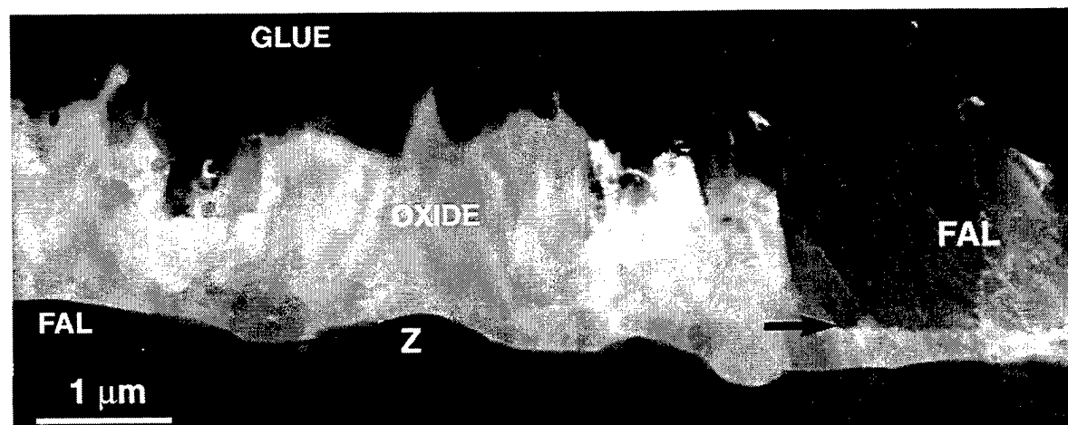
Fig. 7 STEM annular dark-field of coated-and-oxidized FAL. The location of the original coating is indicated by the arrow.
