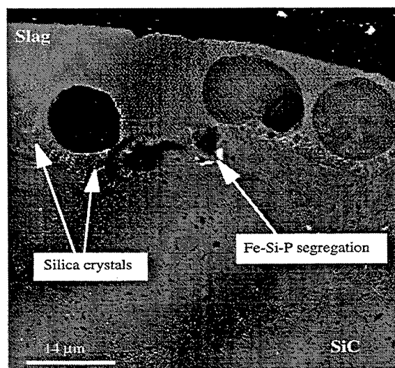
Fig. 16. Backscattered image of the slag/SiC interface for a specimen exposed to Baldwin slag at 1430°C.
