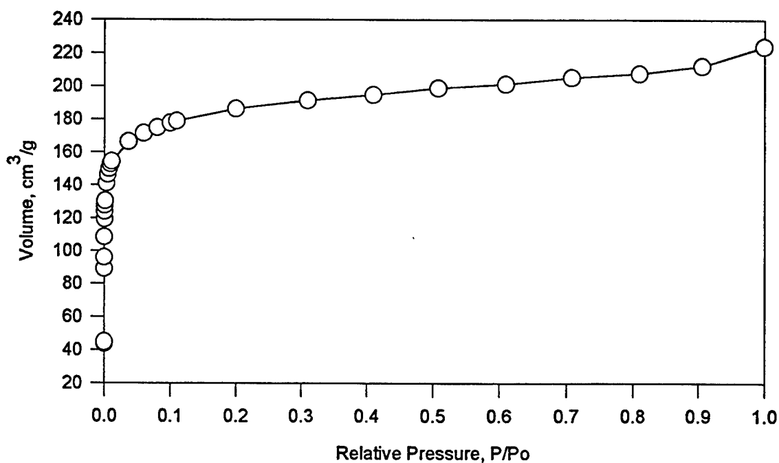
Figure 1. Typical 77K \text{N}_2 isotherm for sample SMW8A
