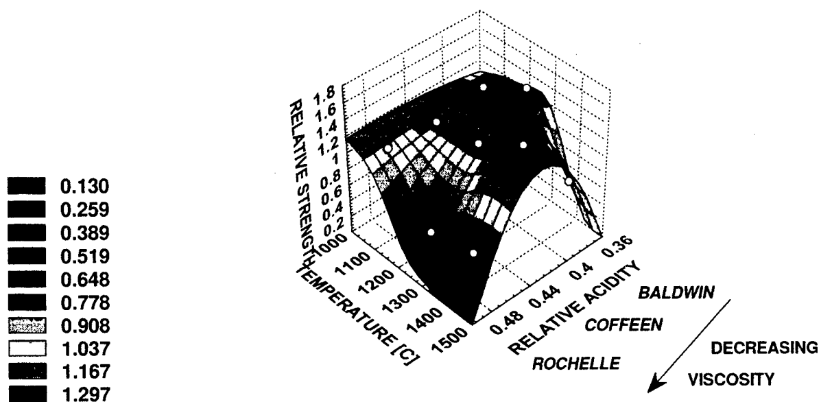
Fig. 5. Relative retained strength for the sintered \alpha -Si specimens after exposure for 500 h.
