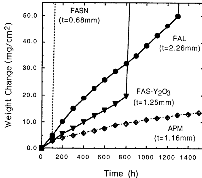
Fig. 4. Total weight gain (specimen + spall) for 100-h cycles at 1300°C in laboratory air. Starting specimen thicknesses ( t ) are noted.
