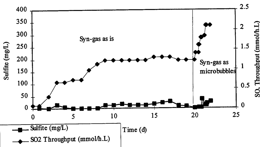
Figure 2: Biodesulfurization of SO x using coal synthesis gas as a carbon and energy source. The rate of desulfurization has been markedly increased by the introduction of synthesis gas as microbubbles rather than conventional gas sparging.
