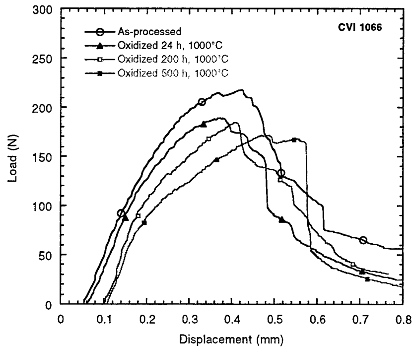
Fig. 3. Load vs displacement curves for a CVI 1066 (C/Al 2 O 3 -TiO 2 -C interface) composite as-processed and after oxidation at 1000°C for up to 500 h in air
