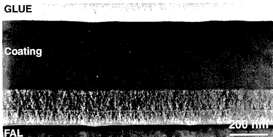
Fig. 1 TEM image of the structure of an as-deposited alumina coating (~ 0.7 \mu\text{m} thick).
