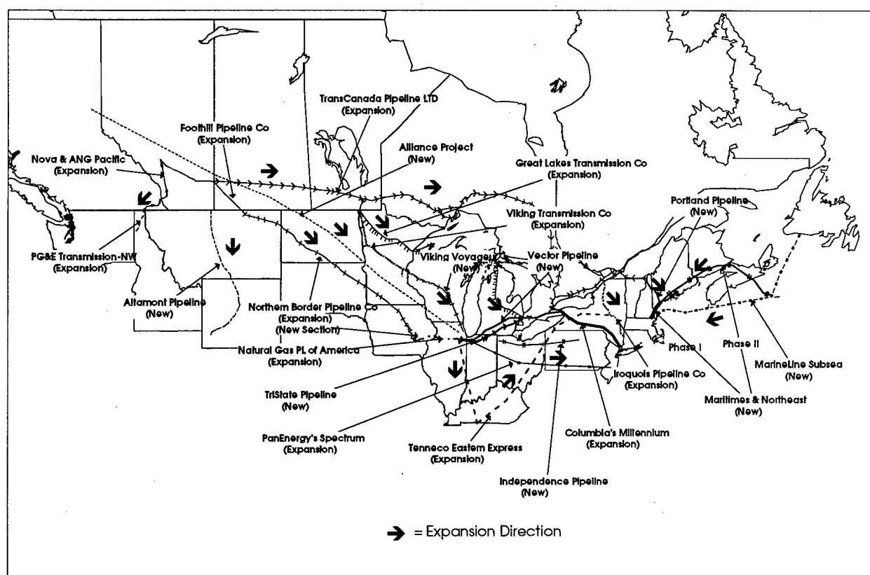
Figure B3. Planned Projects Related to Imports of Canadian Gas, 1998-2000
