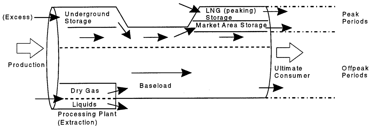
Figure 1. Generalized Schematic of Natural Gas Pipeline Transmission
