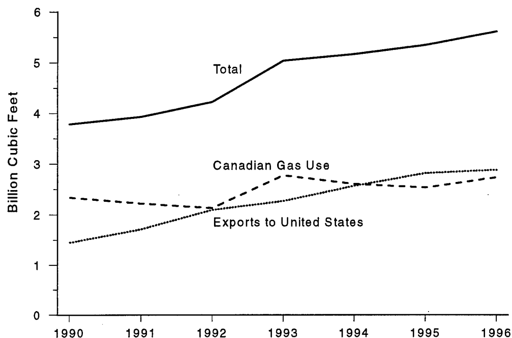
Figure 6. Canadian Gas Exports to the United States and Total Canadian Gas Production, 1990-1996
