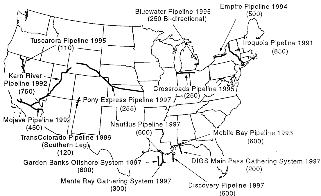
Figure 10. Capacity of New Natural Gas Pipeline Systems Placed in Service in the United States Between 1990 and 1997
