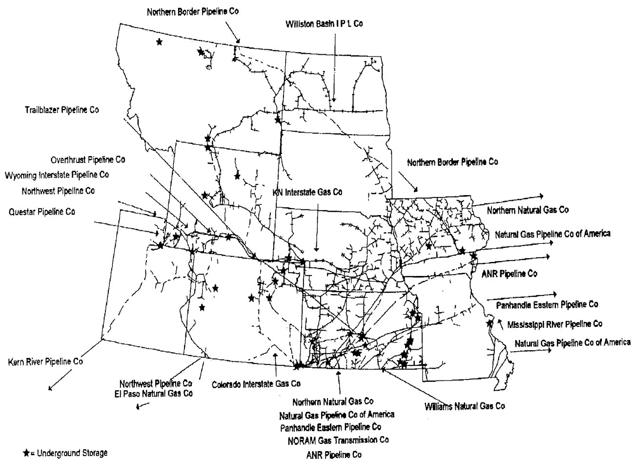
Figure A1. Major Interstate Natural Gas Pipelines in the Central Region
