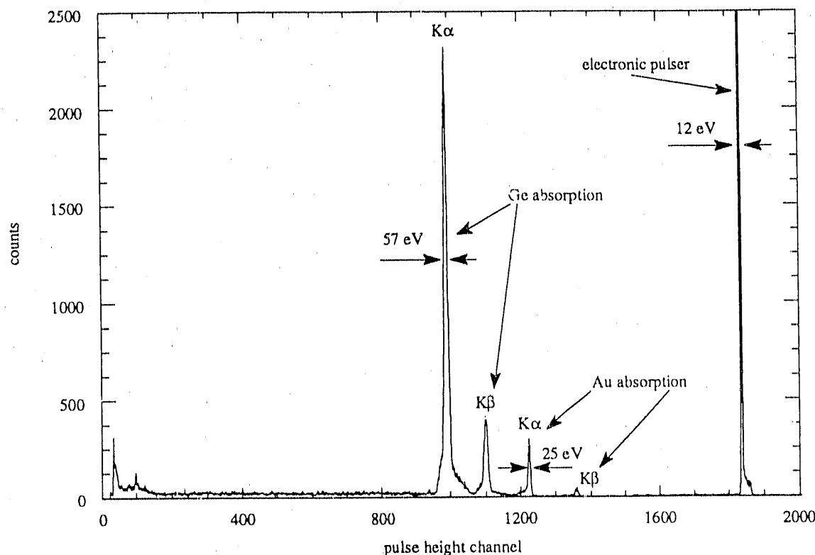
Figure 1. An x-ray spectrum obtained with an NTD germanium calorimeter 100 \mu\text{m} x 100 \mu\text{m} x 250 \mu\text{m} long operating at 0.1 K. The detector was illuminated with Mn K\alpha and K\beta x-rays giving rise to the four peaks in the center of the figure. The peak on the far right is from an electronic pulser which is used to measure the electronic noise. The 25 eV FWHM resolution indicated by the Au absorption peak includes contributions from the Mn K\alpha_1 and K\alpha_2 lines. Accounting for these two lines within the peak shown yields an actual energy resolution of 19 eV.
