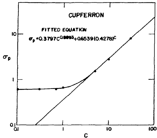
Fig. A-7. Standard deviation of calculated pCi/24-h sample vs observed counts per minute.
