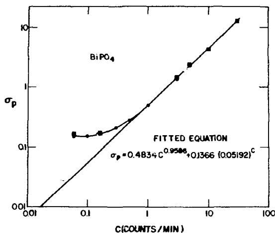
Fig. A-8. Computed values of \sigma_p vs C.
