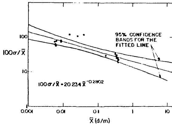
Fig. B-1. Mean vs relative standard deviation for NTA method.
