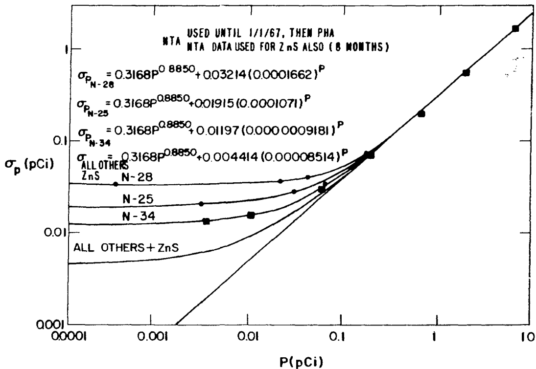
Fig. B-2. Computed values of \sigma_p vs P .
