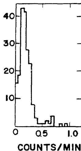
Fig. A-2. Frequency distribution of BiPO 4 ppt. blanks.
