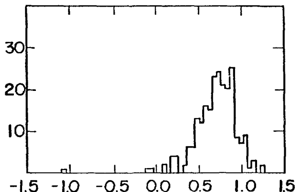
Fig. A-4. Fractional \text{BiPO}_4 -ppt. recovery.
