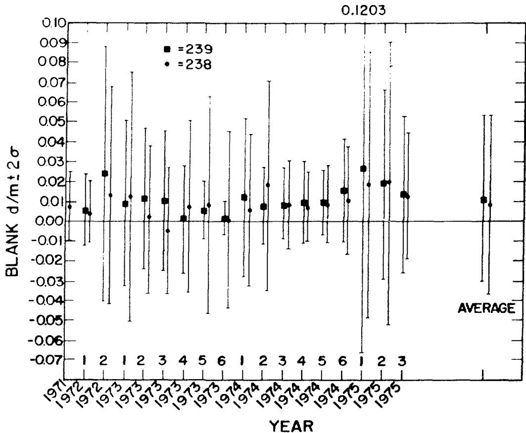
Fig. C-1. Average blank \pm 2 \sigma vs time.
