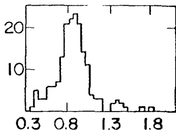
Fig. A-3. Fractional cupferron recovery.
