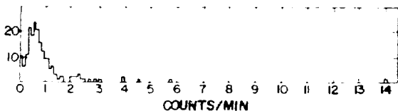
Fig. A-1. Frequency distribution of cupferron blanks.
