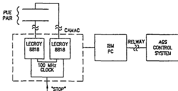
Fig. 1. IBCM digitizing hardware configuration.
