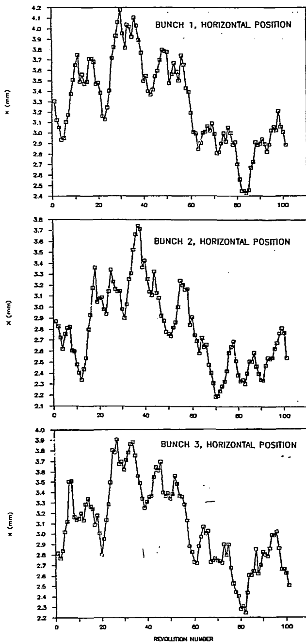
Fig. 2. Horizontal coordinates of successive bucket passings at 210 ms.
