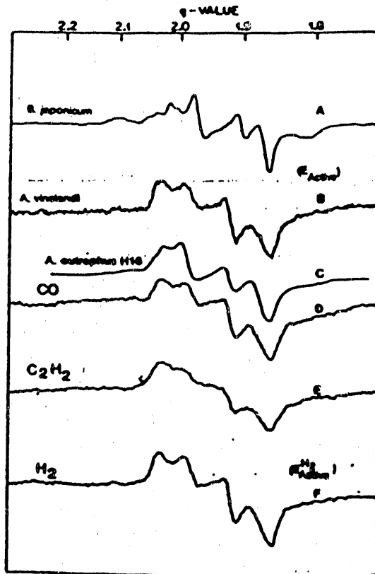
Fig. 2. EPR Spectra of NiFe Hydrogenases
