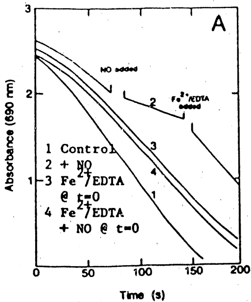
Figure 1 NO (5 \mu M) Reversibly Inhibits Membrane-associated Hydrogenase H_2 Oxidation Activity
