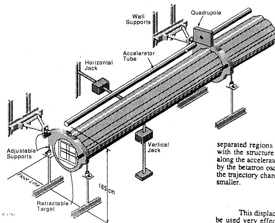
Fig. 2 Schematic view of position jacks to produce offsets in the center of the girders. The position of the end supports holding the quadrupoles remains fixed.
