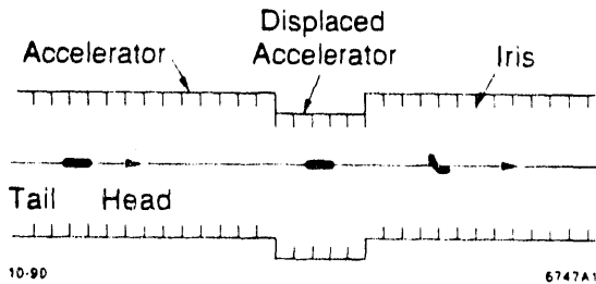
Fig. 1 Displaced accelerator structures produce wakefields effects.
