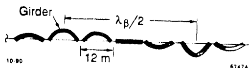
Fig. 3 Use of distorted accelerator girders to make structure offsets at the betatron spatial frequency.
