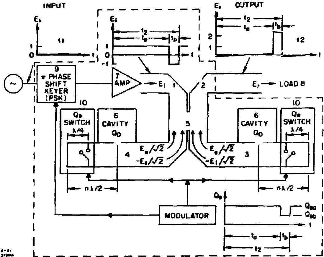
Fig. 6. REC system using 9-dB hybrids.
