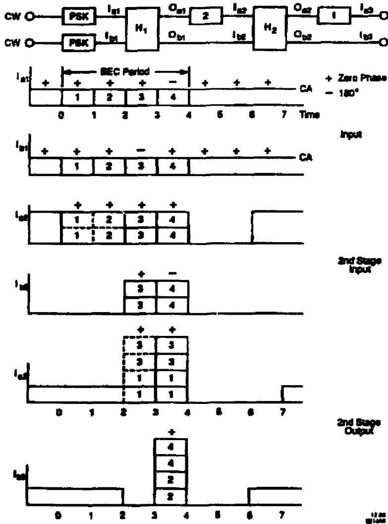
Fig. 2. 2-Stage BEC Coding.
