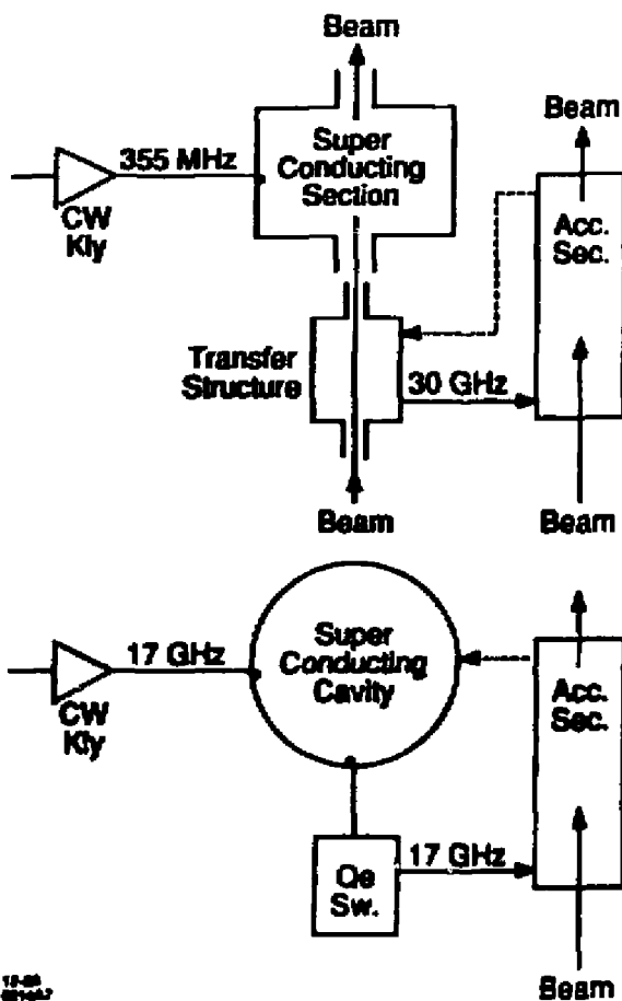
Fig. 7. Comparison of REC and CLIC SYSTEMS.
