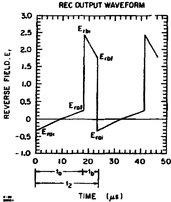
Fig. 5. Typical REC output waveforms.
