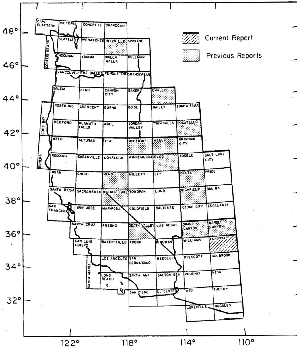
FIGURE 1. Location Map for the Flagstaff 1° x 2° NTMS Quadrangle
