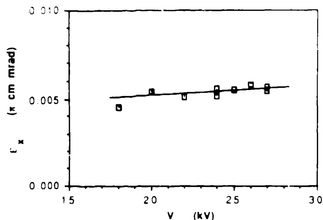
Fig 3 \epsilon_x vs V for the SAS. These measurements are for I_d held constant at 120 A. The line is a guide to the eye.
