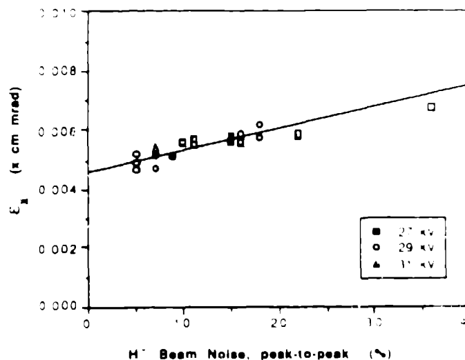
Fig 5 The rms emittance, \epsilon_x , vs the H^- beam noise at three different extraction voltages (inset) for the 4X source. The line through the data is primarily a guide to the eye, but it implies a 1.7% increase in emittance for each \pm 1\% of beam noise. Thus, operation at the lowest noise is desirable, and can be achieved as described in the text.
