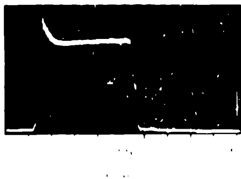
Fig. 1. The photograph of a 27\text{-keV} , 80\text{-mA} pulsed H^- beam from a 0.25\text{-cm} diam emitter. The I_d = 12 \text{ A} . The bandwidth in the H^- current pulse is 1 \text{ MHz} .
