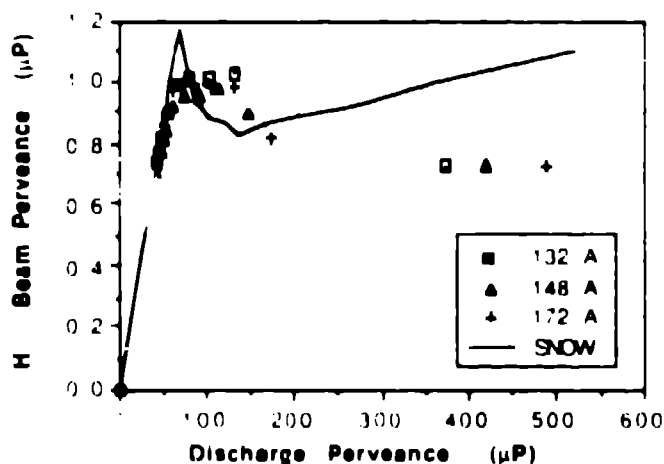
Fig. 7 The measured electron equivalent H^- beam perveance ( \mu P ) vs the discharge perveance ( \mu P ) for the 4X source. The data are for three different discharge currents (inset). Also plotted on the same graph is the SNOW simulation of the 4X source target perveance vs. the injection perveance.
