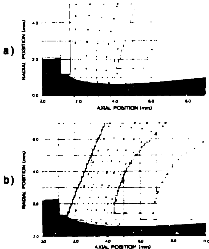
Fig. 6 a) SNOW simulation for the SAS circular extraction system b) SNOW simulation for the 4X source circular extraction system
