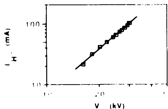
Fig. 2. The extracted H^- current, I_{H^-} , vs the extraction voltage, V , at 12 \text{ A} discharge in the SAS. The error is about \pm 3\% for I_{H^-} .
