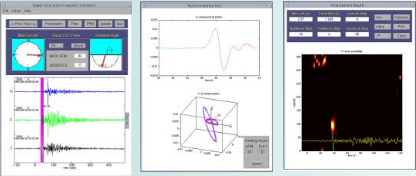
New capabilities for DOE’s SAC2000 computer code include an interactive tool that improves the analyst’s ability to detect and identify seismic phases. It allows users to pick phases and rotate signals (left), filter the data, interactively analyze three-component particle motions (center), and compute maximum-likelihood probabilities for selected wavetypes (right). The tool has helped solve problems such as incorrect sensor orientation.
