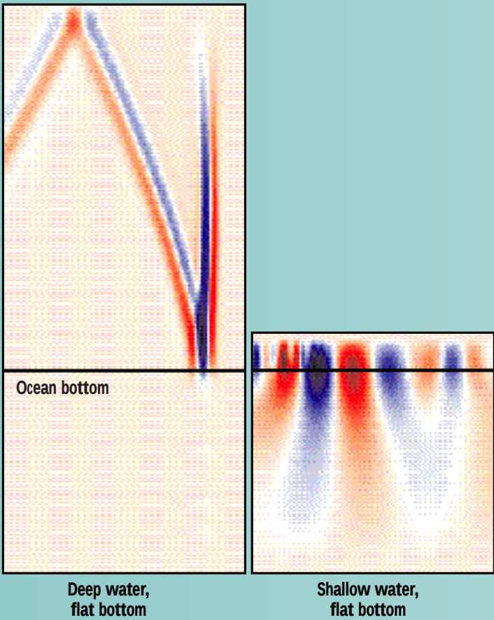
Ocean depth can have a large effect on the source signal of an underwater explosion. Here, in two wavefield “snapshots” for explosions in deep and in shallow water, the colors show the amplitude of the propagating wave. Note that the shallow-water case has a significantly different appearance and that more energy couples into the ocean bottom.
