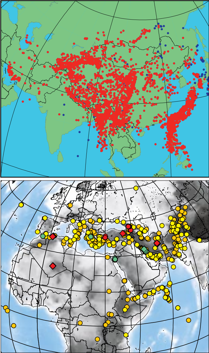
Phase 1 of the DOE seismic reference-event data set is complete. The locations of reference events for Asia and the Middle East/ North Africa that will be included in the initial version of the Knowledge Base are shown. Each dot represents a single event; the color represents further information on the event, for example, the type of information that was used to constrain the location. Developing these extensive reference-event data sets is required before the correction surfaces for the location and identification algorithms can be calculated.
