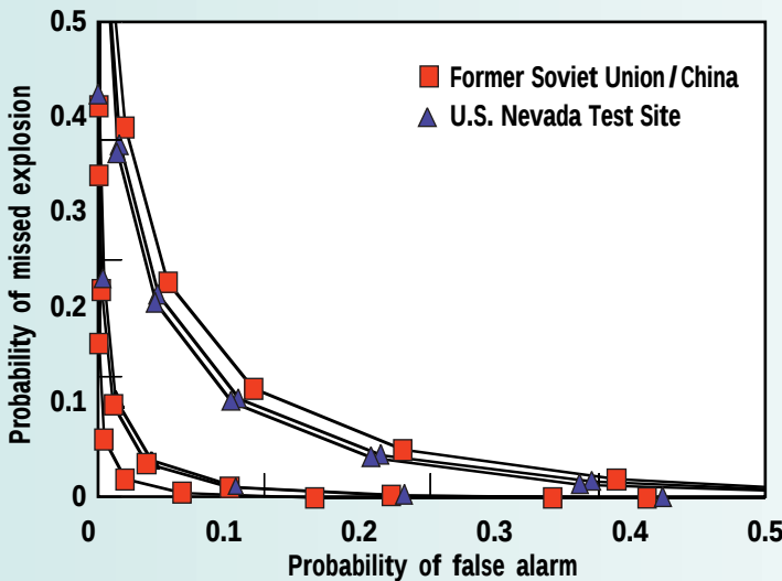
The goal for identification algorithms is to be able to differentiate between explosions and earthquakes in uncharacterized regions as well as we can at the well-characterized U.S. Nevada Test Site. Our algorithms based on ratios of seismic wave phases reach this goal. Here, application of three different algorithms to events in the Former Soviet Union and China (recorded at station WMQ in China), presented as curves showing the tradeoff between missed explosions and false alarms, gives results close to those at the Nevada Test Site.
