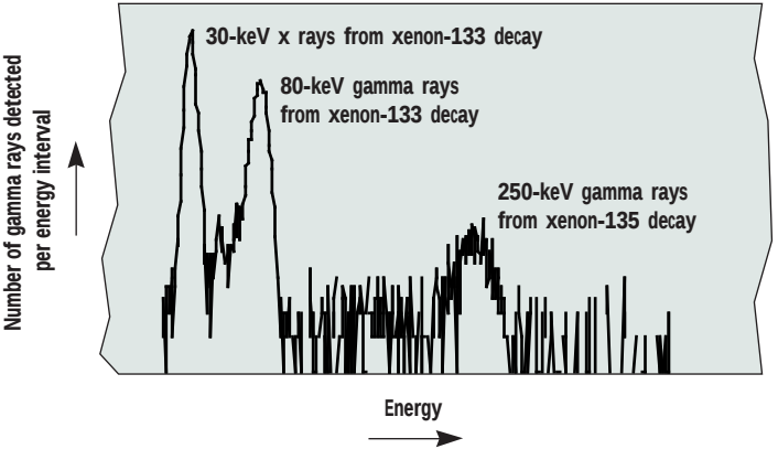
An example gamma-ray spectrum of radioactive isotopes of xenon gas detected by the Automated Radioxenon Sampler/Analyzer demonstrates its sensitivity. The system is able to detect and identify gamma rays even from xenon-135, which has a half-life of only 9 hours. The xenon-135/xenon-133 ratio is useful in distinguishing nuclear explosion debris from reactor releases.
