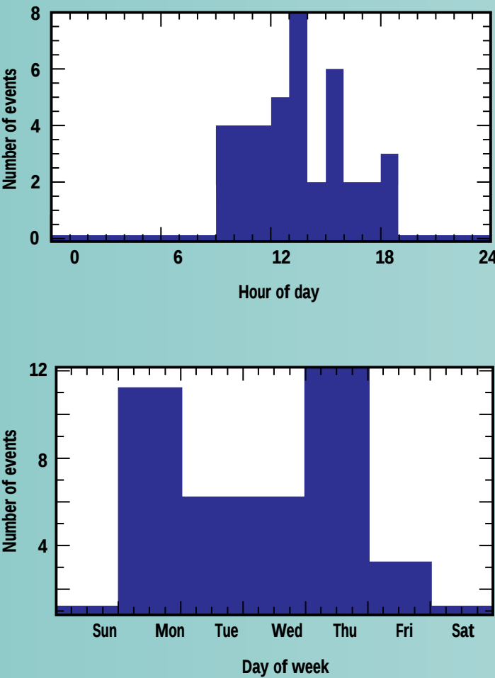
Mining explosions are useful reference events, but in regions with limited access, the challenge is to know which events are from mines. We know that mining explosions tend to occur at the same times of day. Cluster analysis reveals time patterns that are typical of mining practices in the region.
