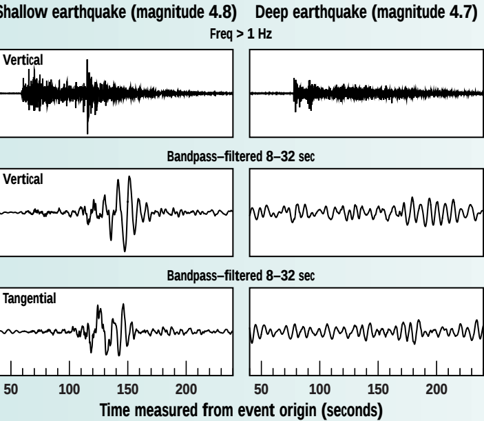
Identification using algorithms that incorporate shear-wave-blockage data must also consider other types of phenomena that can be mistaken for blockage. For example, we have found that some seismic waveforms that seemingly reveal blockage are actually produced by very deep seismic events under certain conditions. Here, two earthquakes with similar magnitudes recorded at station WMQ in China show very different waveforms—the deep-earthquake signal has no shear-wave component (the large amplitude in the center of the shallow-earthquake signal).
