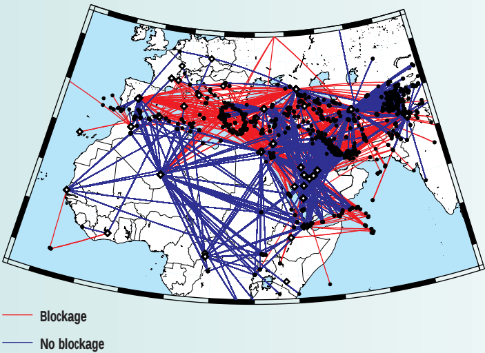
Seismic shear waves, a critical parameter in event identification, can be blocked by regional geologic structures. Analysis of these blockages allows us to determine which stations are the best to monitor a given region.
