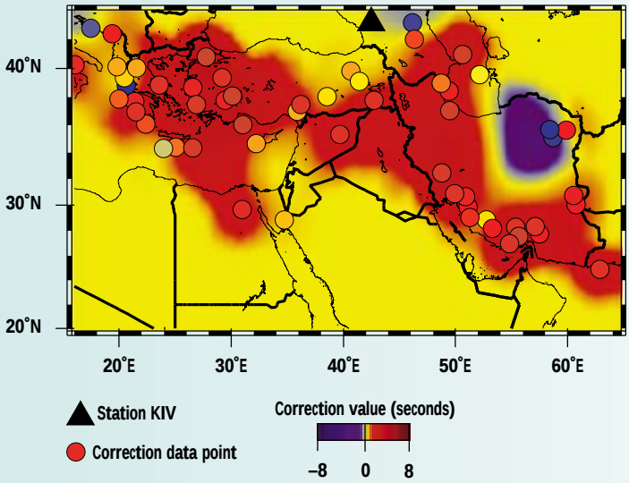
Region- and station-specific corrections to seismic-signal travel times are represented as correction surfaces in the Knowledge Base. In our preliminary correction surface for a subregion of the Middle East for seismic station KIV, the colored dots show the data and the color variations from red to blue show the values, in seconds, for the correction surface. Values read off this surface are used to correct the arrival times of seismic events at KIV that are used as input into event-location algorithms. We will develop similar correction surfaces for all of the key monitoring stations in our regions of interest.
