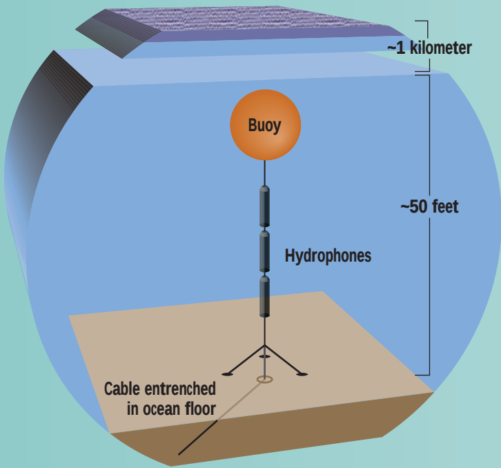
Existing sensor technology for the ocean-monitoring system meets CTBT requirements. At a typical hydrophone station, the sensors float above the ocean floor at a depth of about 1 kilometer.
