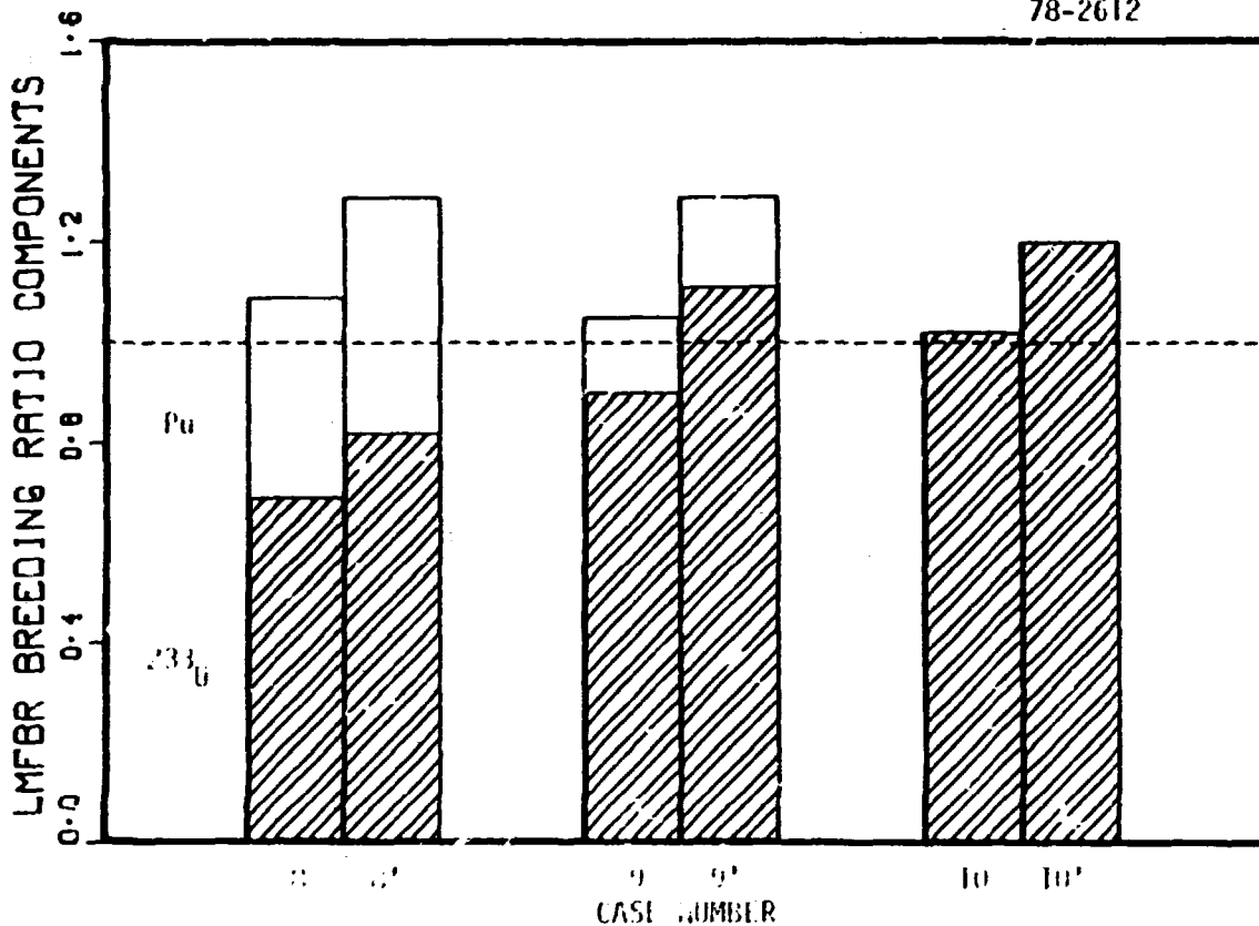
Fig. 4.6-1. Breeding Ratio Components for LMFBRs Operating on ^{233}\text{U} . (Cases 8,8' for 20\% ^{233}\text{U}/\text{U} , and Cases 9,9' for 40\% ^{233}\text{U}/\text{U} ; Cases 10,10' for ^{233}\text{U}/\text{Th} with no ^{235}\text{U} ; see Tables 4.6-1 and 4.6-1.)
