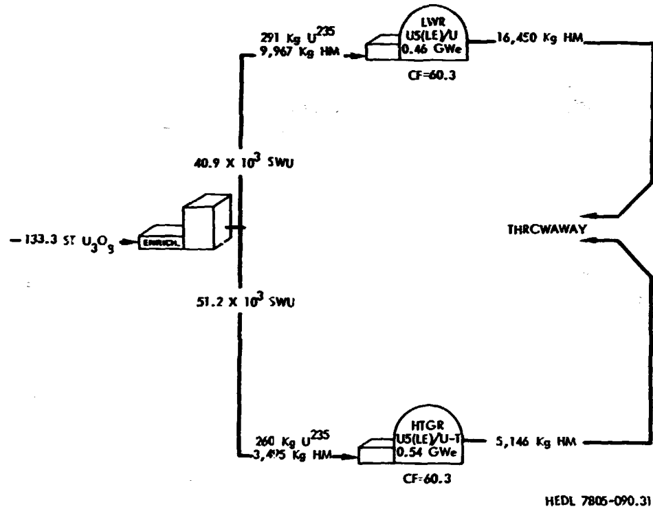
(c) Case 1G: LWRs Followed by HTGRs; High-Cost U_3O_8 Supply.
