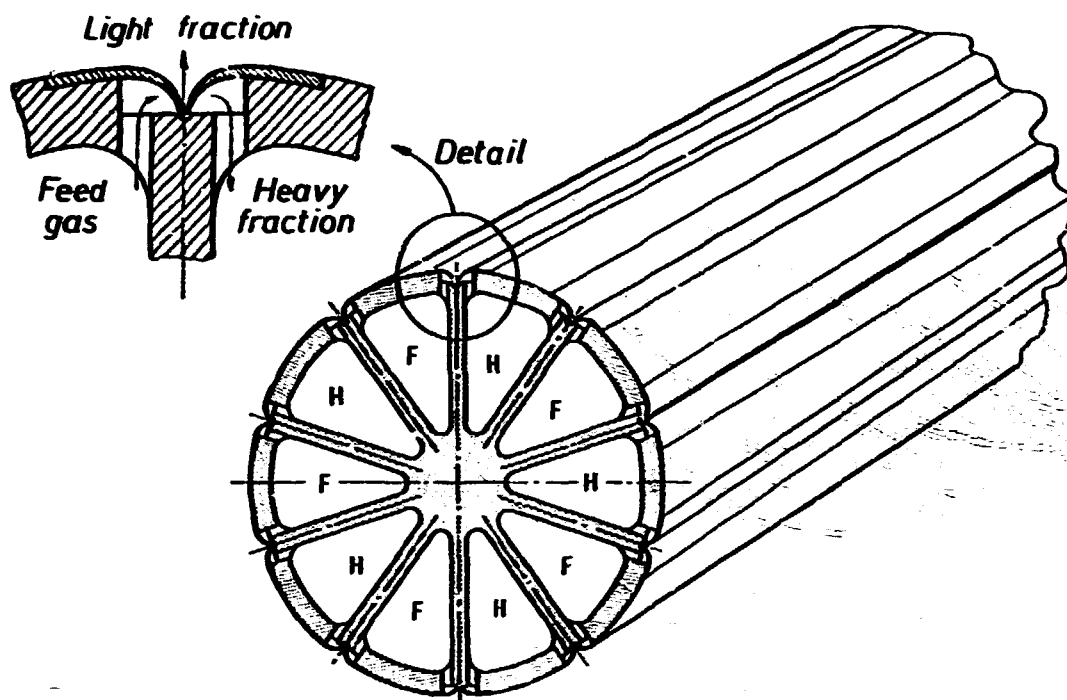
Fig. A-3. Becker Separating Element With Ten Slits
