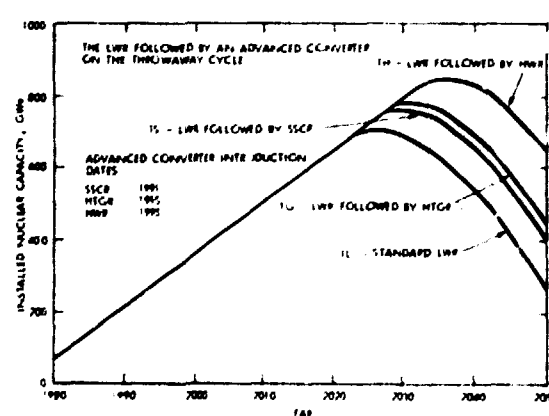
Fig. 6.2-7. The Effect on the Nuclear Contribution of Adding Advanced Converters on the Throwaway Cycle (Intermediate-Cost U_3O_8 Supply).
