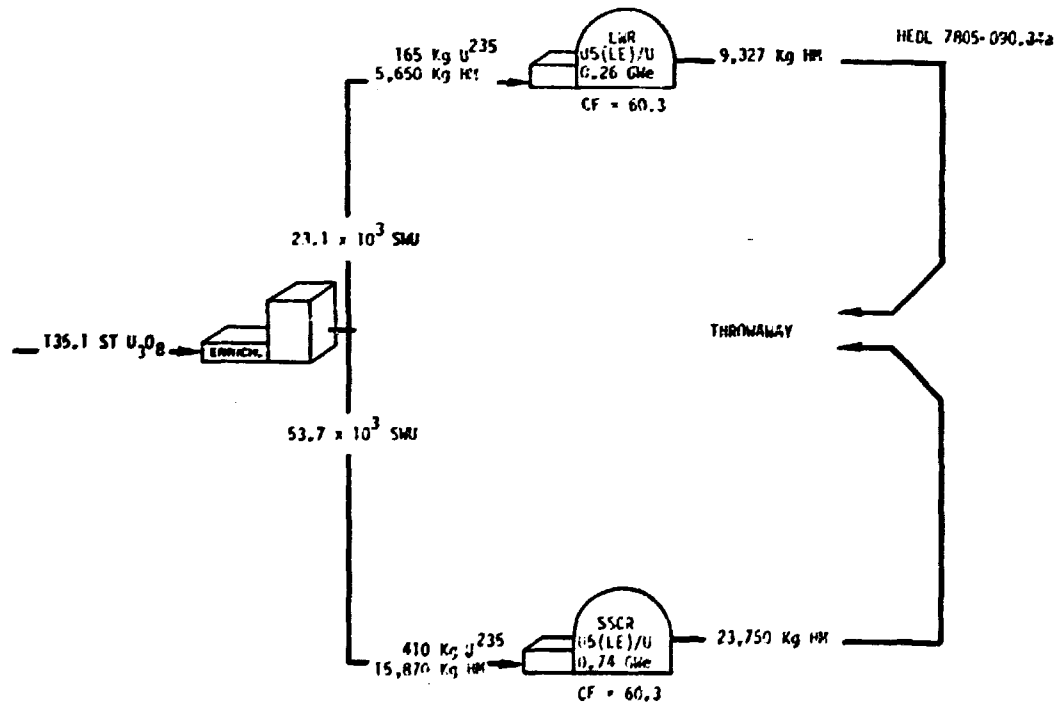
(b) Case 1S: LWRs Followed by SSCRs; High-Cost U_3O_8 Supply.
