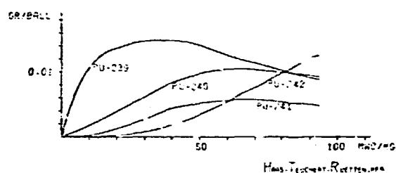
Fig. 4.4-1. Buildup of the Plutonium Isotopic Composition in the HEU/Th Fuel.
