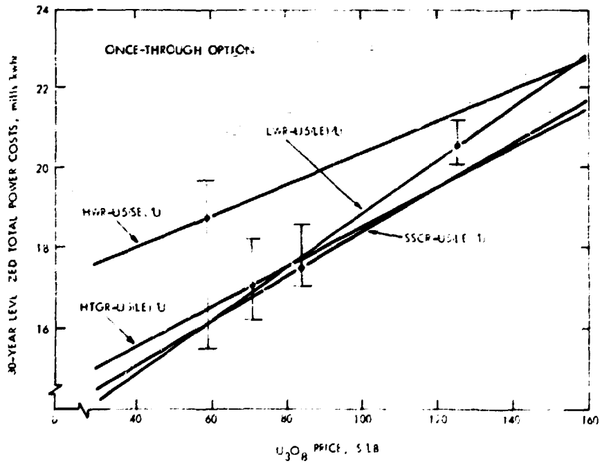
Fig. 6.1-9. Total Power Cost of Various Reactor Systems as a Function of U_3O_8 Price (Constant U_3O_8 Price with Once-Through Option).
