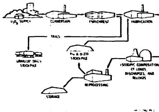
Fig. 6.1-6. Nuclear Fuel-Cycle Model.
