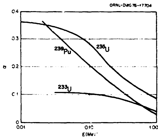
Fig. 4.0-1. Nuclear Parameters of the Principal Fissile and Fertile Nuclides at High Neutron Energies. \alpha = \sigma_c/\sigma_f ; \eta = \nu/(1 + \alpha) .
