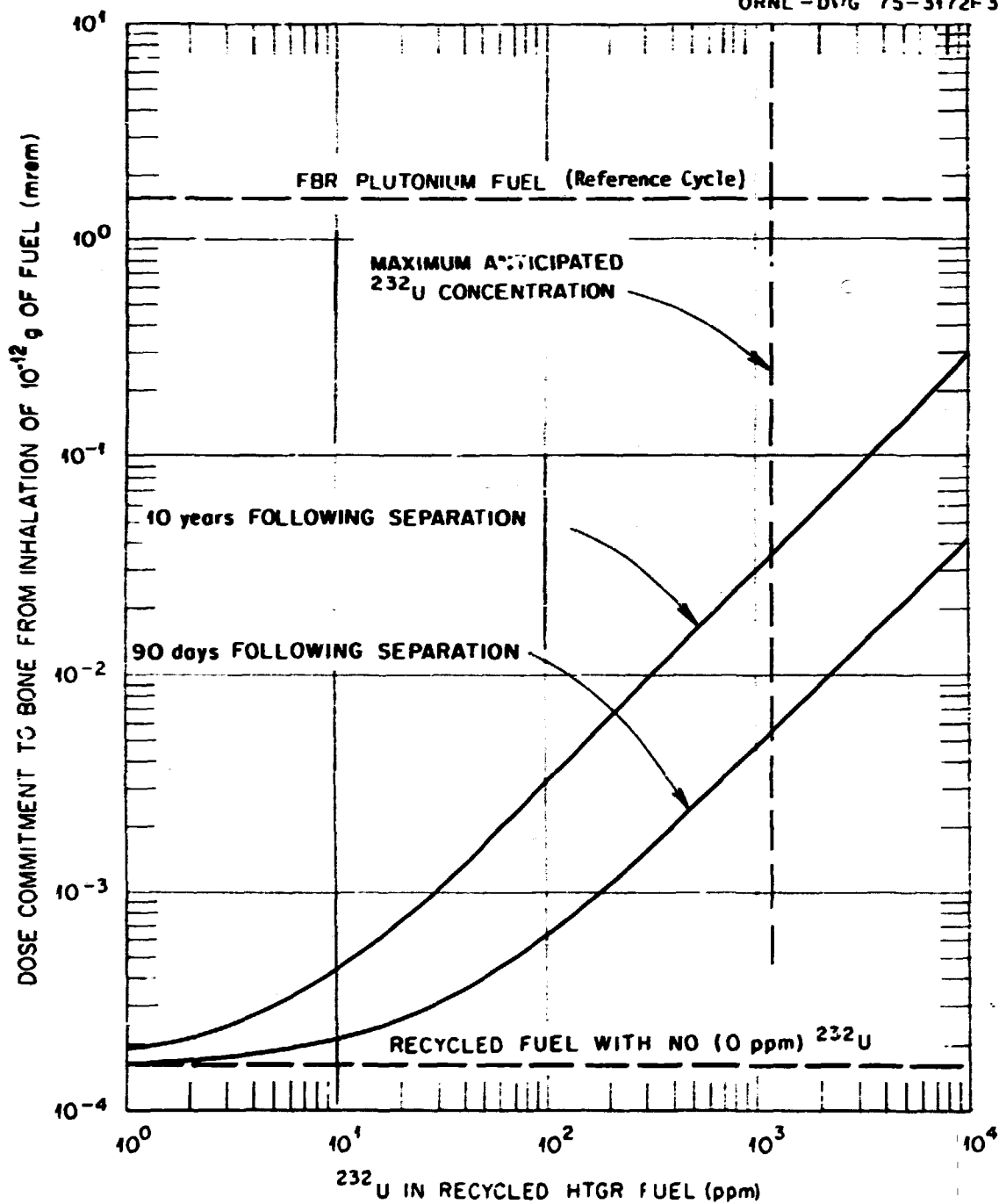
Fig. 3.2-1. Effect of ^{232}\text{U} Concentrations in HTGR Fuel (93% ^{235}\text{U}/\text{U} ) on Dose Commitment to Bone.
