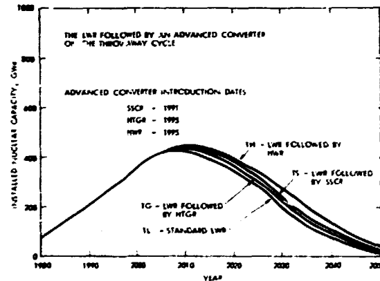
Fig. 6.2-5. The Effect on the Nuclear Contribution of Adding Advanced Converters on the Throwaway Cycle (High-Cost U_3O_8 Supply).
