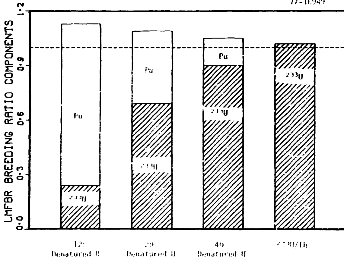
Fig. 4.5-1. Mid-Equilibrium Cycle Breeding Ratio Isotopics for Denatured Oxide-Fueled LMFRs. (ORNL Cases 7, 8, 9, and 10 from Table 4.5-1)
