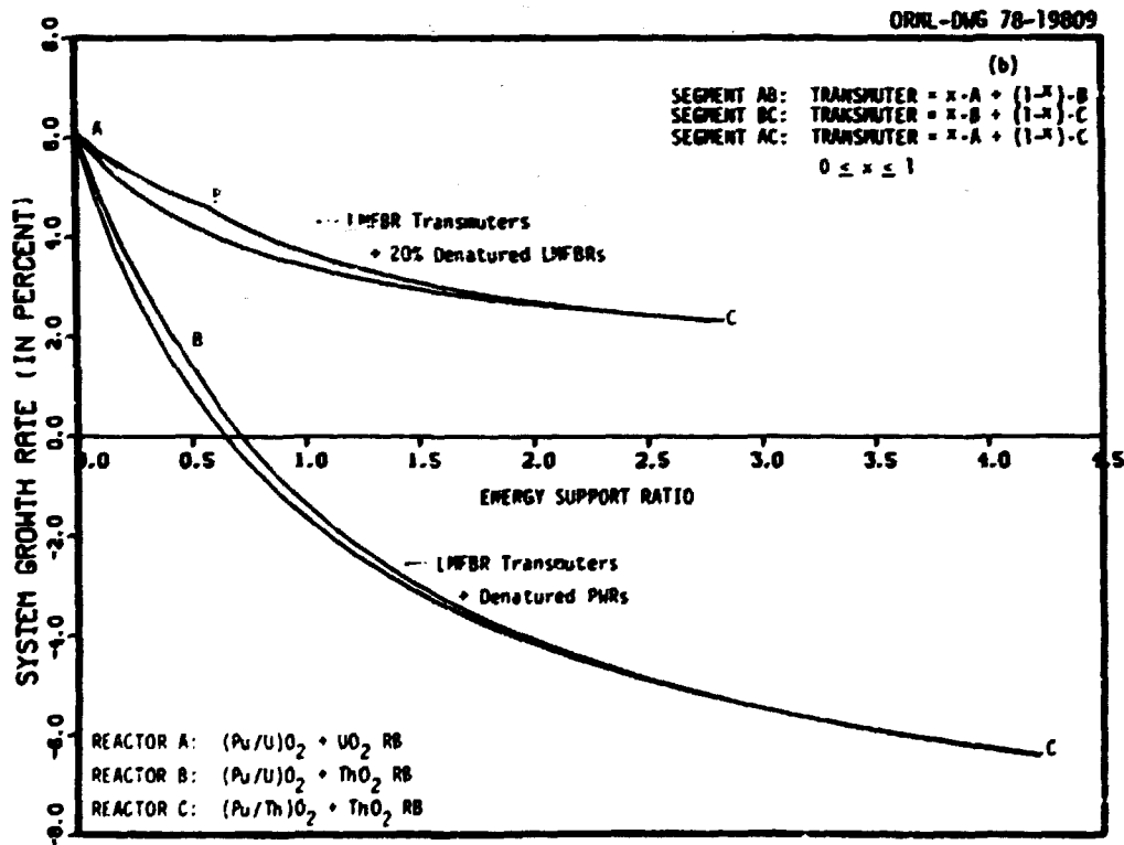
Fig. 7.2-1. Operating Envelopes for Symbiotic Systems Utilizing LMFBTR Transmuters.
