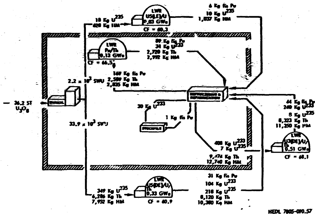
Fig. 6.2-24. Utilization and Movement of Fissile Material in an LWR Nuclear System Minimizing the Production and Use of Plutonium (Case SUL, High-Cost U_3O_8 Supply) (Year 2035).
