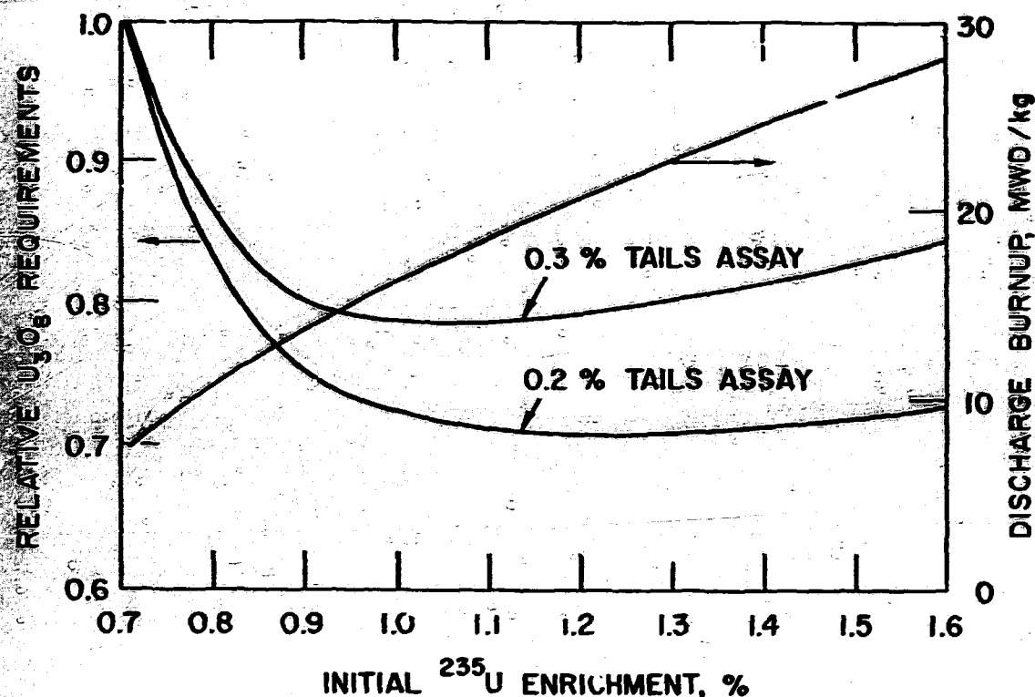
Fig. 4.3-1. Fuel Utilization Characteristics for Enriched-Uranium-Fueled CANDU.
