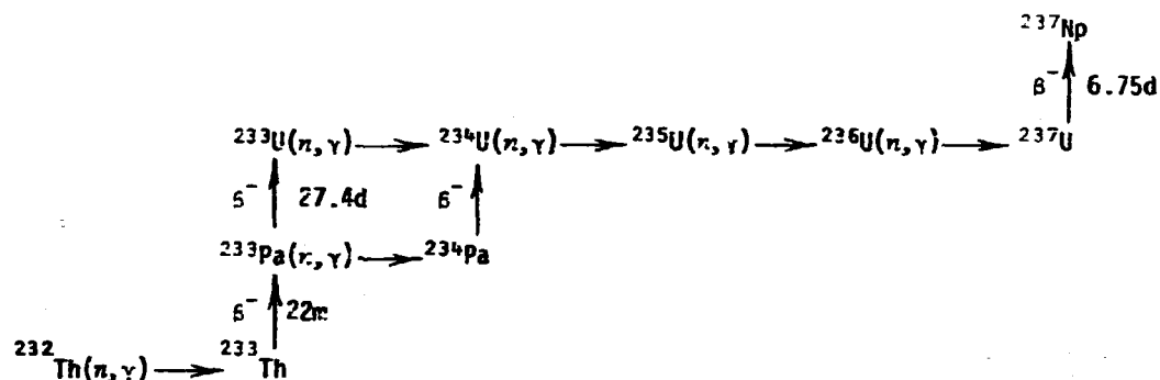
Fig. 4.0-2a. Nuclide Production Chain for ^{232}\text{Th} .
