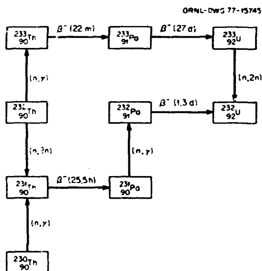
Fig. 3.1-1 Important Reaction Chains Leading to the Production of ^{232}\text{U} .
