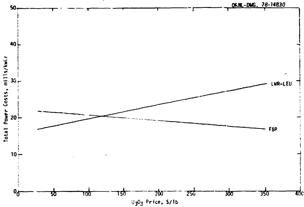
Fig. 6.1-8. Influence of U_3O_8 Price on Total Power Costs.
