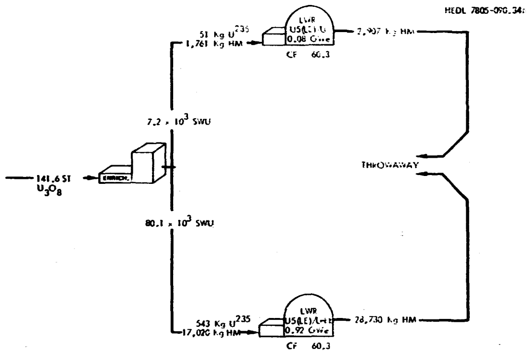
(a) Case 1L: LWRs Only; High-Cost U_3O_8 Supply.
