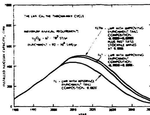
Fig. 6.2-9. The Effect of Enrichment Tails Composition on the Nuclear Contribution with the LWR on the Throwaway Cycle (High-Cost U_3O_8 Supply).
