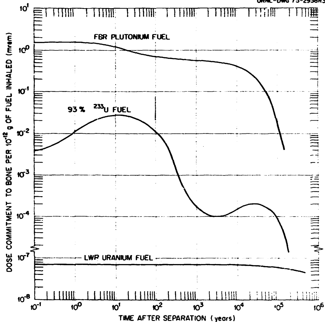
Fig. 3.2-2. Relative Radiotoxicity of FBR Plutonium Fuel, HTGR Fuel (93% ^{233}\text{U}/\text{U} ) and LWR Uranium Fuel as a Function of the Time after Separation at Reprocessing Plant.
