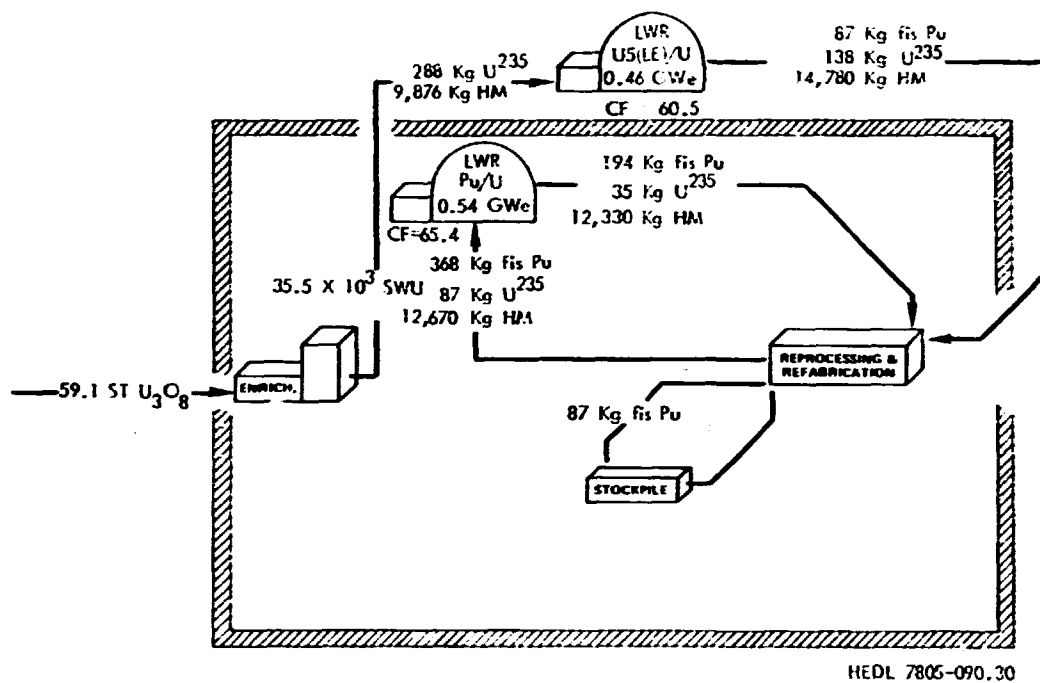
Fig. 6.2-16. Utilization and Movement of Fissile Material in a Nuclear System Consisting of LWRs Operating with Plutonium and/or Uranium Recycle (Case 2L, High-Cost U_3O_8 supply) (Year 2035).
