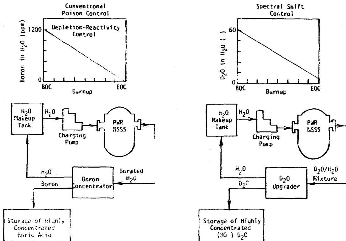
Fig. 4.2-1. Basic Spectral Shift Control Modifications.
