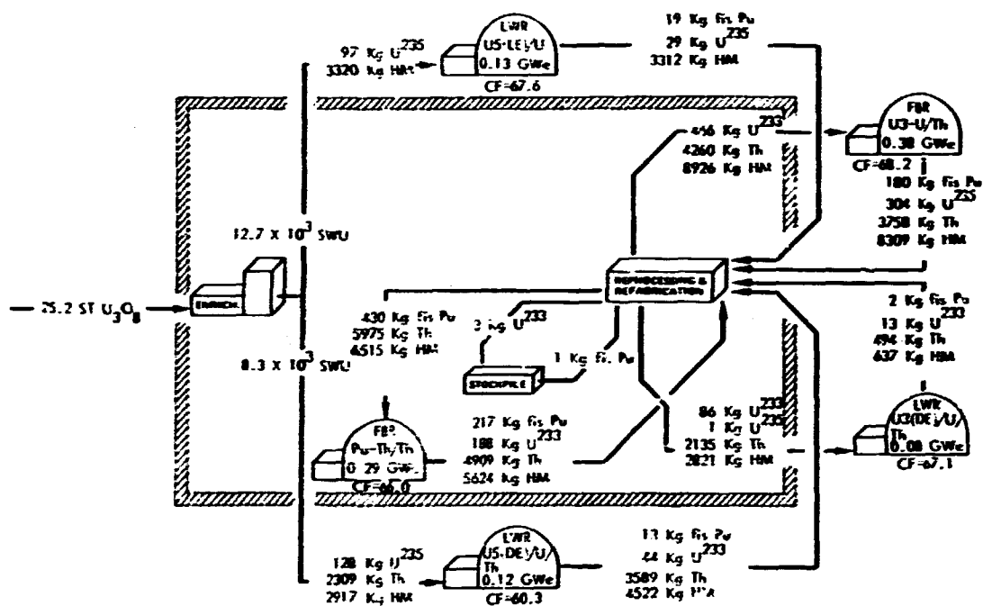
Fig. 6.2-35. Utilization and Movement of Fissile Material in an LWR-FBR Nuclear System with Heavy "Pu-to- 239 Pu". Transmutation Rate (Case 8L, high-Cost U_3O_8 Supply) (Year 2035).
