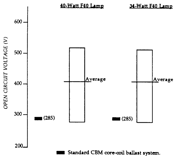
FIGURE 2.7 OPEN CIRCUIT VOLTAGE FOR ELECTRONIC BALLASTS OPERATING F40 LAMPS
