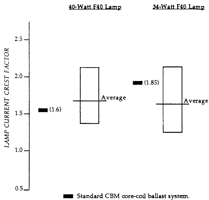
FIGURE 2.6 LAMP CURRENT CREST FACTOR FOR ELECTRONIC BALLASTS OPERATING F40 LAMPS
