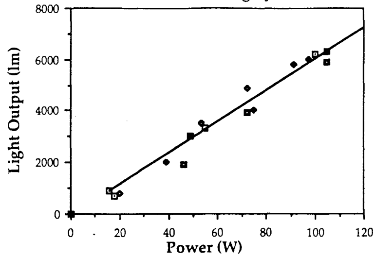
FIGURE 2.25 Light Output of 40W F40 Lamps With Core-Coil Dimming Systems
