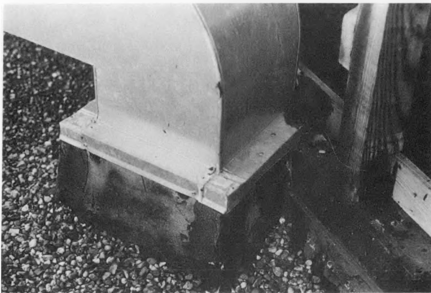
Figure 22. Modification of a Curb Supporting a Ventilator
