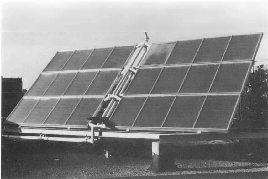
Figure C.5 Collector Frames Supported by Stub Columns
