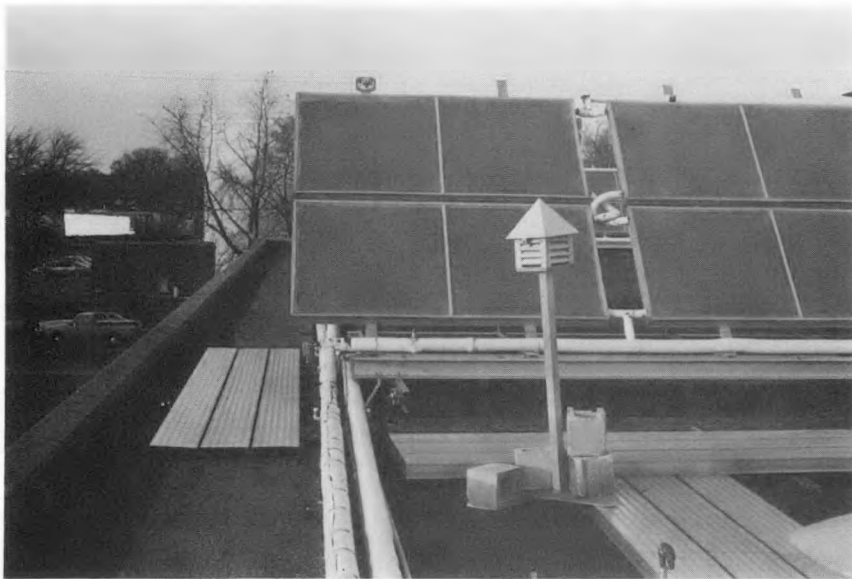
Figure C.32 Hollow Aluminum Sections Used as Walkways
