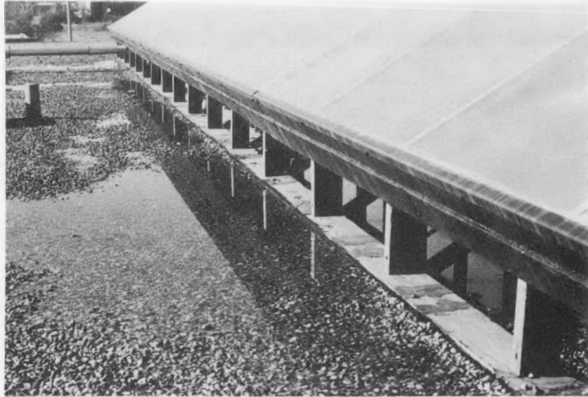
Figure C.11 Wooden Sleeper Mechanically Attached to Roof
