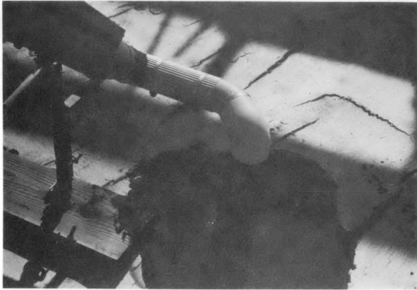
Figure C.15 Excessive Quantity of Asphalt Around Pipe Penetration With Undetermined Type of Flashing
