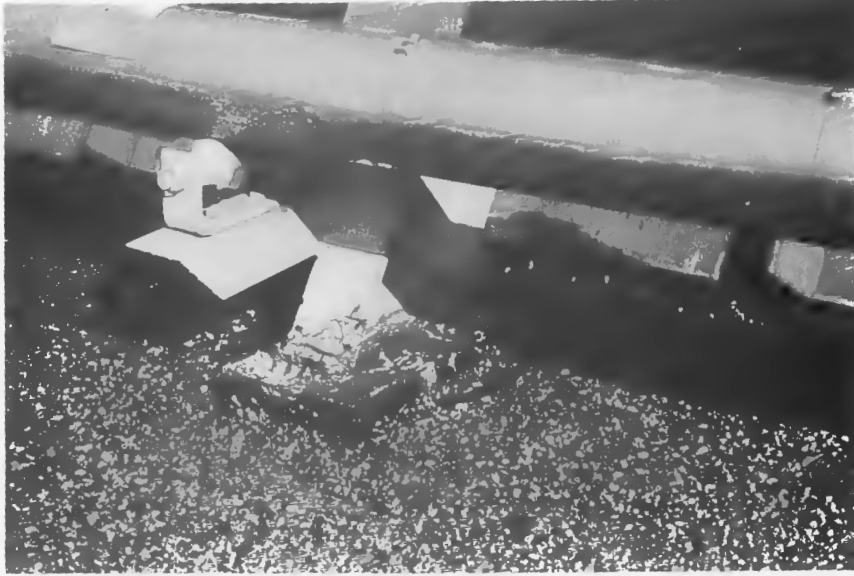
Figure C.25 Pipe Roller Support Attached to Collector Frame
