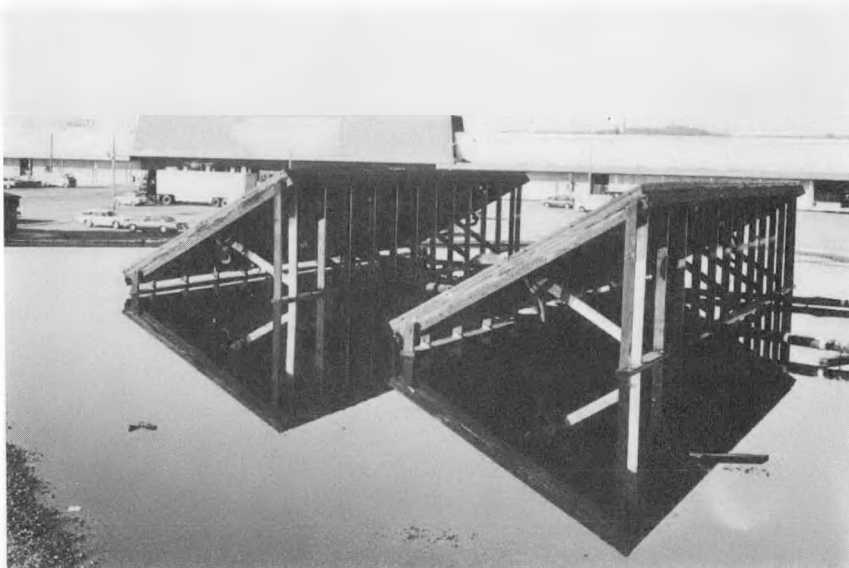
Figure C.2 Ponded Water Over 2 inches (50 mm) Deep Around Collectors
