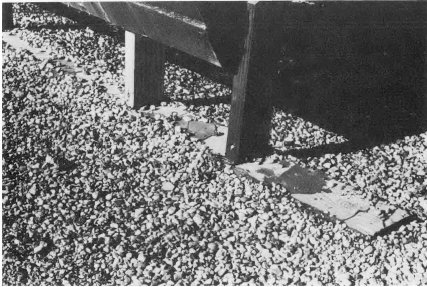
Figure C.13 Sleeper Which Had Sunk into Asphalt Flood Coat and Aggregate Surfacing
