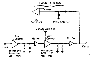
Fig. 4. IF active filter circuit.
