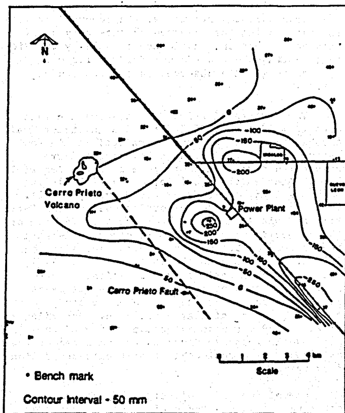
Figure 3. Surface elevation changes (in mm) between 1979 and 1981.
