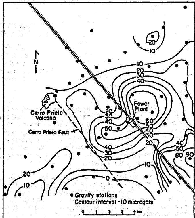
Figure 2. Gravity changes (in microgals) between 1979-1980 and 1980-81.
