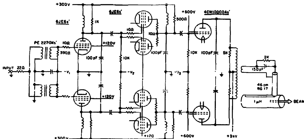
Fig. 6. Circuit diagram of the power amplifier.
