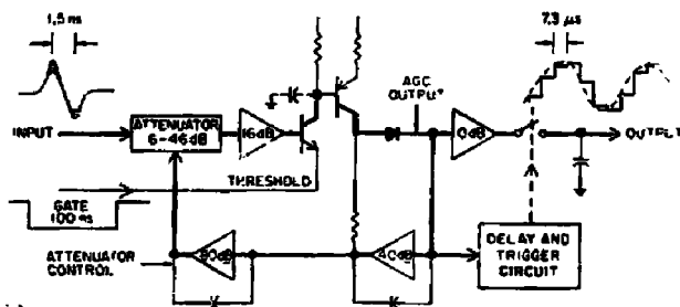
Fig. 2. Principle of the beam oscillation detection.
