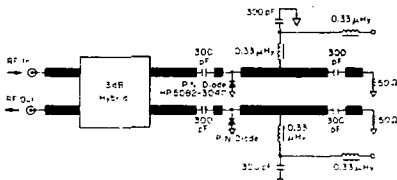
Fig. 10. Variable attenuator circuit diagram.
