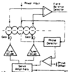
Fig. 1. Block diagram of the cavity servo loops.
