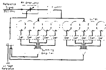
Fig. 8. Block diagram of the amplitude feedback loop.
