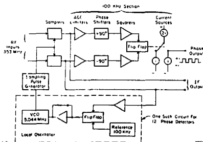
Fig. 5. Principle of the phase detectors.
