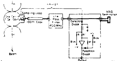
Fig. 9. RF amplitude detector circuit diagram.
