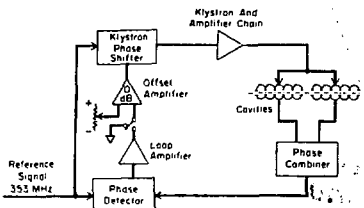
Fig. 4. Circuit of the phase control loop.
