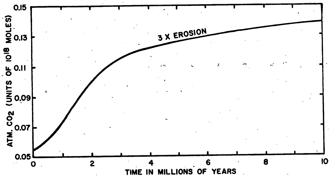
FIGURE 5 Increase in the CO 2 content of the atmosphere due to a threefold increase in the rate of erosion derived from Garrels et al. , 1976.
