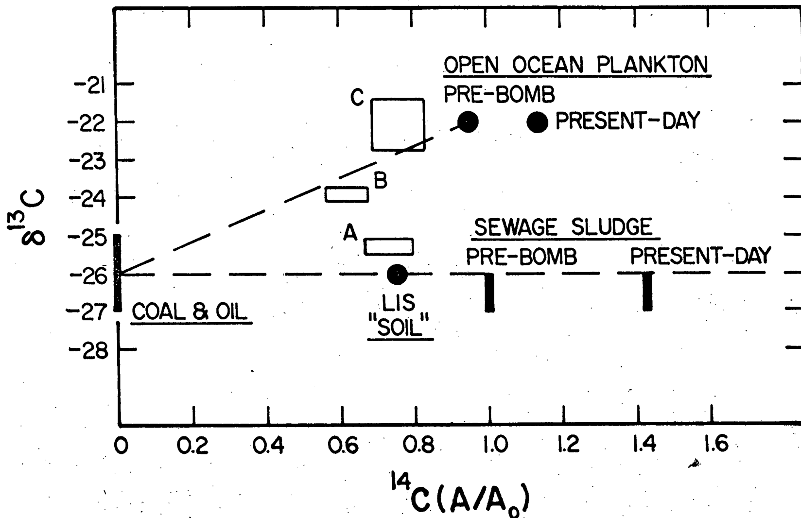
FIGURE 1 ^{13}\text{C} versus ^{14}\text{C} diagram for potential organic carbon sources to the New York Bight. The ^{14}\text{C} axis ( \text{A}/\text{A}_0 ) is the ratio of the specific activity (A) of the sample to 0.95 times the specific activity of NBS-1 oxalic acid ( \text{A}_0 ). The areas marked A, B, and C are the three sites in the New York Bight identified in Table 2.
