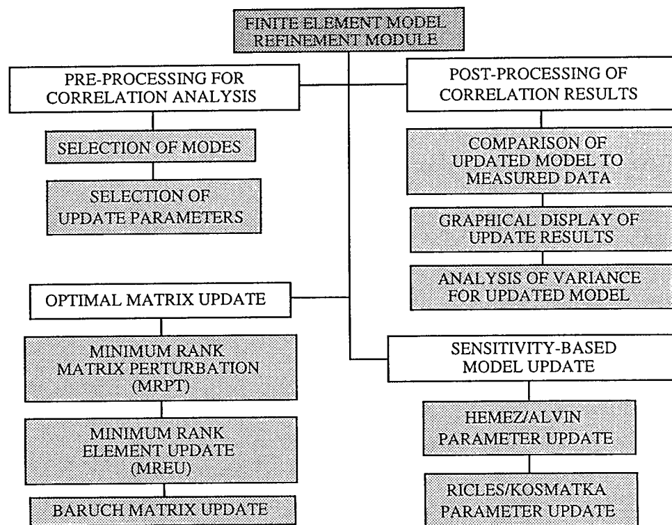
Figure 4: Flowchart of Finite Element Model Refinement Module
