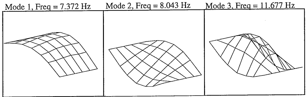
Figure 7: Identified Mode Shapes for Alamosa Canyon Bridge
