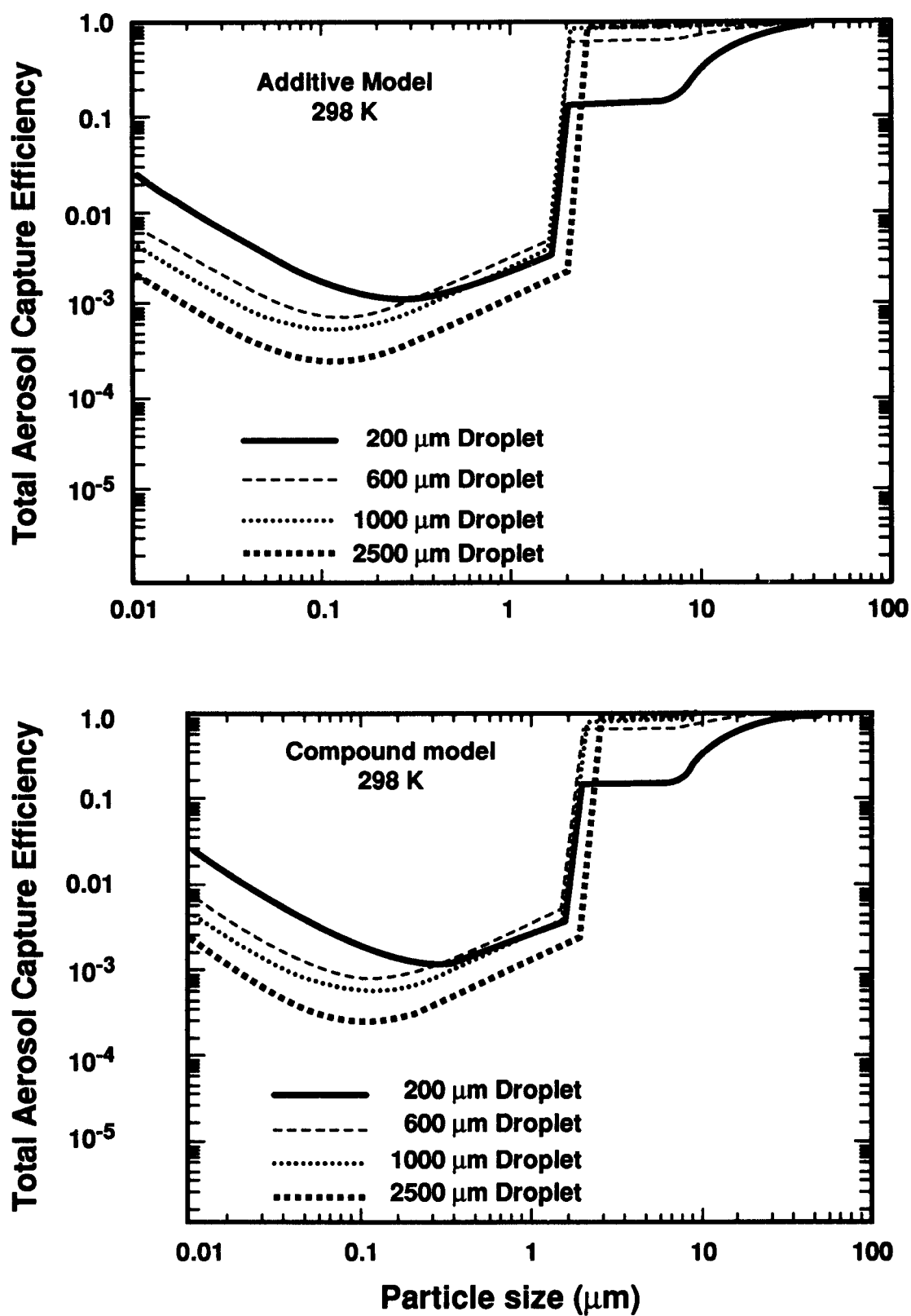
Figure 19 \epsilon'(\text{total}) , the compound model, and \epsilon(\text{total}) , the additive model, as functions of aerosol particle size and water drop size
